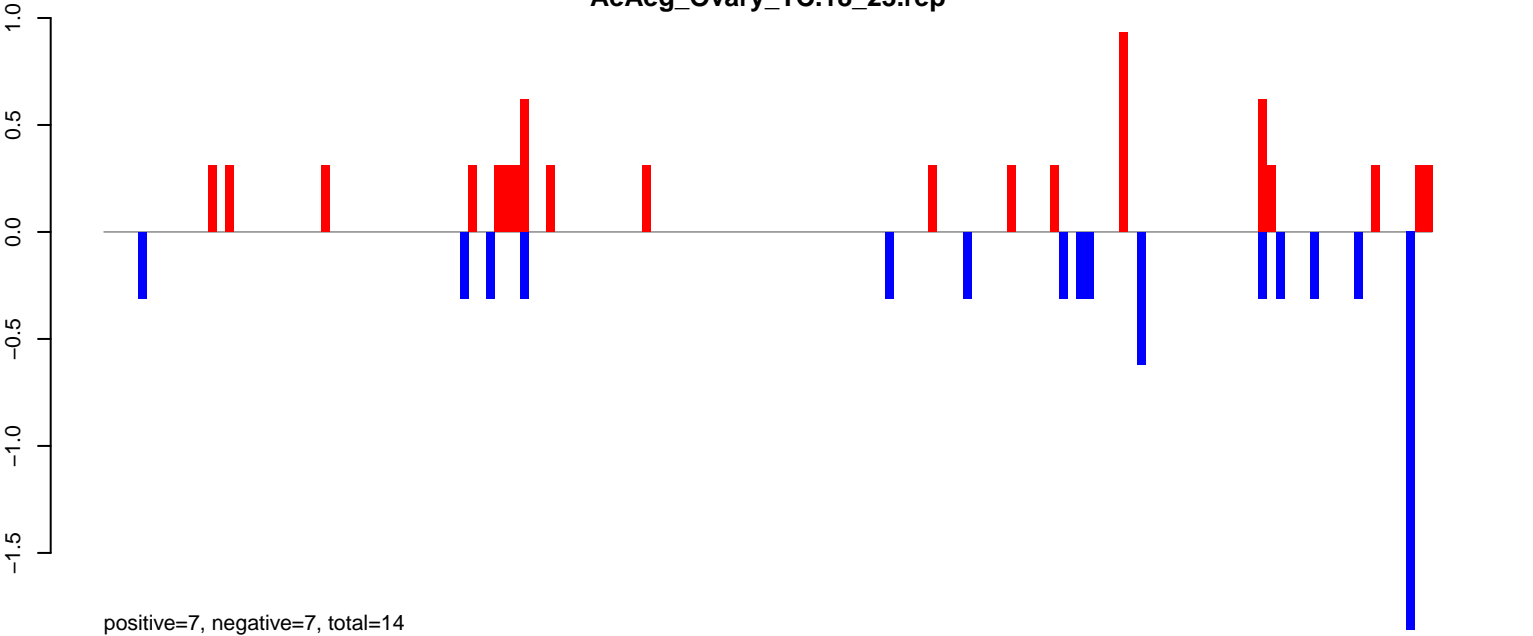
AeAeg_Ovary_TC.24_35.rep
