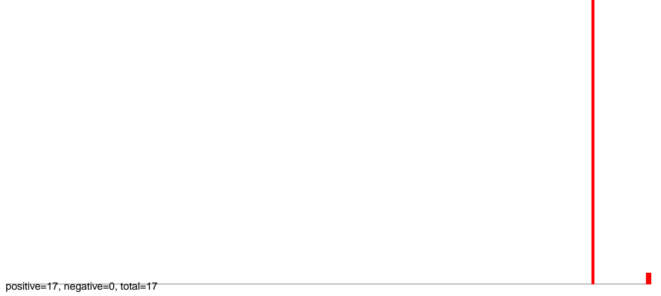
AeAeg_Ovary_TC.24_35.rep
