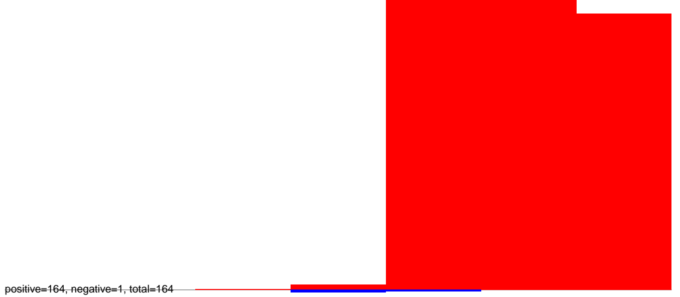
AeAeg_Aag2smallIRNA_DENV1_rep2.24_35.rep
