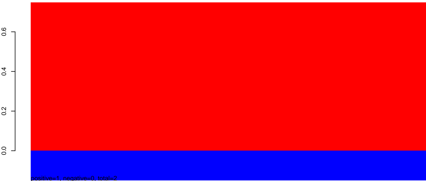
AeAeg_Aag2smallIRNA_DENV1_rep2.24_35.rep
