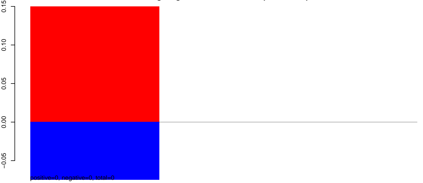
AeAeg_Aag2smallIRNA_DENV1_rep2.24_35.rep
