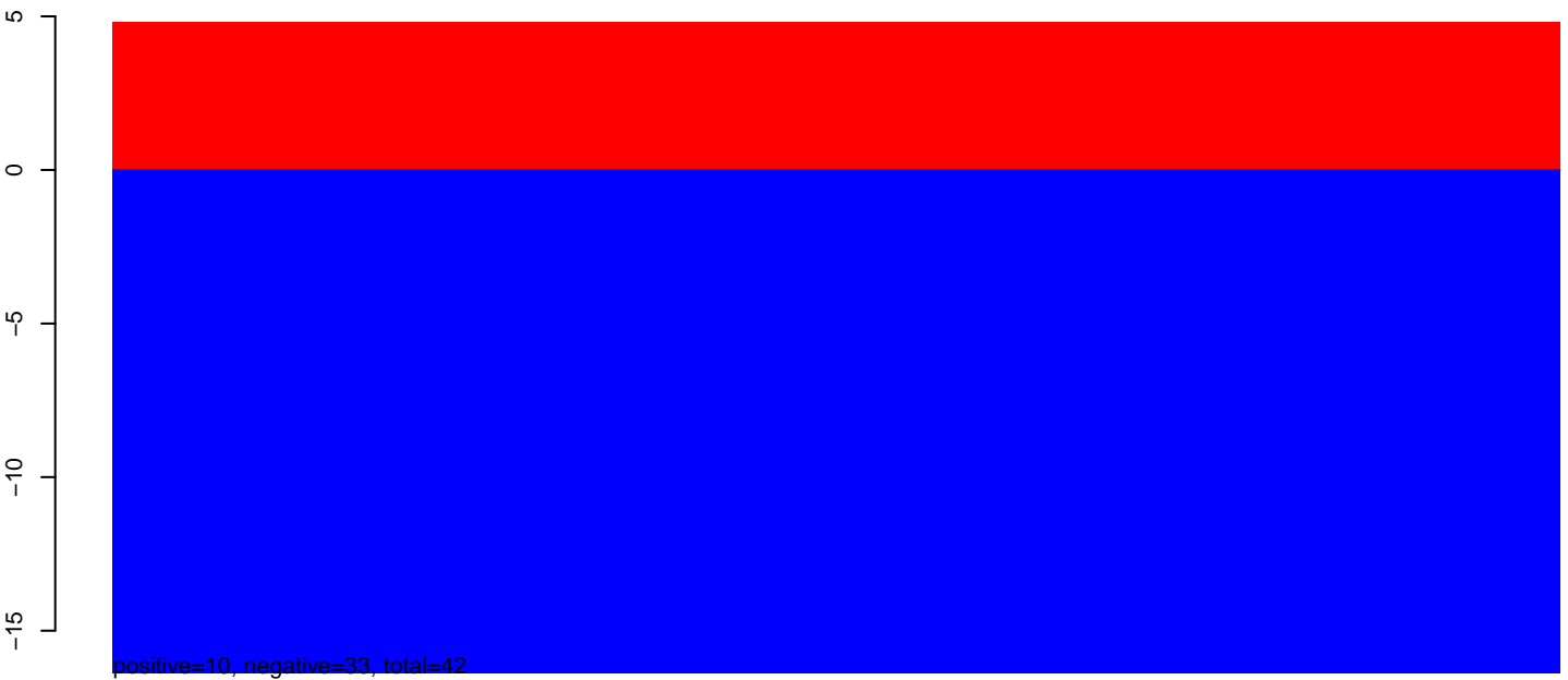
AeAeg_Aag2smallIRNA_DENV1_rep2.24_35.rep
