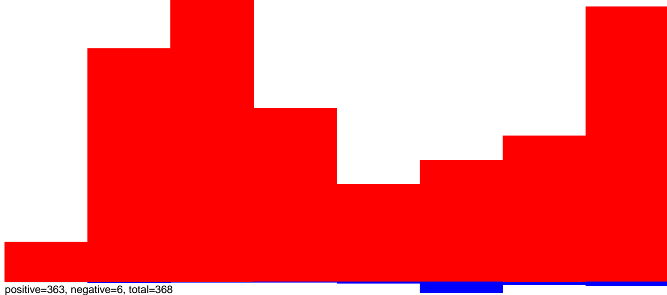
AeAeg_Aag2smallRNA_DENV2NGC_rep2.24_35.rep
