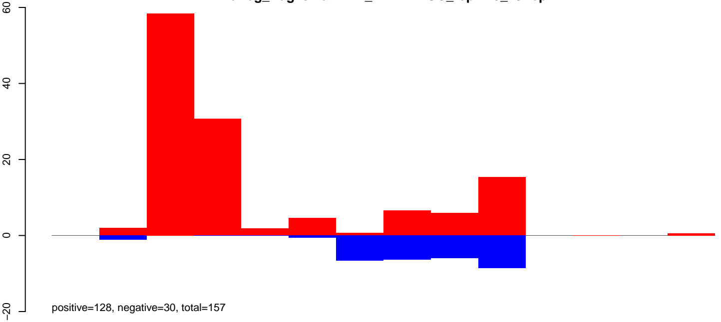
AeAeg_Aag2smallRNA_DENV2NGC_rep2.24_35.rep
