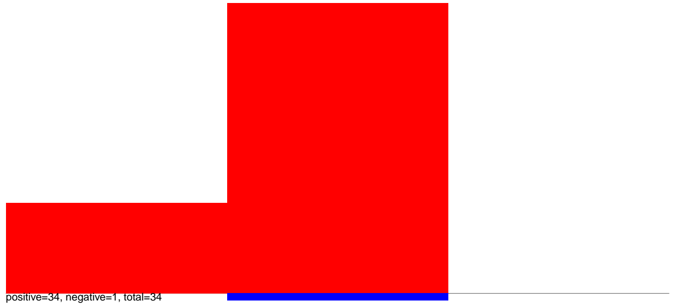
AeAeg_Aag2smallRNA_DENV2NGC_rep2.24_35.rep
