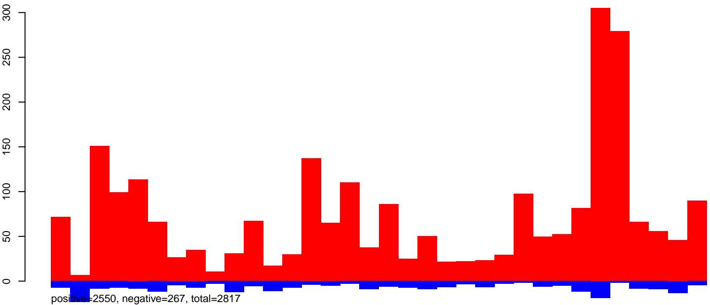
AeAeg_Aag2smallRNA_DENV2NGC_rep2.24_35.rep
