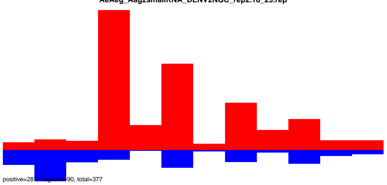
AeAeg_Aag2smallRNA_DENV2NGC_rep2.24_35.rep
