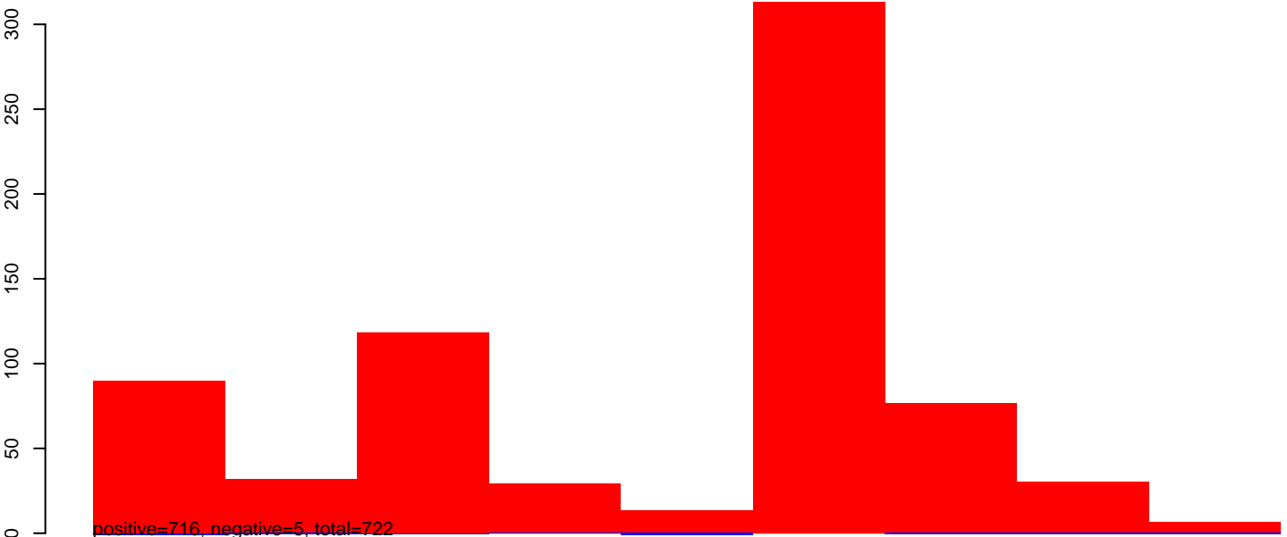
AeAeg_Aag2smallRNA_DENV2NGC_rep2.24_35.rep
