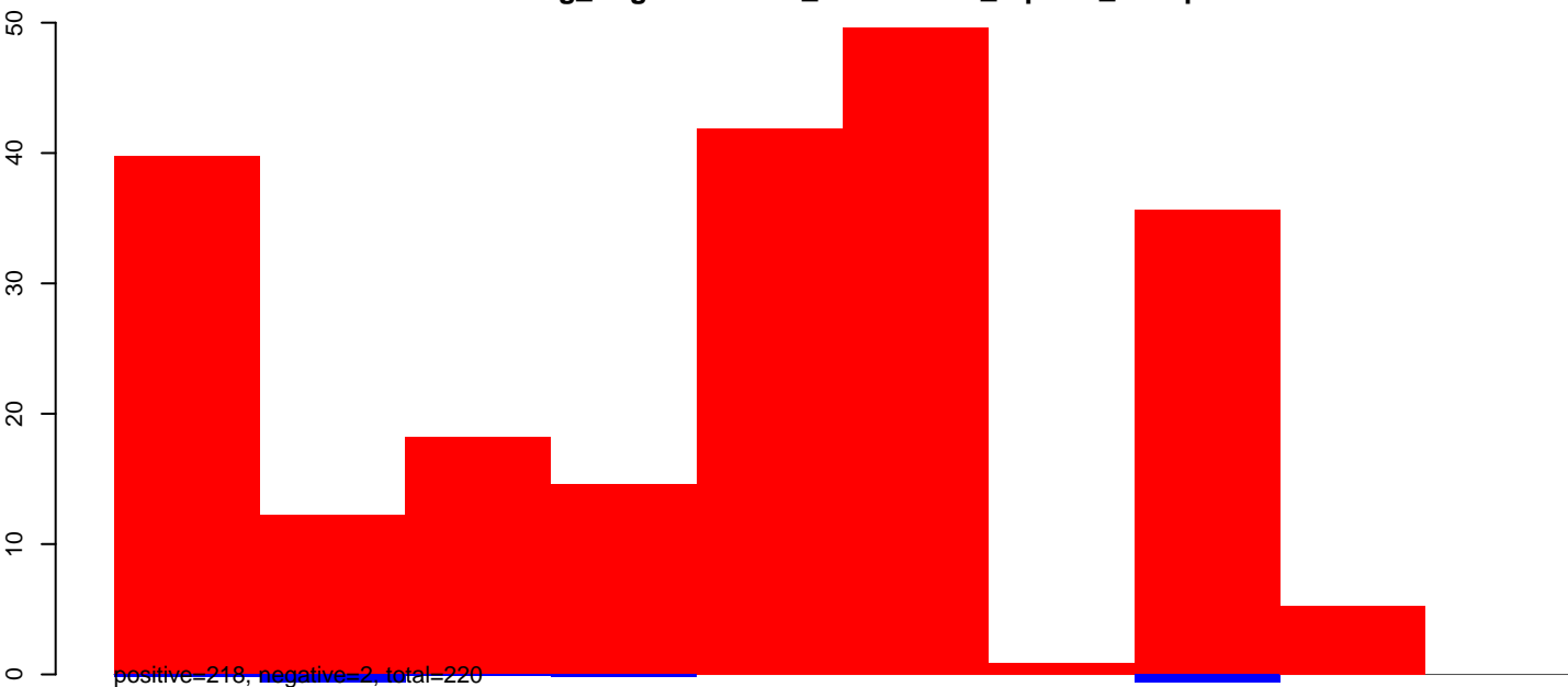
AeAeg_Aag2smallRNA_DENV2NGC_rep2.24_35.rep
