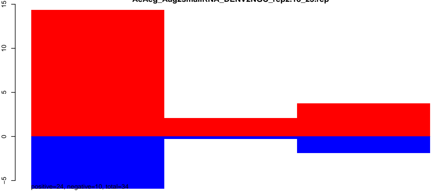
AeAeg_Aag2smallRNA_DENV2NGC_rep2.24_35.rep
