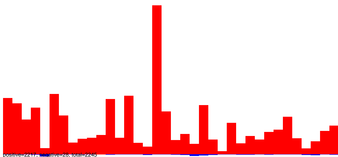
AeAeg_Aag2smallRNA_DENV2NGC_rep2.24_35.rep
