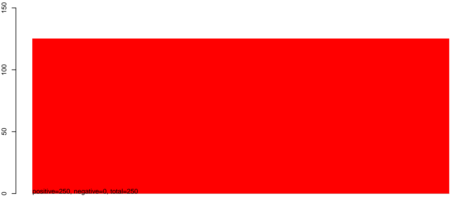
AeAeg_Aag2smallRNA_DENV2NGC_rep2.24_35.rep
