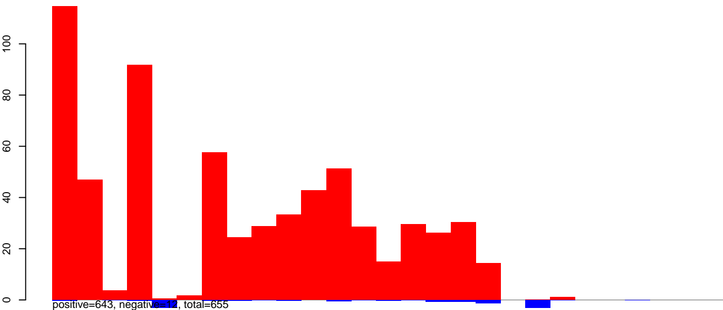
AeAeg_Aag2smallRNA_DENV2NGC_rep2.24_35.rep
