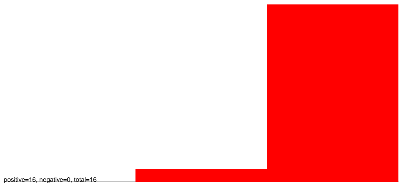
AeAeg_Aag2smallRNA_DENV2NGC_rep2.24_35.rep
