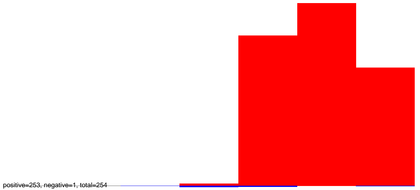
AeAeg_Aag2smallRNA_DENV2NGC_rep2.24_35.rep
