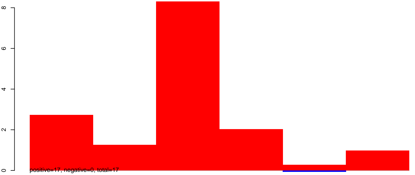
AeAeg_Aag2smallRNA_DENV2NGC_rep2.24_35.rep
