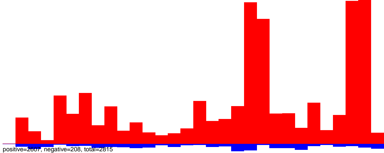
AeAeg_Aag2smallRNA_DENV2NGC_rep2.24_35.rep
