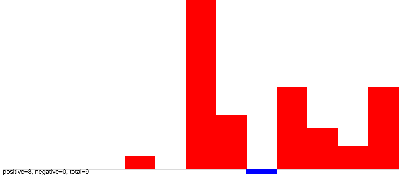
AeAeg_Aag2smallRNA_DENV2NGC_rep2.24_35.rep
