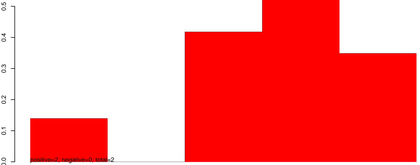
AeAeg_Aag2smallRNA_DENV2NGC_rep2.24_35.rep
