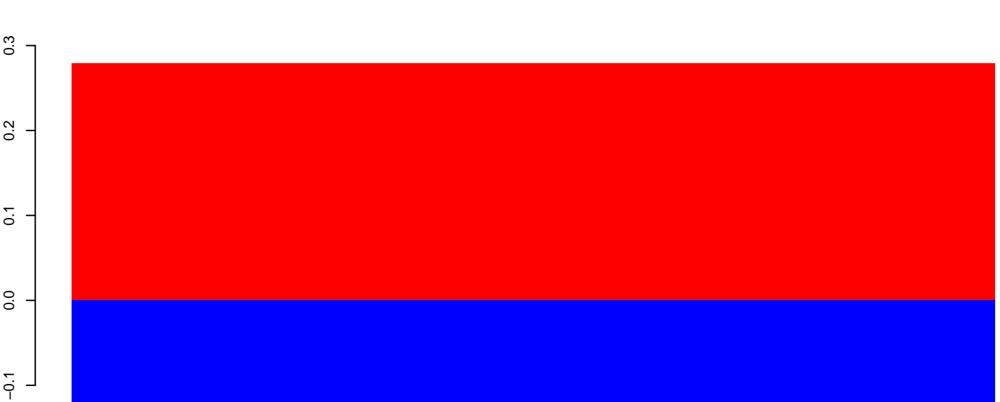
AeAeg_Aag2smallRNA_DENV2NGC_rep2.24_35.rep
