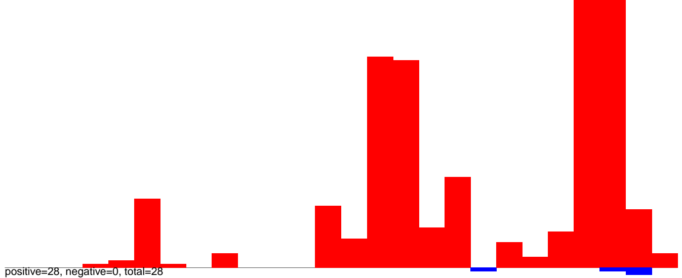
AeAeg_Aag2smallRNA_DENV2NGC_rep2.24_35.rep
