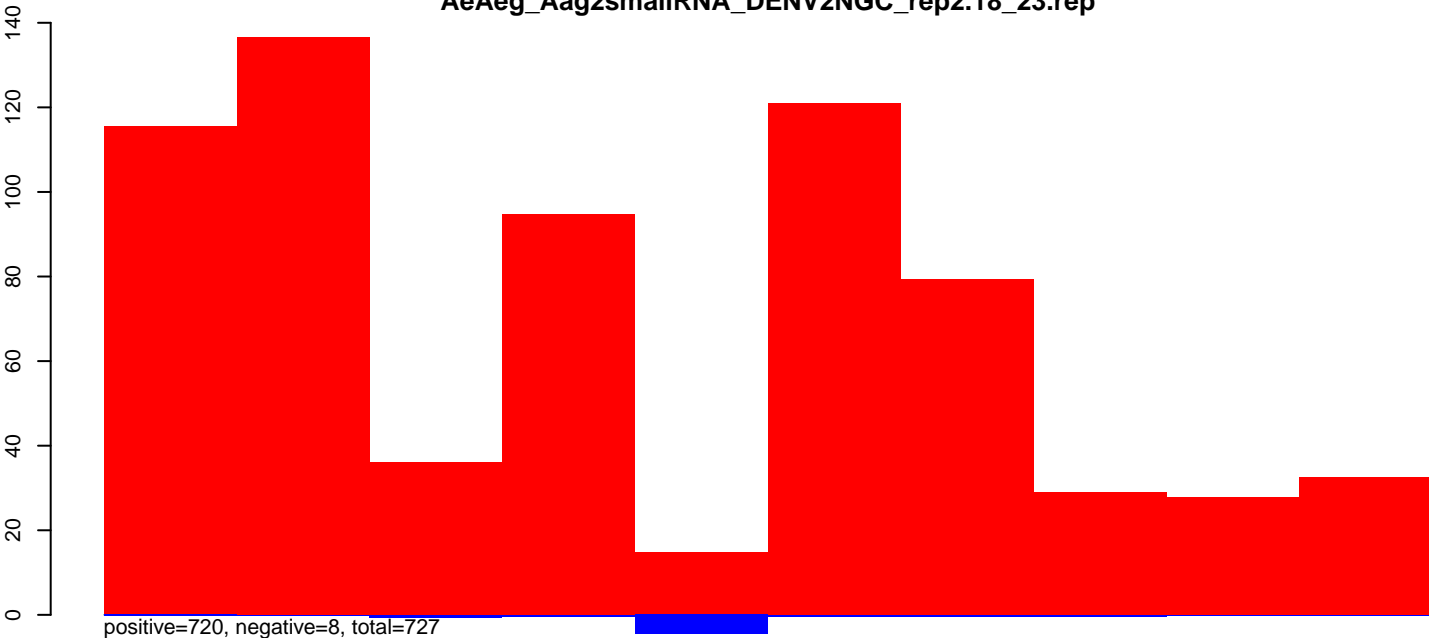
AeAeg_Aag2smallRNA_DENV2NGC_rep2.24_35.rep
