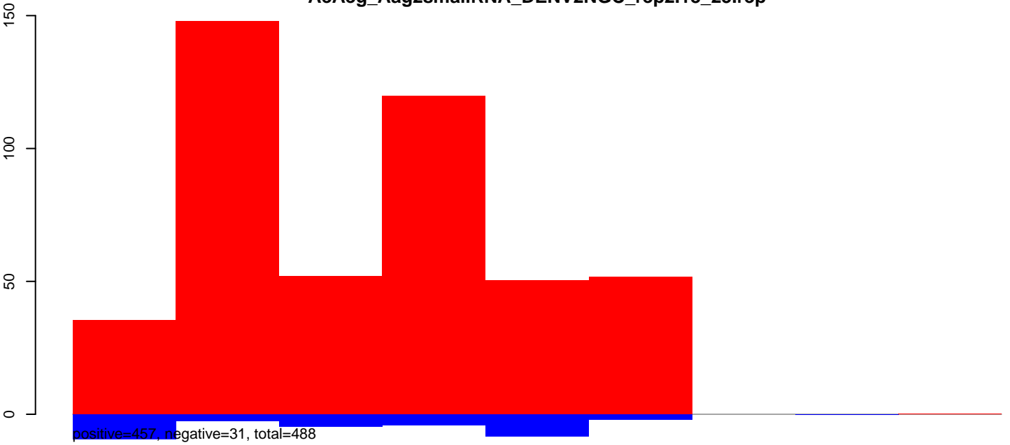
AeAeg_Aag2smallRNA_DENV2NGC_rep2.24_35.rep
