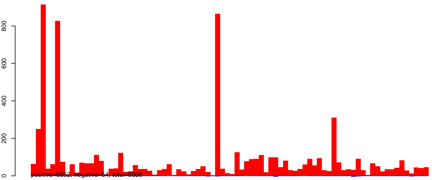
AeAeg_Aag2smallRNA_DENV2NGC_rep2.24_35.rep
