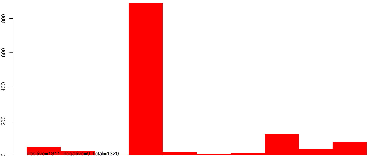
AeAeg_Aag2smallRNA_DENV2NGC_rep2.24_35.rep
