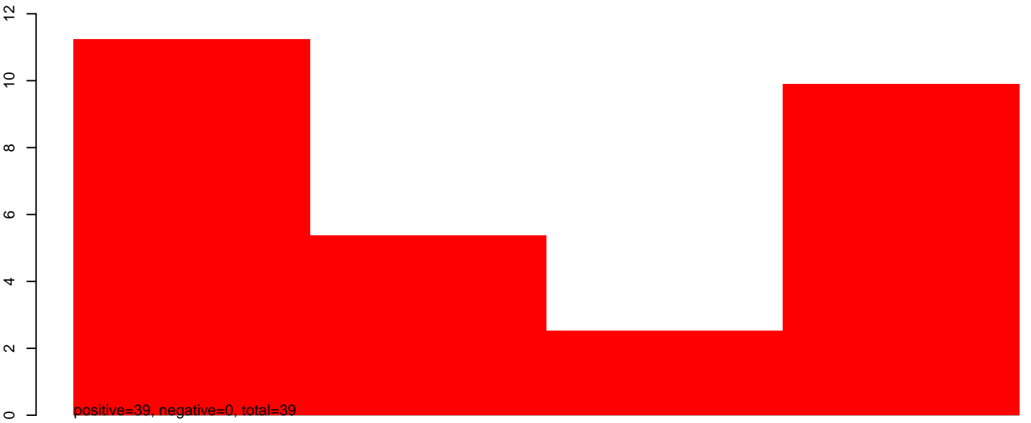
AeAeg_Aag2smallRNA_DENV2NGC_rep2.24_35.rep
