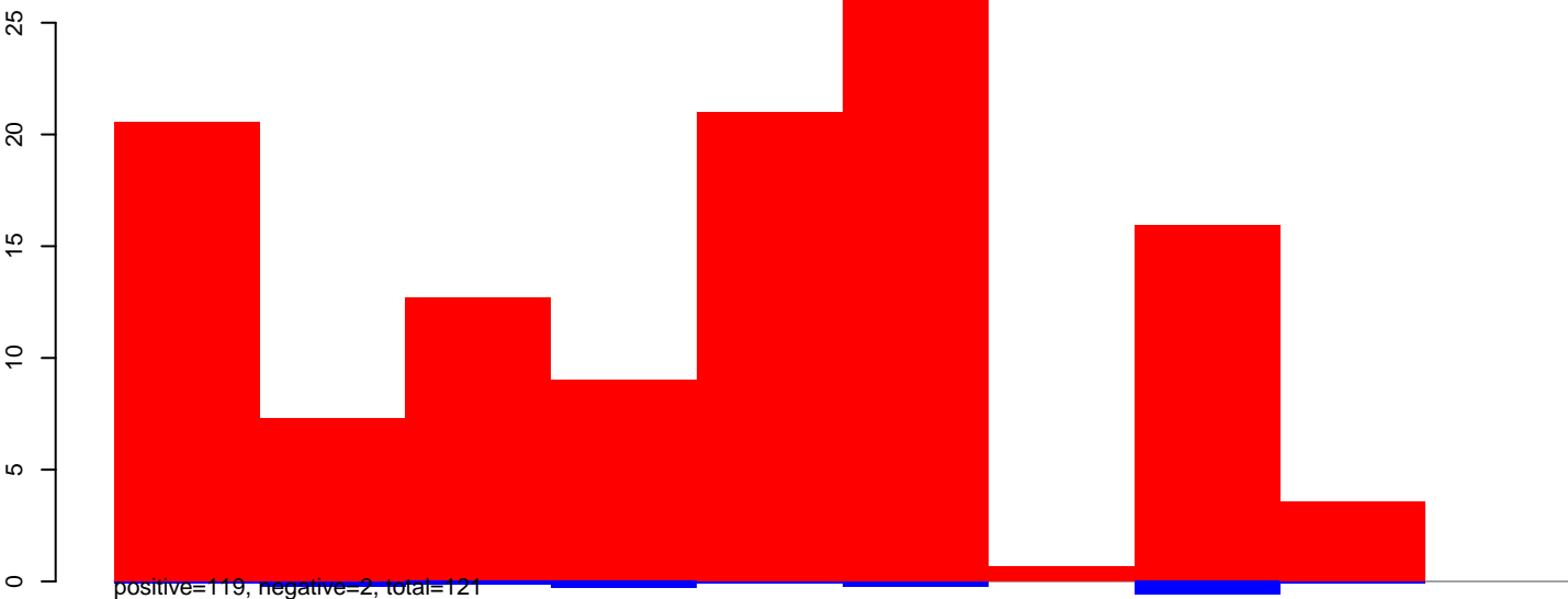
AeAeg_Aag2smallRNA_ZikaOW_rep1.24_35.rep
