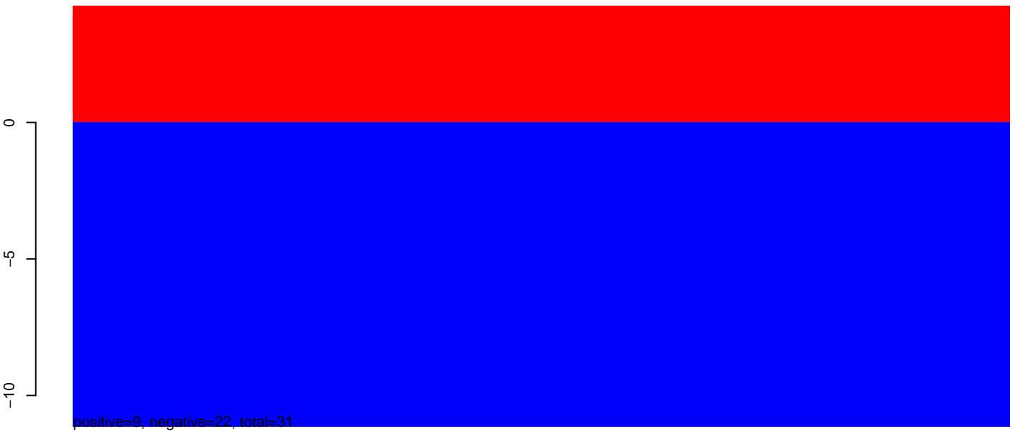
AeAeg_Aag2smallRNA_ZikaOW_rep1.24_35.rep
