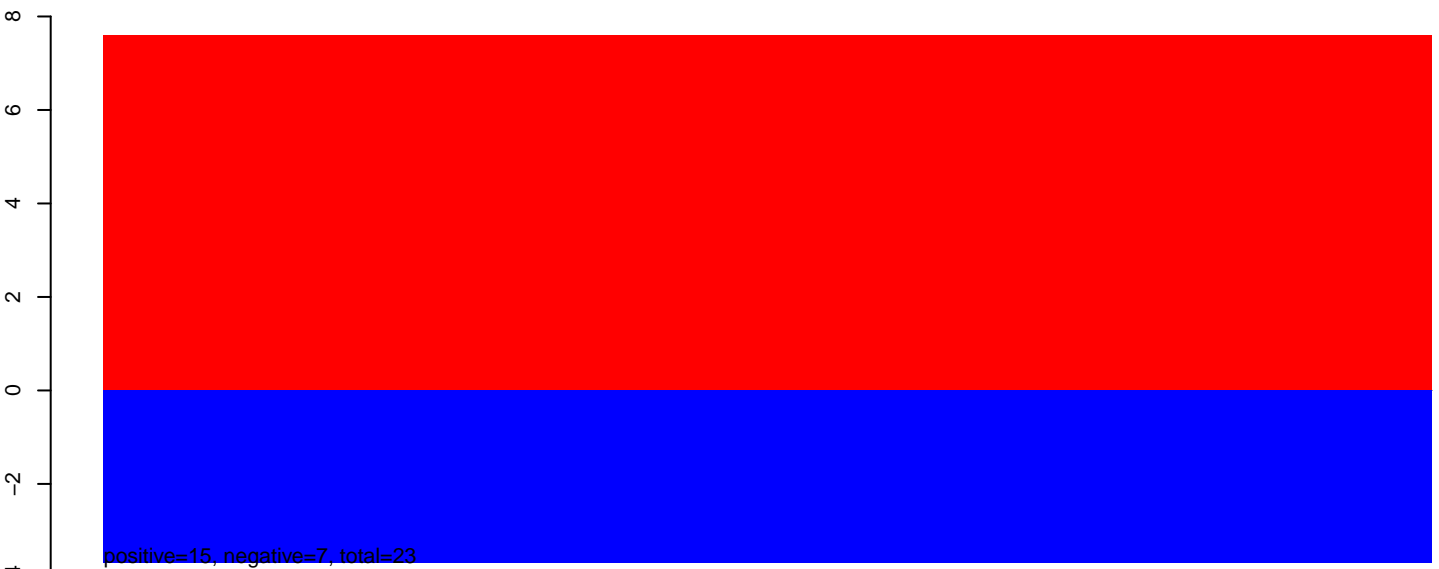
AeAeg_Aag2smallRNA_ZikaOW_rep1.24_35.rep
