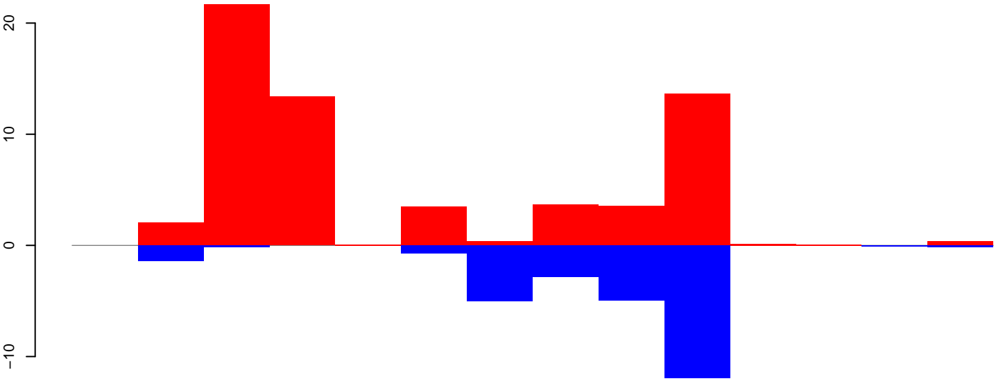
AeAeg_Aag2smallRNA_ZikaOW_rep1.18_23.rep
