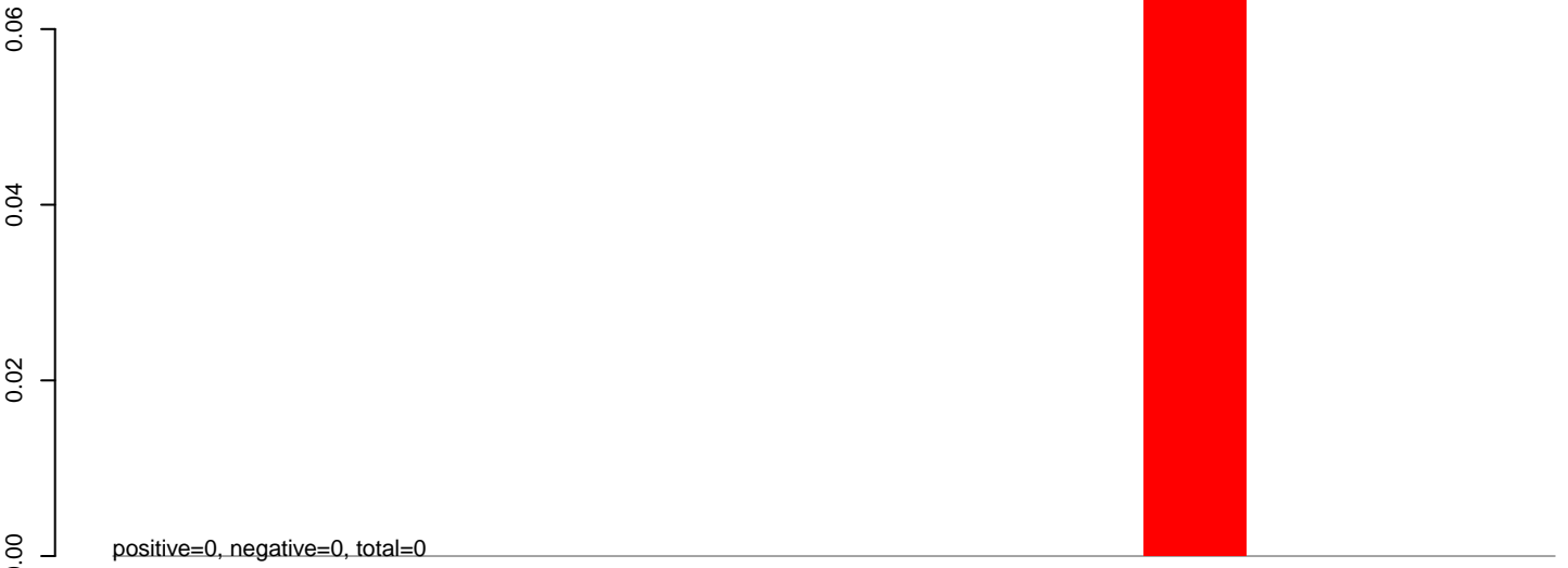
AeAeg_Aag2smallRNA_ZikaOW_rep1.24_35.rep
