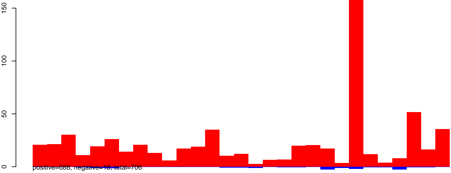
AeAeg_Aag2smallRNA_ZikaOW_rep1.24_35.rep
