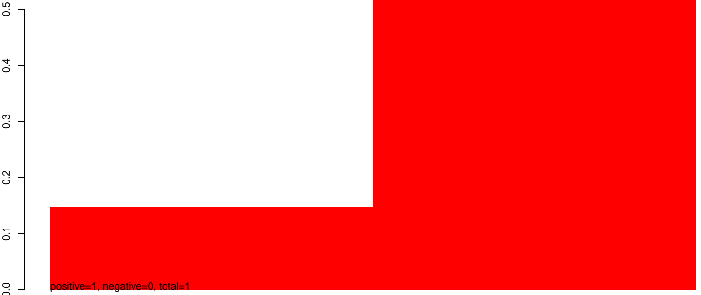
AeAeg_Aag2smallRNA_ZikaOW_rep1.24_35.rep
