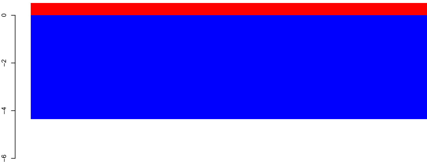
AeAeg_Aag2smallRNA_ZikaOW_rep1.18_23.rep
