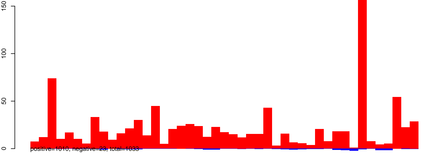
AeAeg_Aag2smallRNA_ZikaOW_rep1.24_35.rep
