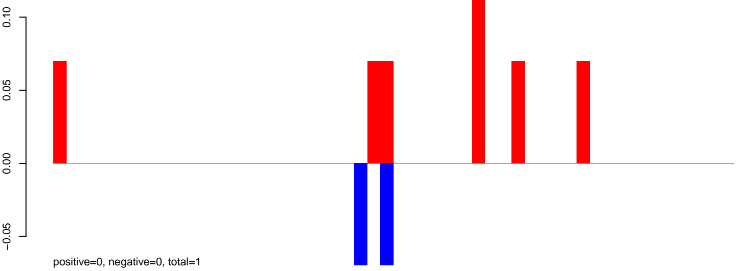
AeAeg_Aag2smallRNA_DENV2NGC_rep2.24_35.rep
