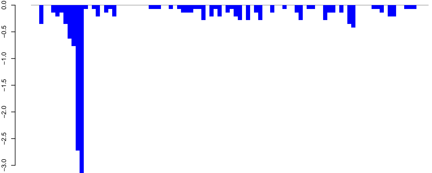
AeAeg_Aag2smallRNA_DENV2NGC_rep2.24_35.rep
