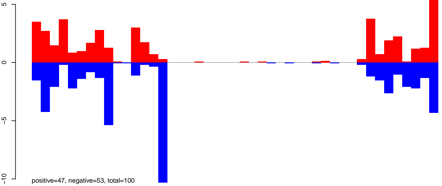
AeAeg_Aag2smallRNA_DENV2NGC_rep2.24_35.rep
