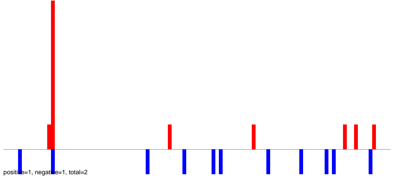
AeAeg_Aag2smallRNA_DENV2NGC_rep2.24_35.rep
