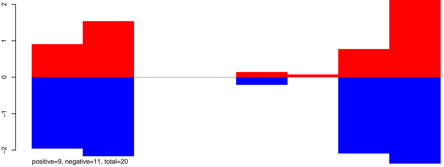
AeAeg_Aag2smallRNA_DENV2NGC_rep2.24_35.rep
