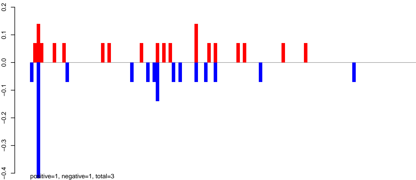
AeAeg_Aag2smallRNA_DENV2NGC_rep2.24_35.rep
