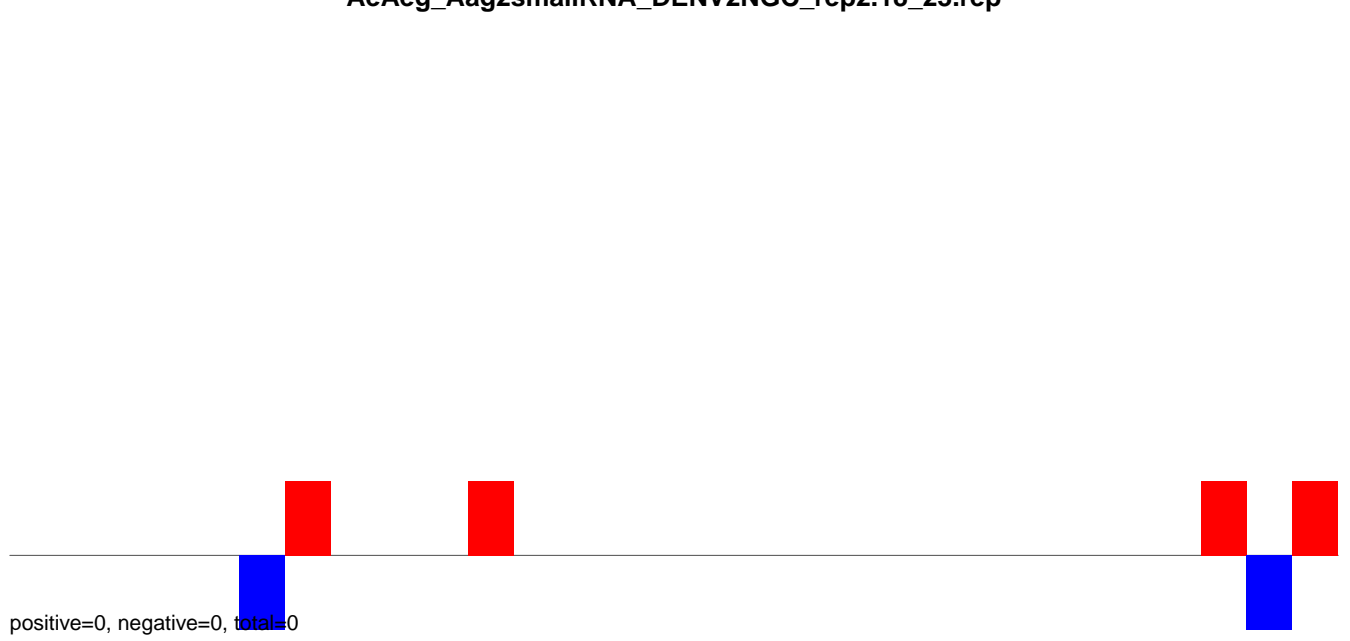
AeAeg_Aag2smallRNA_DENV2NGC_rep2.24_35.rep
