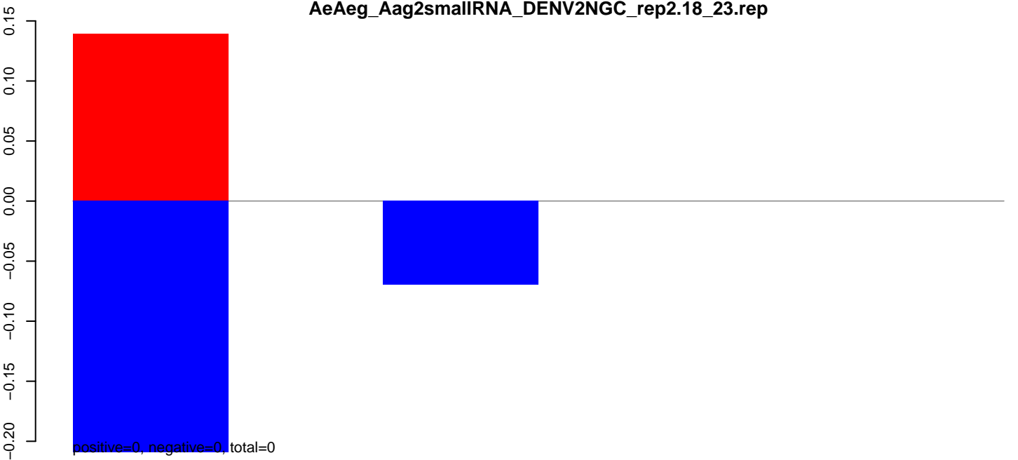
AeAeg_Aag2smallRNA_DENV2NGC_rep2.24_35.rep
