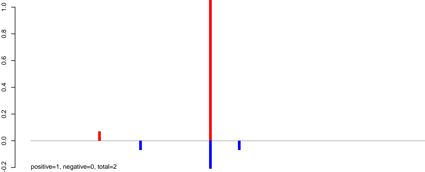
AeAeg_Aag2smallRNA_DENV2NGC_rep2.24_35.rep
