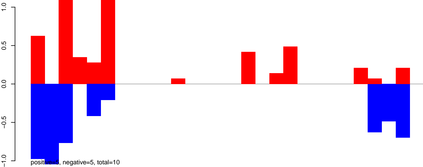
AeAeg_Aag2smallRNA_DENV2NGC_rep2.24_35.rep
