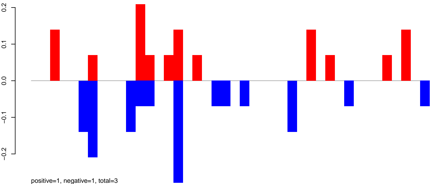
AeAeg_Aag2smallRNA_DENV2NGC_rep2.24_35.rep
