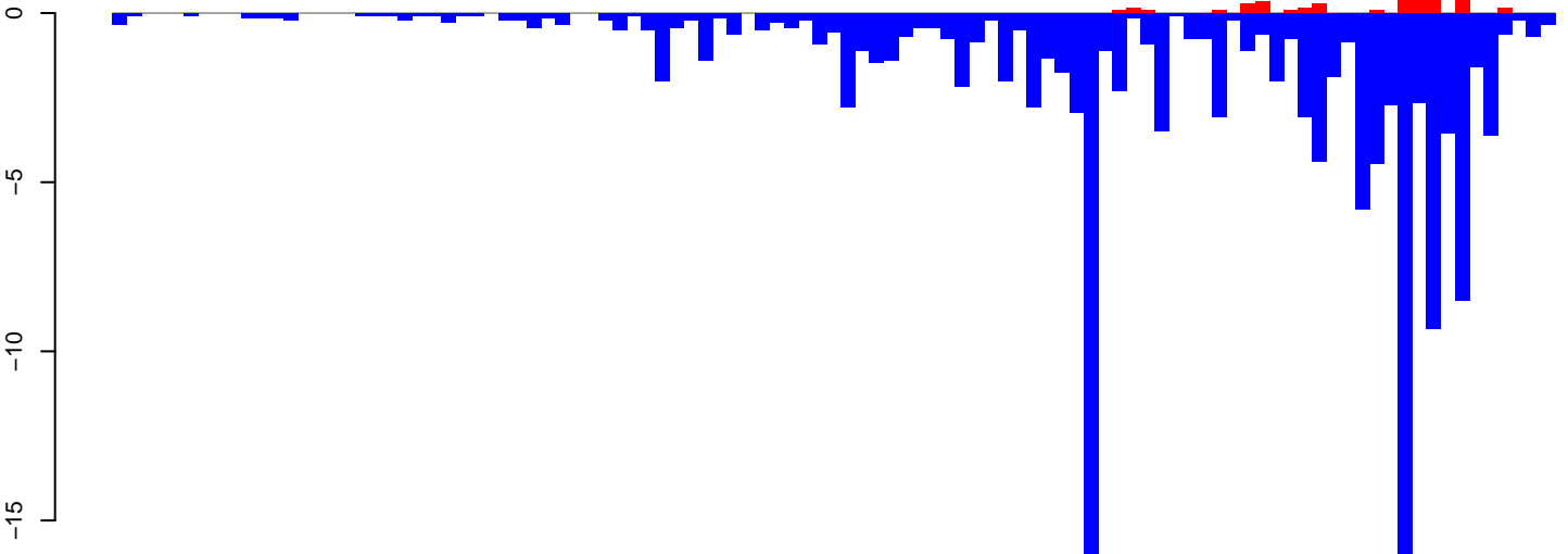
AeAeg_Aag2smallRNA_DENV2NGC_rep2.24_35.rep
