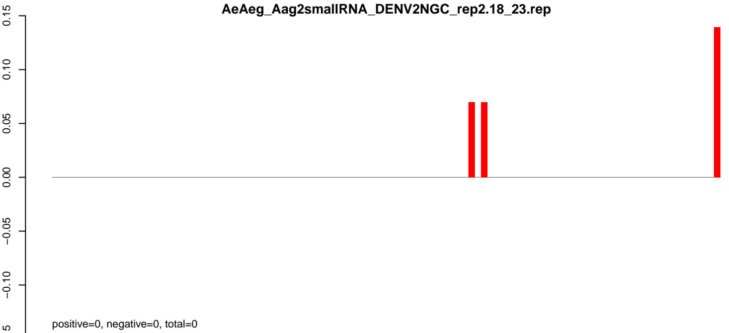
AeAeg_Aag2smallRNA_DENV2NGC_rep2.24_35.rep
