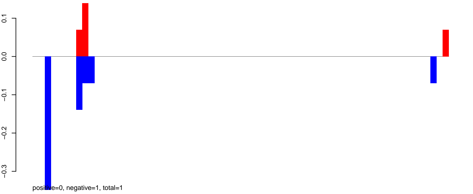
AeAeg_Aag2smallRNA_DENV2NGC_rep2.24_35.rep
