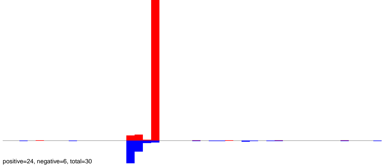
AeAeg_Aag2smallRNA_DENV2NGC_rep2.24_35.rep
