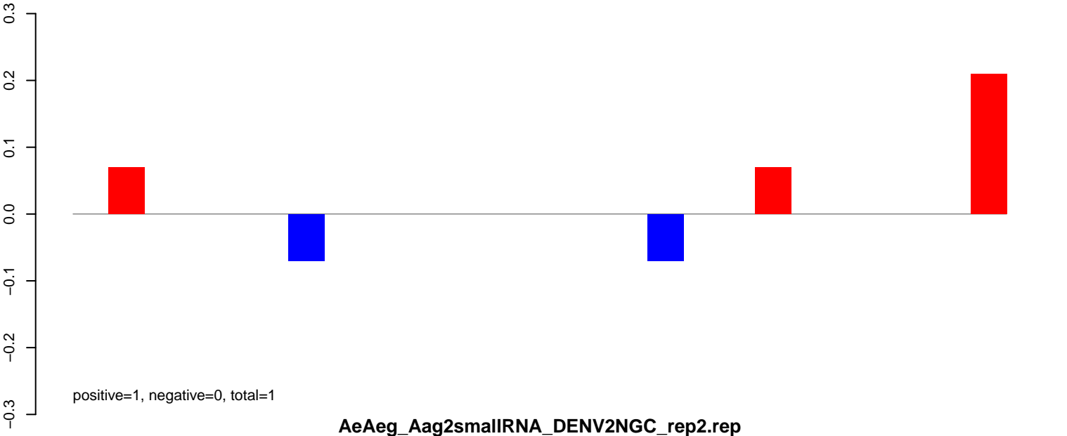
AeAeg_Aag2smallRNA_DENV2NGC_rep2.24_35.rep
