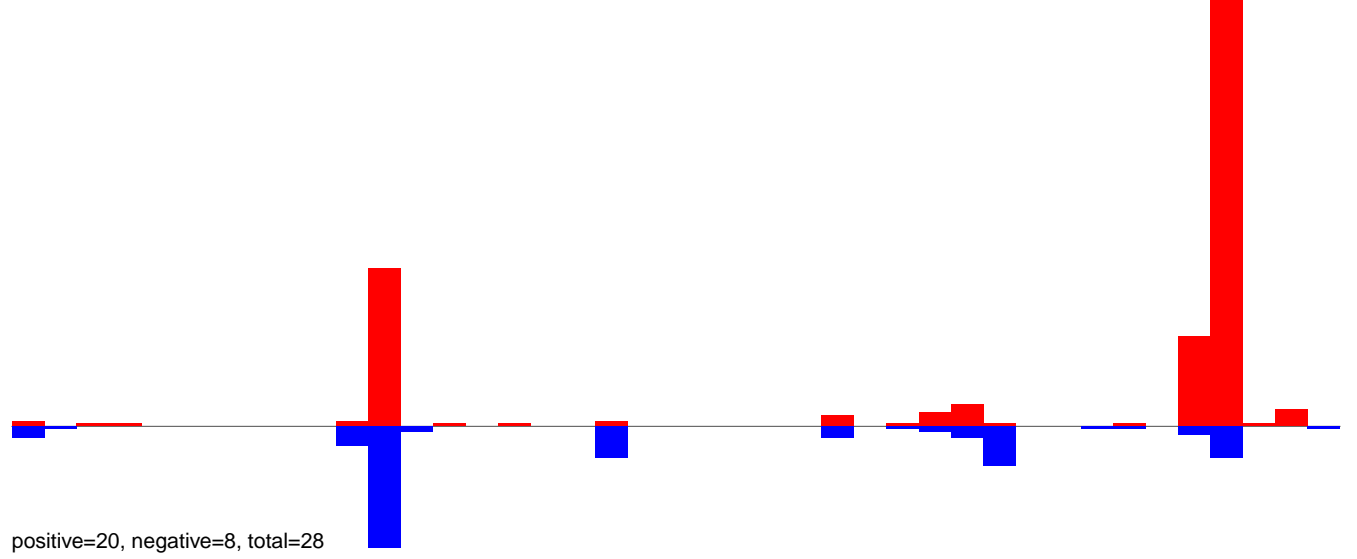
AeAeg_Aag2smallRNA_DENV2NGC_rep2.24_35.rep
