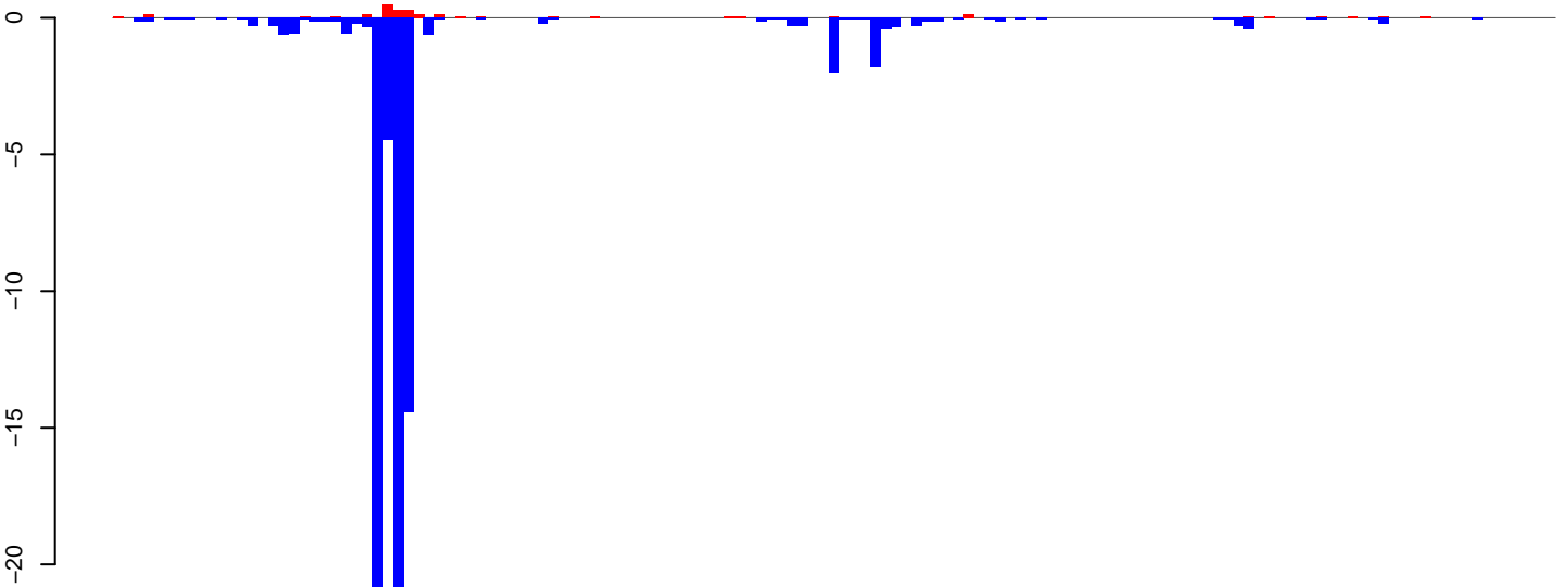
AeAeg_Aag2smallRNA_DENV2NGC_rep2.24_35.rep
