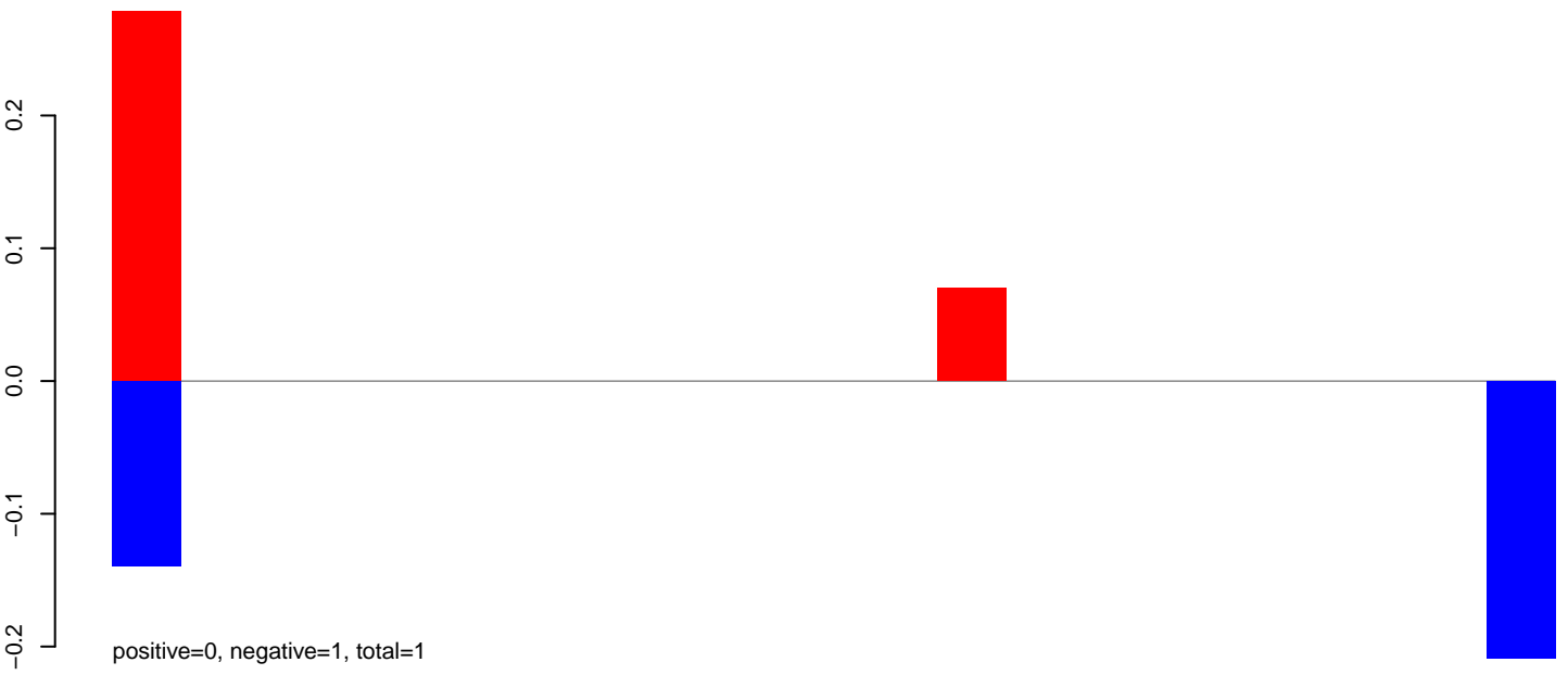
AeAeg_Aag2smallRNA_DENV2NGC_rep2.24_35.rep
