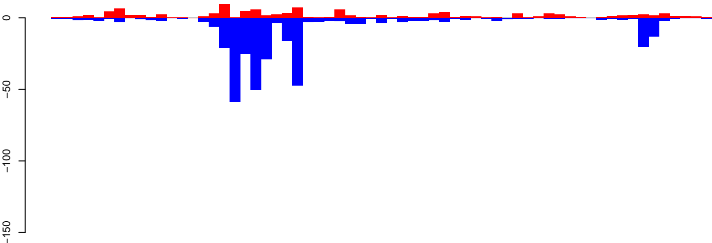
AeAeg_Aag2smallRNA_DENV2NGC_rep2.24_35.rep
