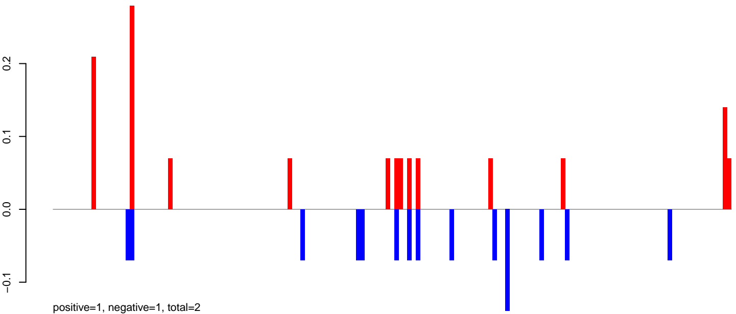
AeAeg_Aag2smallRNA_DENV2NGC_rep2.24_35.rep
