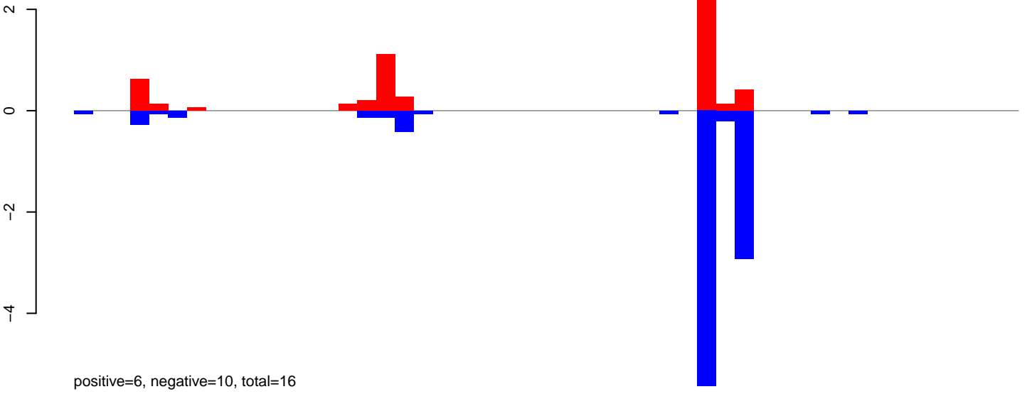
AeAeg_Aag2smallRNA_DENV2NGC_rep2.24_35.rep
