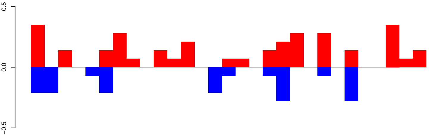
AeAeg_Aag2smallRNA_DENV2NGC_rep2.24_35.rep
