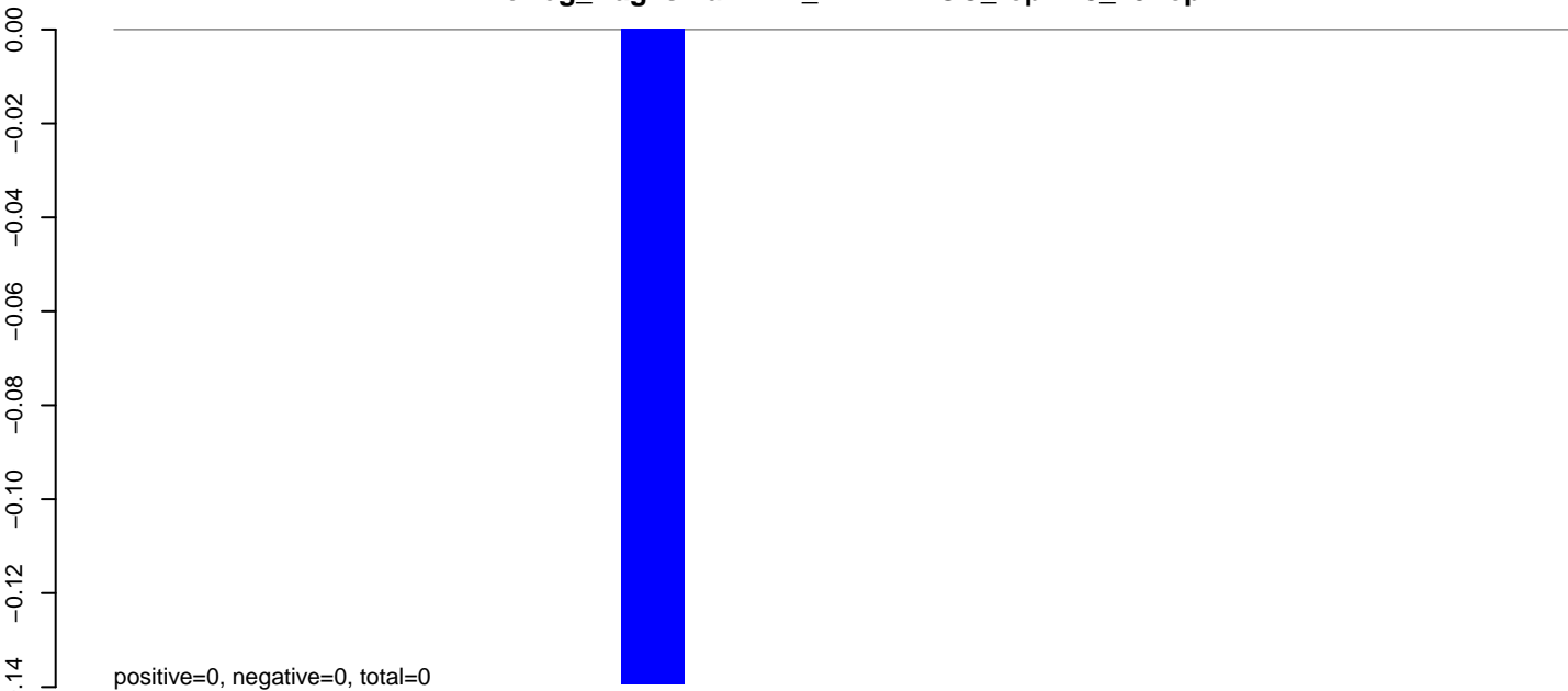
AeAeg_Aag2smallRNA_DENV2NGC_rep2.24_35.rep
