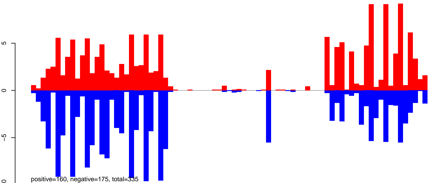
AeAeg_Aag2smallRNA_DENV2NGC_rep2.24_35.rep
