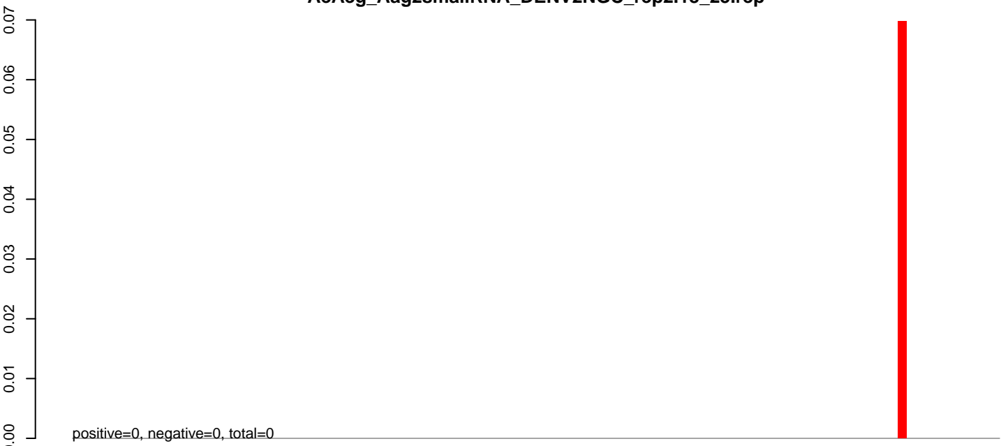
AeAeg_Aag2smallRNA_DENV2NGC_rep2.24_35.rep
