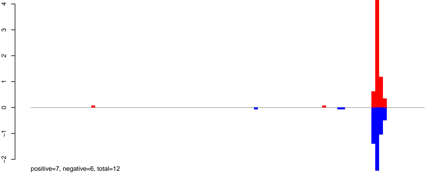
AeAeg_Aag2smallRNA_DENV2NGC_rep2.24_35.rep
