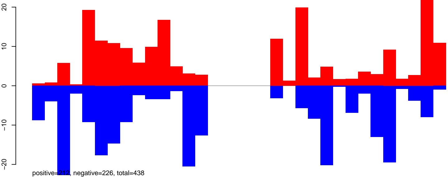
AeAeg_Aag2smallRNA_DENV2NGC_rep2.24_35.rep
