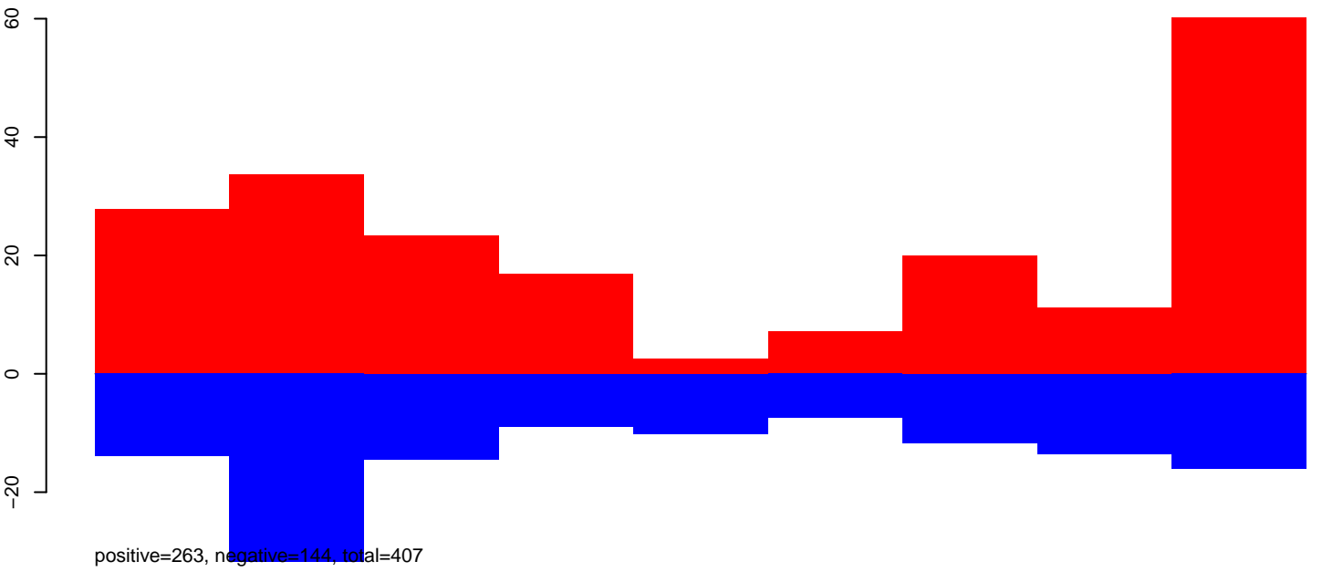
AeAeg_Aag2smallRNA_DENV2NGC_rep2.24_35.rep
