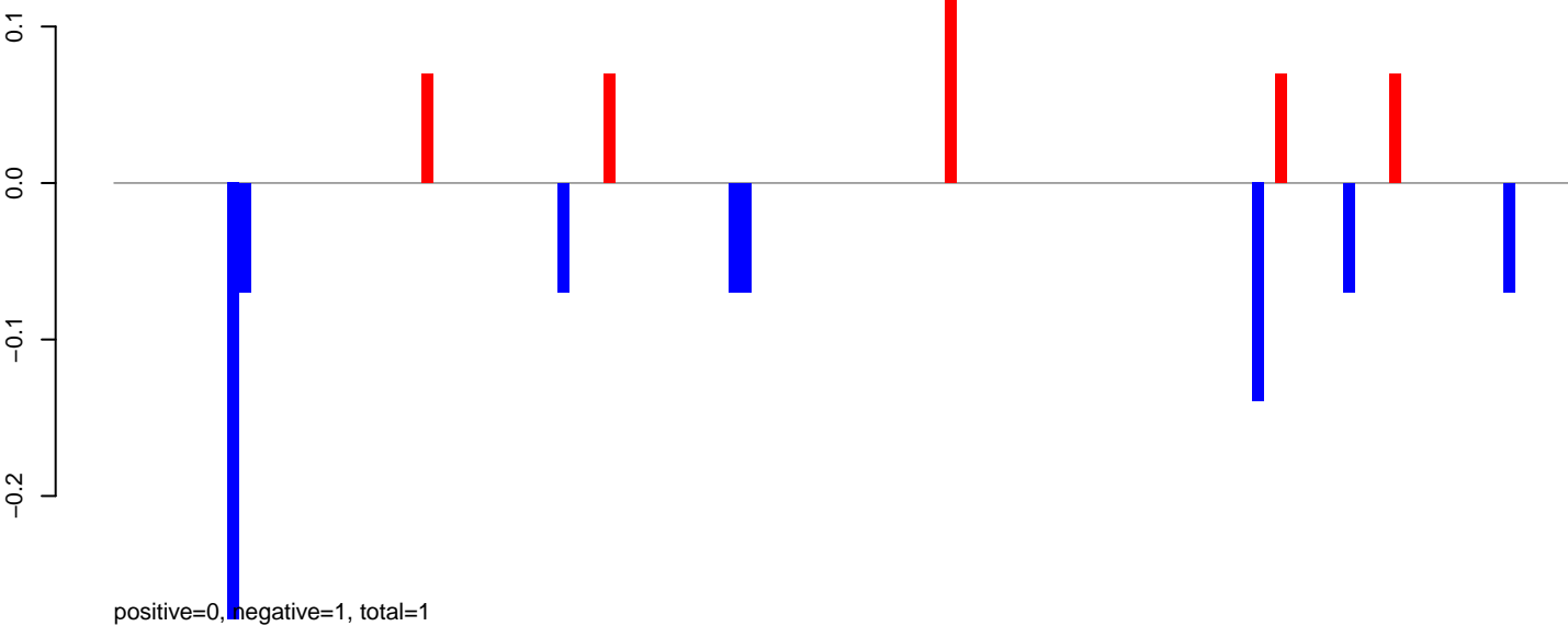
AeAeg_Aag2smallRNA_DENV2NGC_rep2.24_35.rep
