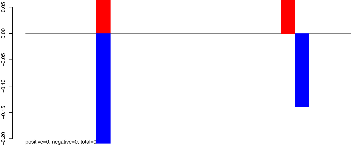
AeAeg_Aag2smallRNA_DENV2NGC_rep2.24_35.rep
