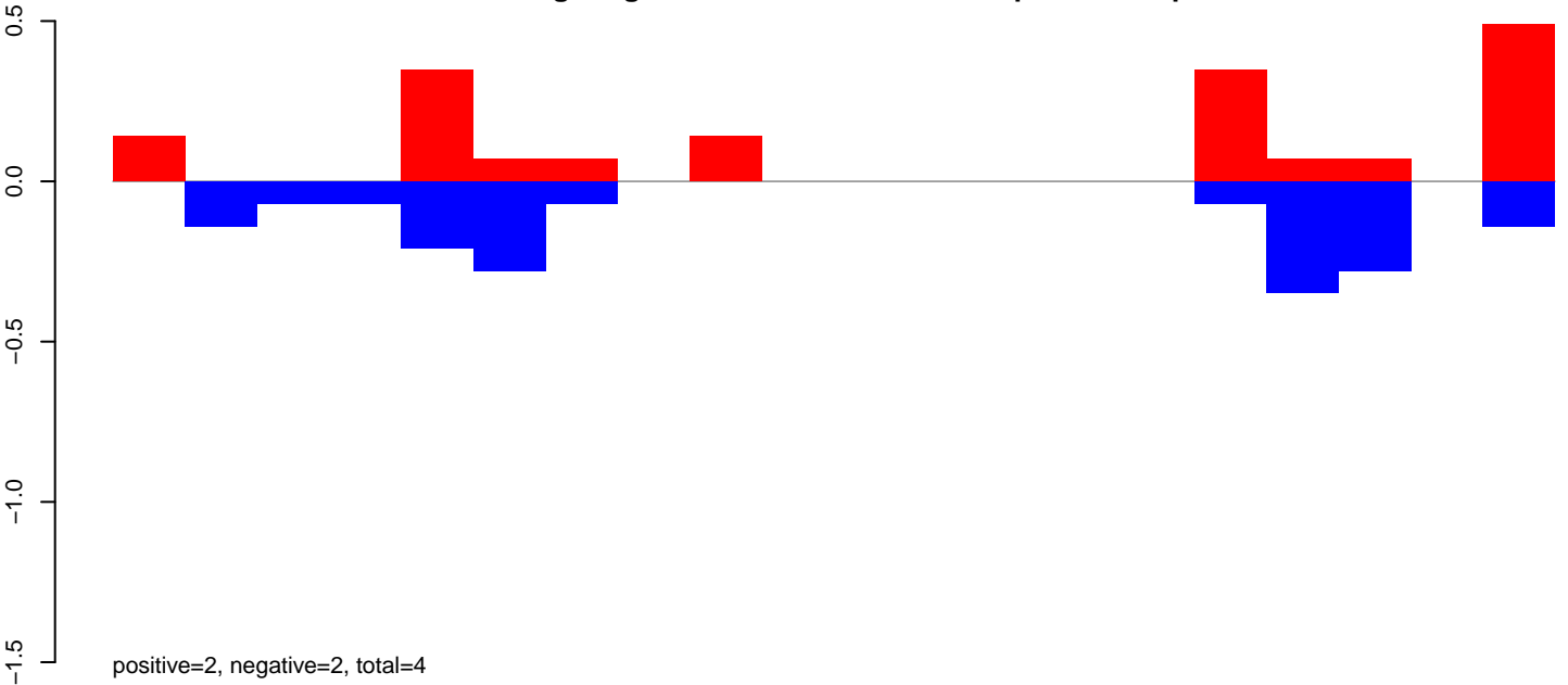
AeAeg_Aag2smallRNA_DENV2NGC_rep2.24_35.rep
