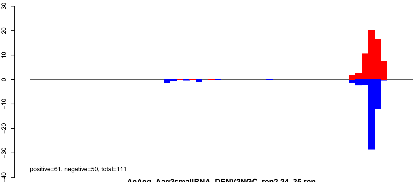
AeAeg_Aag2smallRNA_DENV2NGC_rep2.24_35.rep
