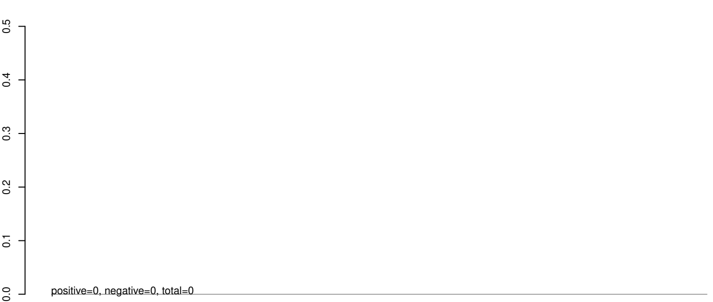
AeAeg_Aag2_Piwi4_IP1_RA.rep
