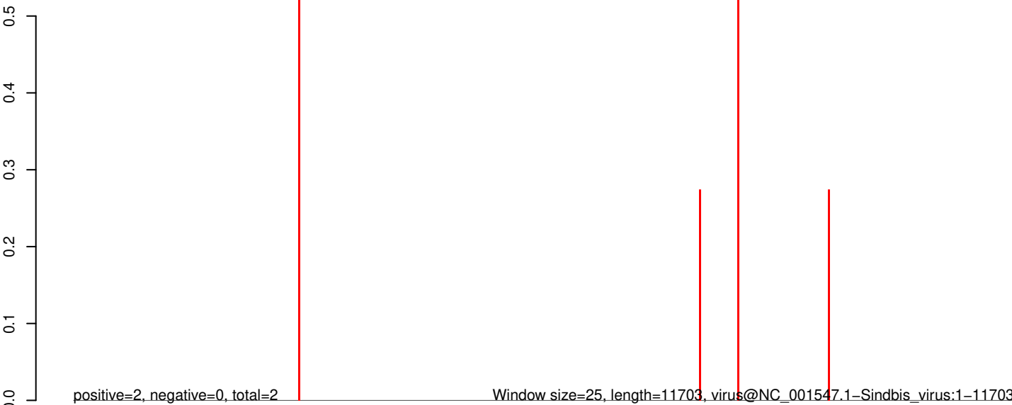
AeAeg_Aag2_Piwi4_IP1_RA.rep
