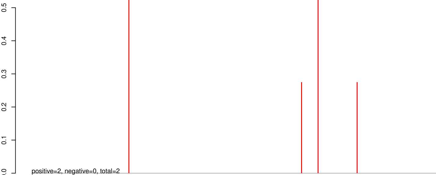
AeAeg_Aag2_Piwi4_IP1_RA.24_35.rep
