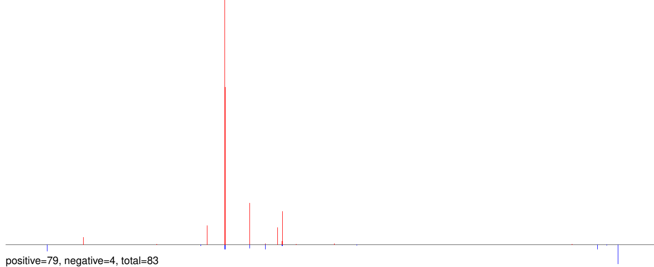
AeAeg_Whole_ZIKV_BM_RNA_GP.24_35.rep
