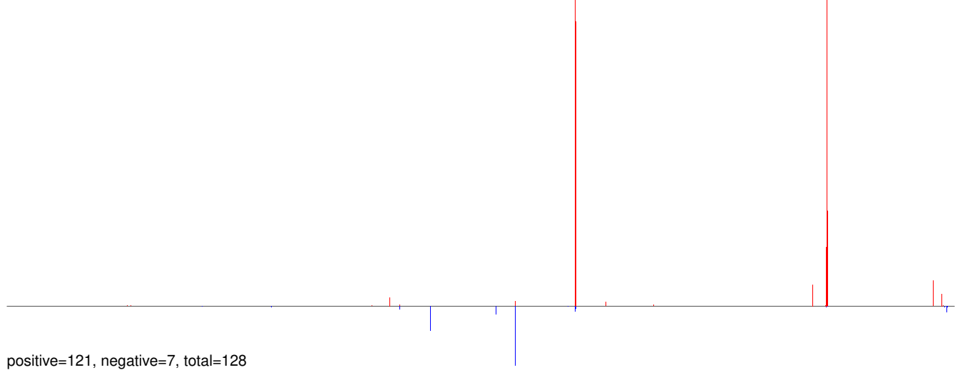
AeAeg_Whole_ZIKV_BM_RNA_GP.24_35.rep
