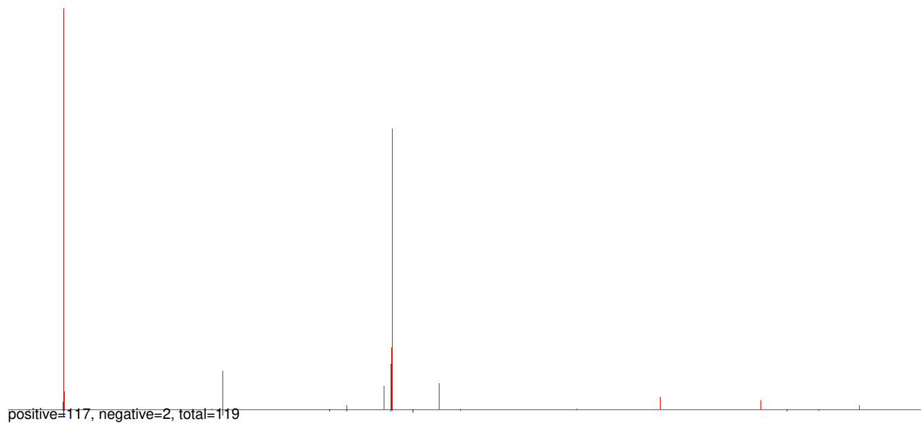
AeAeg_Whole_ZIKV_BM_RNA_GP.24_35.rep
