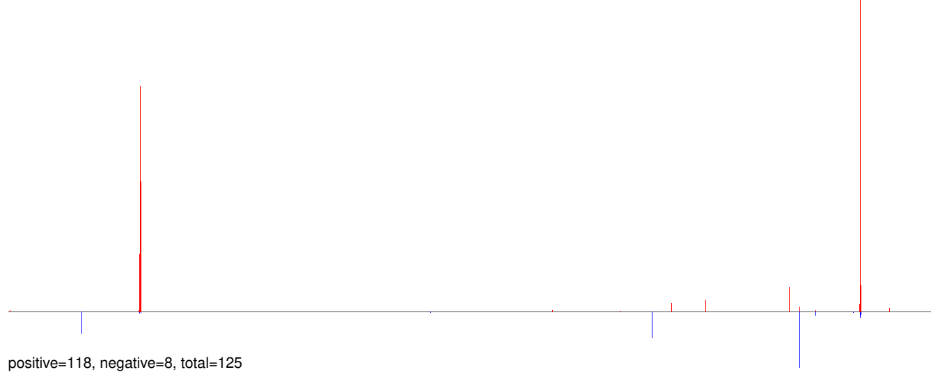
AeAeg_Whole_ZIKV_BM_RNA_GP.24_35.rep
