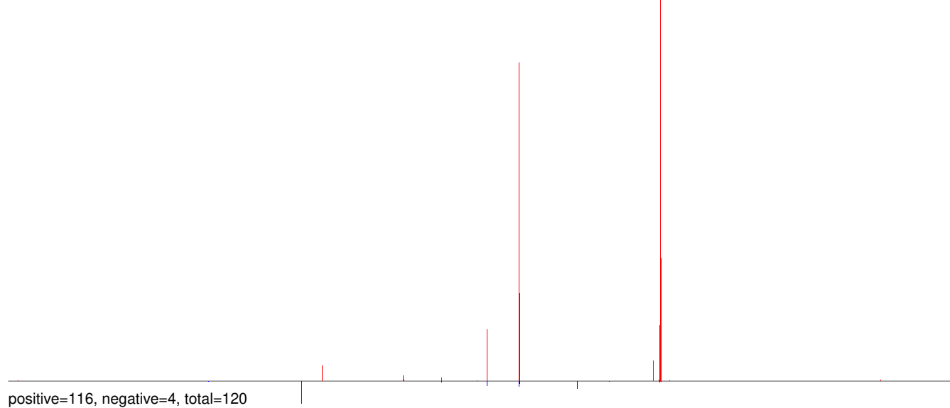
AeAeg_Whole_ZIKV_BM_RNA_GP.24_35.rep
