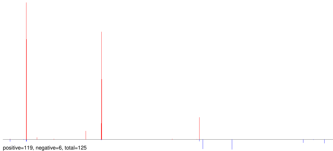
AeAeg_Whole_ZIKV_BM_RNA_GP.24_35.rep
