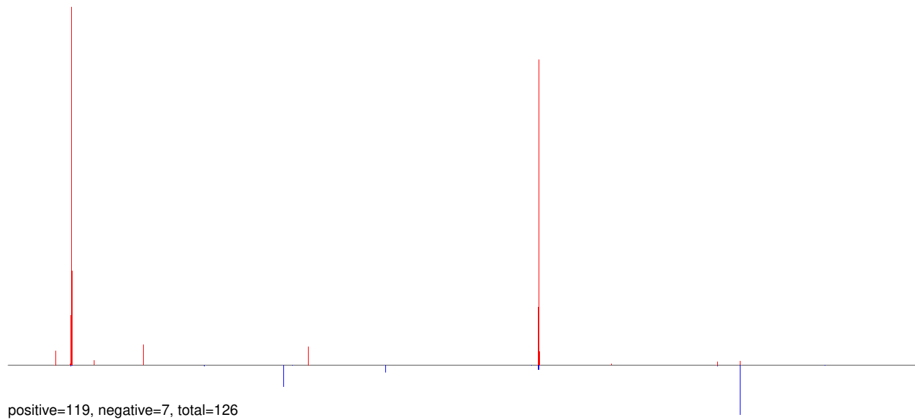
AeAeg_Whole_ZIKV_BM_RNA_GP.24_35.rep
