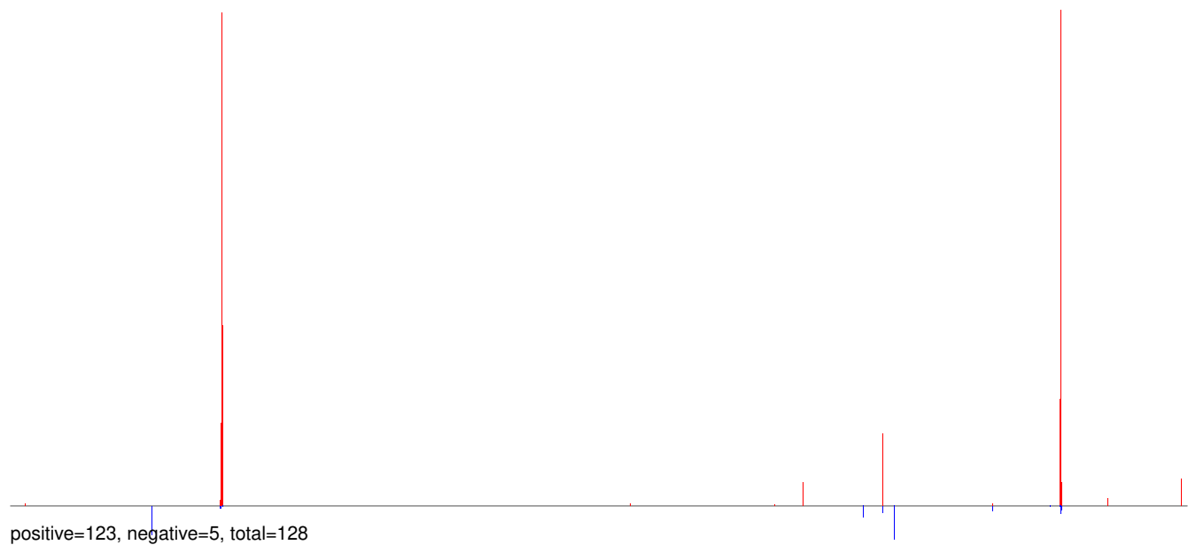
AeAeg_Whole_ZIKV_BM_RNA_GP.24_35.rep
