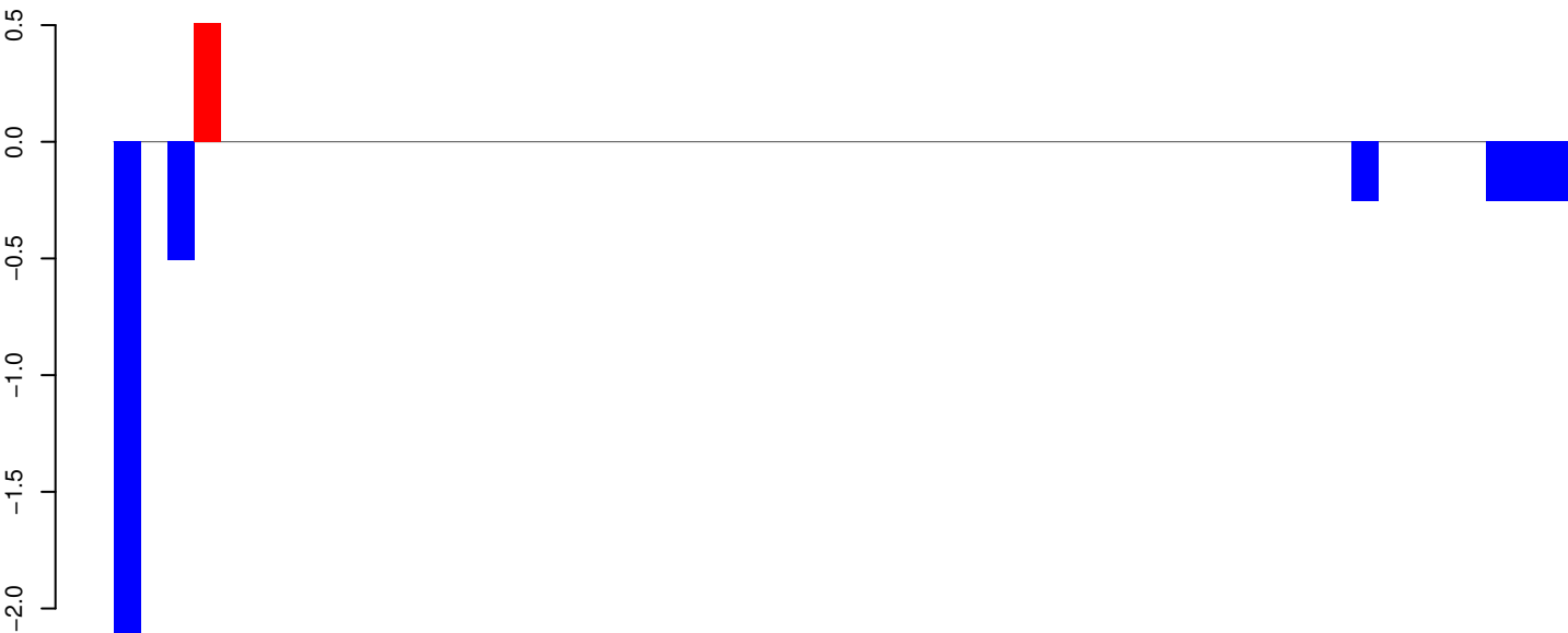
AeAeg_Aag2SINV_Piwi4.IP.24_35.rep
