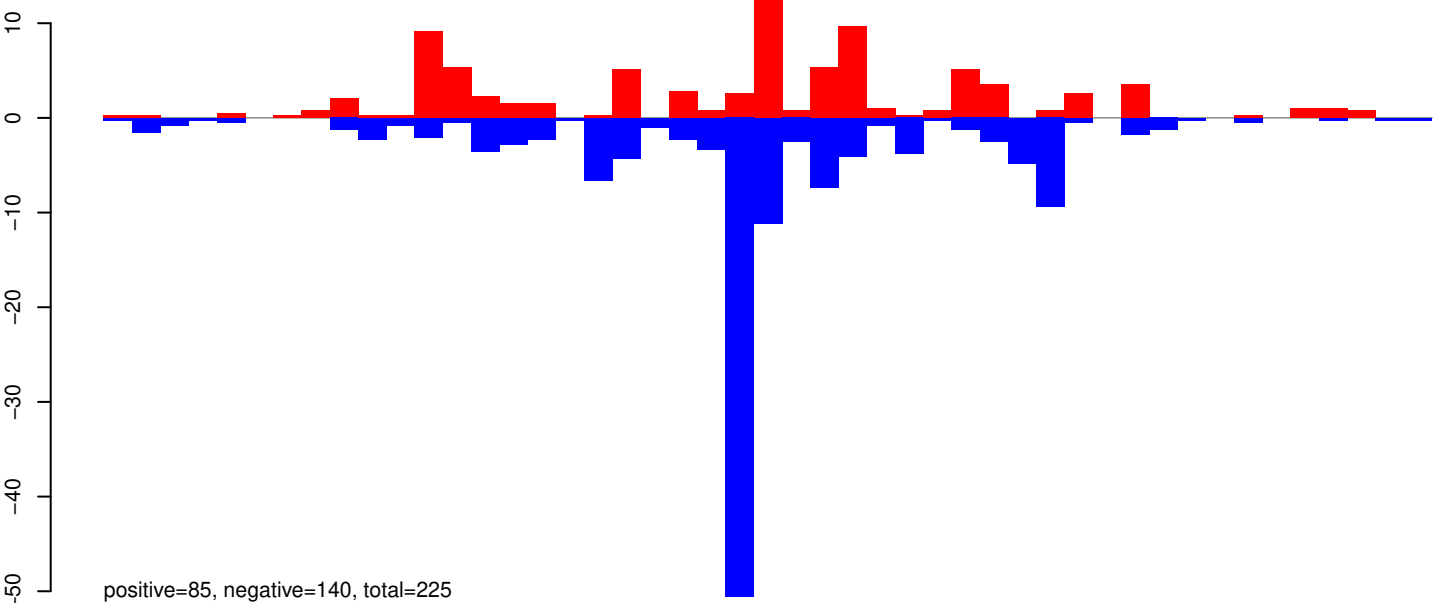
AeAeg_Aag2SINV_Piwi4.IP.24_35.rep
