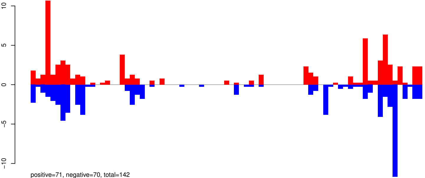
AeAeg_Aag2SINV_Piwi4.IP.24_35.rep
