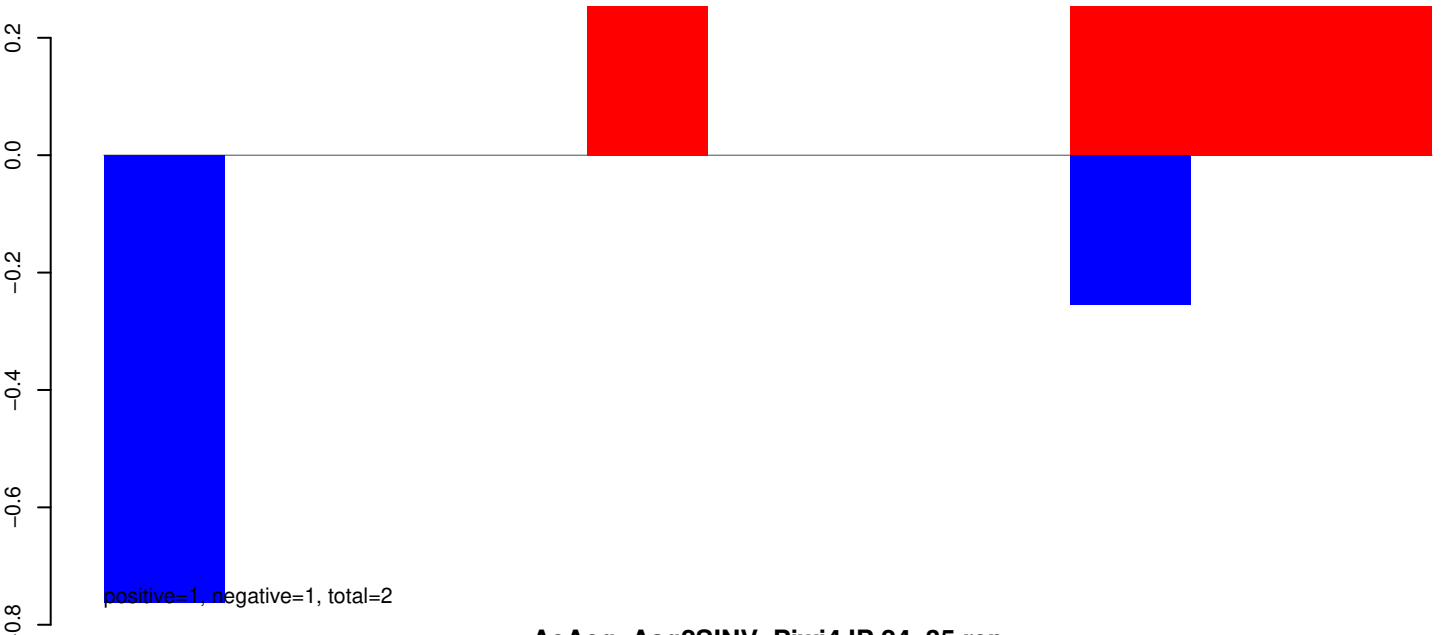
AeAeg_Aag2SINV_Piwi4.IP.24_35.rep
