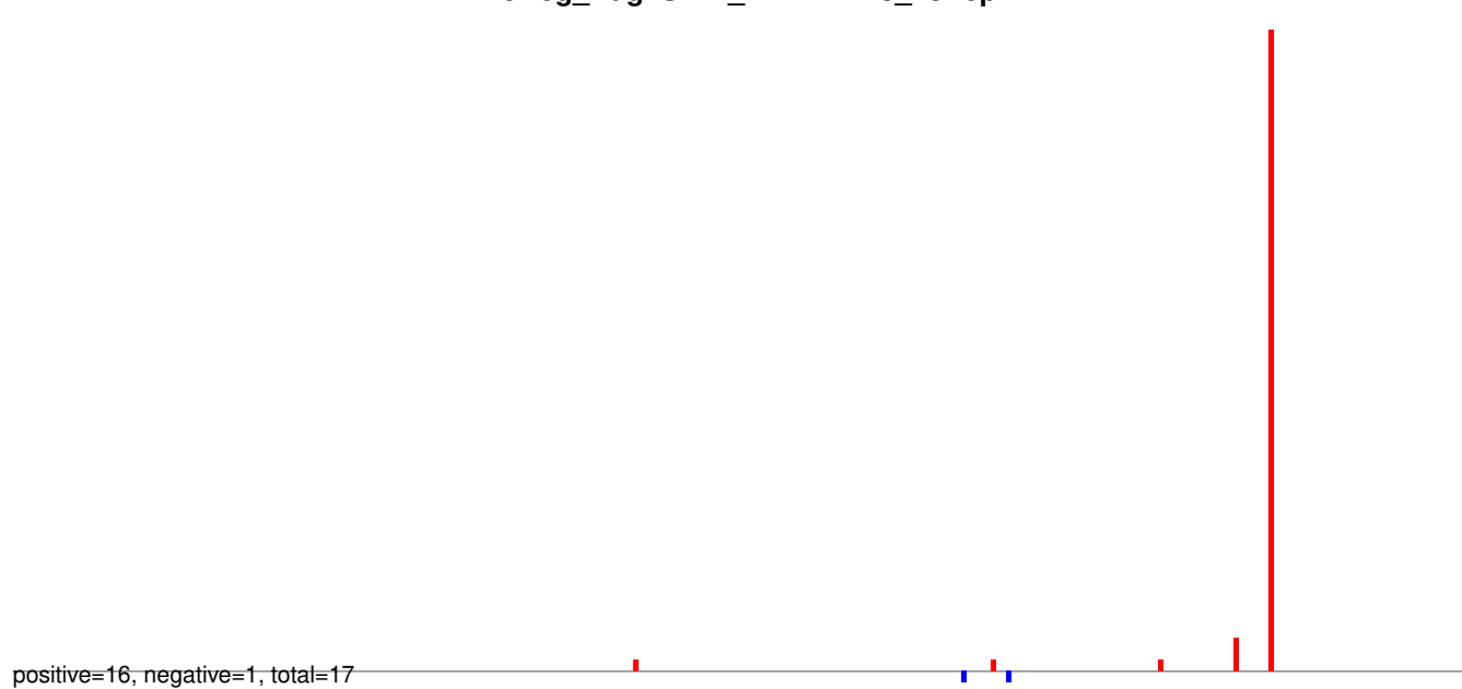
AeAeg_Aag2SINV_Piwi4.IP.24_35.rep
