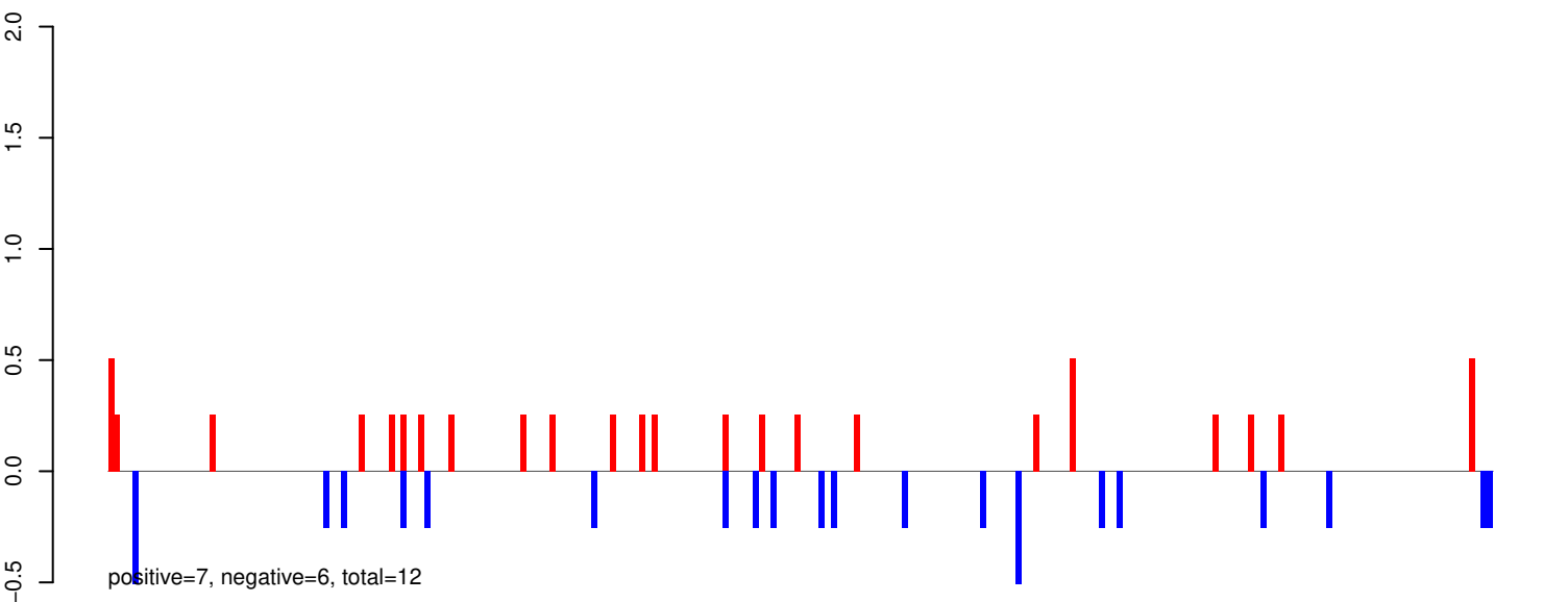
AeAeg_Aag2SINV_Piwi4.IP.24_35.rep
