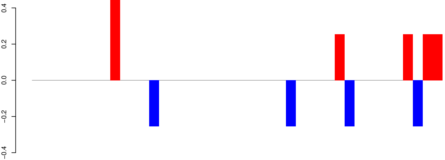
AeAeg_Aag2SINV_Piwi4.IP.24_35.rep
