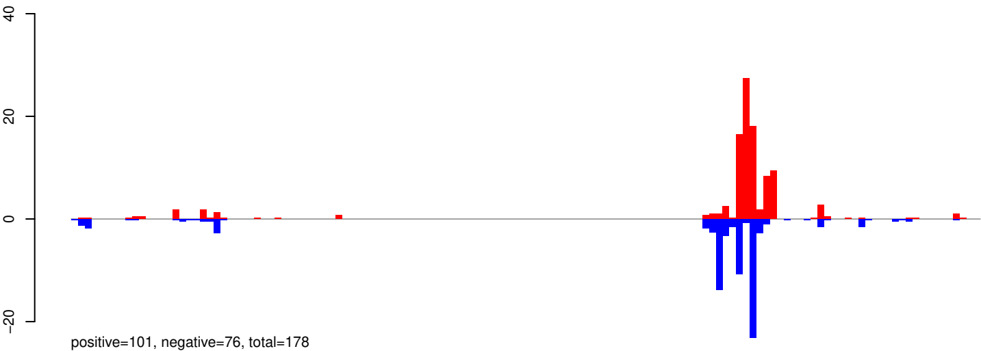
AeAeg_Aag2SINV_Piwi4.IP.24_35.rep
