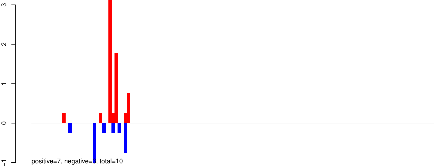
AeAeg_Aag2SINV_Piwi4.IP.24_35.rep
