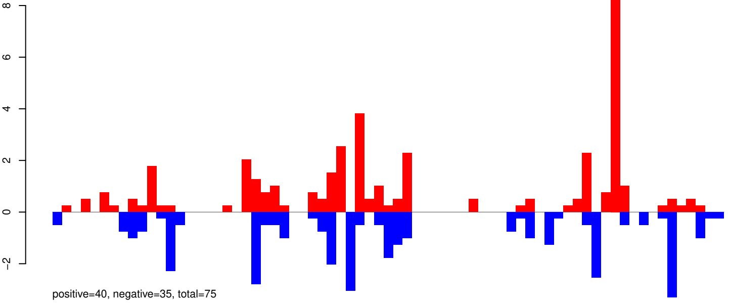
AeAeg_Aag2SINV_Piwi4.IP.24_35.rep
