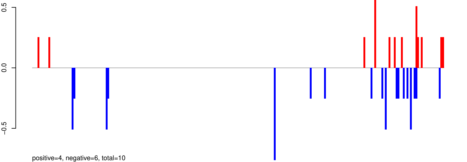
AeAeg_Aag2SINV_Piwi4.IP.24_35.rep
