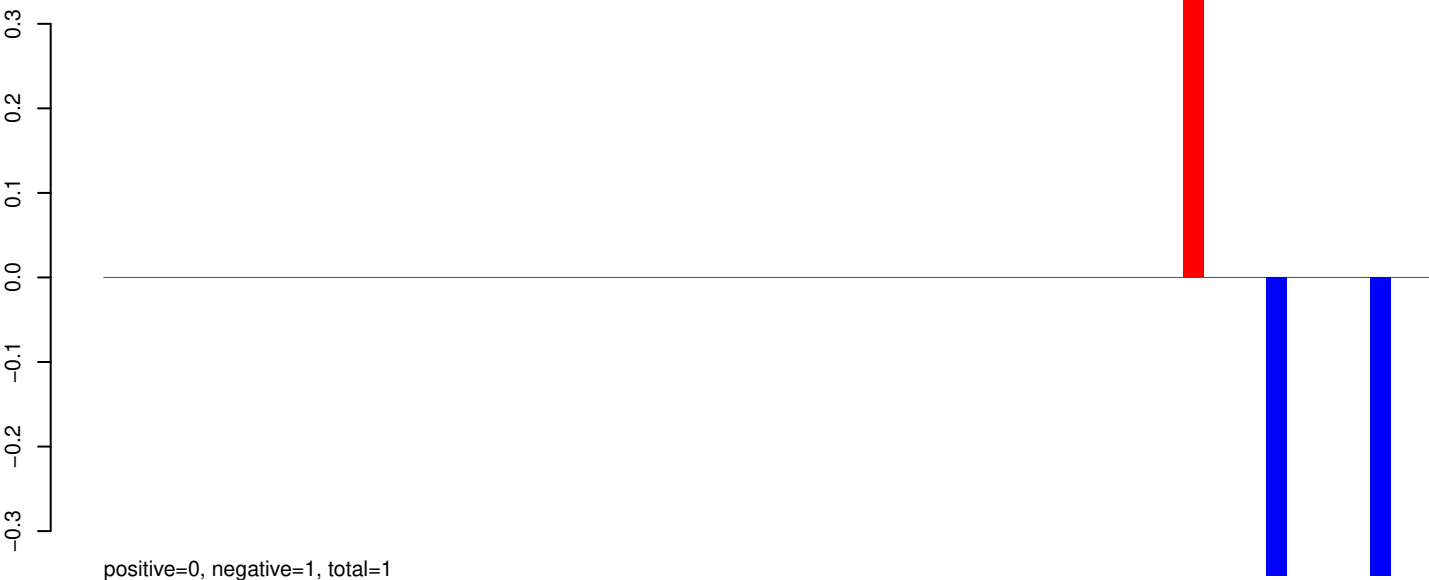
AeAeg_Aag2SINV_Piwi6.IP.24_35.rep
