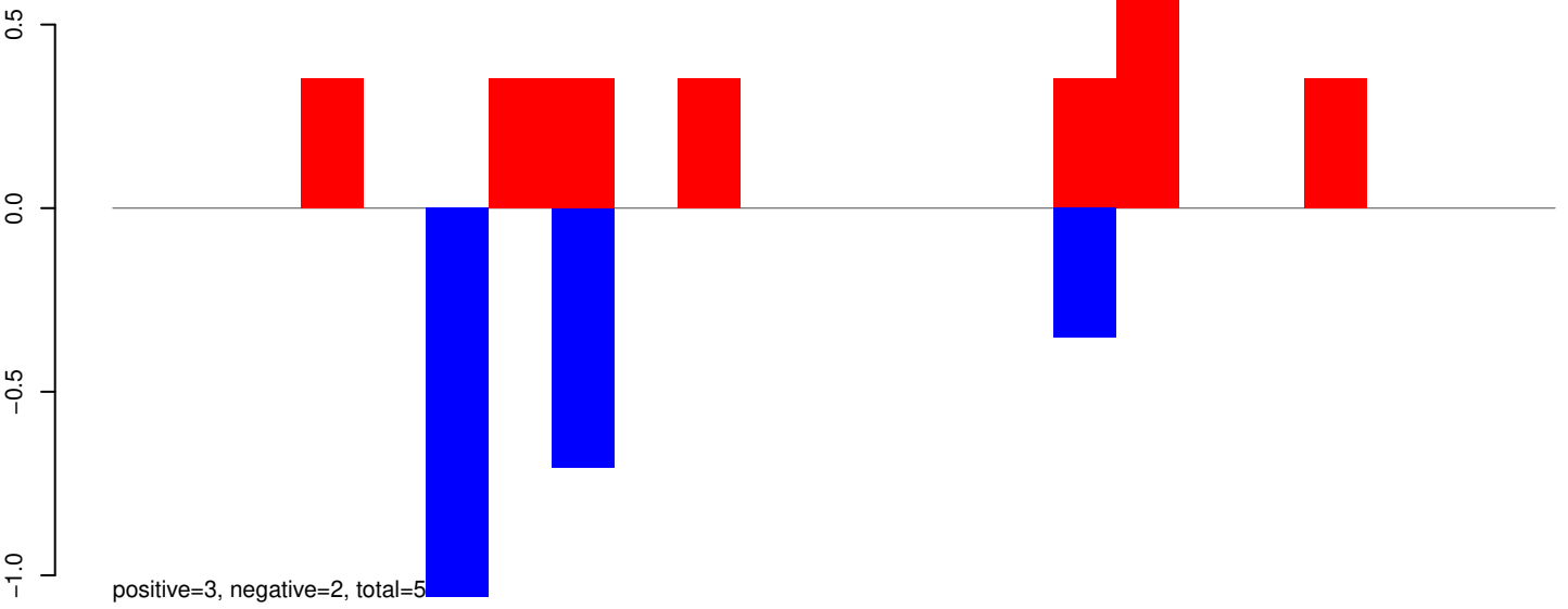
AeAeg_Aag2SINV_Piwi6.IP.24_35.rep
