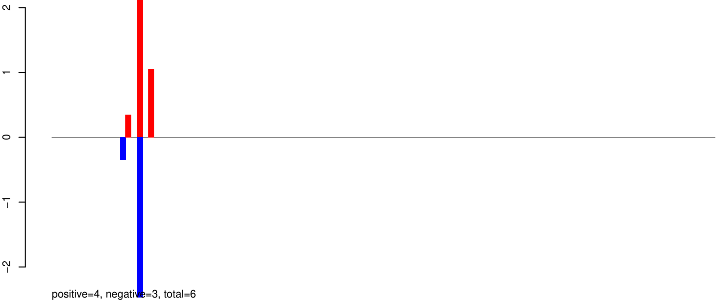
AeAeg_Aag2SINV_Piwi6.IP.24_35.rep
