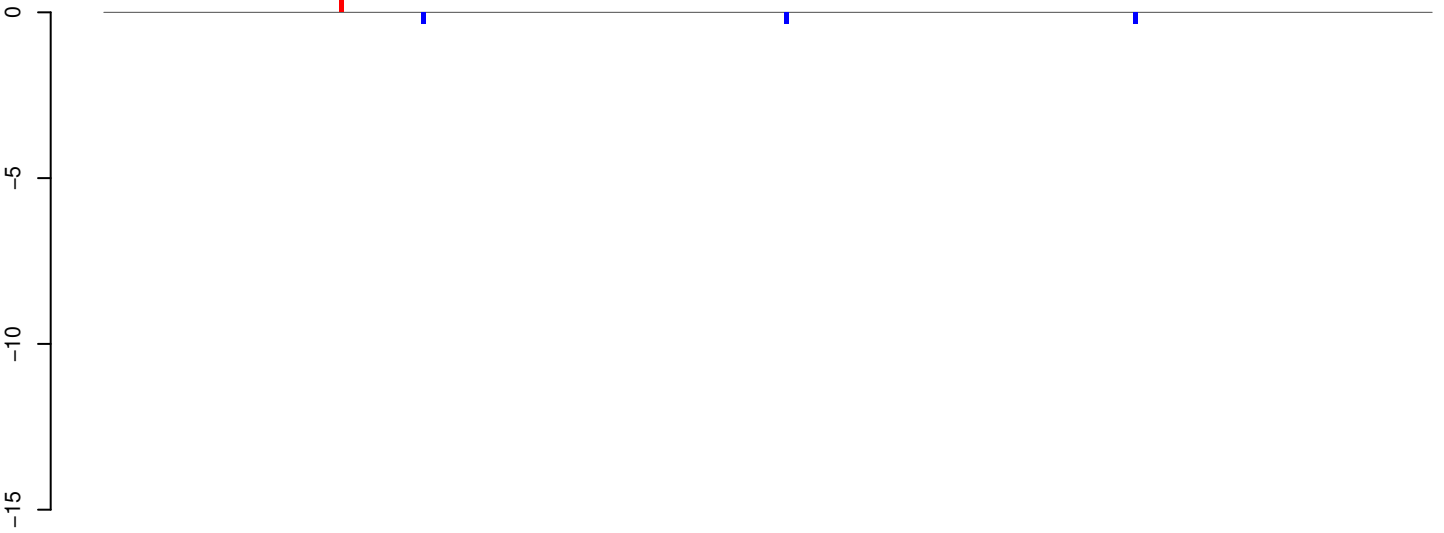
AeAeg_Aag2SINV_Piwi6.IP.18_23.rep
