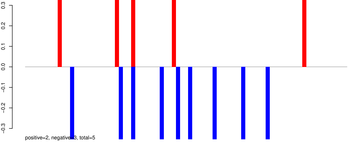
AeAeg_Aag2SINV_Piwi6.IP.24_35.rep
