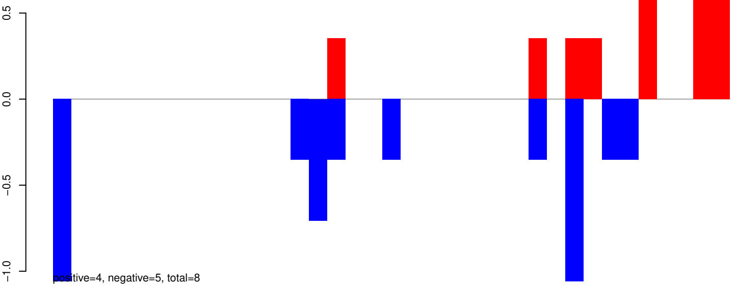
AeAeg_Aag2SINV_Piwi6.IP.24_35.rep
