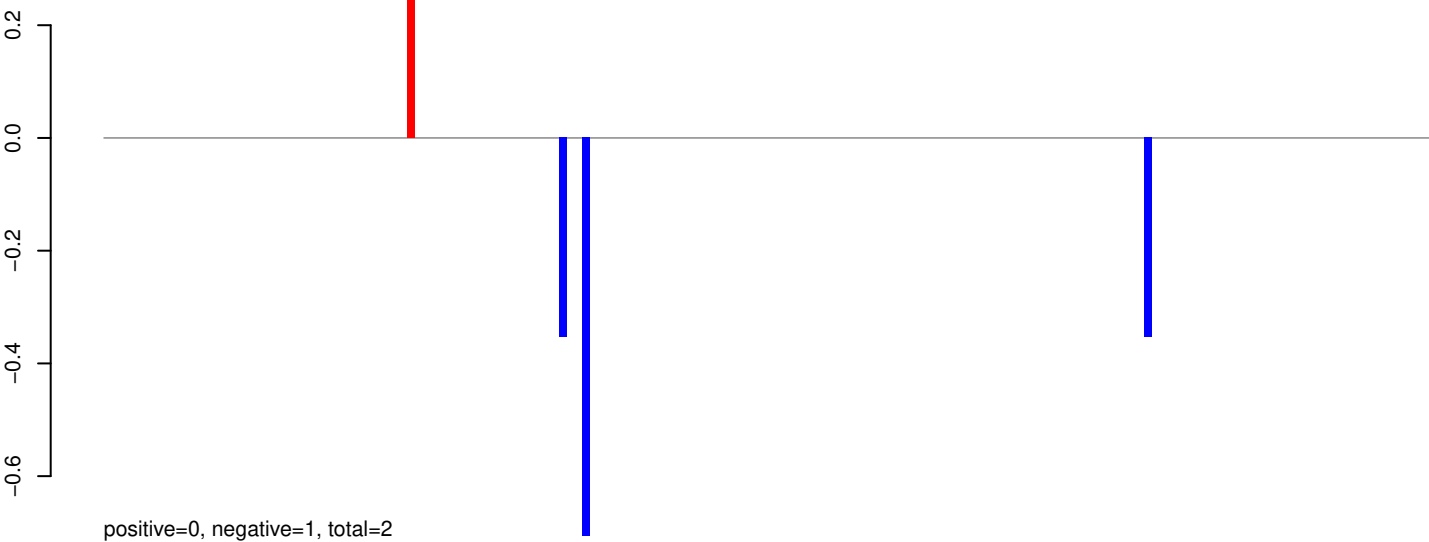
AeAeg_Aag2SINV_Piwi6.IP.24_35.rep
