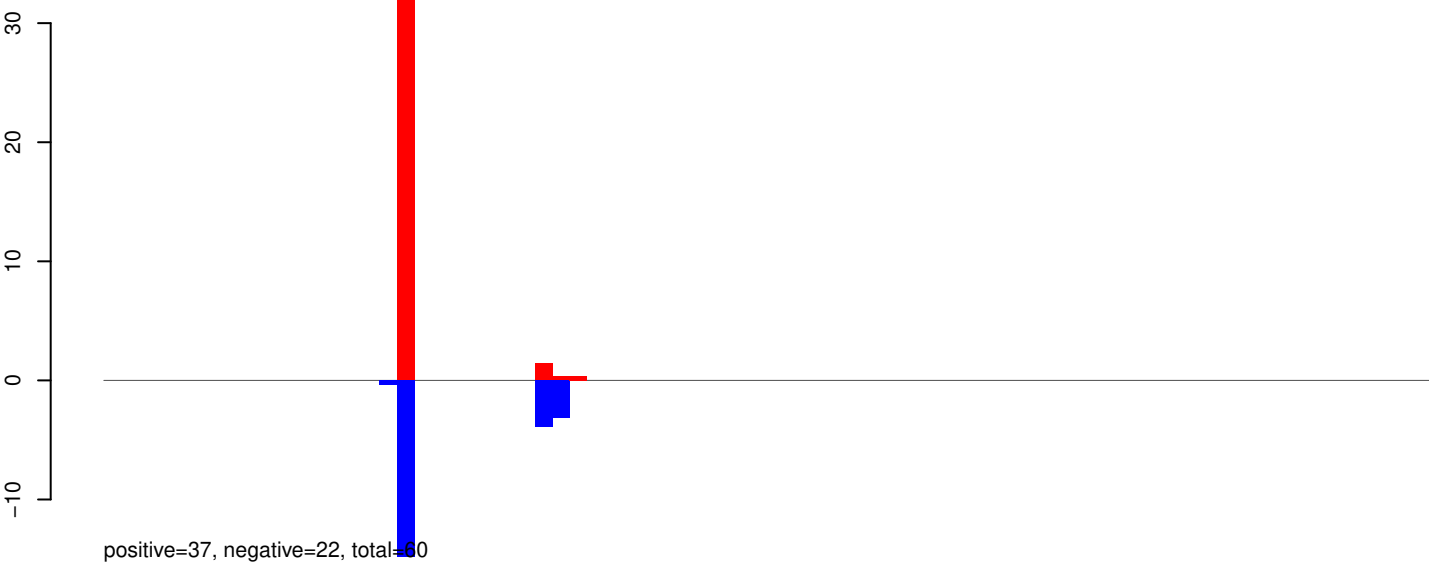
AeAeg_Aag2SINV_Piwi6.IP.24_35.rep
