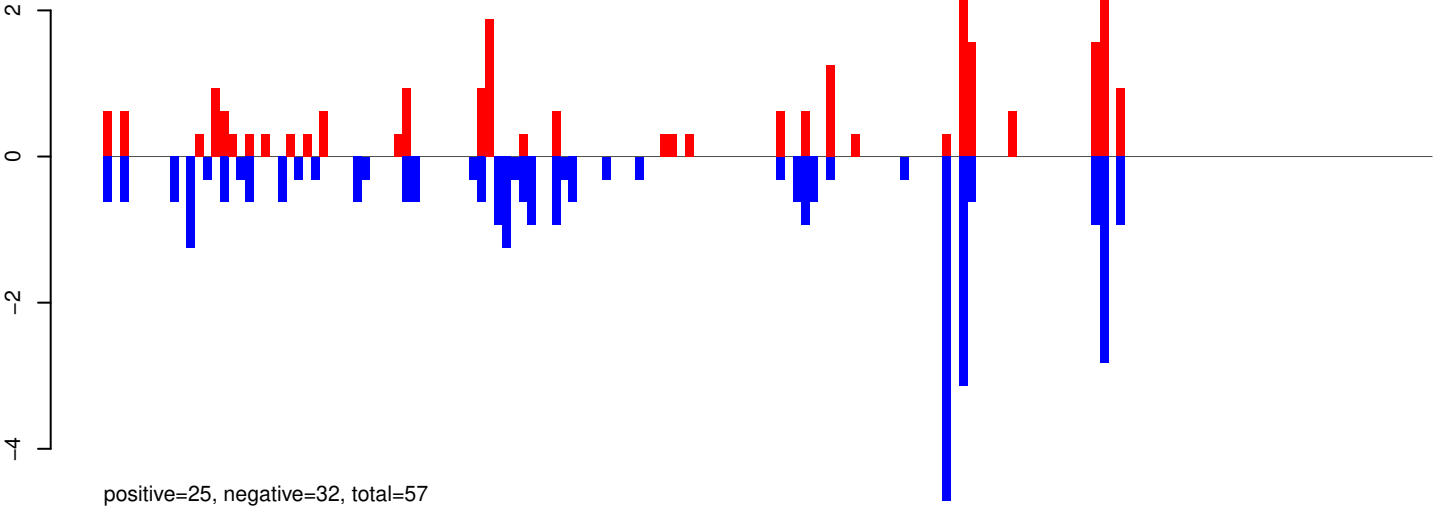
AeAeg_Aag2SINV_Piwi5.IP.24_35.rep
