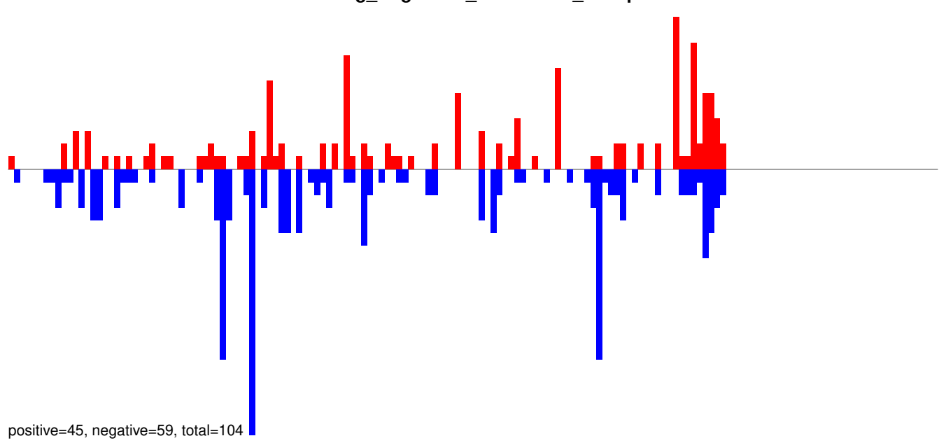
AeAeg_Aag2SINV_Piwi5.IP.24_35.rep
