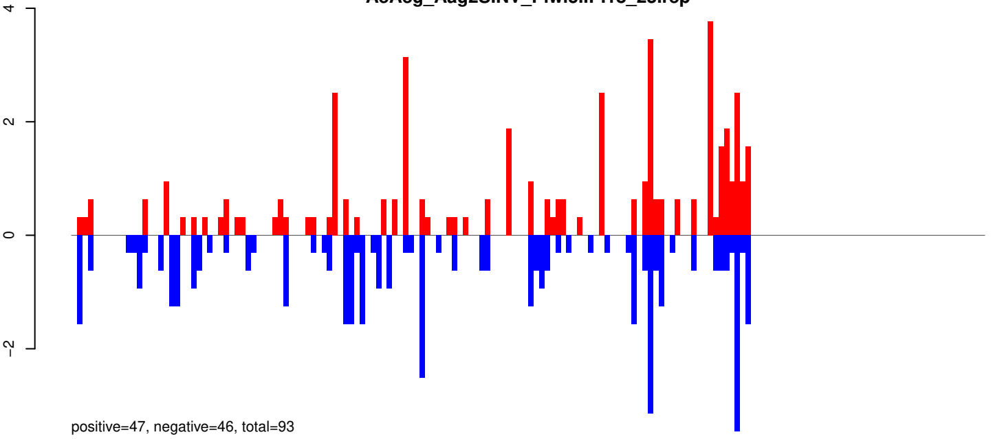
AeAeg_Aag2SINV_Piwi5.IP.24_35.rep
