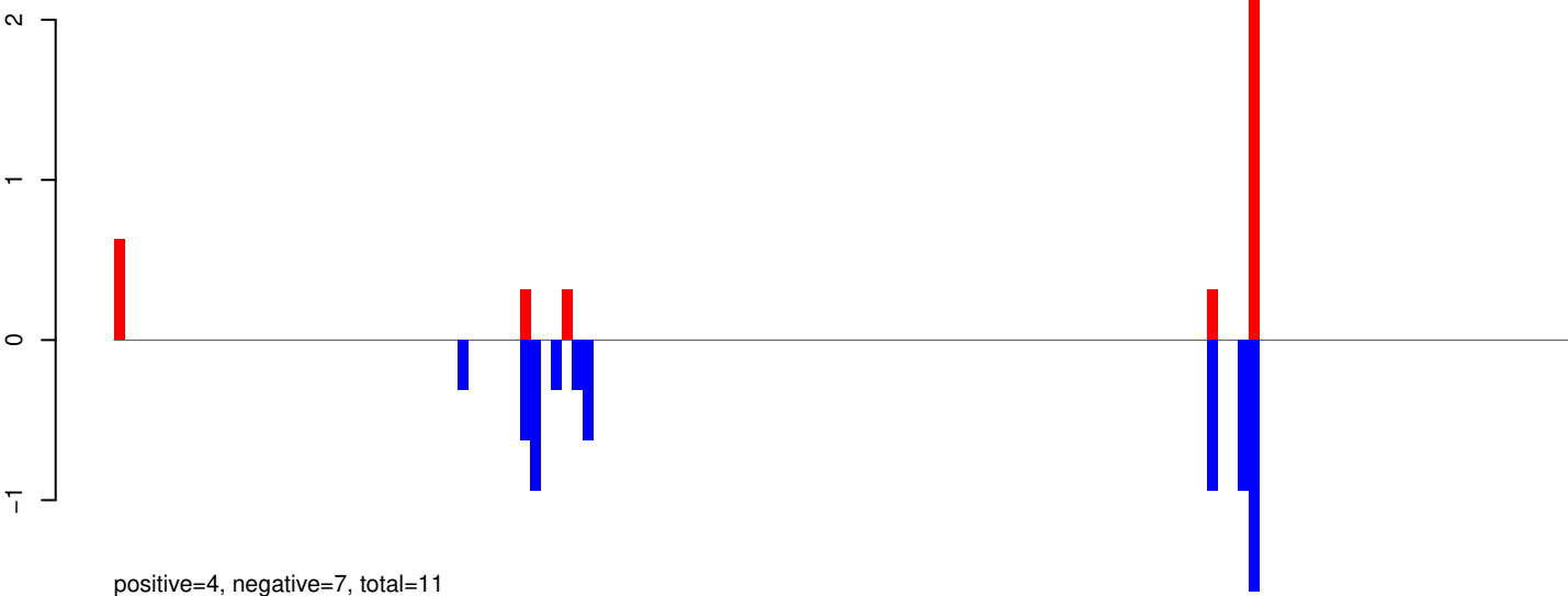
AeAeg_Aag2SINV_Piwi5.IP.24_35.rep
