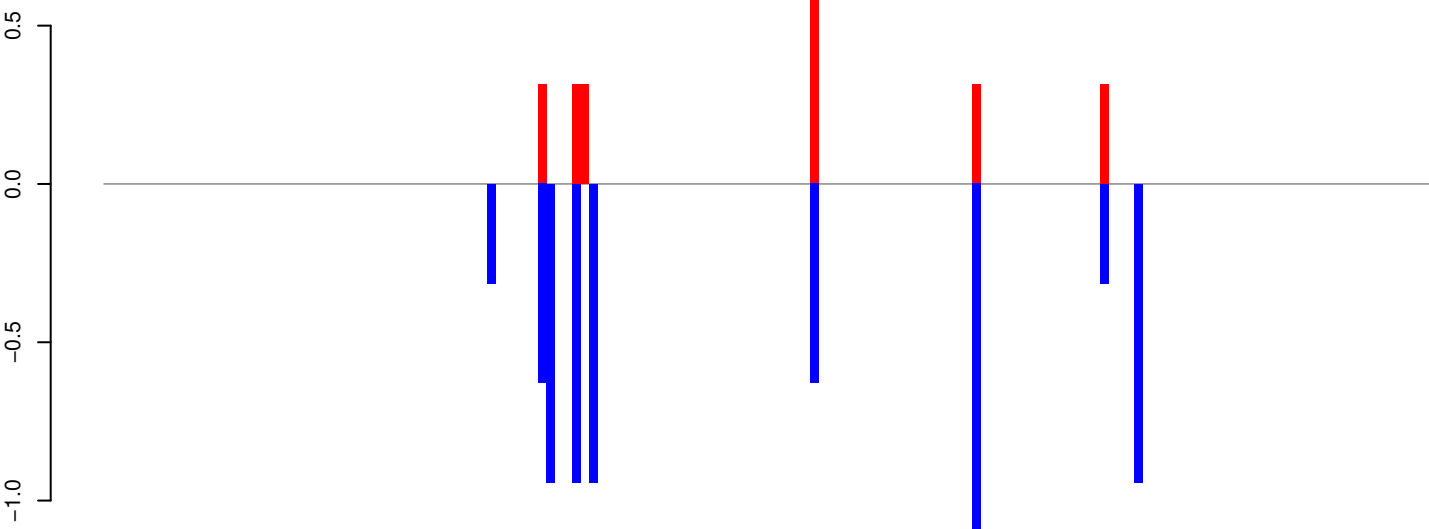
AeAeg_Aag2SINV_Piwi5.IP.18_23.rep
