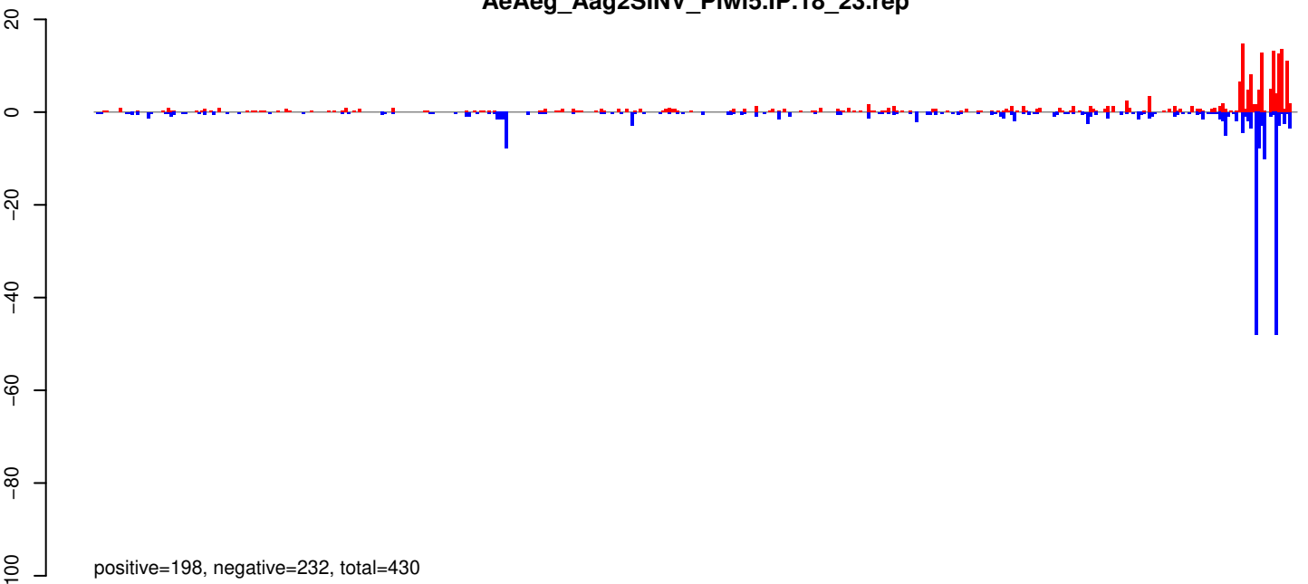
AeAeg_Aag2SINV_Piwi5.IP.24_35.rep
