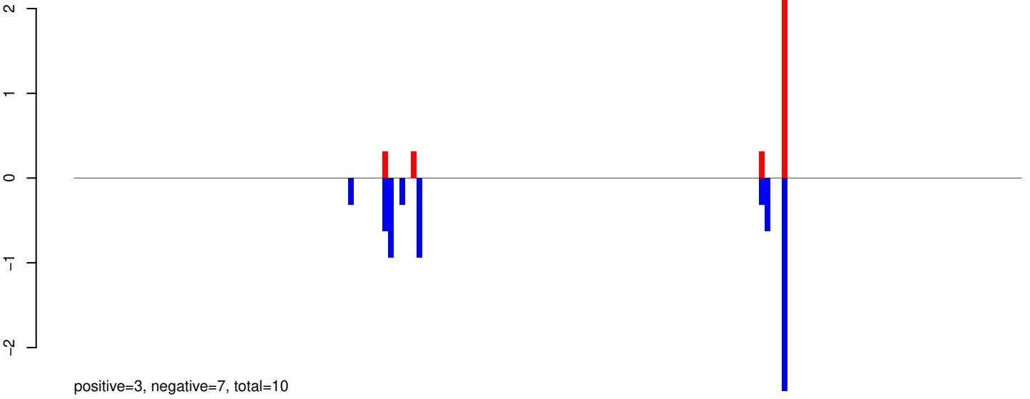
AeAeg_Aag2SINV_Piwi5.IP.24_35.rep
