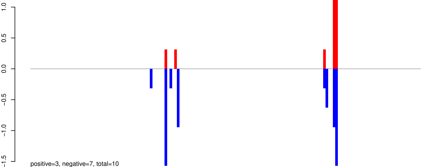
AeAeg_Aag2SINV_Piwi5.IP.24_35.rep
