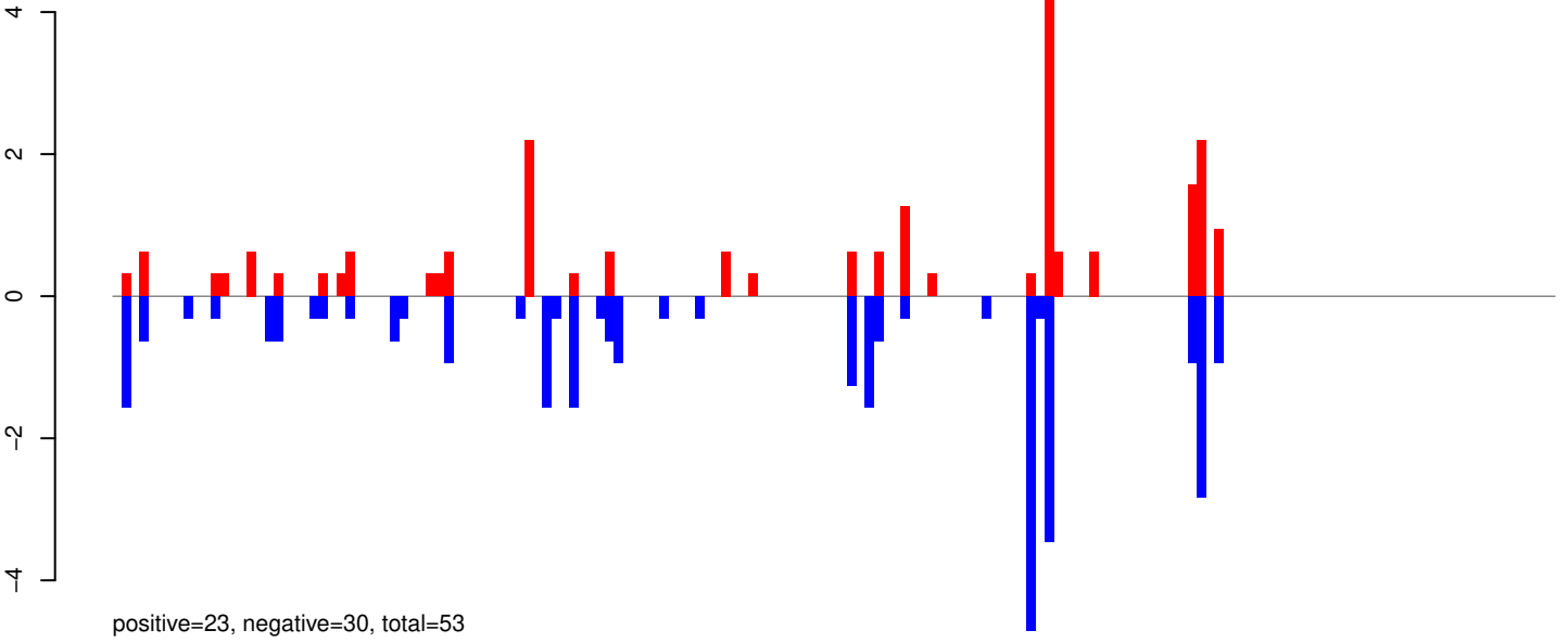
AeAeg_Aag2SINV_Piwi5.IP.24_35.rep
