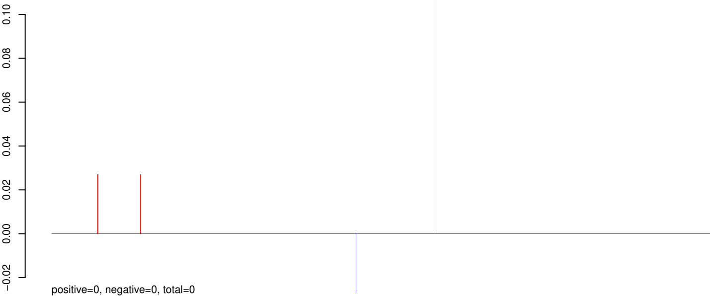
AeAlbo_BUNV_U4.4_rep1_ES.24_35.rep
