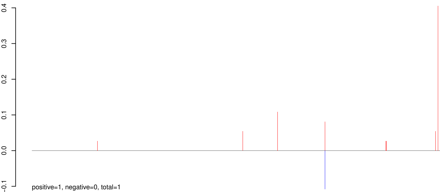
AeAlbo_BUNV_U4.4_rep1_ES.24_35.rep
