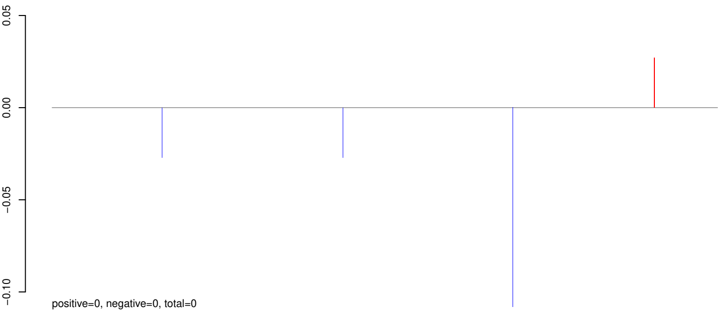
AeAlbo_BUNV_U4.4_rep1_ES.24_35.rep
