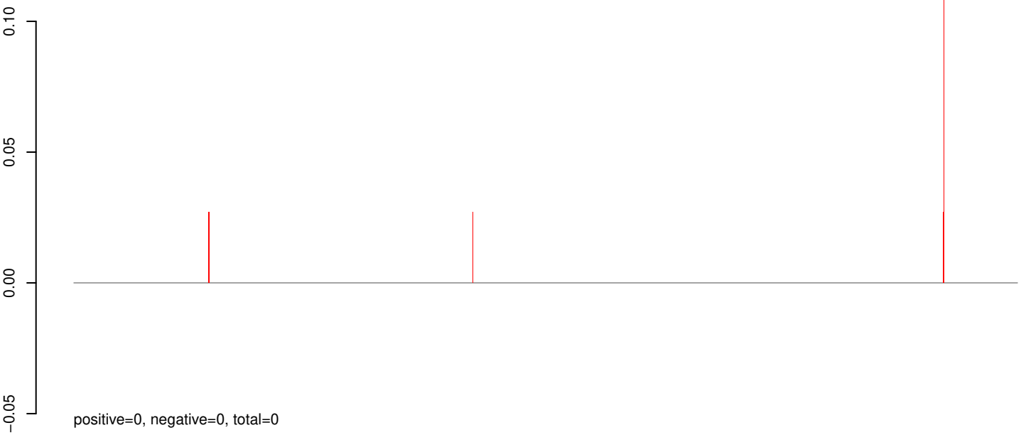
AeAlbo_BUNV_U4.4_rep1_ES.24_35.rep
