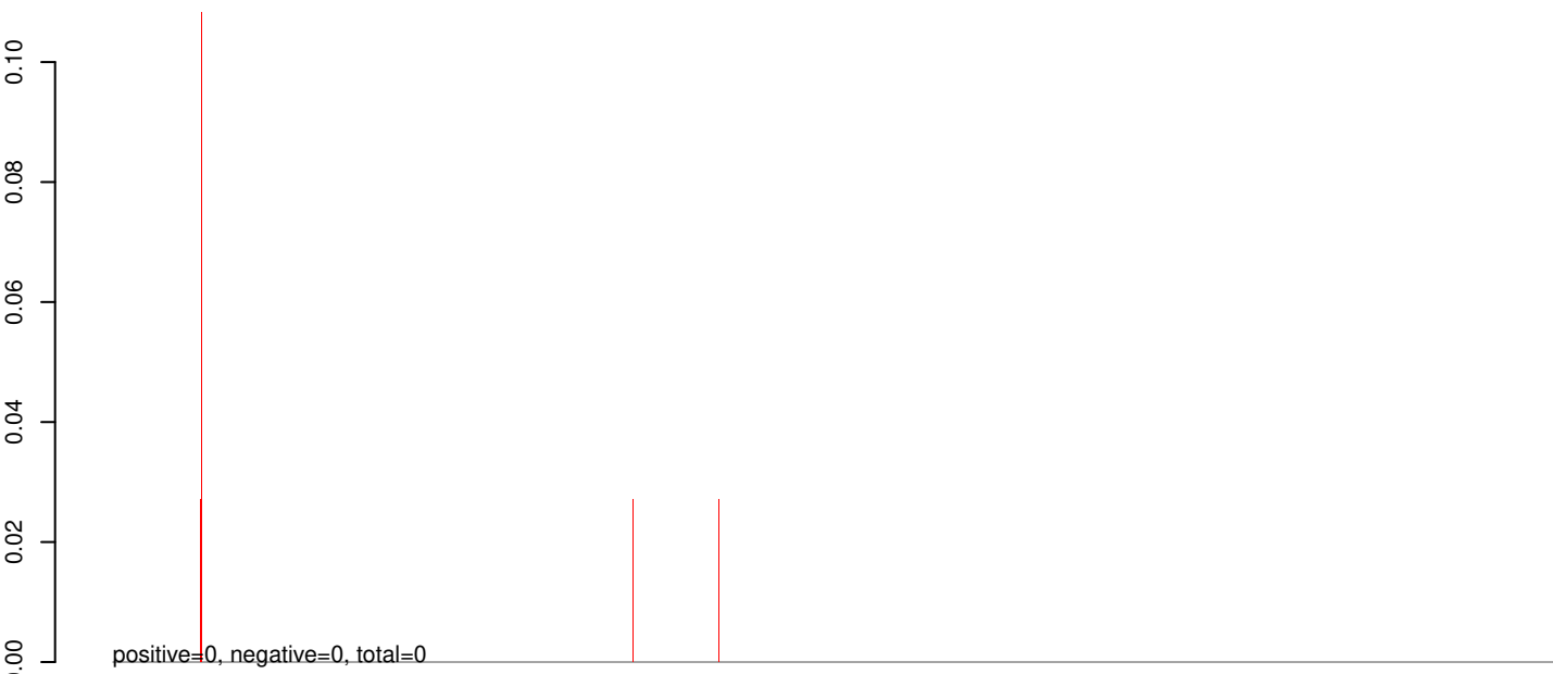
AeAlbo_BUNV_U4.4_rep1_ES.24_35.rep
