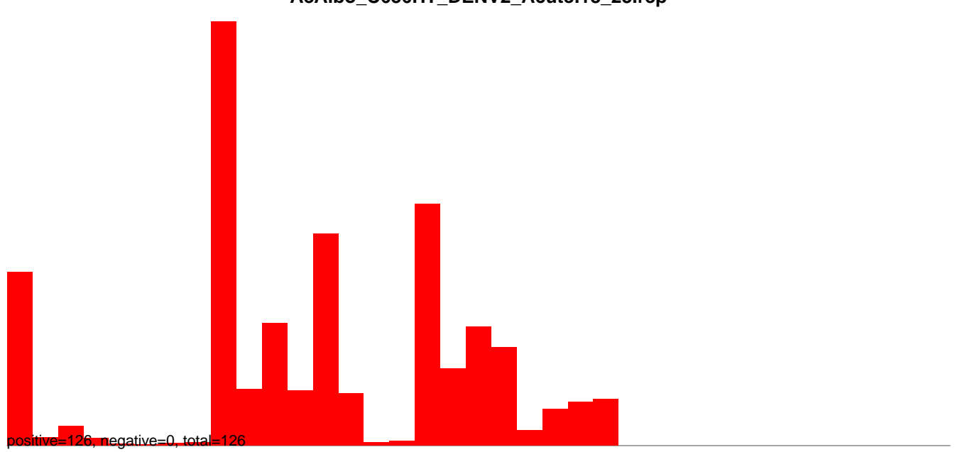
AeAlbo_C636HT_DENV2_Acute.24_35.rep
