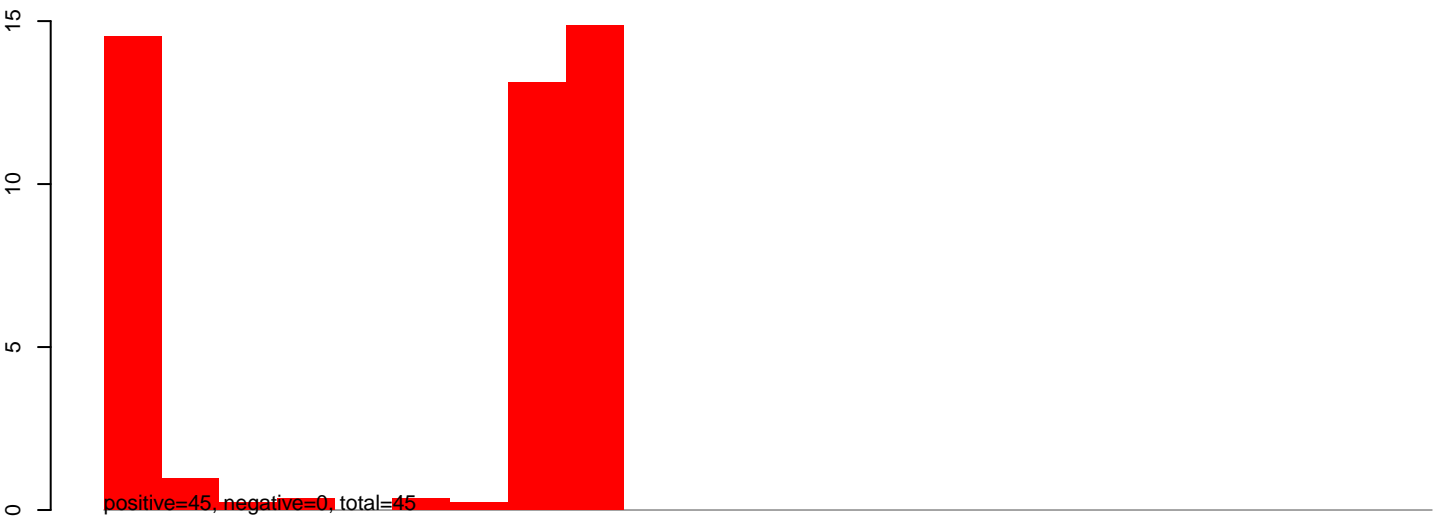
AeAlbo_C636HT_DENV2_Acute.24_35.rep
