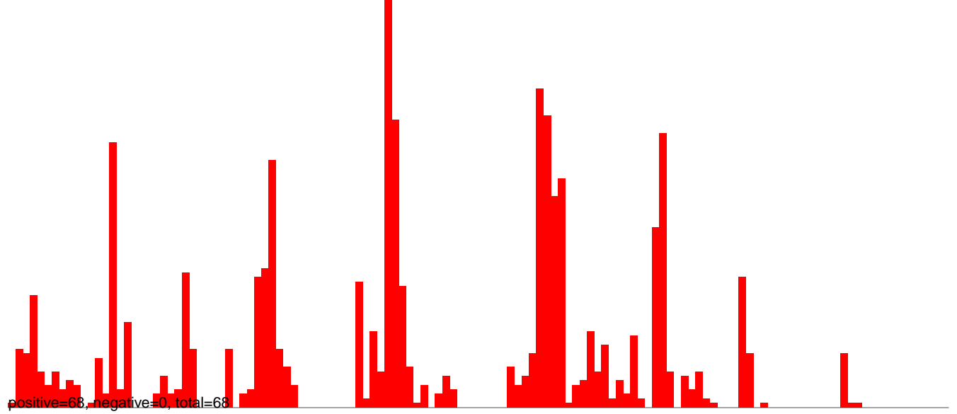
AeAlbo_C636HT_DENV2_Acute.24_35.rep
