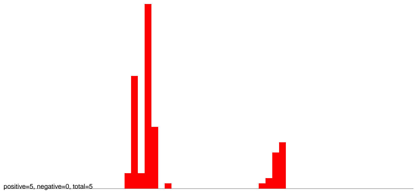
AeAlbo_C636HT_DENV2_Acute.24_35.rep
