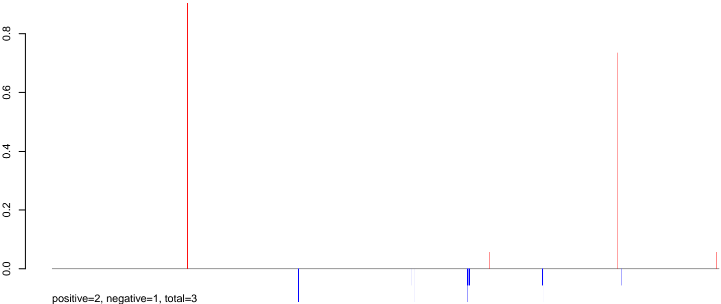
AeAlbo_C636HT_DENV2_Acute.24_35.rep
