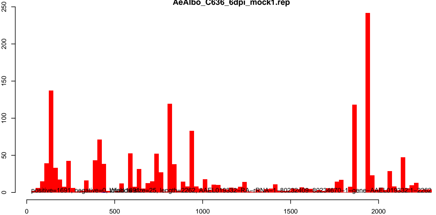
AeAlbo_C636_6dpi_mock1.rep
