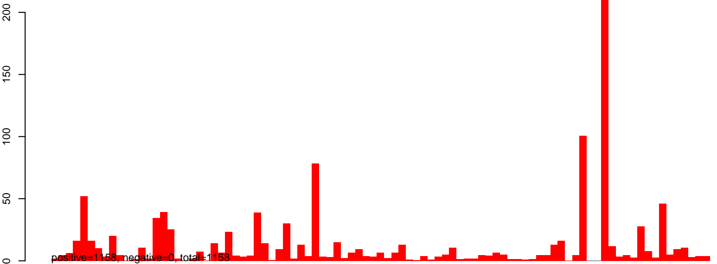
AeAlbo_C636_6dpi_mock1.24_35.rep
