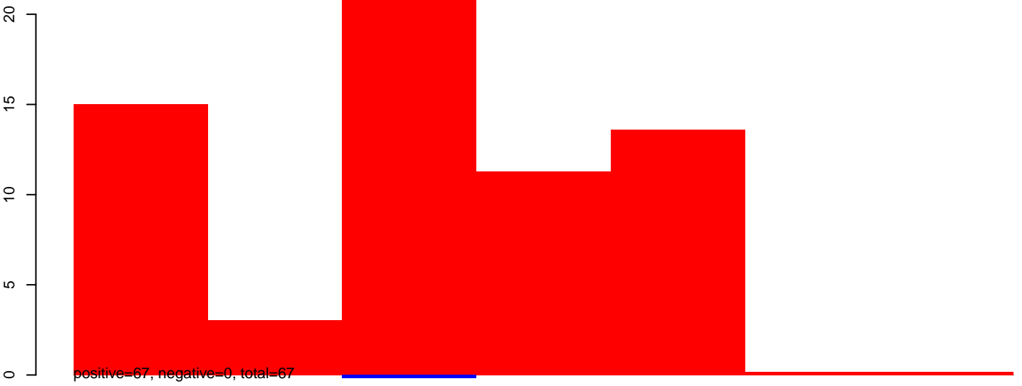
AeAlbo_C636_6dpi_mock1.24_35.rep
