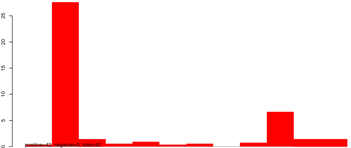
AeAlbo_C636_6dpi_mock1.24_35.rep
