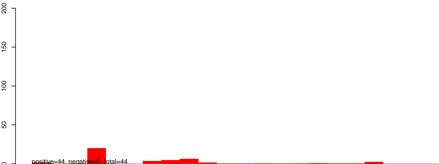
AeAlbo_C636_6dpi_mock1.rep
