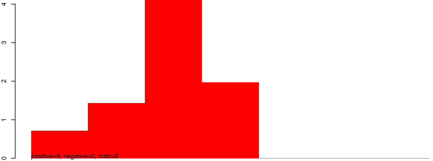
AeAlbo_C636_6dpi_mock1.24_35.rep
