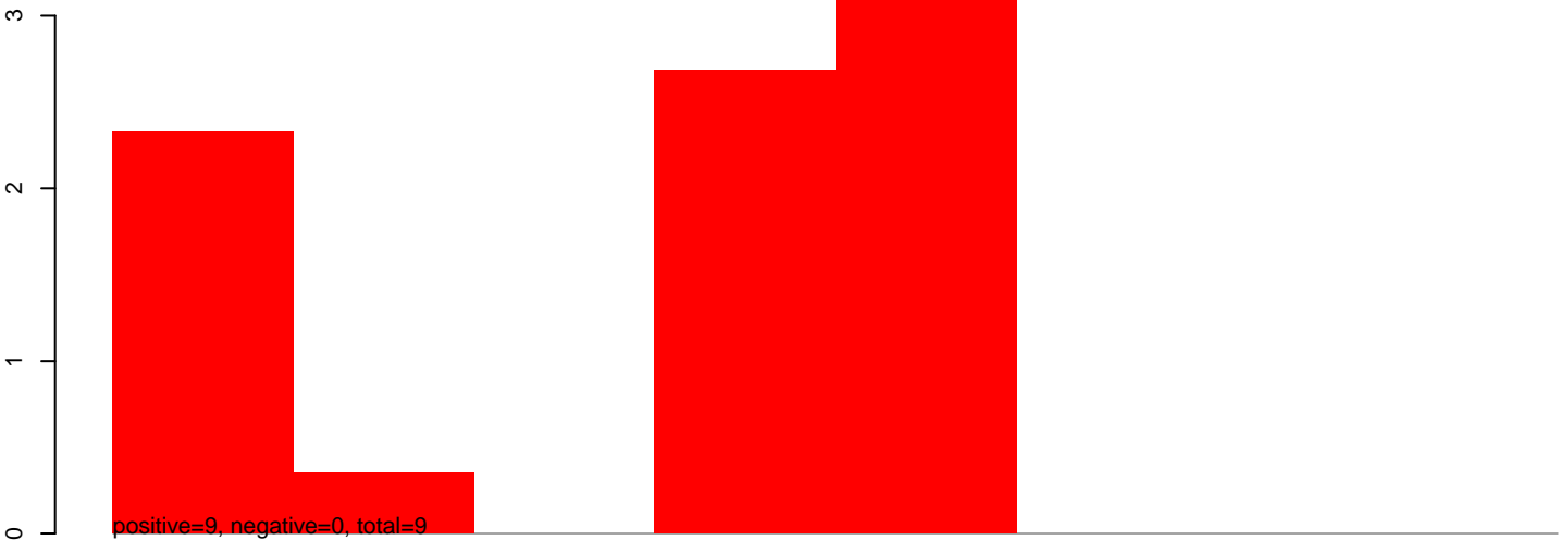
AeAlbo_C636_6dpi_mock1.24_35.rep
