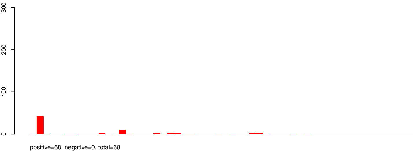
AeAlbo_C636_6dpi_mock1.rep
