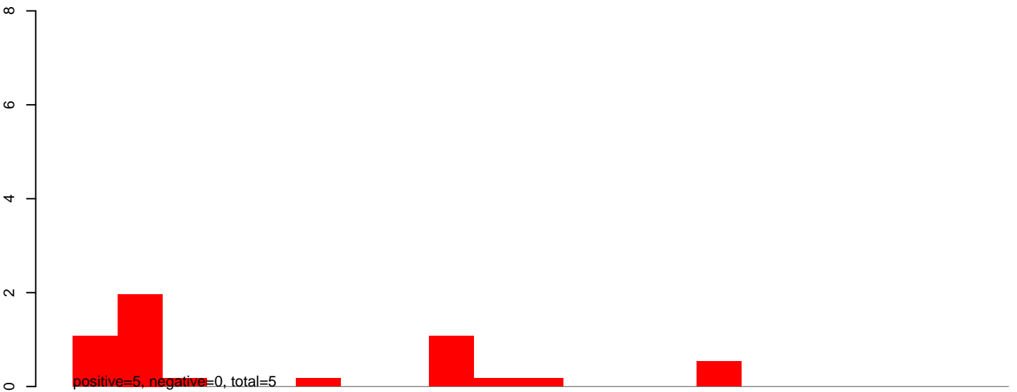
AeAlbo_C636_6dpi_mock1.rep
