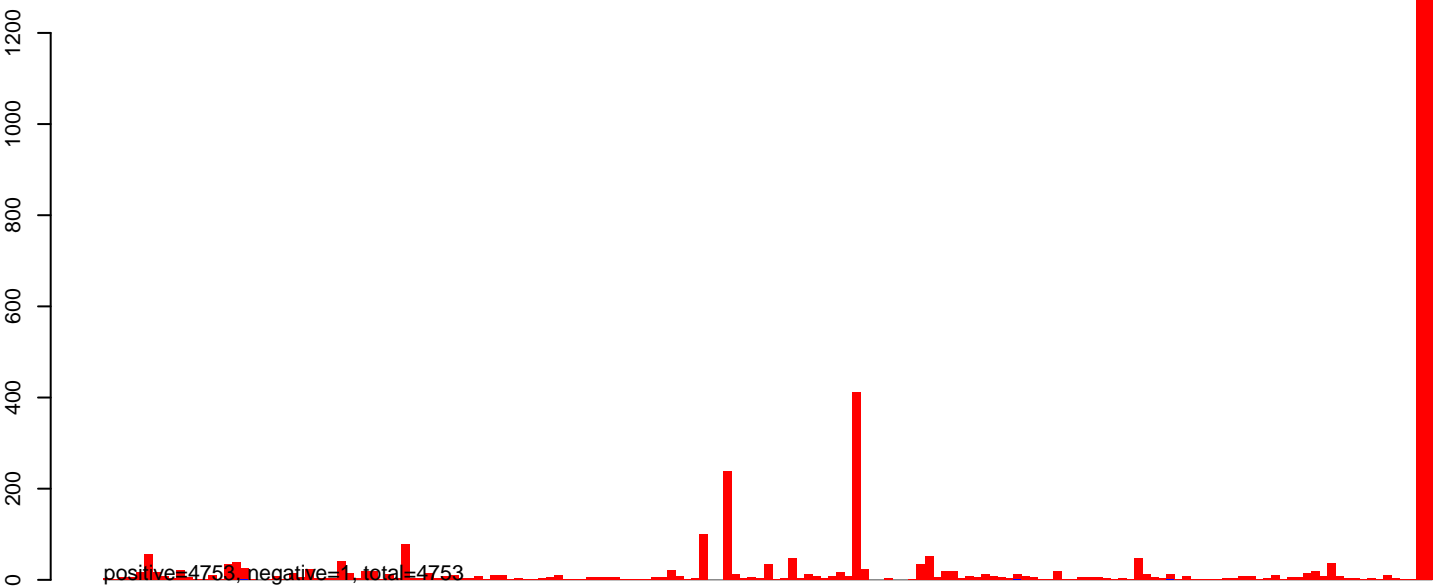
AeAlbo_C636_6dpi_mock1.24_35.rep
