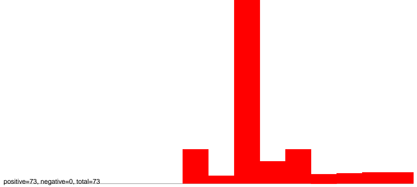
AeAlbo_C636_6dpi_mock1.24_35.rep
