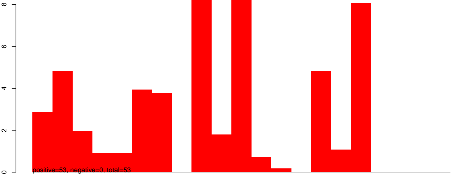
AeAlbo_C636_6dpi_mock1.24_35.rep
