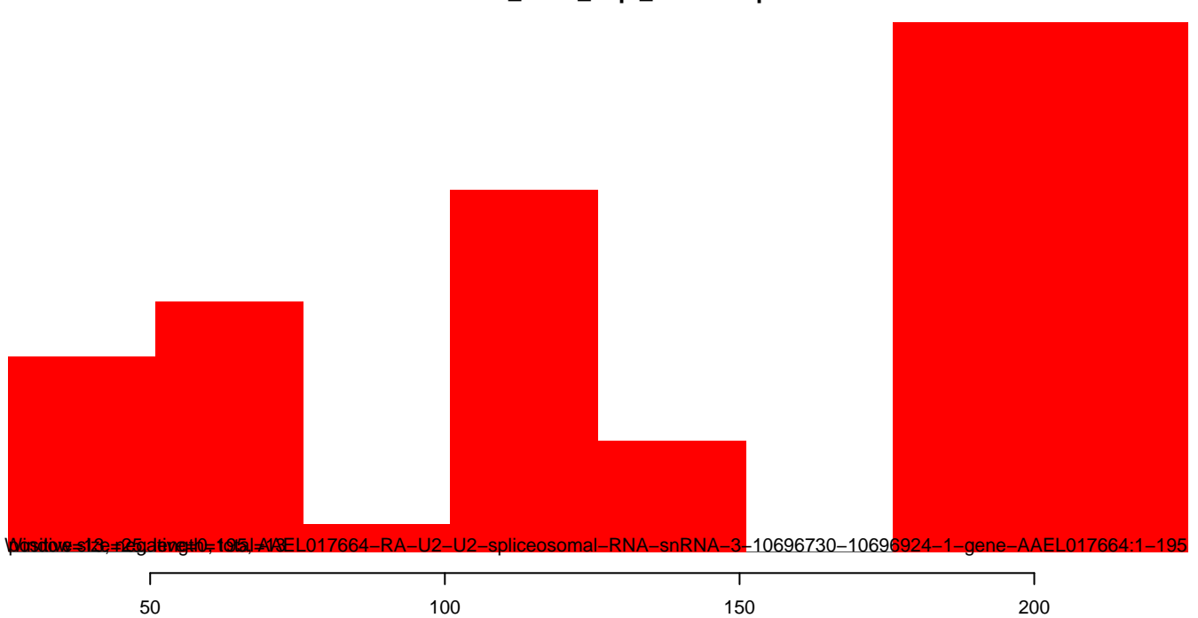
AeAlbo_C636_6dpi_mock1.rep
