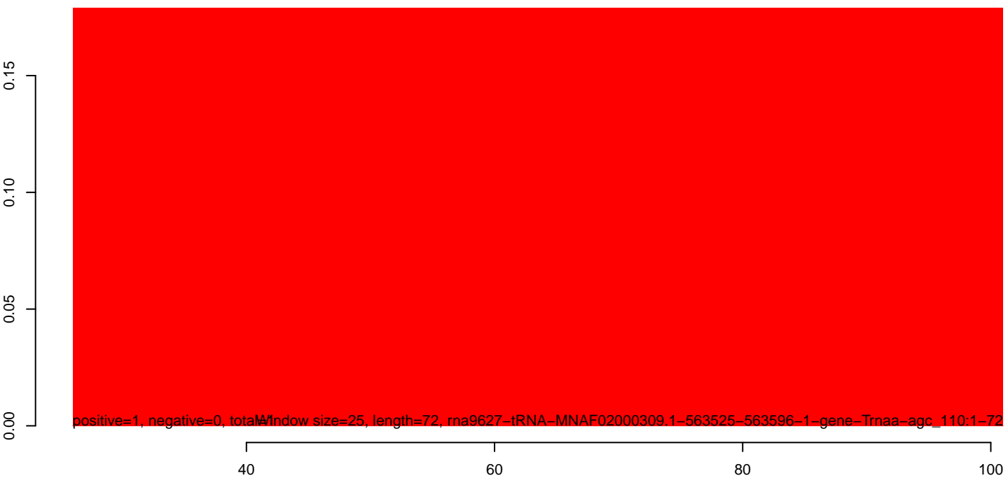
AeAlbo_C636_6dpi_mock1.rep
