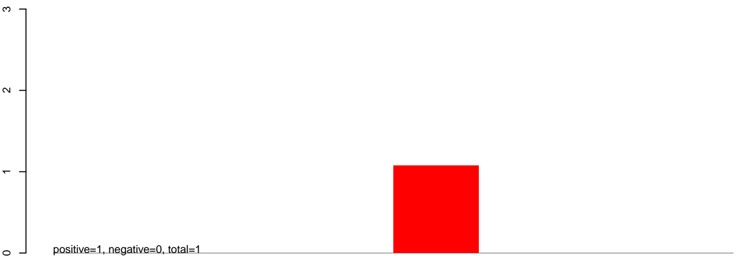
AeAlbo_C636_6dpi_mock1.rep
