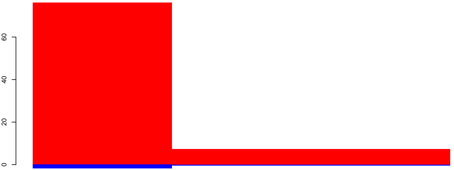
AeAlbo_C636_6dpi_mock1.18_23.rep
