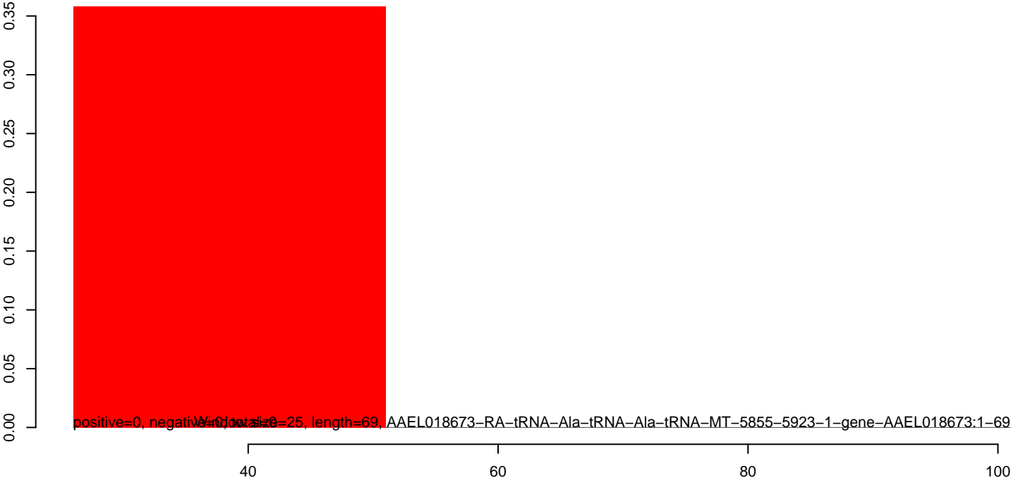
AeAlbo_C636_6dpi_mock1.rep
