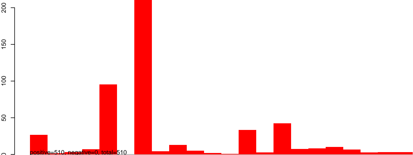
AeAlbo_C636_6dpi_mock1.24_35.rep
