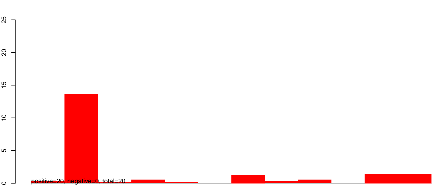
AeAlbo_C636_6dpi_mock1.rep
