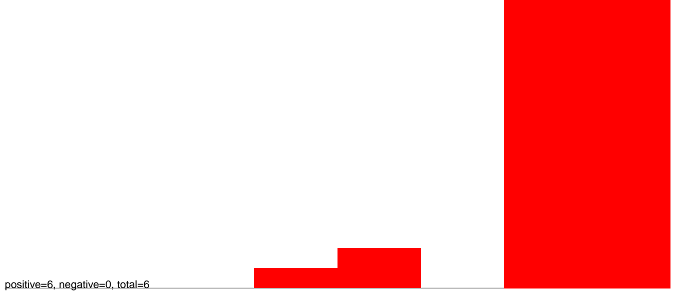
AeAlbo_C636_6dpi_mock1.rep
