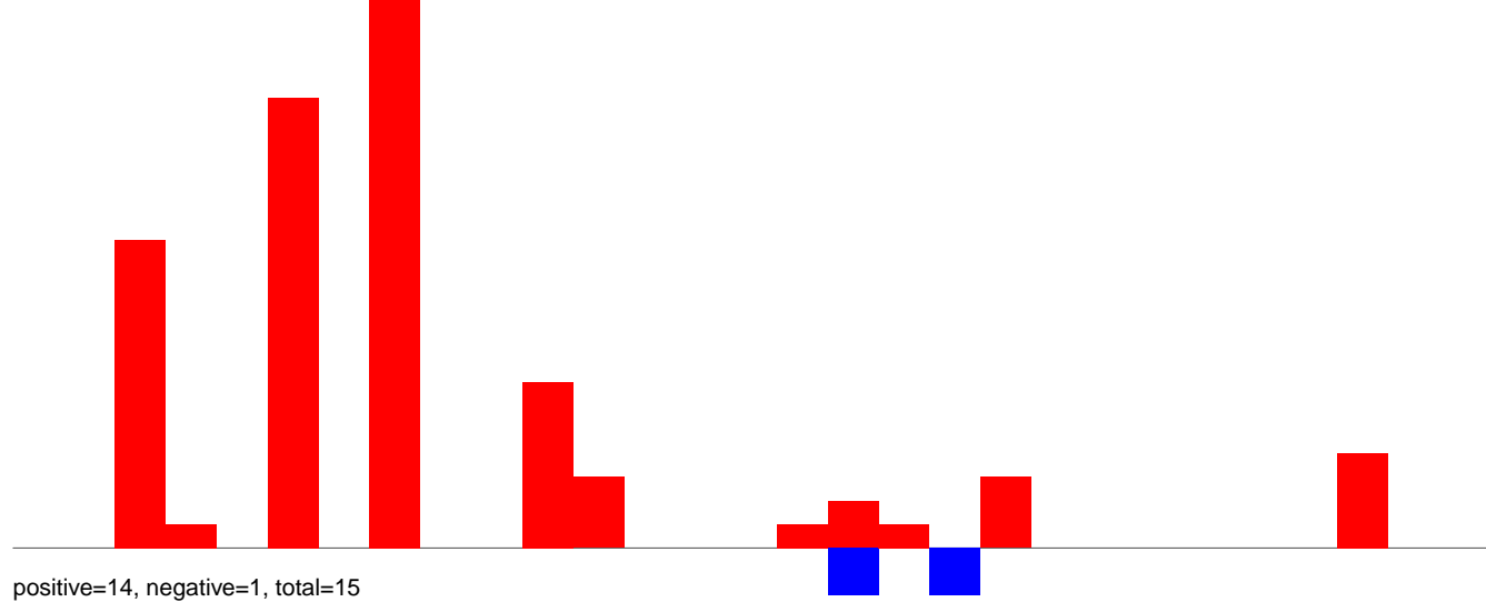
AeAlbo_C636_6dpi_mock1.24_35.rep
