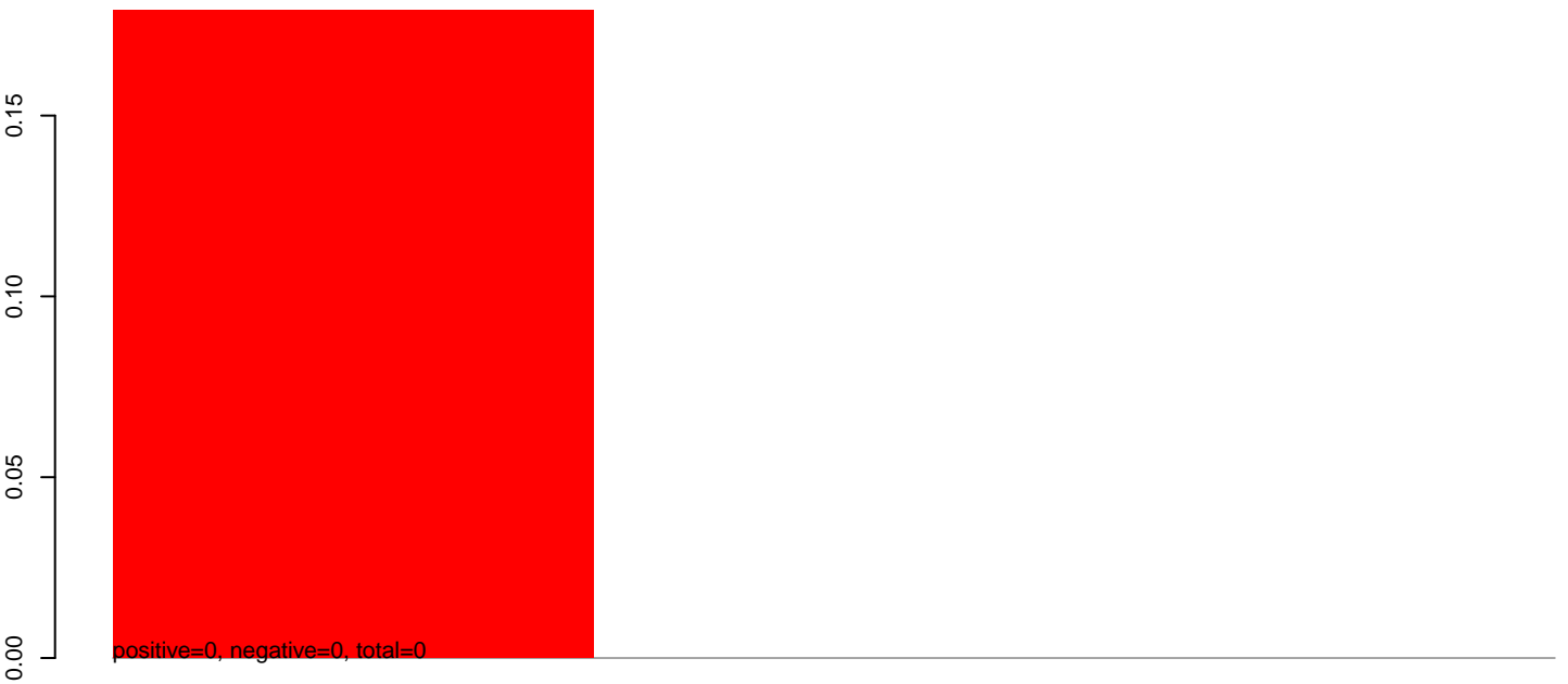
AeAlbo_C636_6dpi_mock1.24_35.rep
