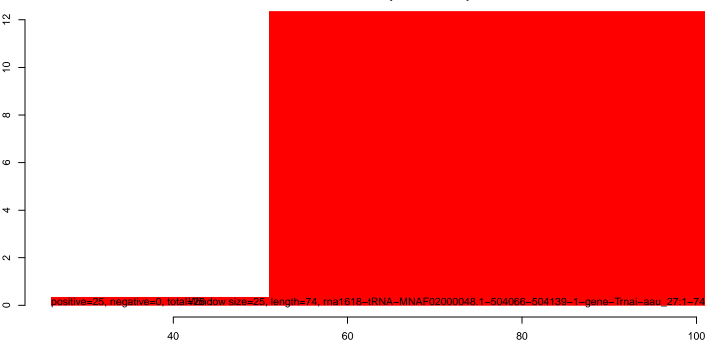
AeAlbo_C636_6dpi_mock1.rep
