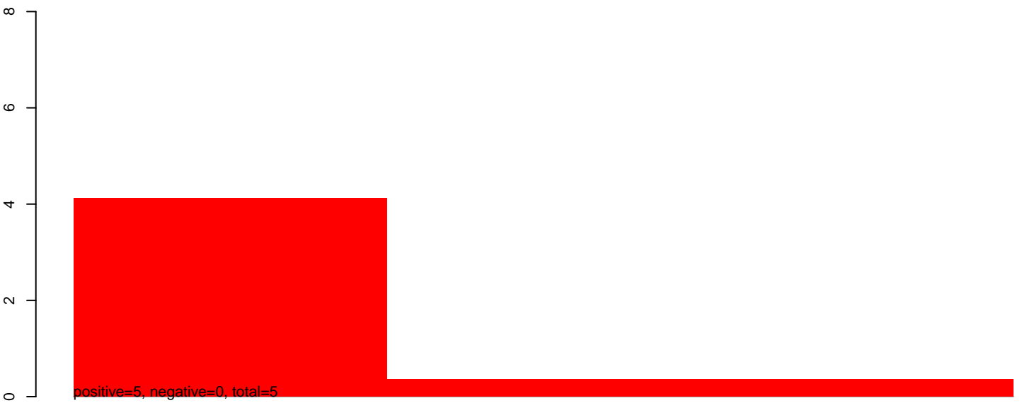
AeAlbo_C636_6dpi_mock1.24_35.rep
