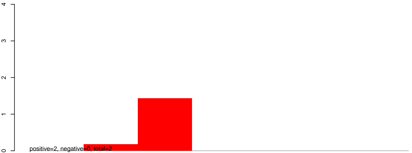
AeAlbo_C636_6dpi_mock1.rep
