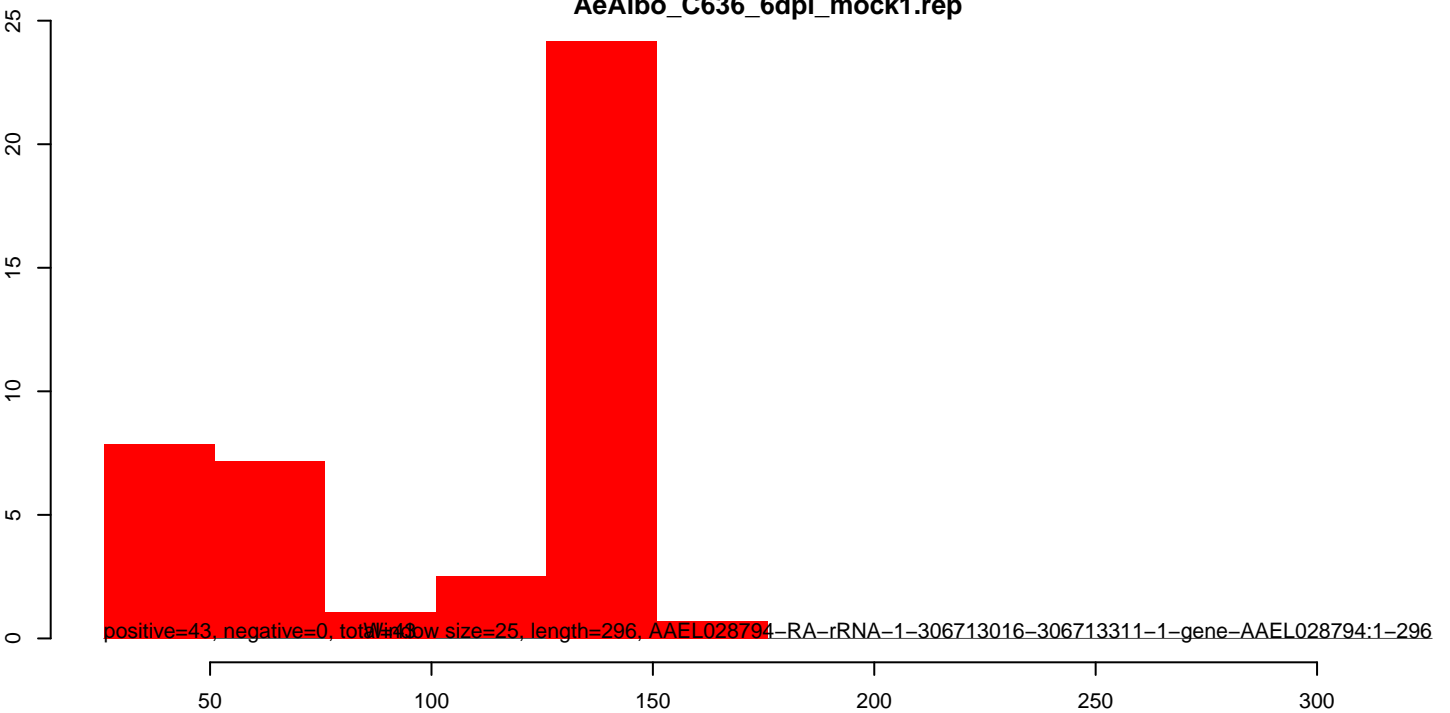
AeAlbo_C636_6dpi_mock1.rep
