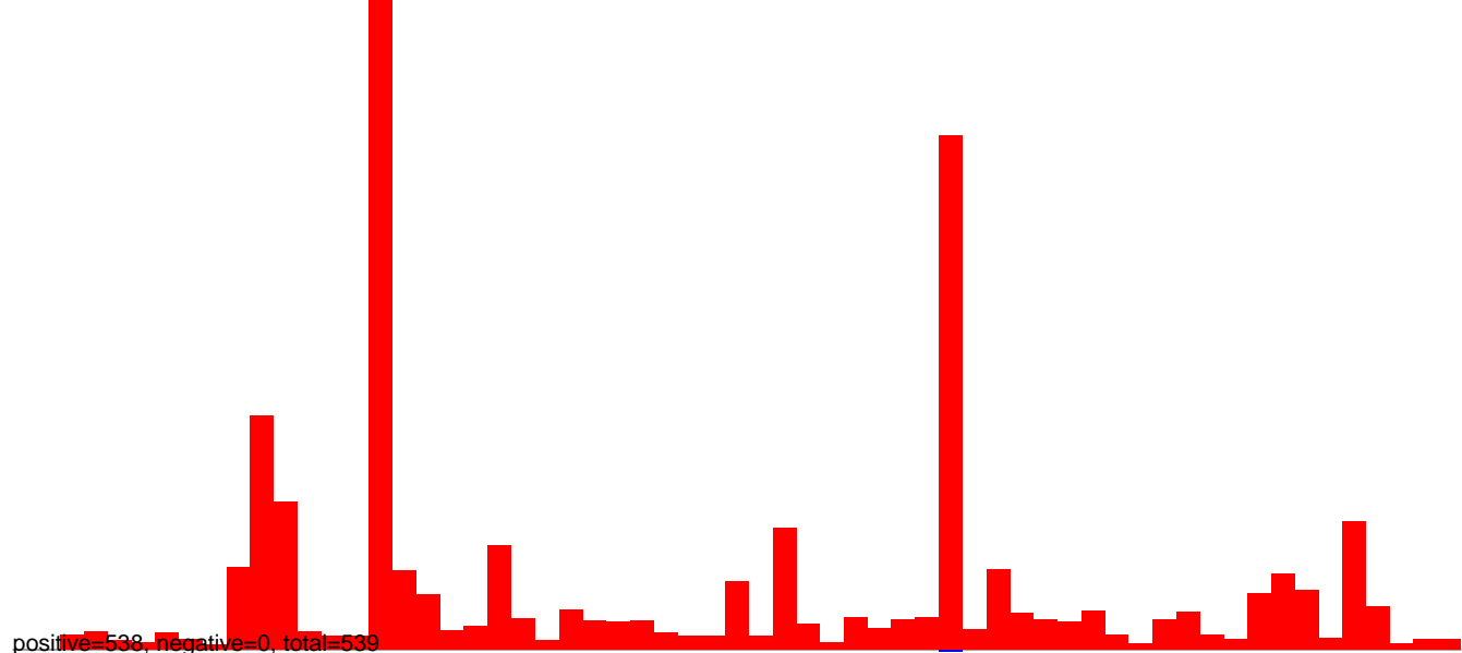
AeAlbo_C636_6dpi_mock1.24_35.rep
