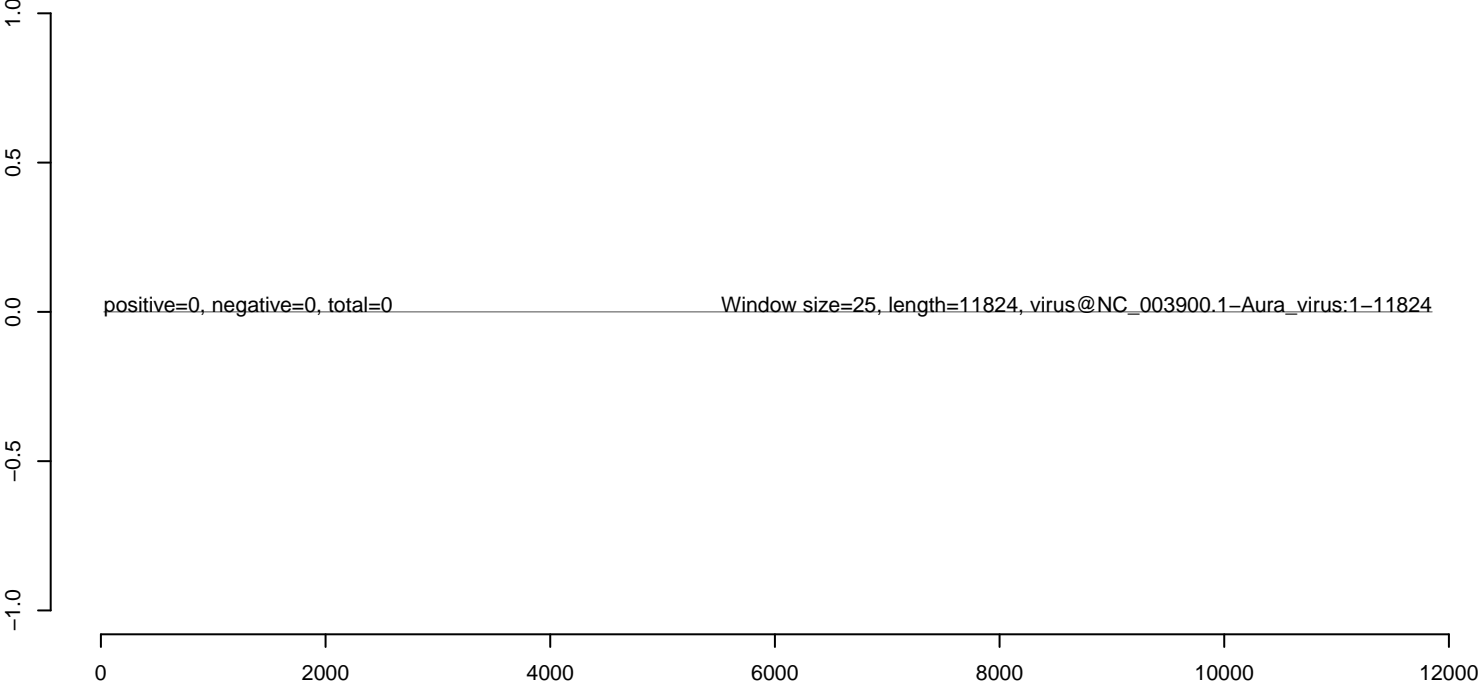
AeAlbo_C636_6dpi_WNV1.rep
