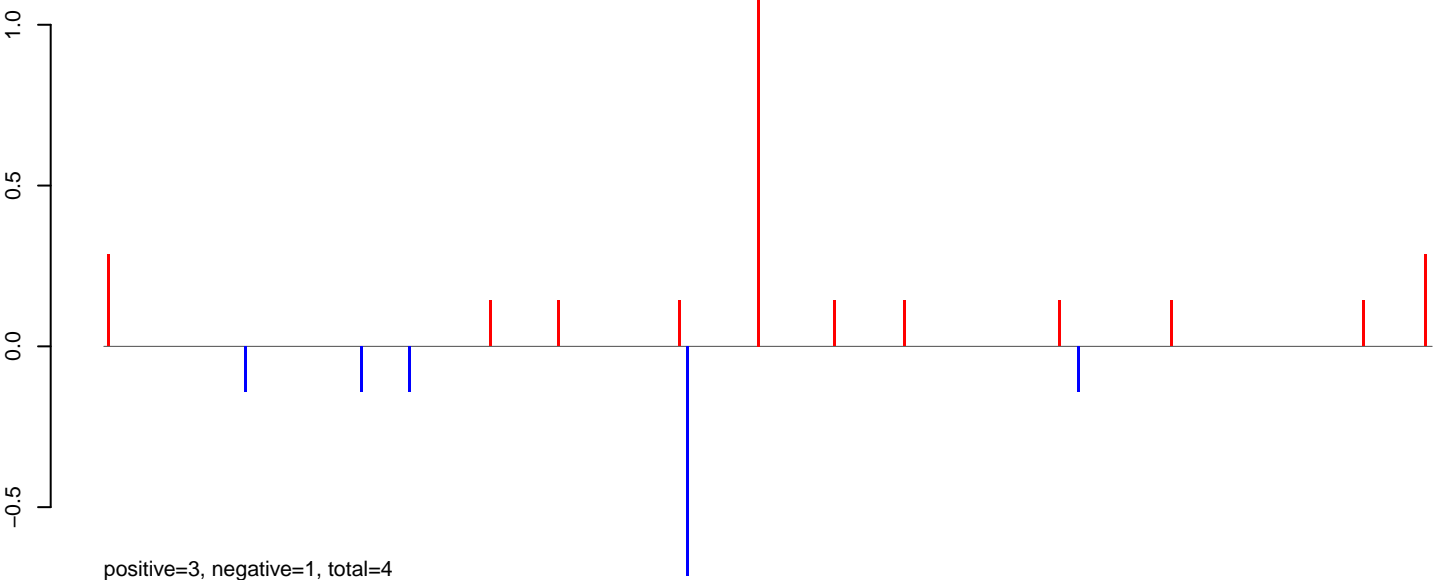
AeAlbo_C636_6dpi_WNV1.24_35.rep
