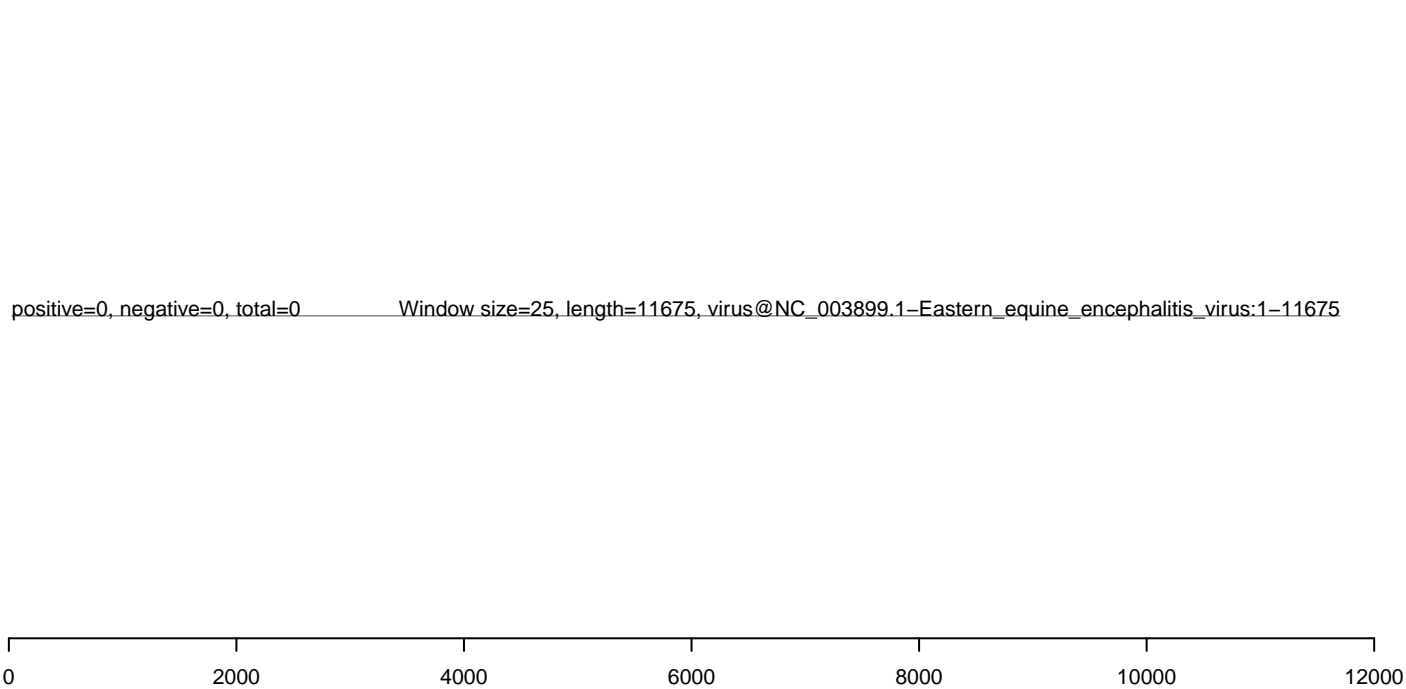
AeAlbo_C636_6dpi_WNV1.rep
