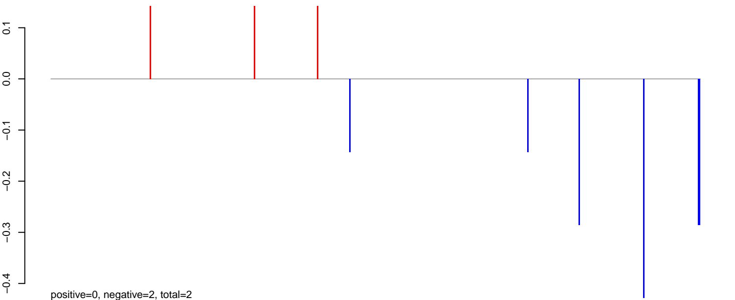
AeAlbo_C636_6dpi_WNV1.24_35.rep
