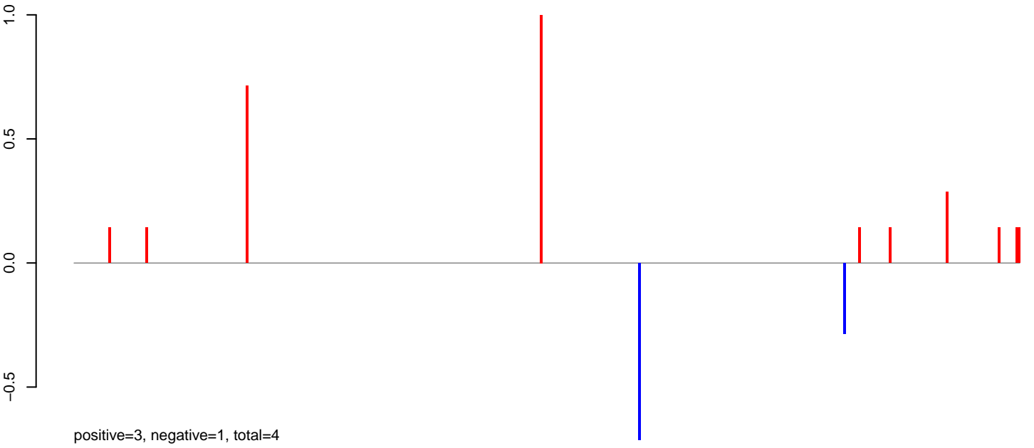
AeAlbo_C636_6dpi_WNV1.24_35.rep
