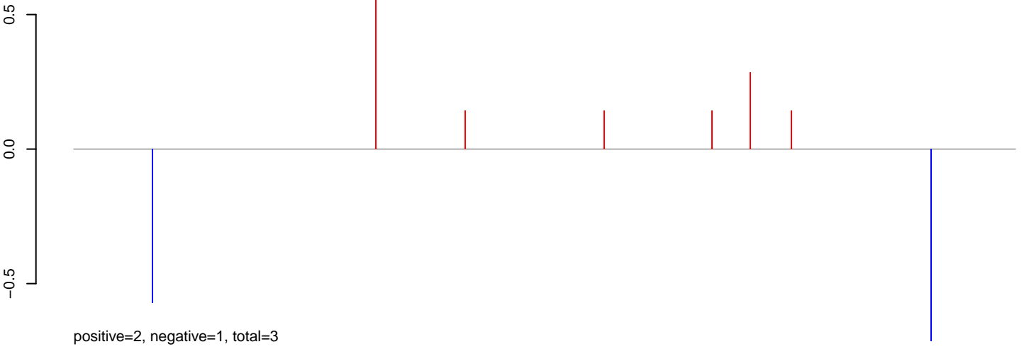
AeAlbo_C636_6dpi_WNV1.24_35.rep
