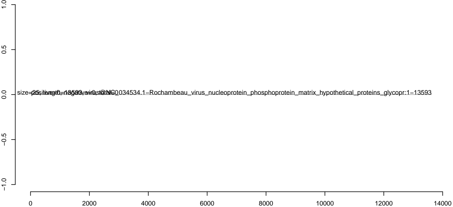
AeAlbo_C636_6dpi_WNV1.rep
