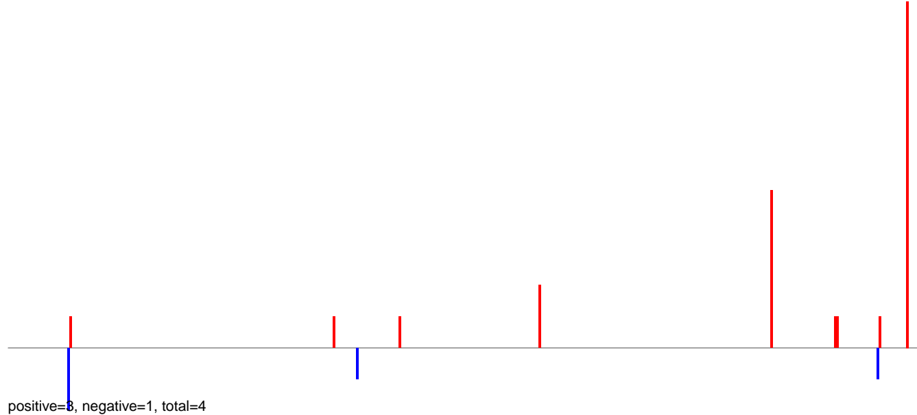
AeAlbo_C636_6dpi_WNV1.24_35.rep
