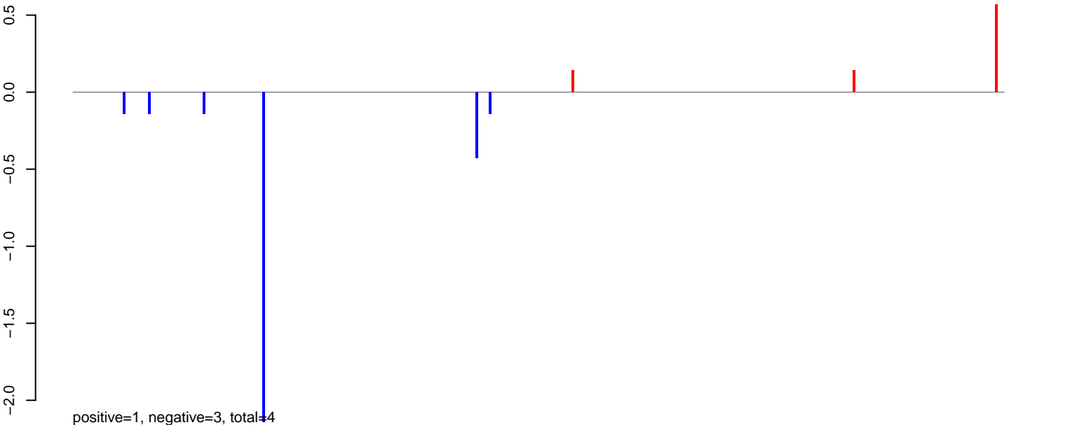
AeAlbo_C636_6dpi_WNV1.24_35.rep
