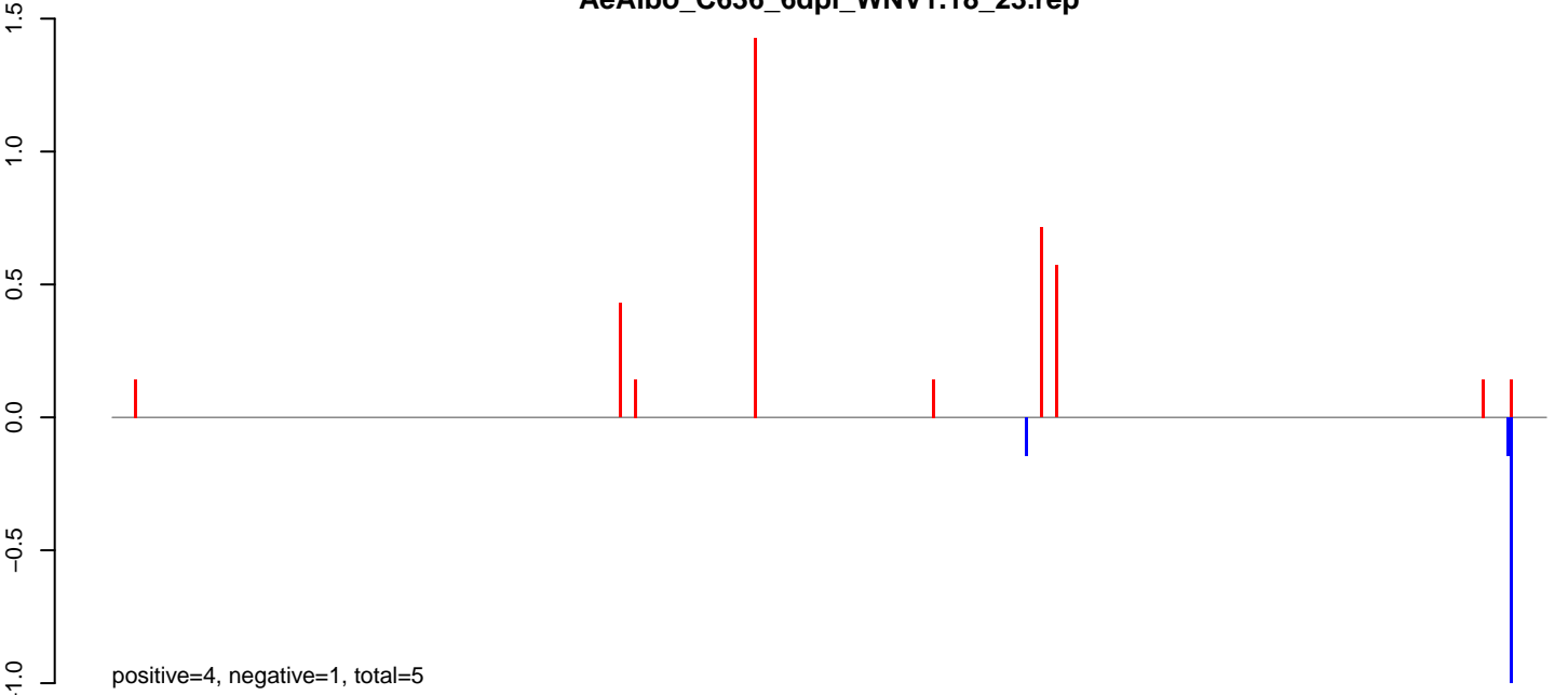
AeAlbo_C636_6dpi_WNV1.24_35.rep
