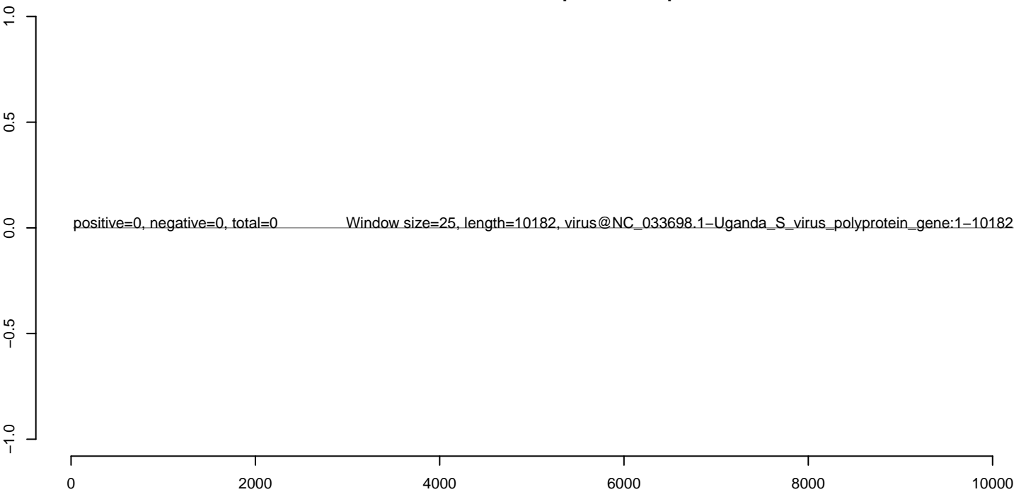
AeAlbo_C636_6dpi_WNV1.rep
