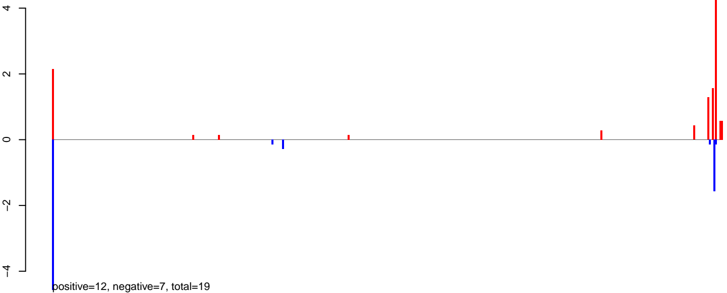
AeAlbo_C636_6dpi_WNV1.24_35.rep
