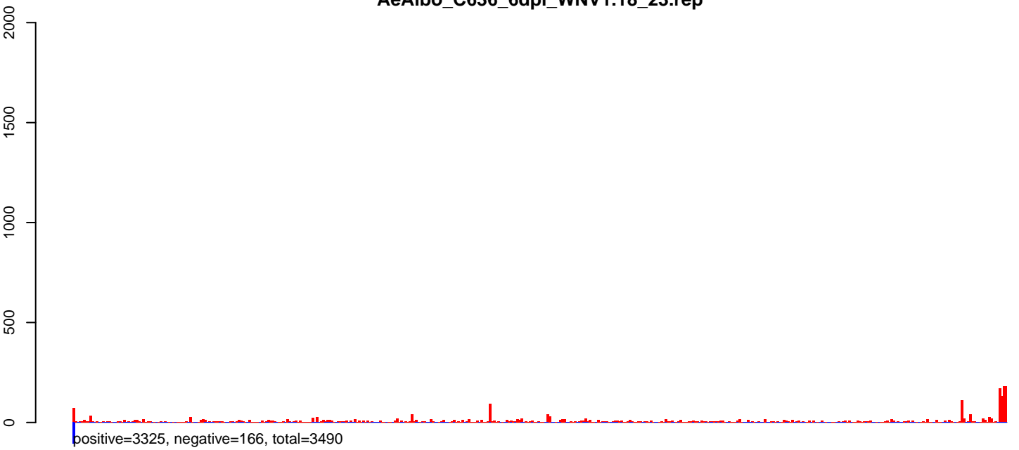
AeAlbo_C636_6dpi_WNV1.24_35.rep
