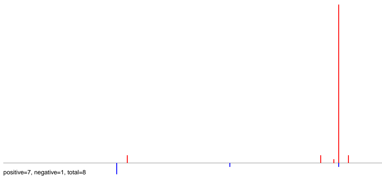
AeAlbo_C636_6dpi_WNV1.24_35.rep
