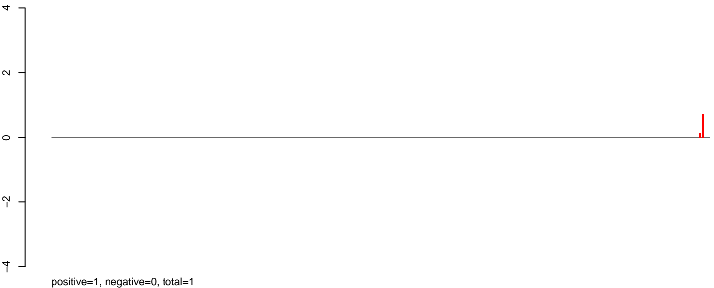
AeAlbo_C636_6dpi_WNV1.rep
