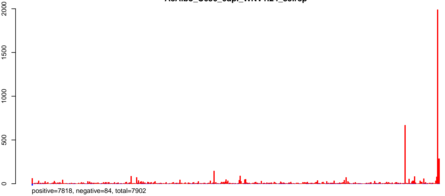
AeAlbo_C636_6dpi_WNV1.rep
