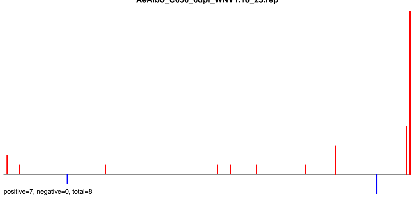
AeAlbo_C636_6dpi_WNV1.24_35.rep
