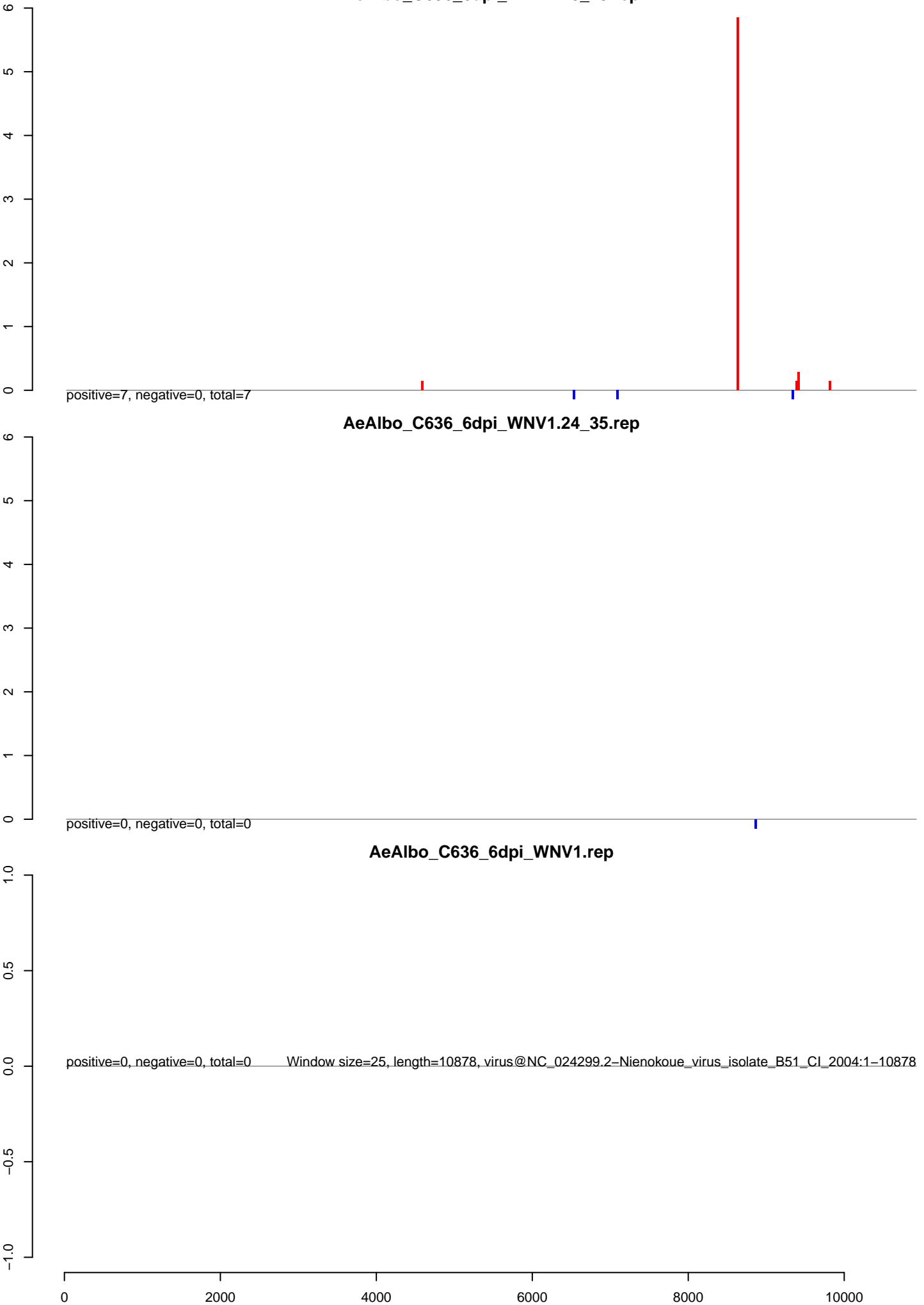
AeAlbo_C636_6dpi_WNV1.18_23.rep
