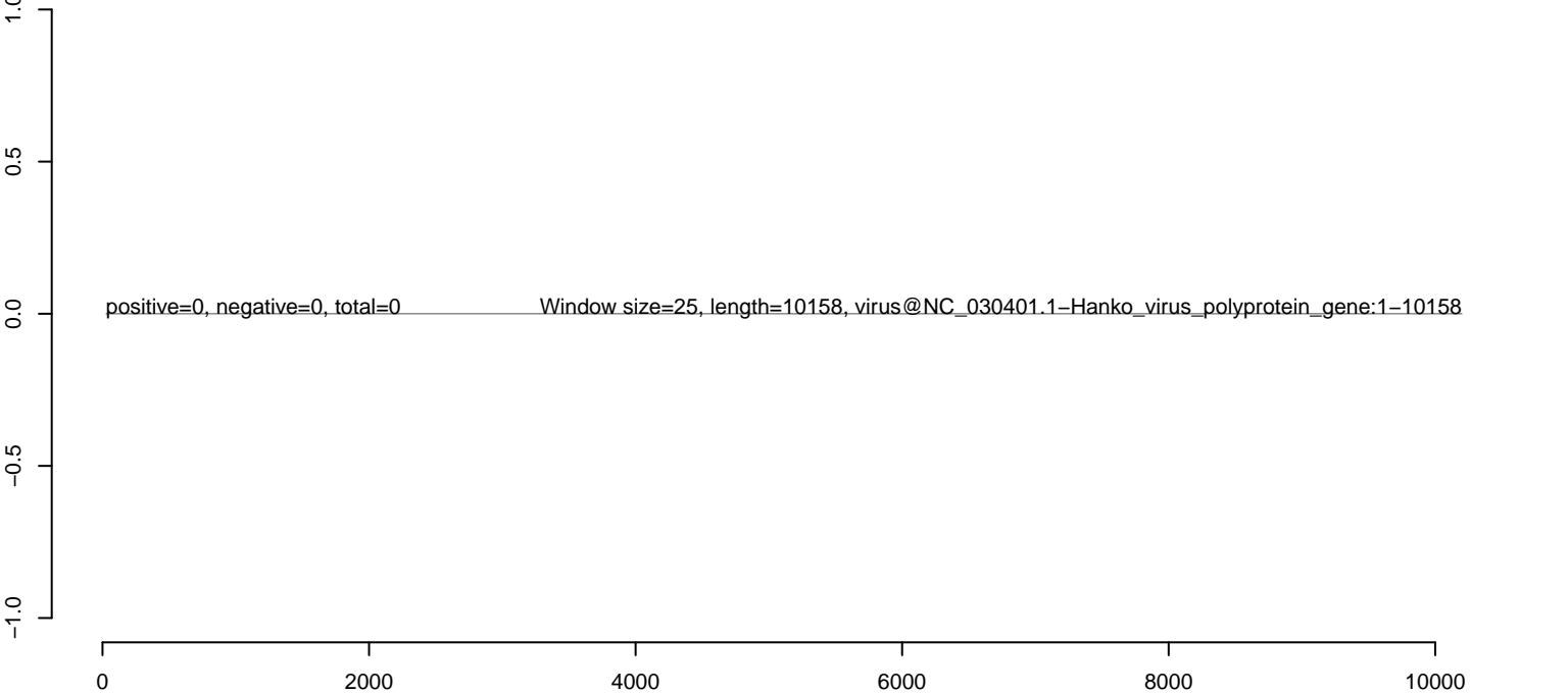
AeAlbo_C636_6dpi_WNV1.rep
