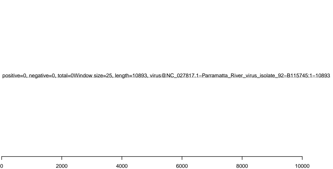
AeAlbo_C636_6dpi_WNV1.rep
