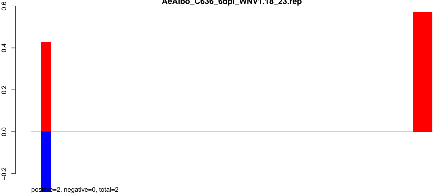
AeAlbo_C636_6dpi_WNV1.24_35.rep
