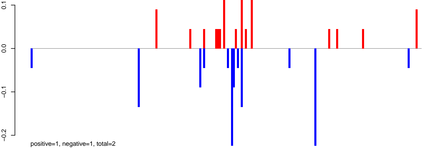
AeAlbo_HeadThor_CHIKV.deltaB2_NOV.24_35.rep
