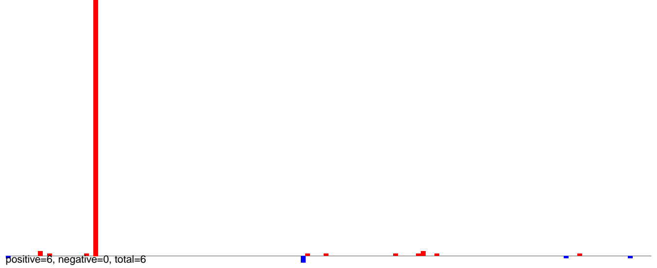
AeAlbo_HeadThor_CHIKV.deltaB2_NOV.24_35.rep
