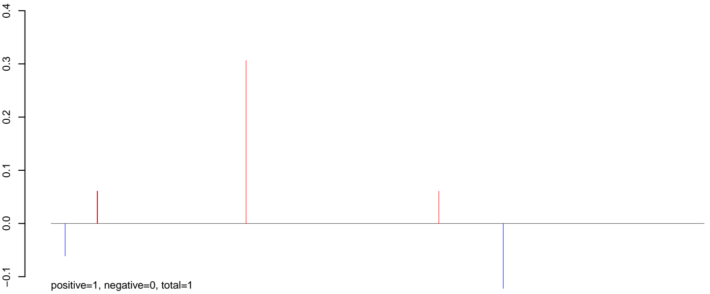
AeAlbo_C636_B2_FHV_r54q.24_35.rep
