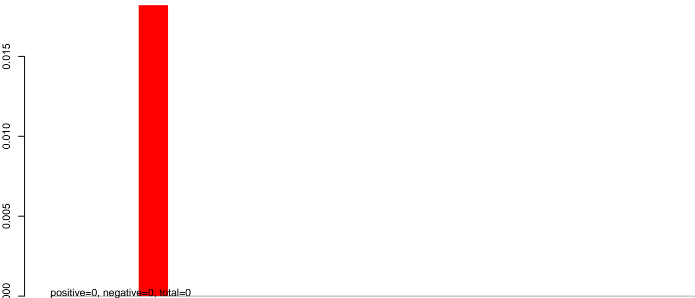
AeAlbo_C636_CHIKV_3dpi.24_35.rep
