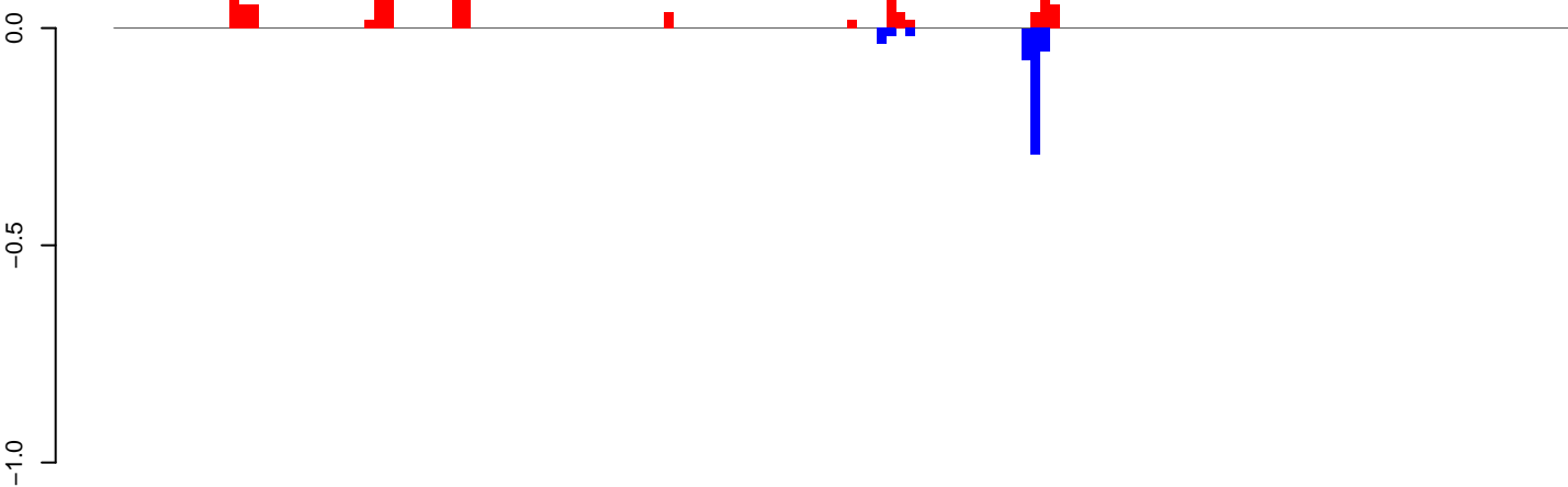
AeAlbo_C636_CHIKV_3dpi.24_35.rep
