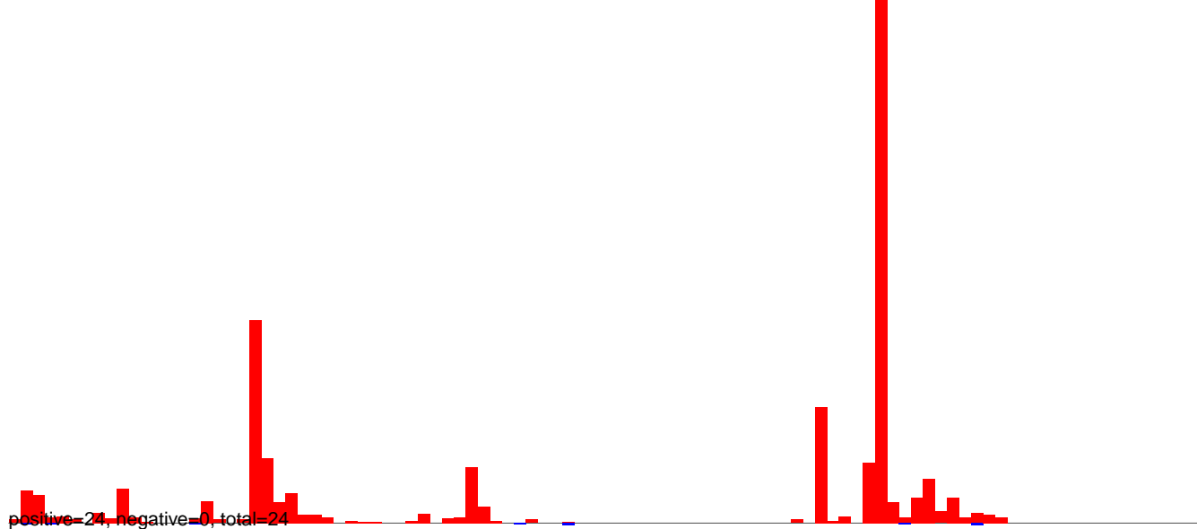
AeAlbo_C636_CHIKV_3dpi.24_35.rep
