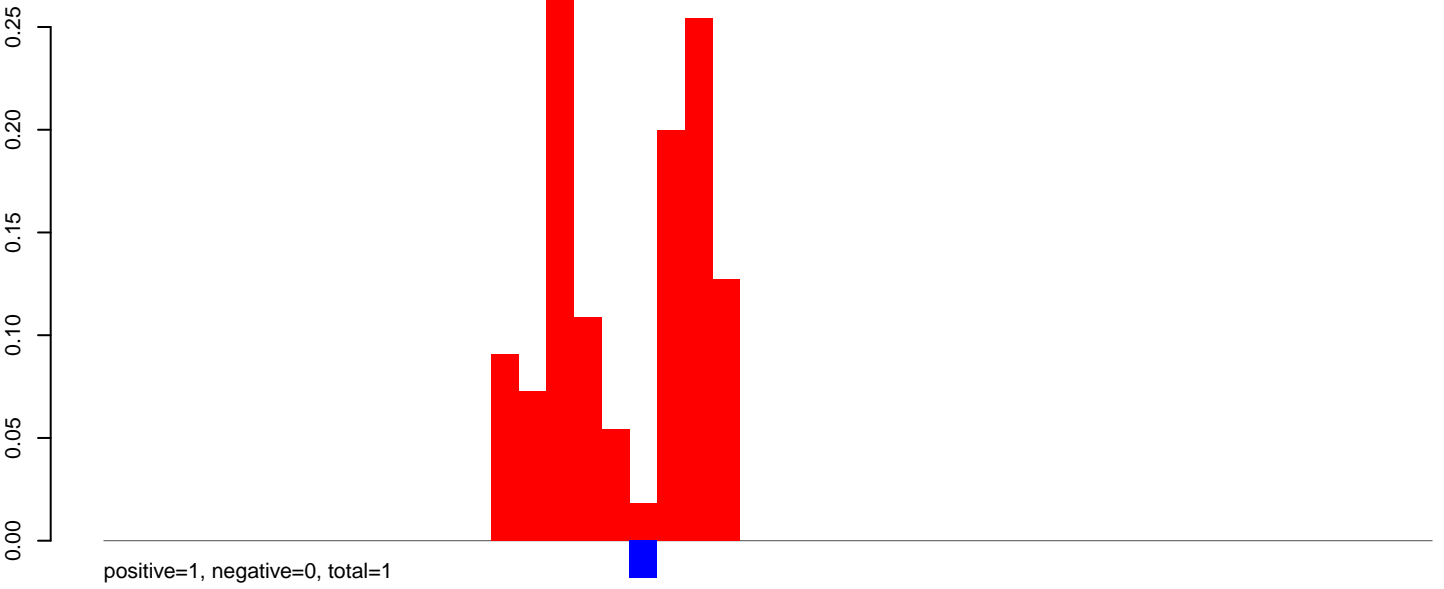
AeAlbo_C636_CHIKV_3dpi.24_35.rep
