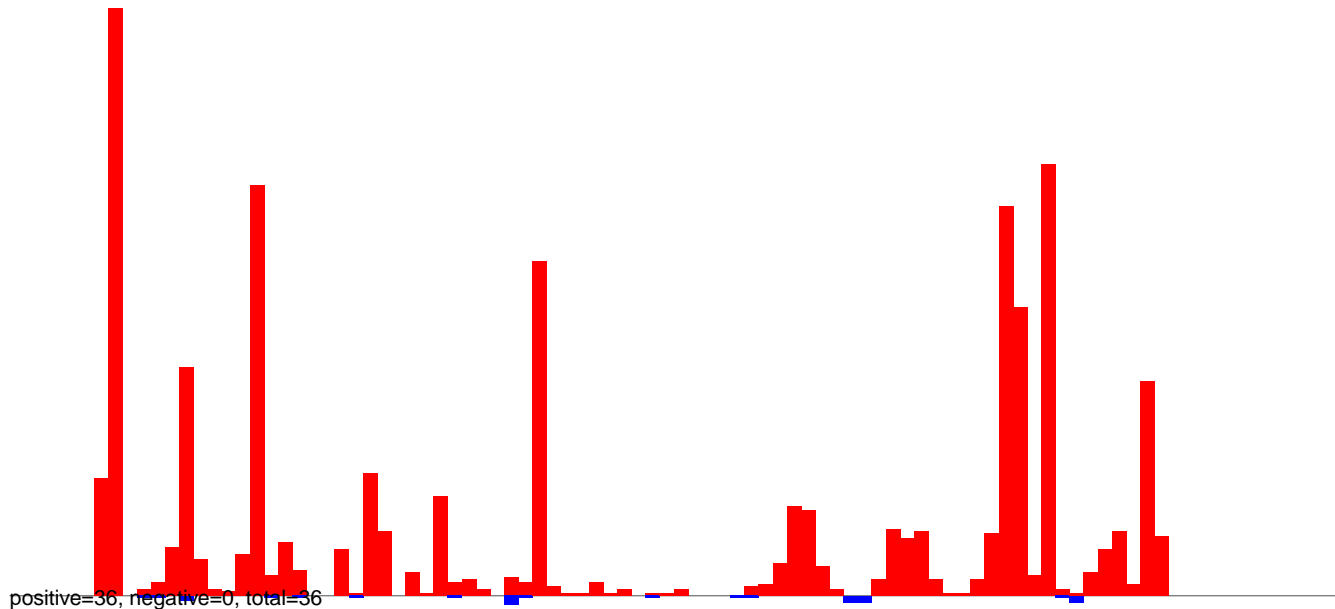
AeAlbo_C636_CHIKV_3dpi.24_35.rep
