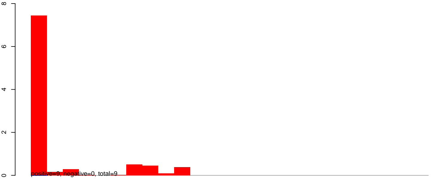
AeAlbo_C636_CHIKV_3dpi.24_35.rep
