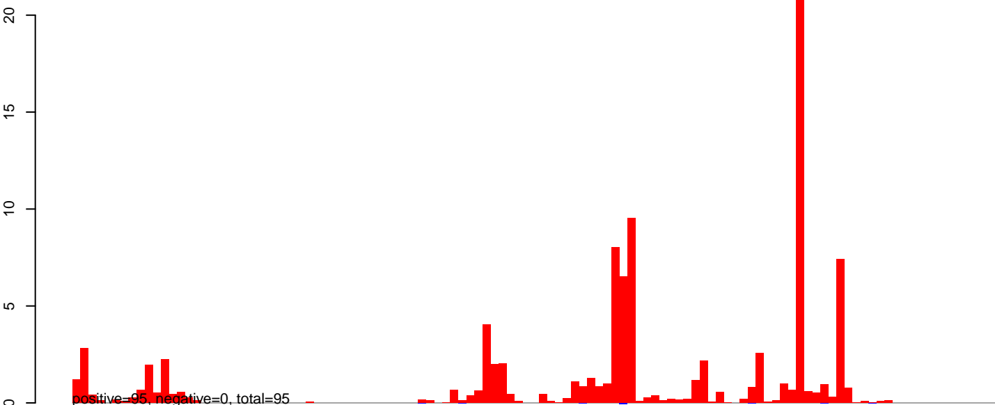
AeAlbo_C636_CHIKV_3dpi.24_35.rep
