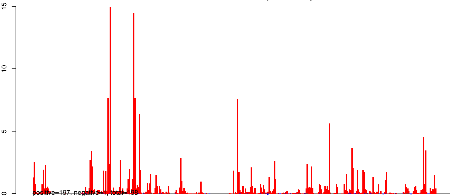
AeAlbo_C636_CHIKV_3dpi.24_35.rep
