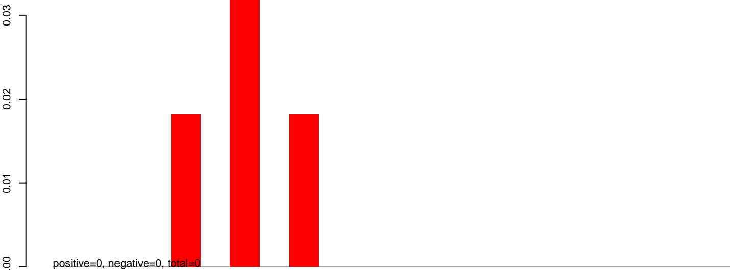
AeAlbo_C636_CHIKV_3dpi.24_35.rep
