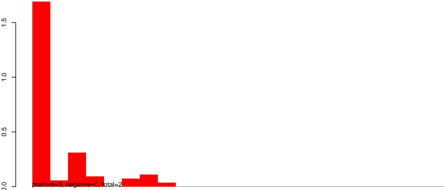
AeAlbo_C636_CHIKV_3dpi.24_35.rep
