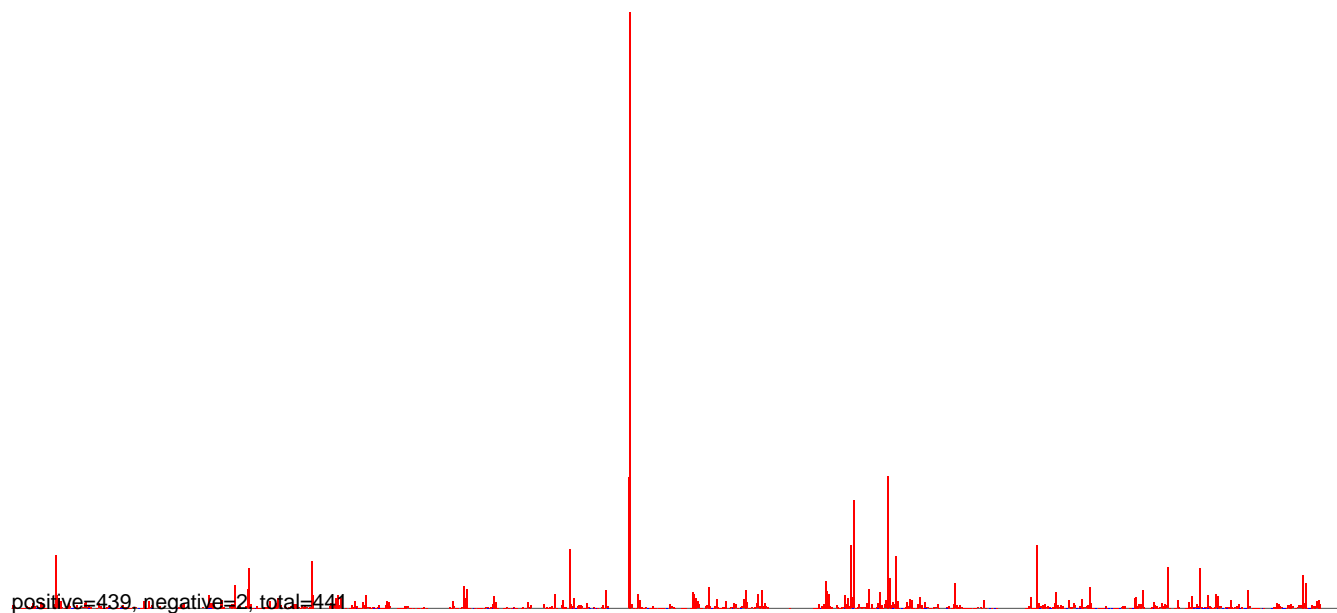
AeAlbo_C636_CHIKV_3dpi.24_35.rep
