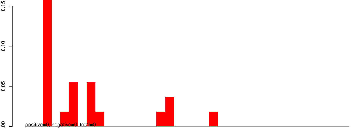
AeAlbo_C636_CHIKV_3dpi.24_35.rep
