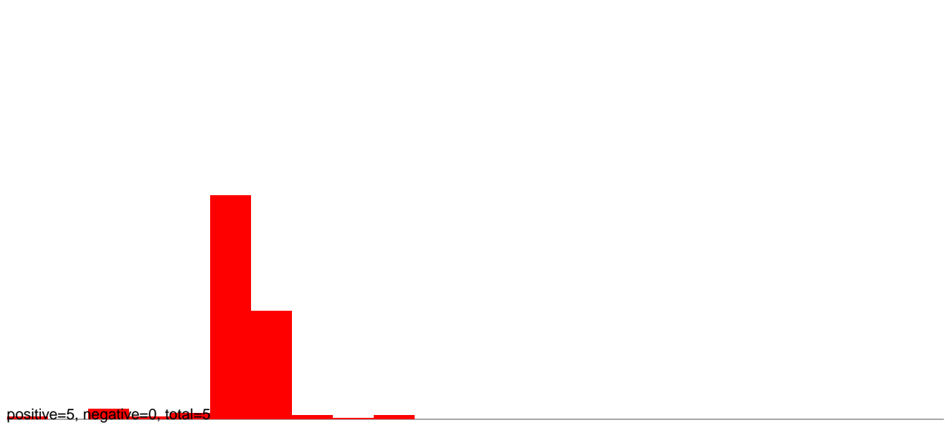
AeAlbo_C636_CHIKV_3dpi.24_35.rep
