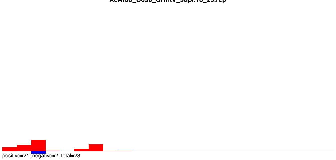
AeAlbo_C636_CHIKV_3dpi.24_35.rep
