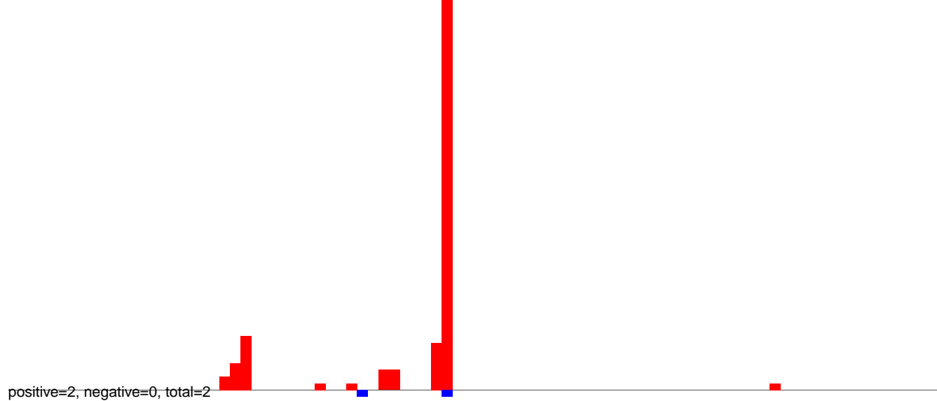
AeAlbo_C636_CHIKV_3dpi.24_35.rep
