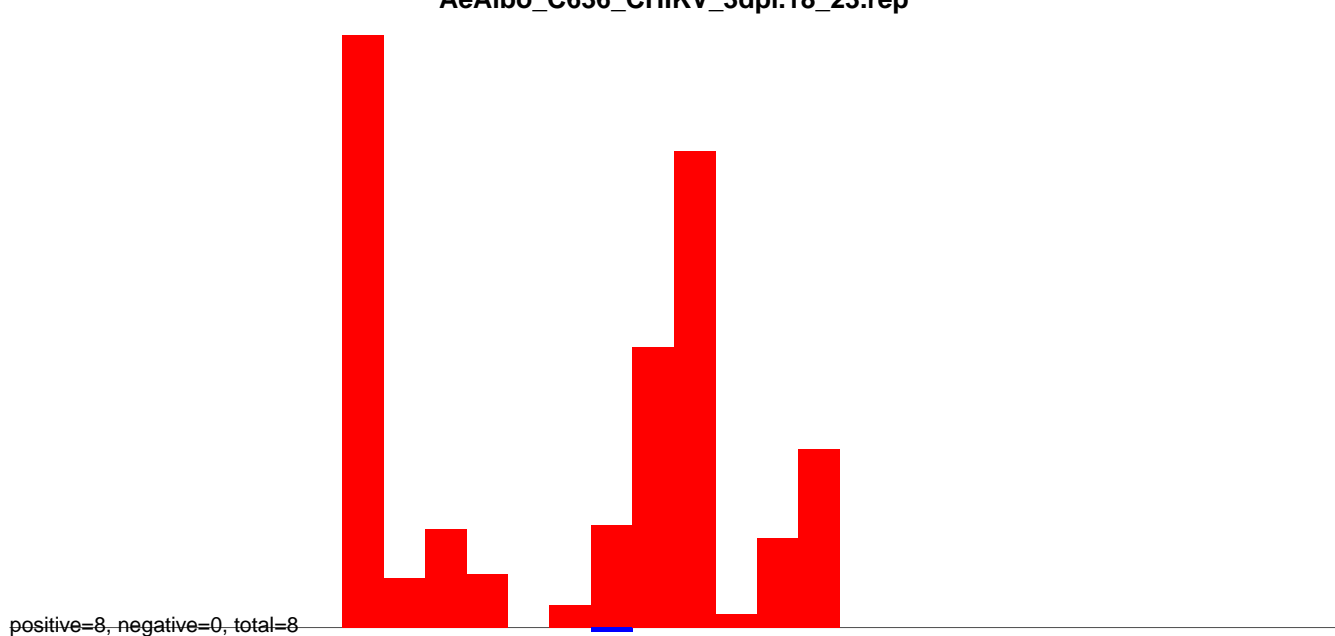
AeAlbo_C636_CHIKV_3dpi.24_35.rep
