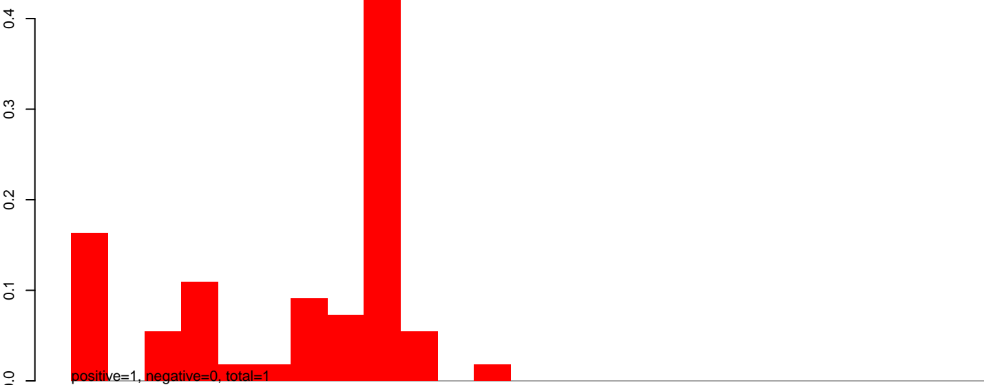
AeAlbo_C636_CHIKV_3dpi.24_35.rep
