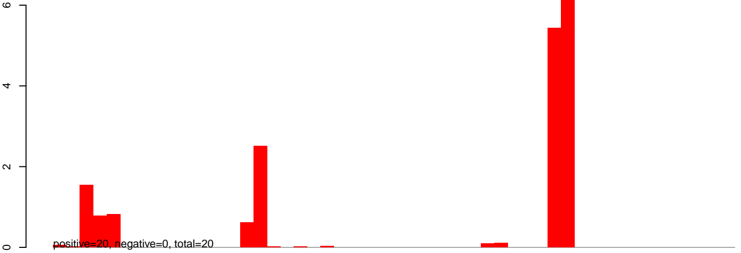
AeAlbo_C636_CHIKV_3dpi.24_35.rep
