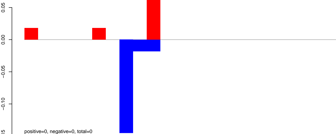
AeAlbo_C636_CHIKV_3dpi.24_35.rep
