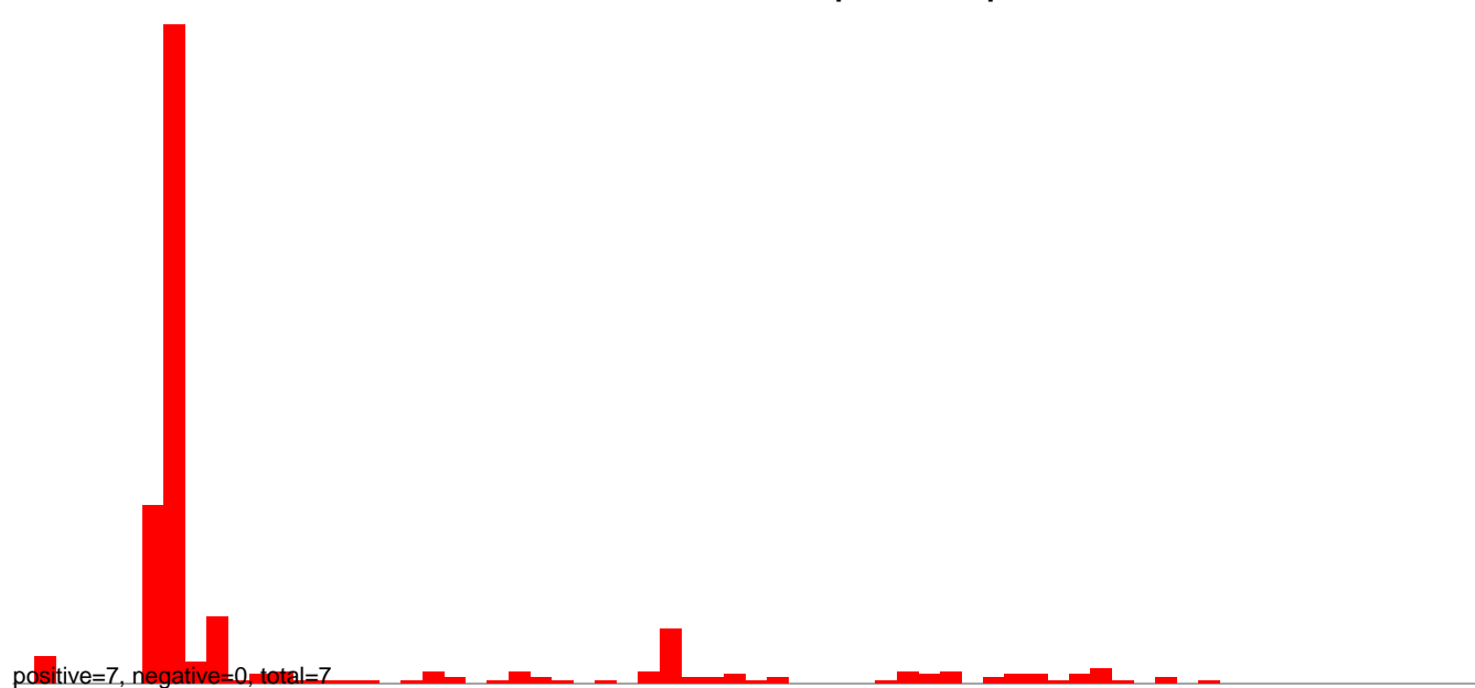
AeAlbo_C636_CHIKV_3dpi.24_35.rep
