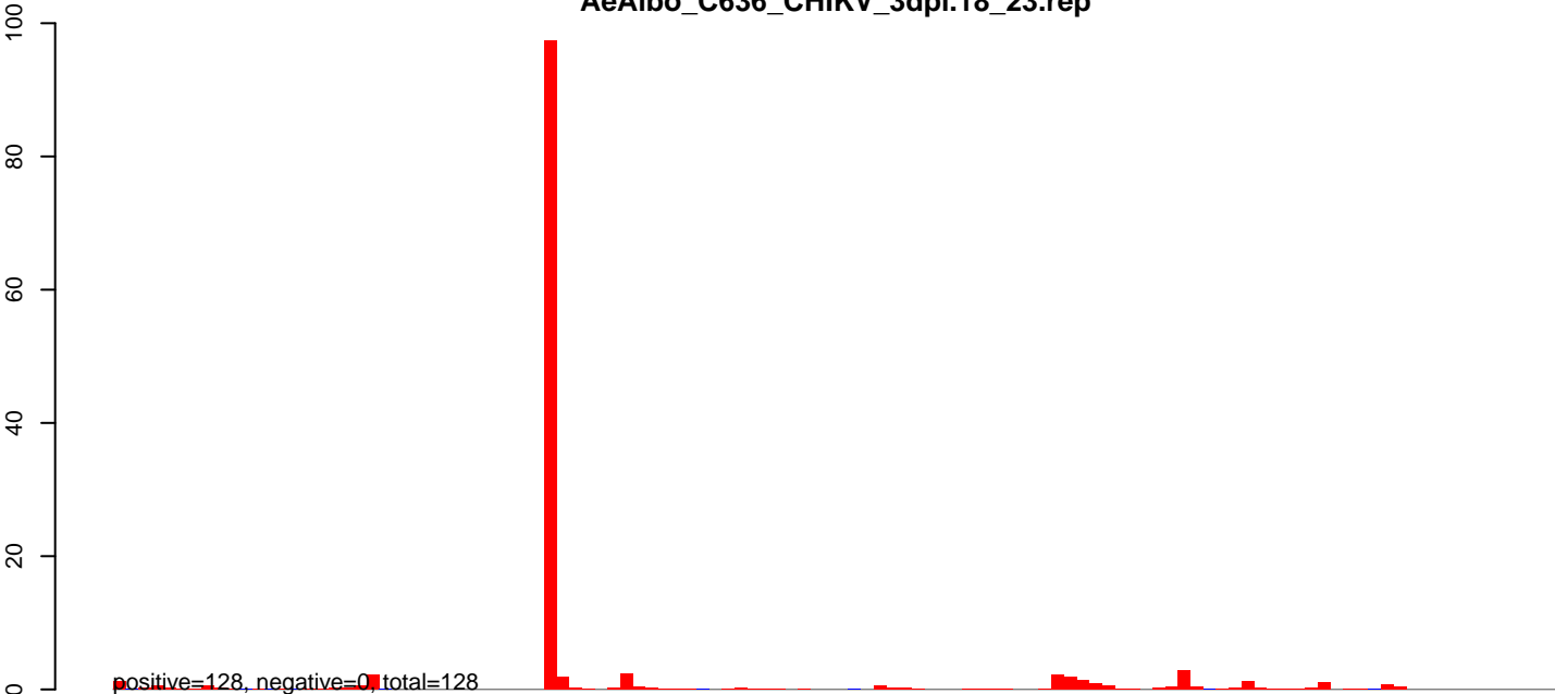
AeAlbo_C636_CHIKV_3dpi.24_35.rep
