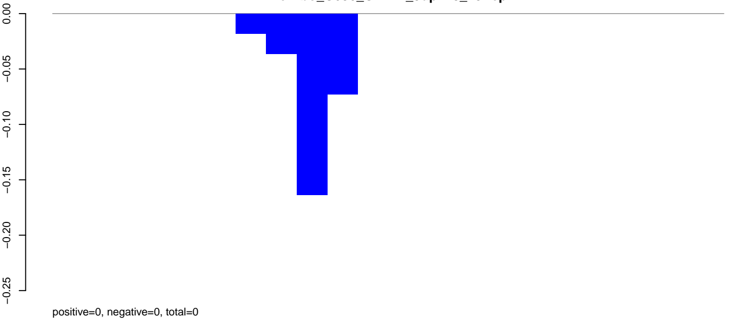
AeAlbo_C636_CHIKV_3dpi.24_35.rep
