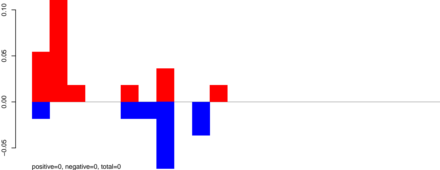
AeAlbo_C636_CHIKV_3dpi.24_35.rep
