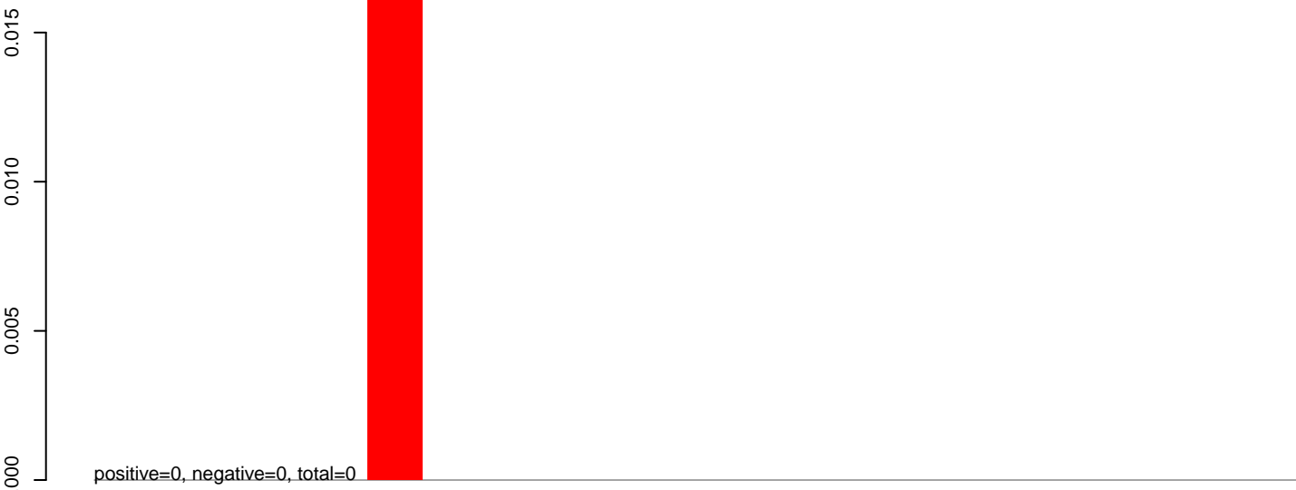
AeAlbo_C636_CHIKV_3dpi.24_35.rep
