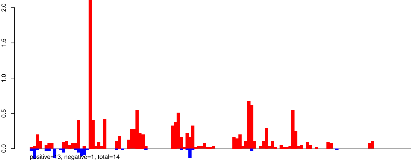
AeAlbo_C636_CHIKV_3dpi.24_35.rep
