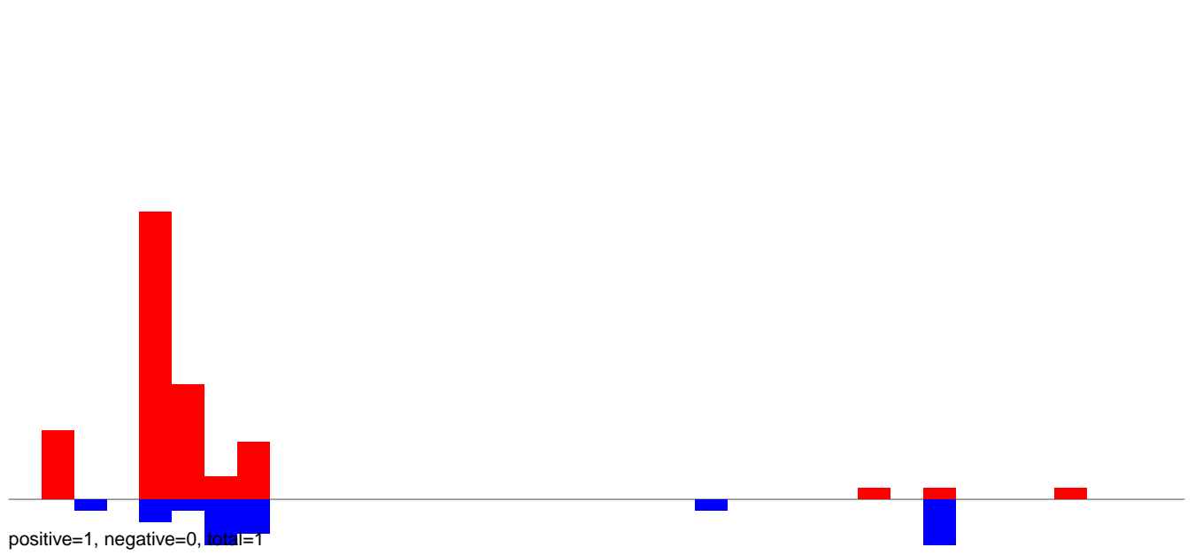
AeAlbo_C636_CHIKV_AZT_3dpi.24_35.rep
