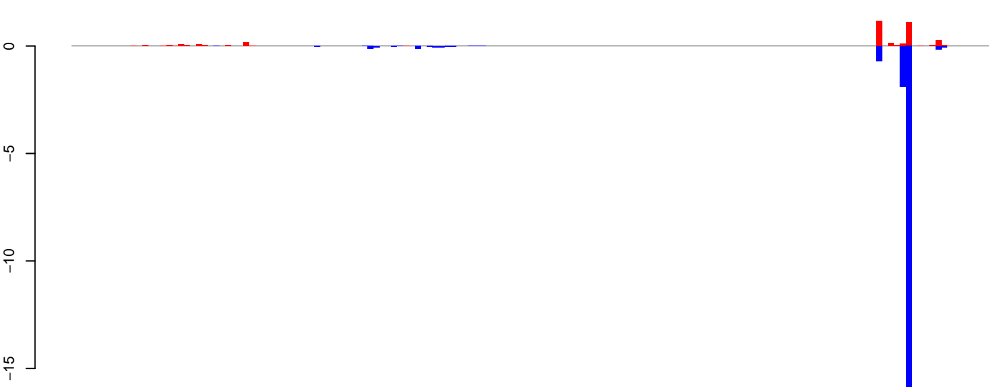
AeAlbo_C636_CHIKV_AZT_3dpi.24_35.rep
