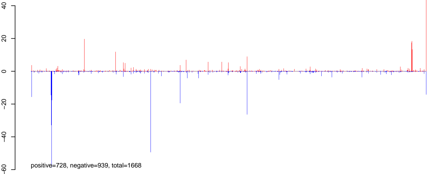
AeAlbo_CHIKV_AZT_3dpi.24_35.rep
