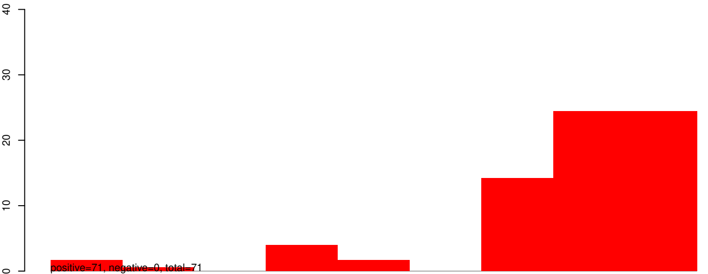
AnGam_Fem_Fat_body_rep1_KM.24_35.rep
