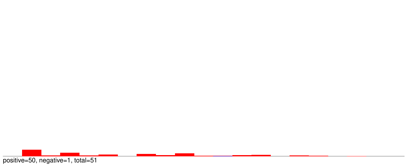
AnGam_Fem_Fat_body_rep1_KM.rep
