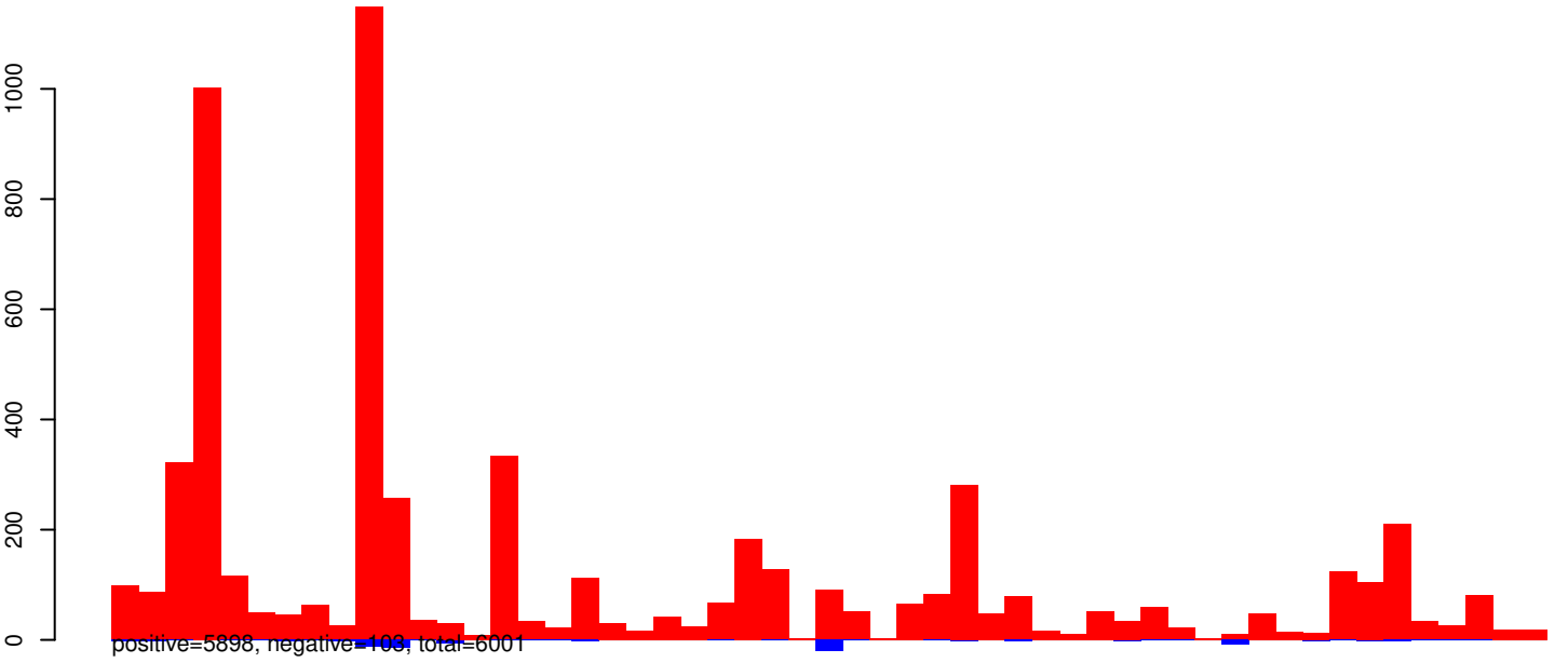
AnGam_Fem_Fat_body_rep1_KM.24_35.rep
