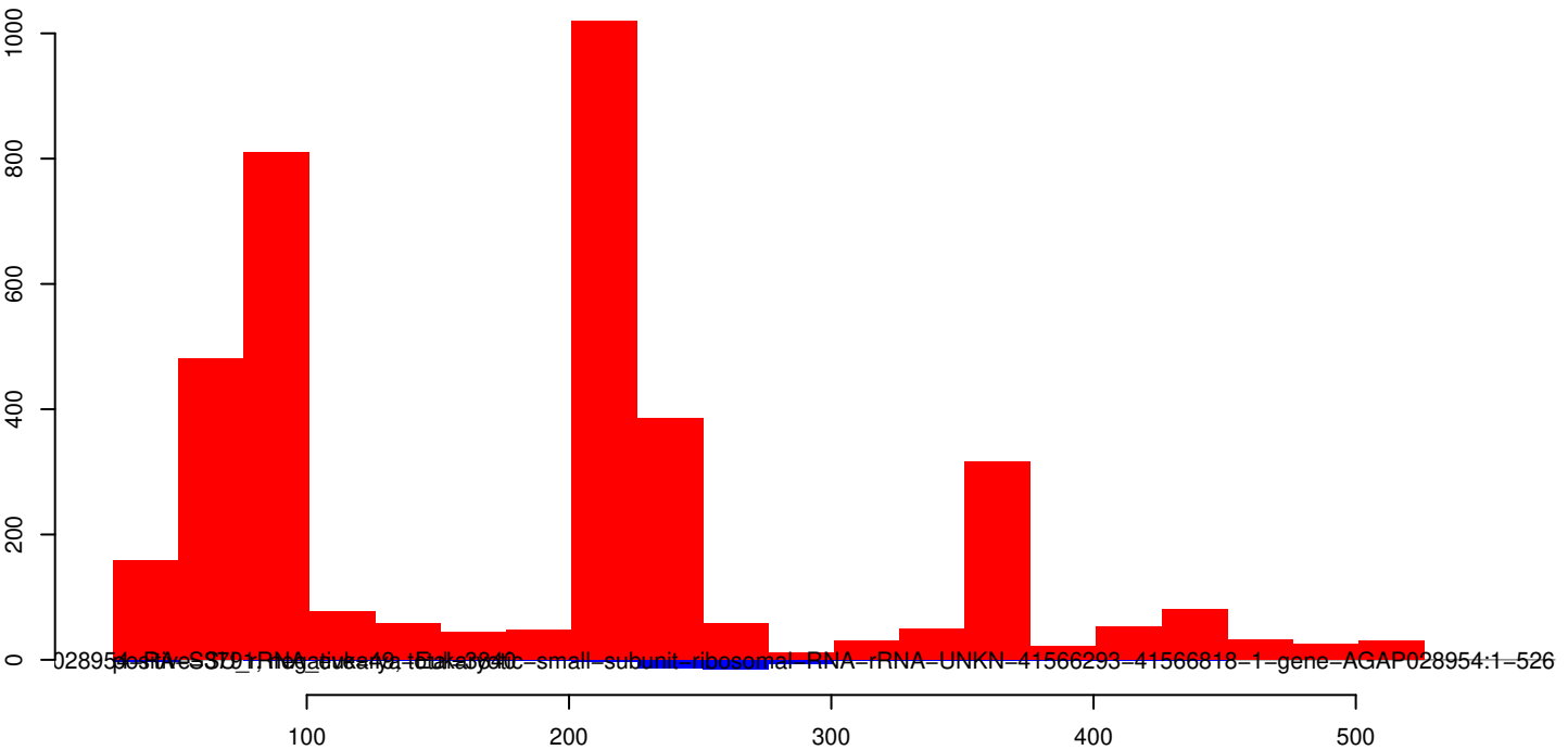
AnGam_Fem_Fat_body_rep1_KM.rep
