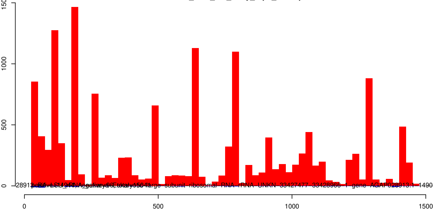
AnGam_Fem_Fat_body_rep1_KM.rep
