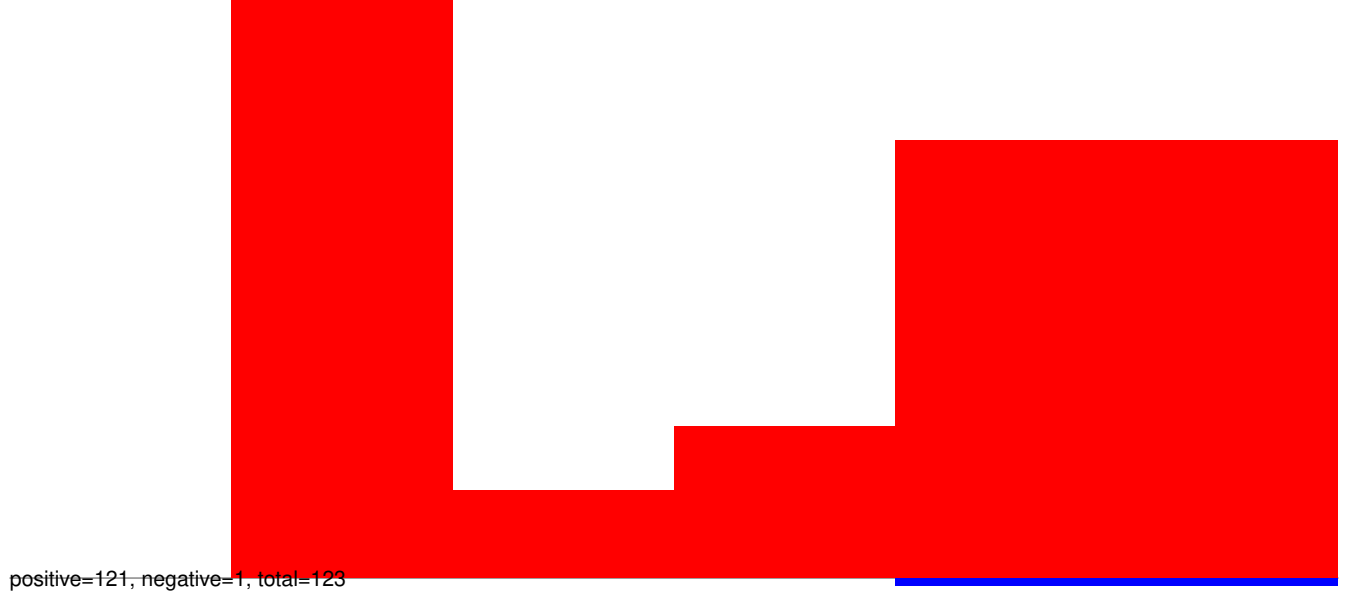
AnGam_Fem_Fat_body_rep1_KM.24_35.rep
