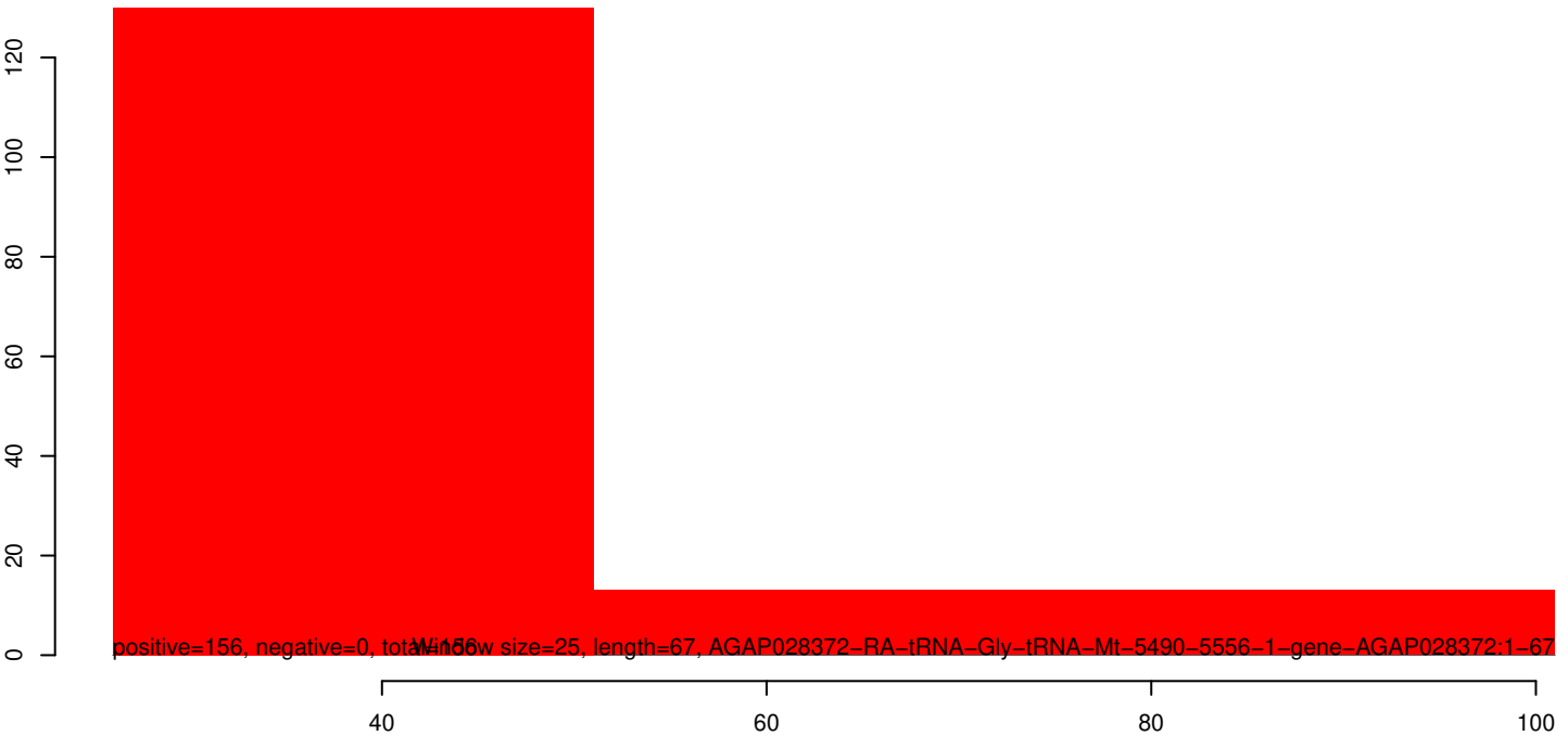
AnGam_Fem_Fat_body_rep1_KM.rep
