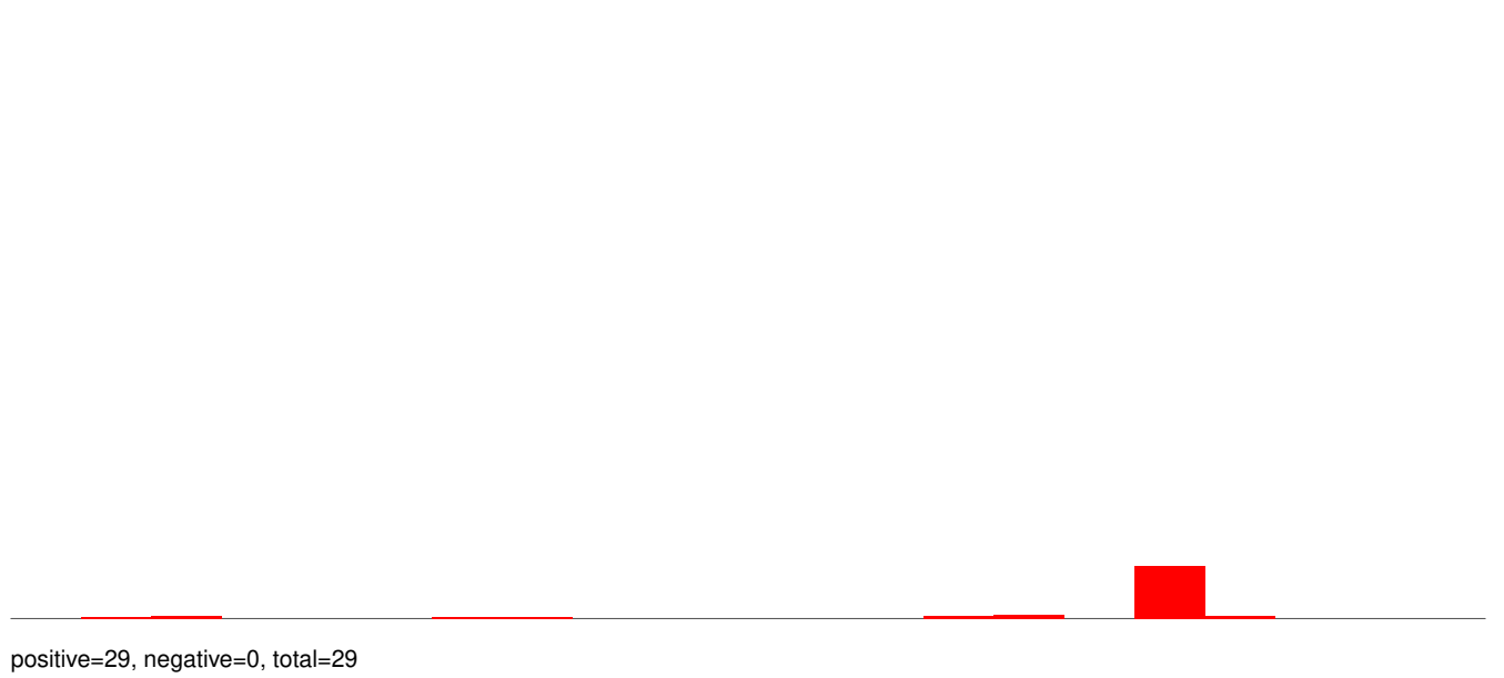
AnGam_Fem_Fat_body_rep1_KM.rep
