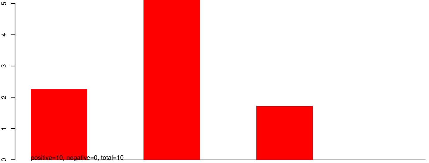
AnGam_Fem_Fat_body_rep1_KM.24_35.rep
