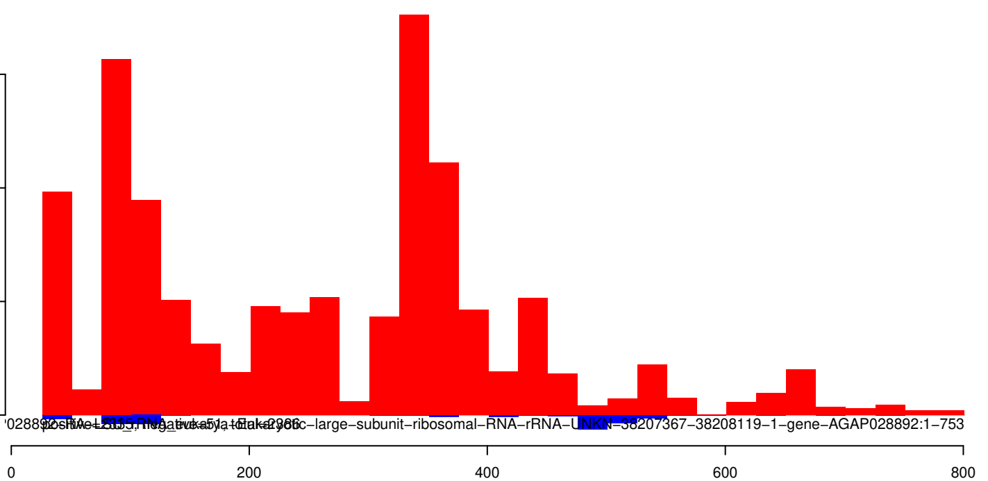
AnGam_Fem_Fat_body_rep1_KM.rep
