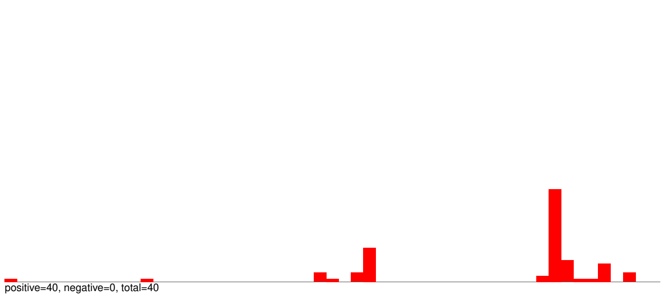
AnGam_Fem_Fat_body_rep1_KM.rep
