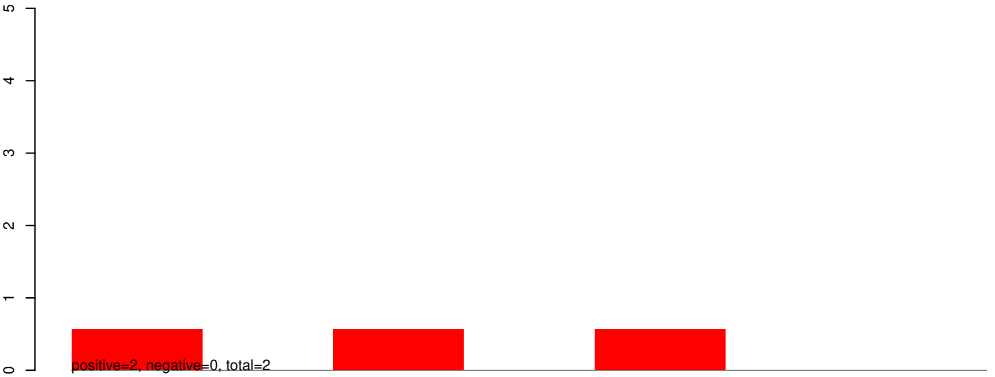
AnGam_Fem_Fat_body_rep1_KM.rep
