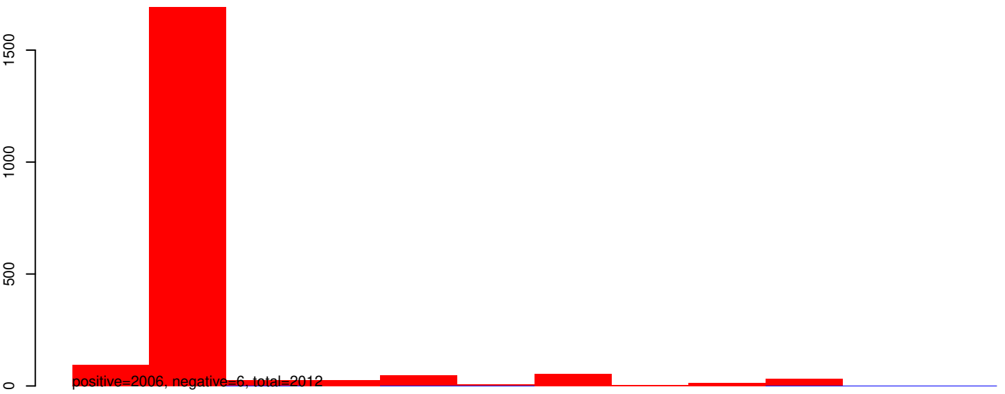
AnGam_Fem_Fat_body_rep1_KM.24_35.rep
