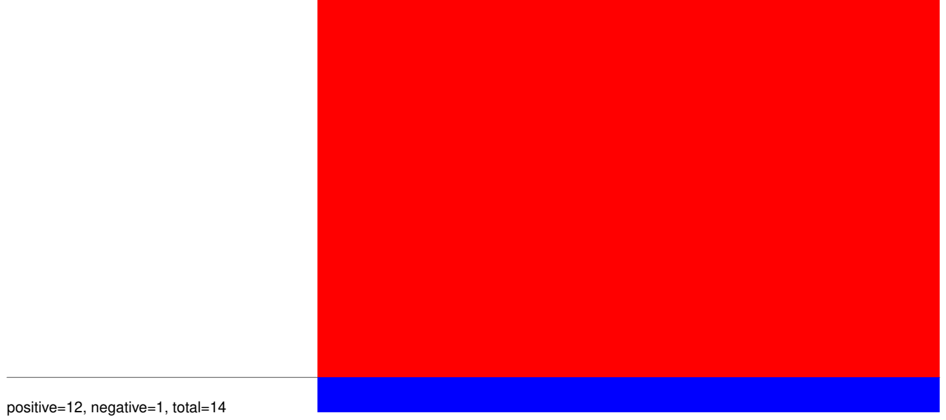
AnGam_Fem_Fat_body_rep1_KM.24_35.rep
