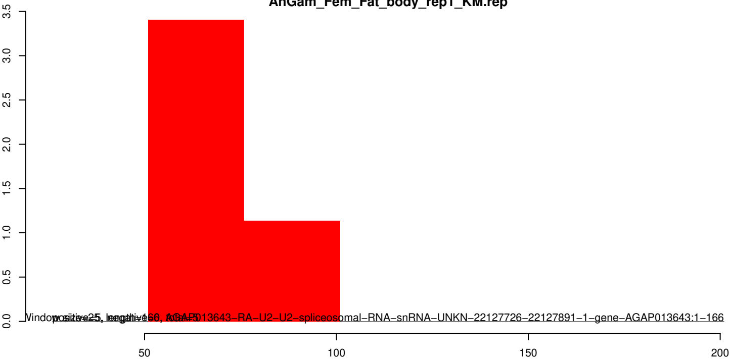
AnGam_Fem_Fat_body_rep1_KM.rep
