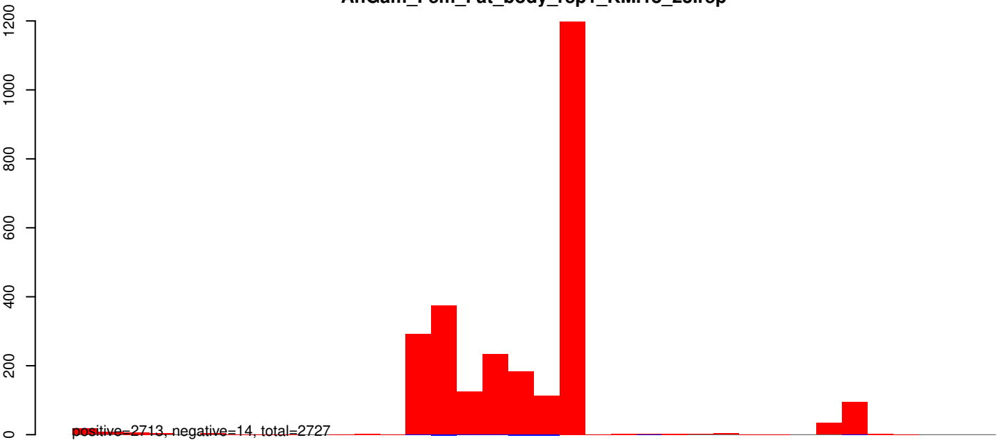
AnGam_Fem_Fat_body_rep1_KM.24_35.rep
