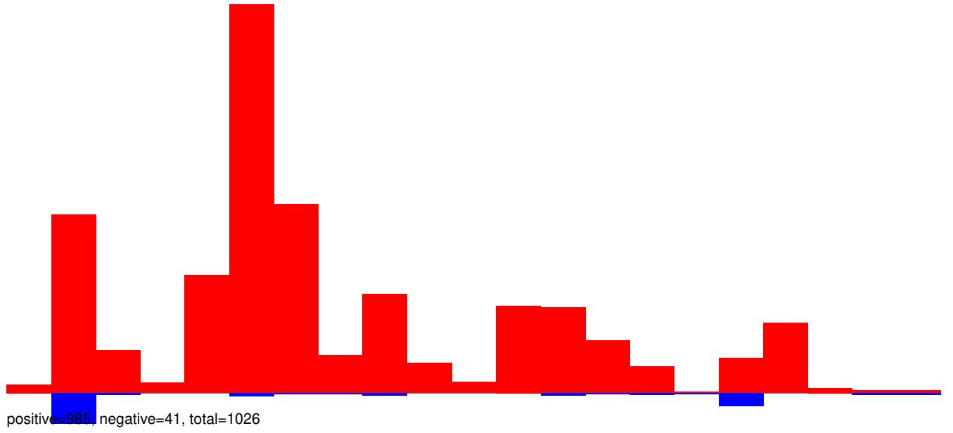
AnGam_Fem_Fat_body_rep1_KM.24_35.rep
