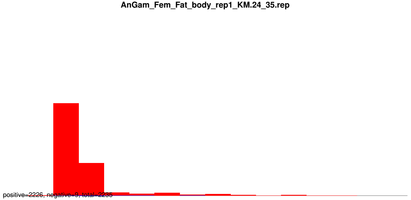
AnGam_Fem_Fat_body_rep1_KM.rep
