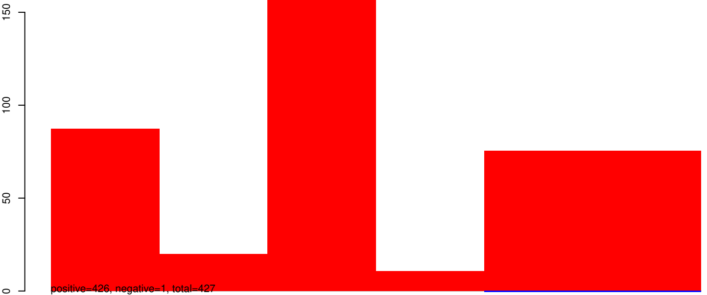
AnGam_Fem_Fat_body_rep1_KM.24_35.rep
