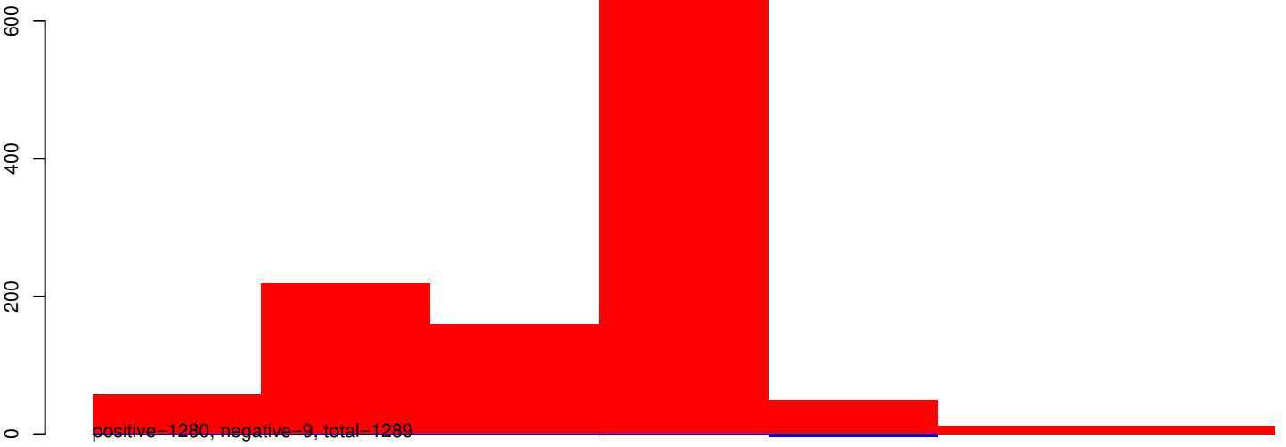
AnGam_Fem_Fat_body_rep1_KM.24_35.rep
