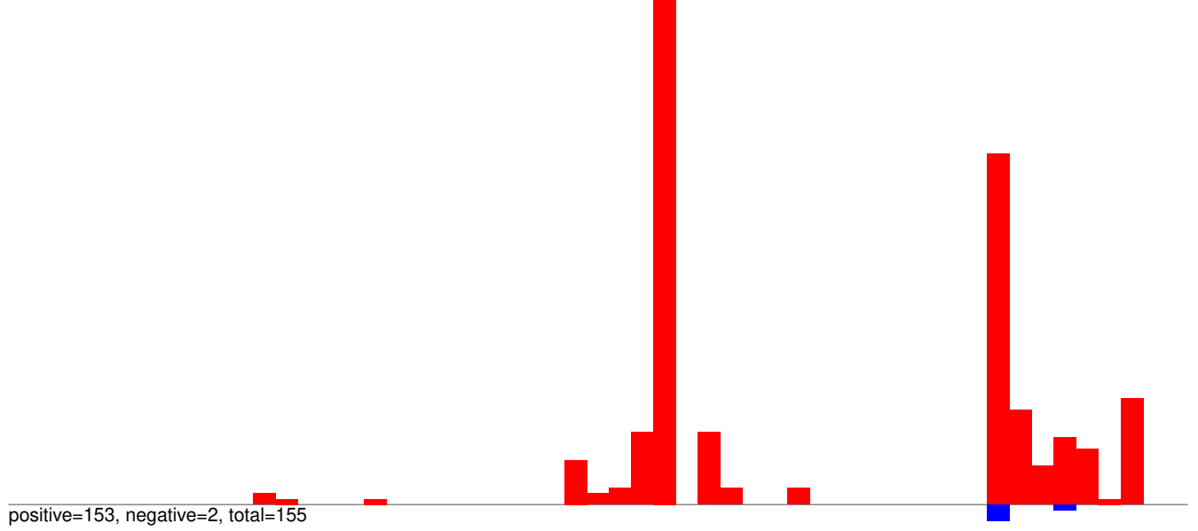
AnGam_Fem_Fat_body_rep1_KM.24_35.rep
