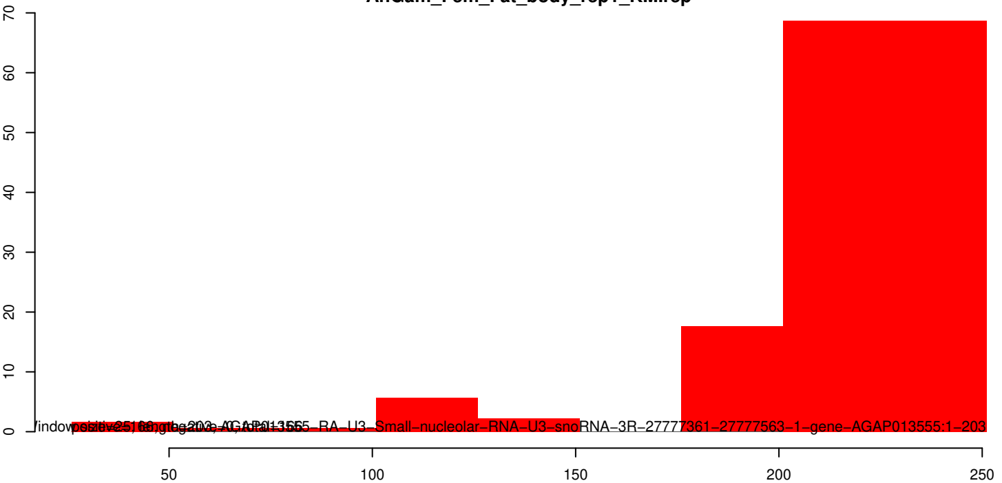
AnGam_Fem_Fat_body_rep1_KM.rep
