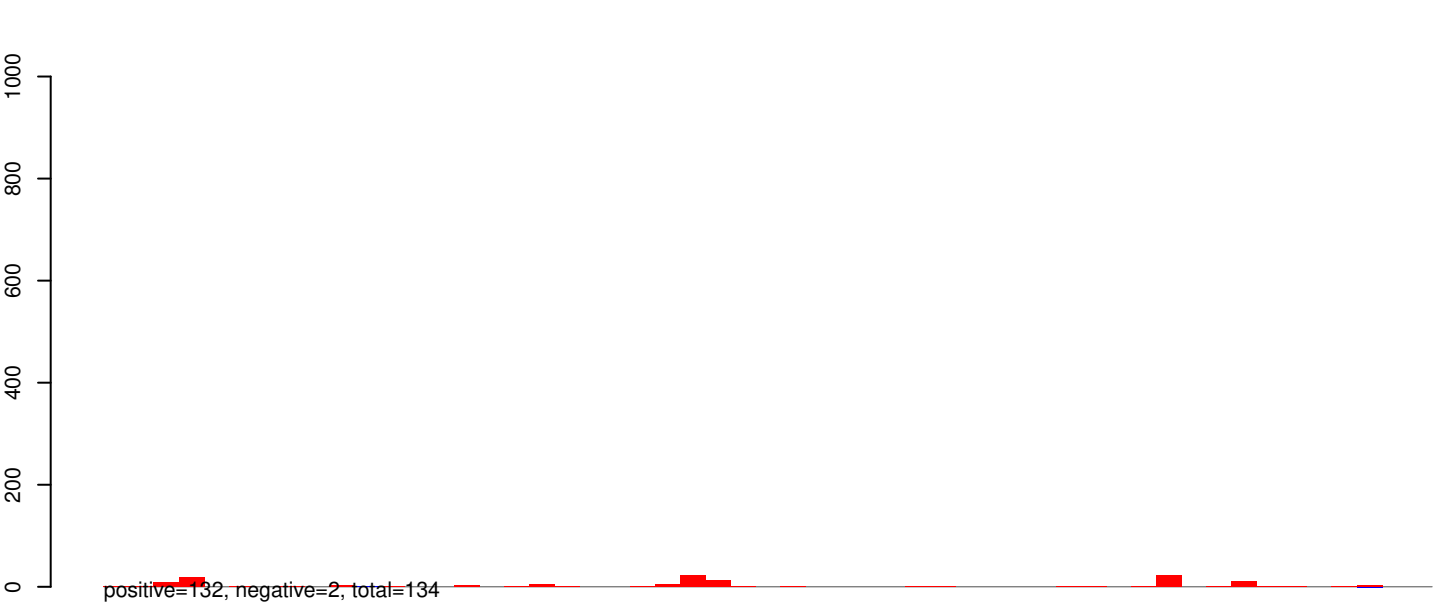
AnGam_Fem_Fat_body_rep1_KM.rep
