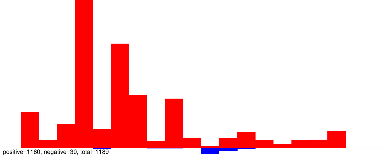
AnGam_Fem_Fat_body_rep1_KM.24_35.rep
