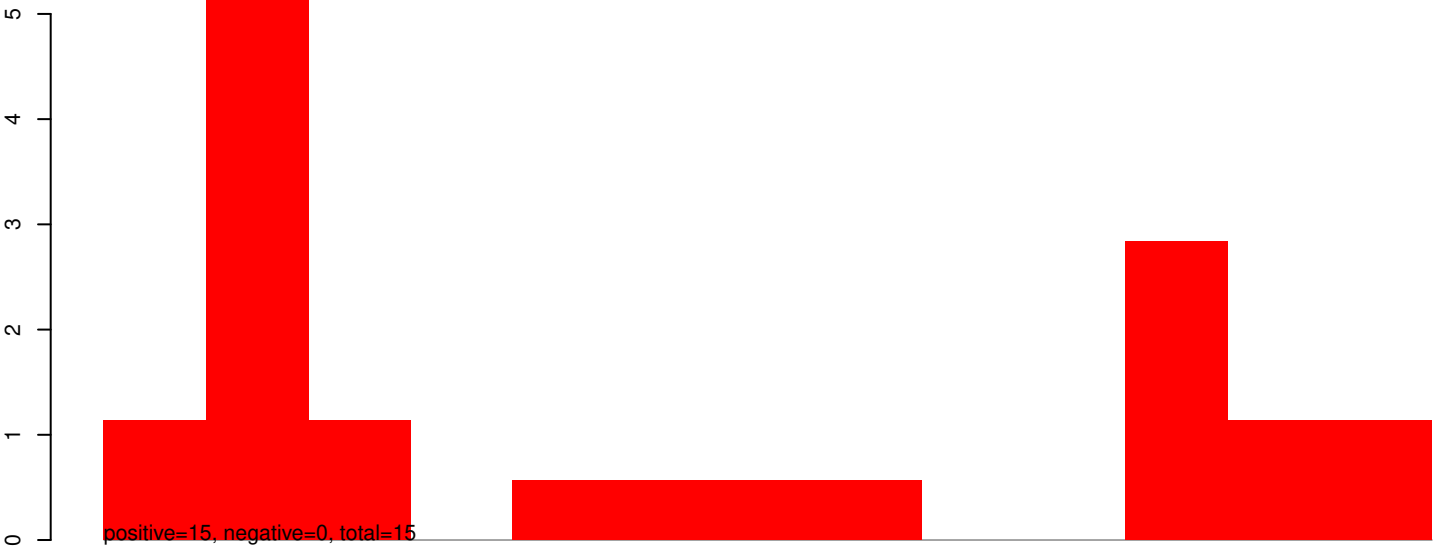
AnGam_Fem_Fat_body_rep1_KM.24_35.rep
