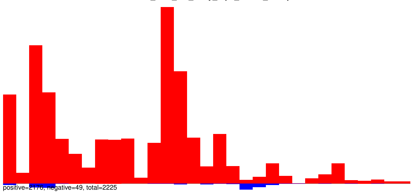
AnGam_Fem_Fat_body_rep1_KM.24_35.rep
