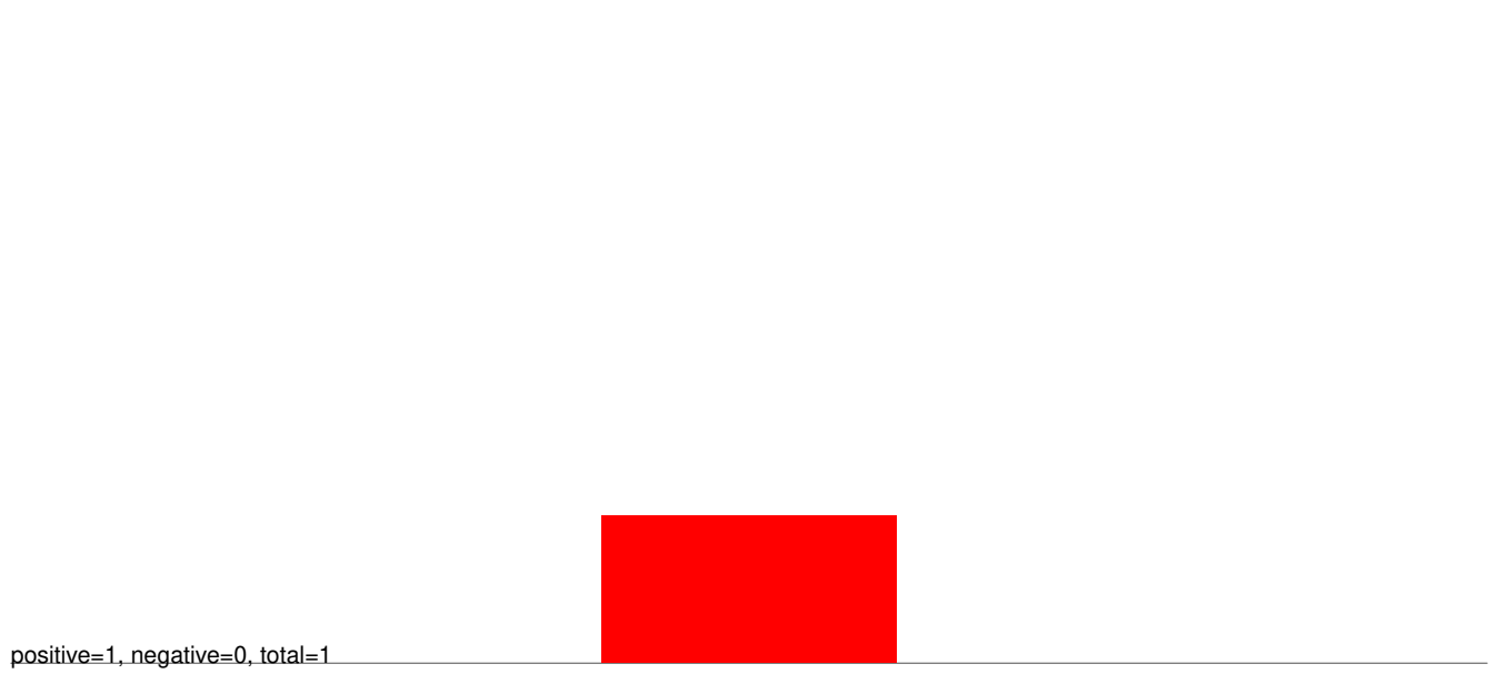
AnGam_Fem_Fat_body_rep1_KM.rep
