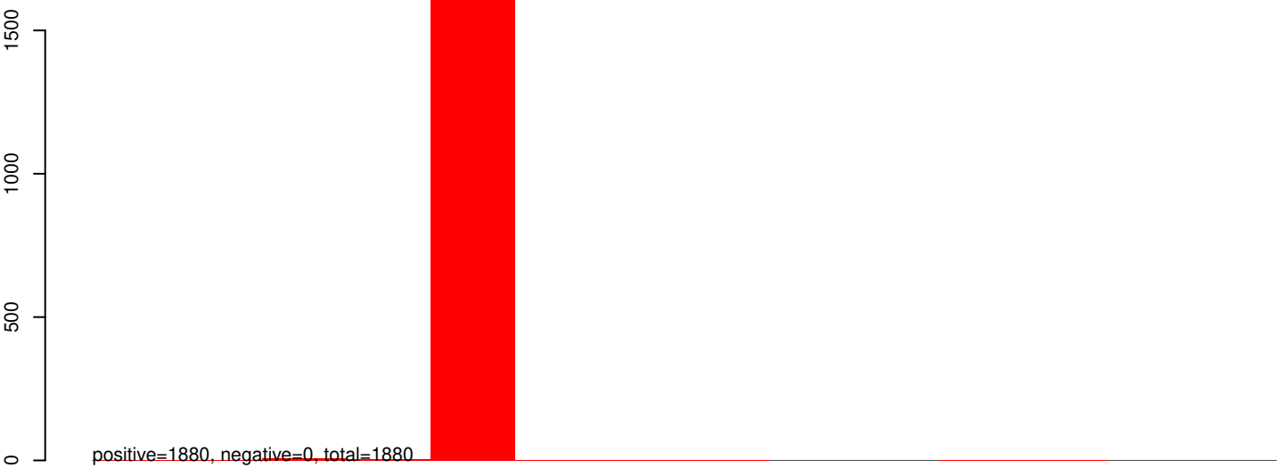
AnGam_Fem_Fat_body_rep1_KM.rep
