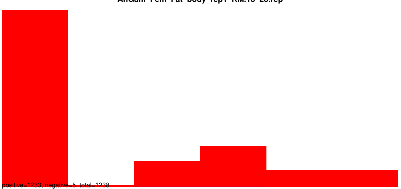
AnGam_Fem_Fat_body_rep1_KM.24_35.rep
