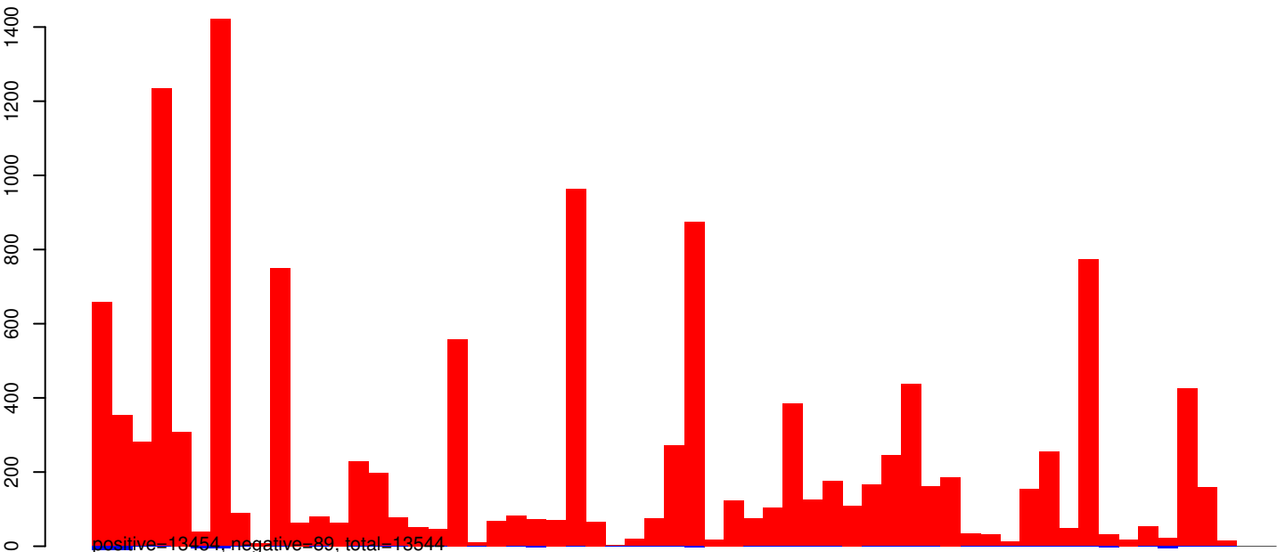
AnGam_Fem_Fat_body_rep1_KM.24_35.rep
