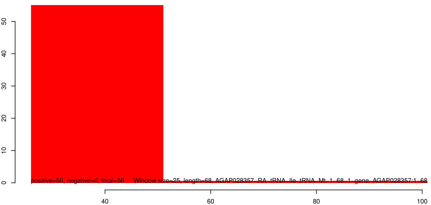
AnGam_Fem_Fat_body_rep1_KM.rep
