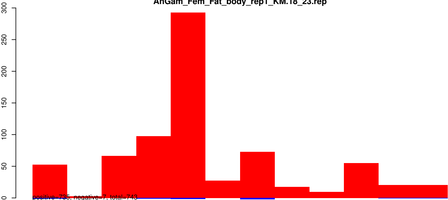
AnGam_Fem_Fat_body_rep1_KM.24_35.rep
