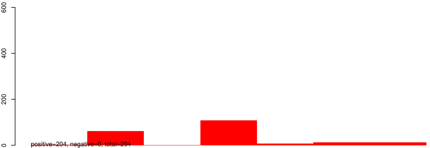
AnGam_Fem_Fat_body_rep1_KM.rep
