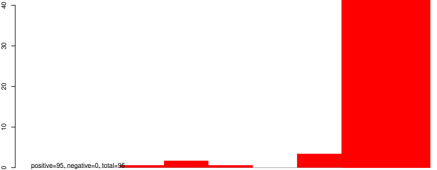
AnGam_Fem_Fat_body_rep1_KM.rep
