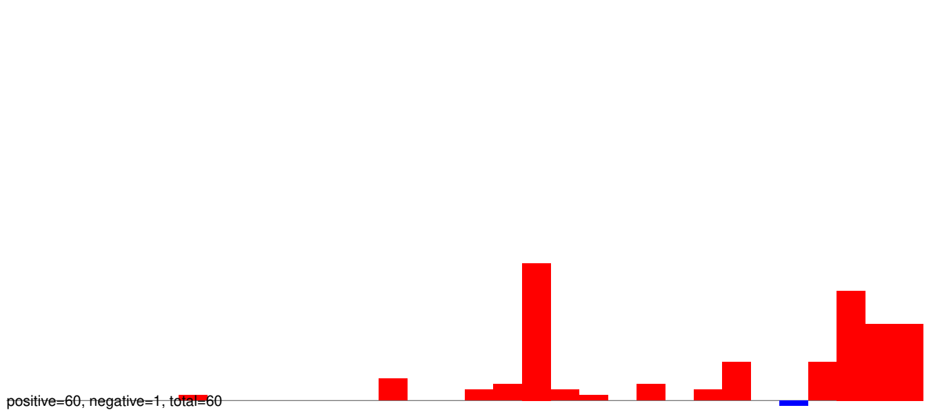
AnGam_Fem_Fat_body_rep1_KM.rep
