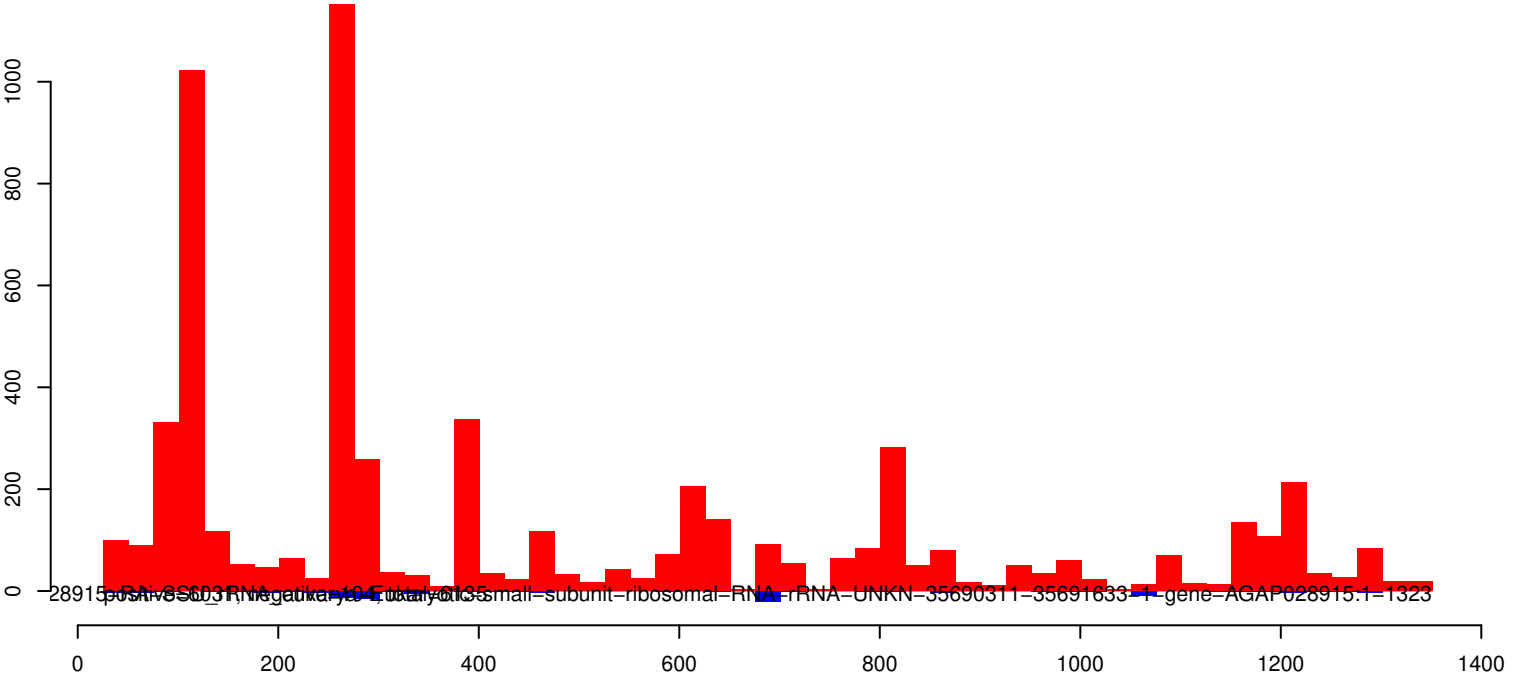
AnGam_Fem_Fat_body_rep1_KM.rep
