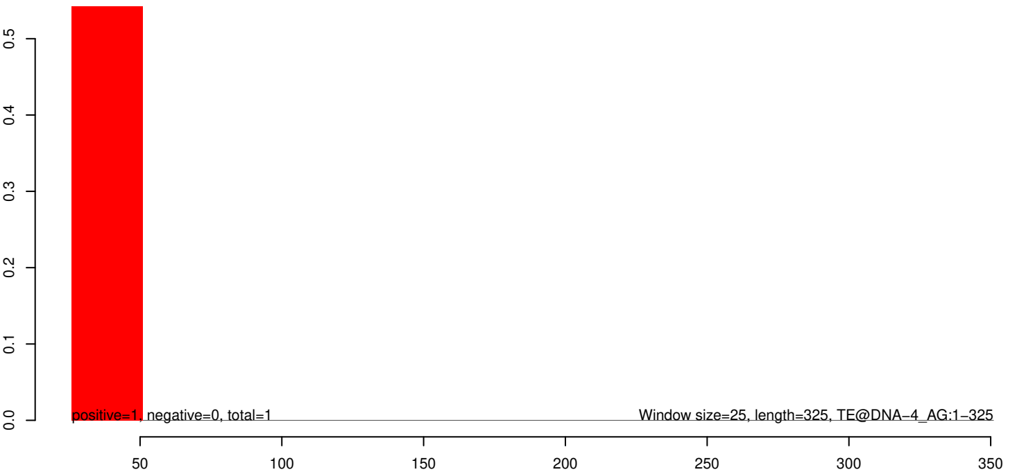
AnGam_Fem_Fat_body_rep2_KM.rep
