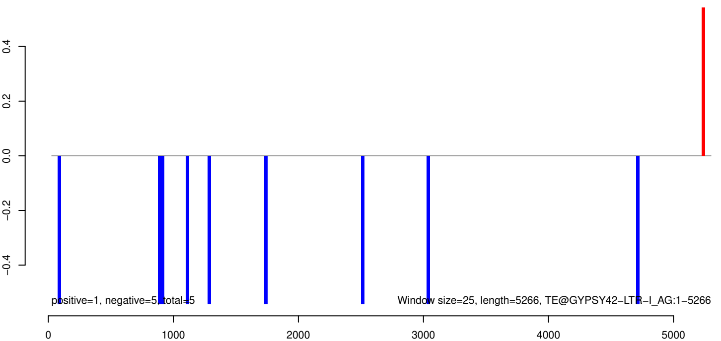
AnGam_Fem_Fat_body_rep2_KM.rep
