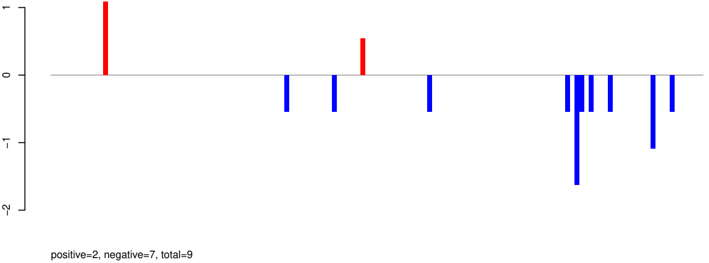
AnGam_Fem_Fat_body_rep2_KM.rep
