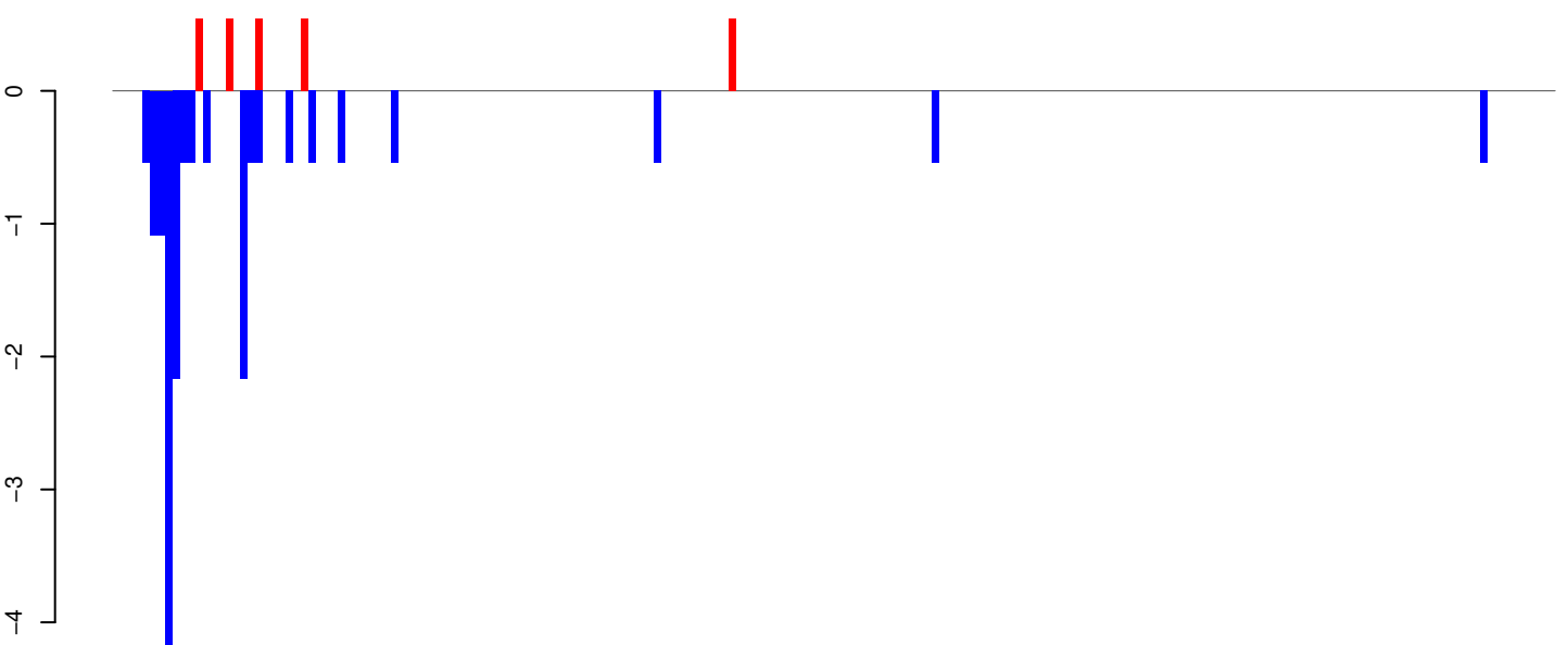
AnGam_Fem_Fat_body_rep2_KM.rep
