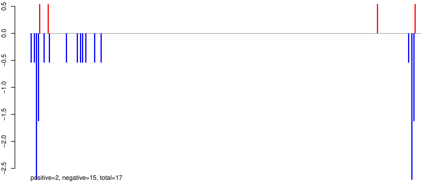
AnGam_Fem_Fat_body_rep2_KM.24_35.rep
