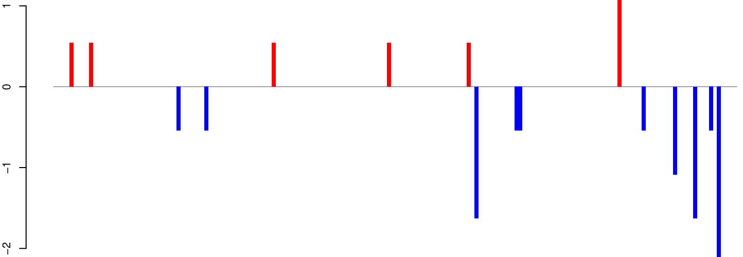
AnGam_Fem_Fat_body_rep2_KM.24_35.rep
