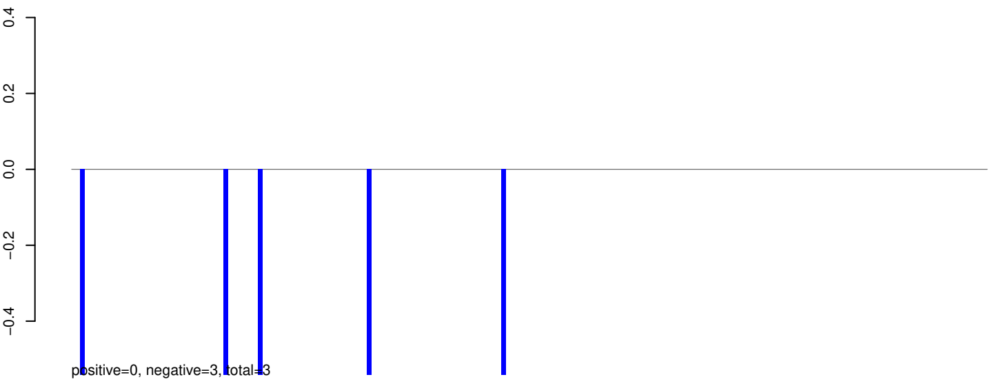
AnGam_Fem_Fat_body_rep2_KM.rep
