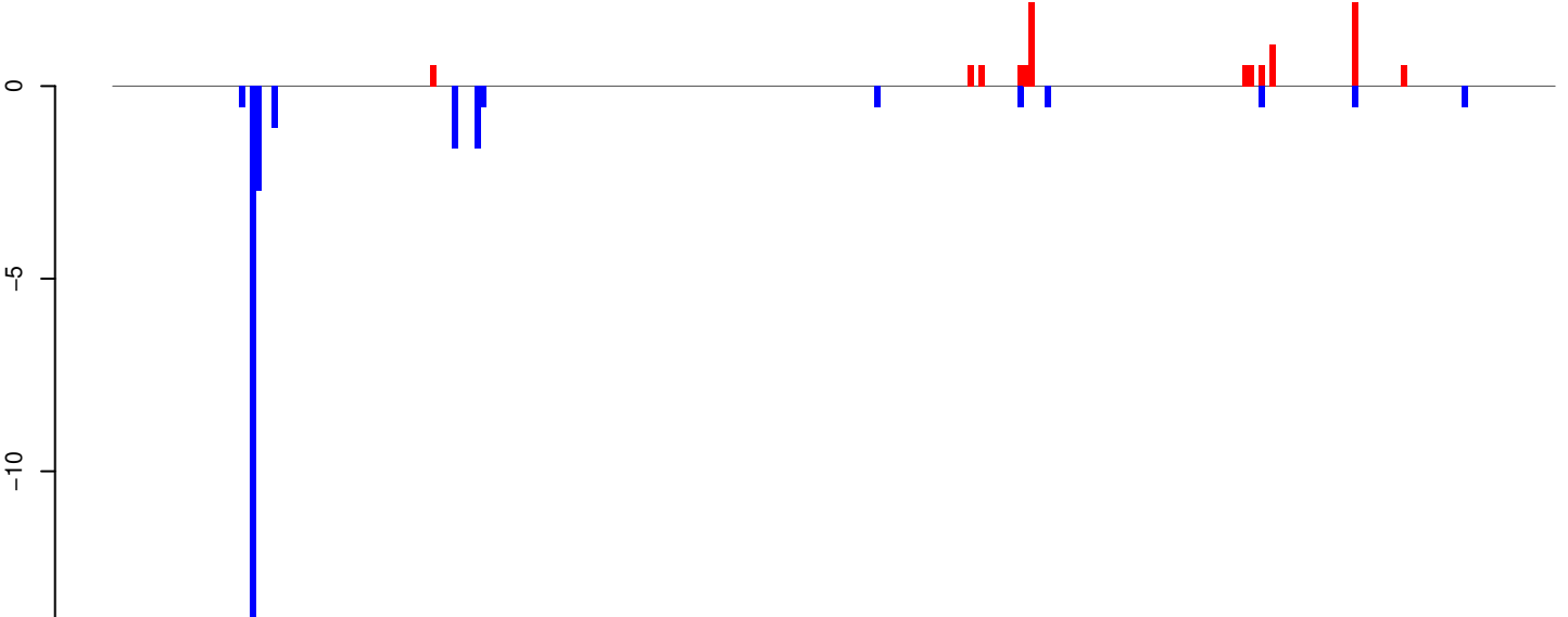
AnGam_Fem_Fat_body_rep2_KM.rep
