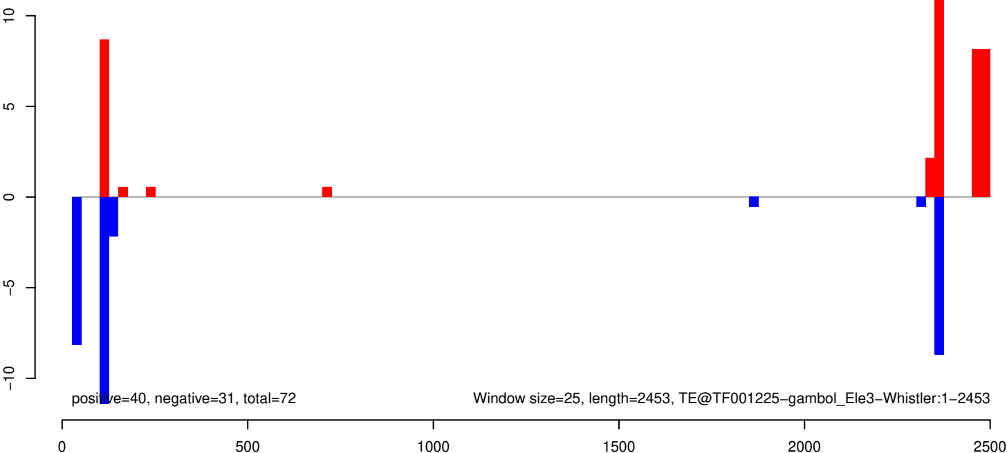
AnGam_Fem_Fat_body_rep2_KM.rep
