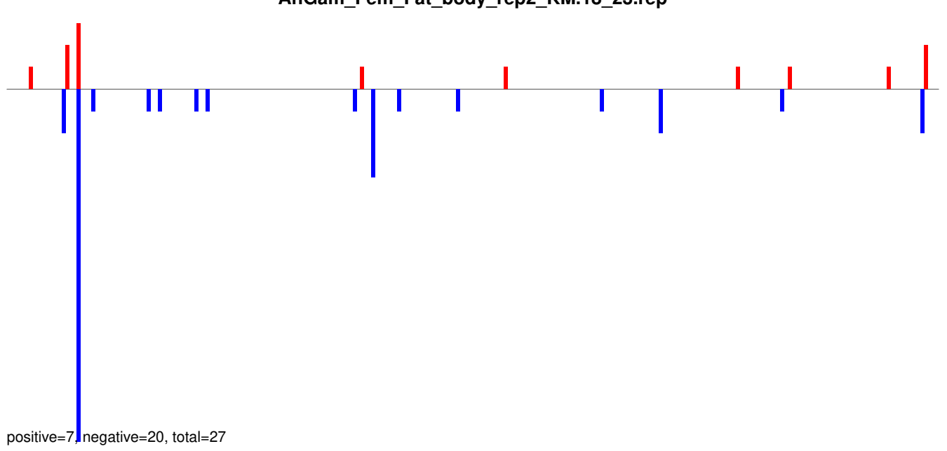
AnGam_Fem_Fat_body_rep2_KM.24_35.rep
