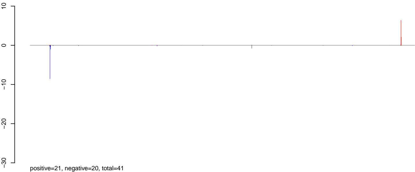
AnGam_WholeFemale_PBInfect_IB.24_35.rep
