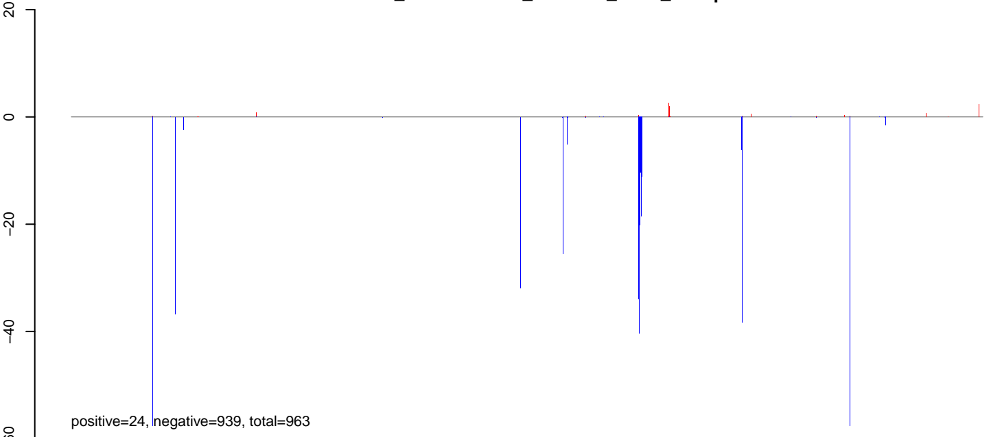
AnGam_WholeFemale_PBI infect_IB.rep
