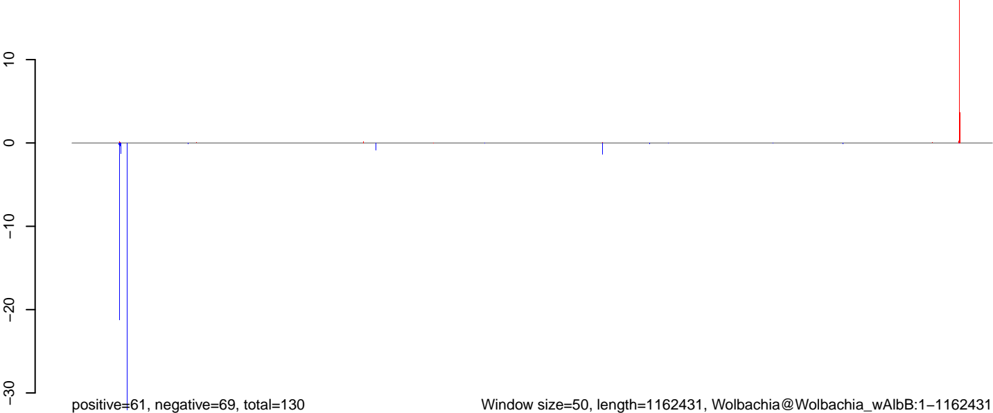
AnGam_WholeFemale_PBInfect_IB.rep
