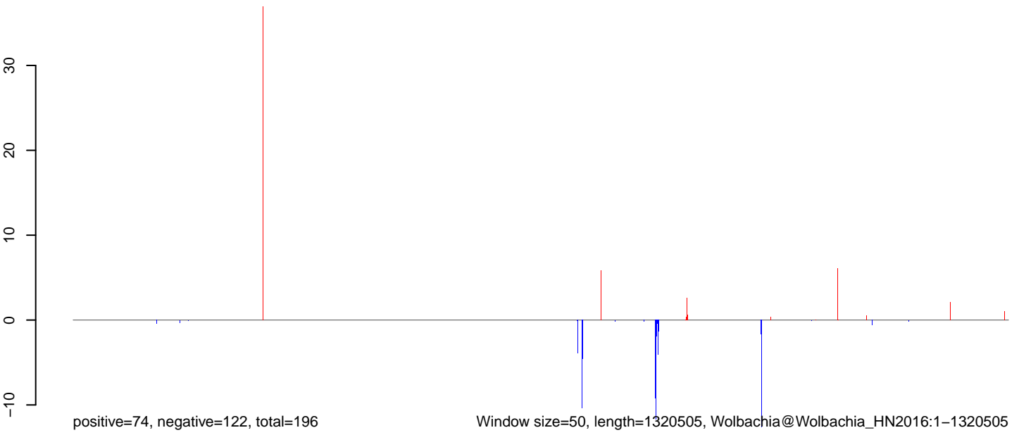
AnGam_larvae_male_TN.rep
