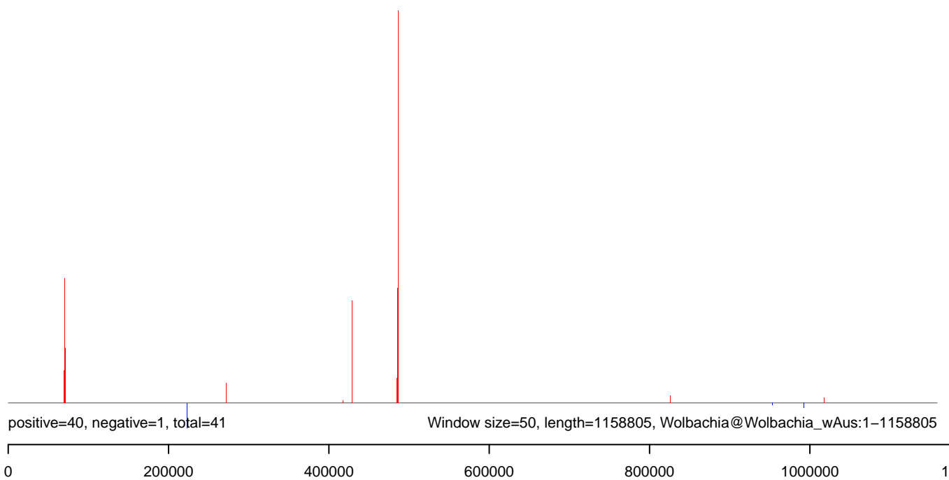
AnGam_larvae_male_TN.rep
