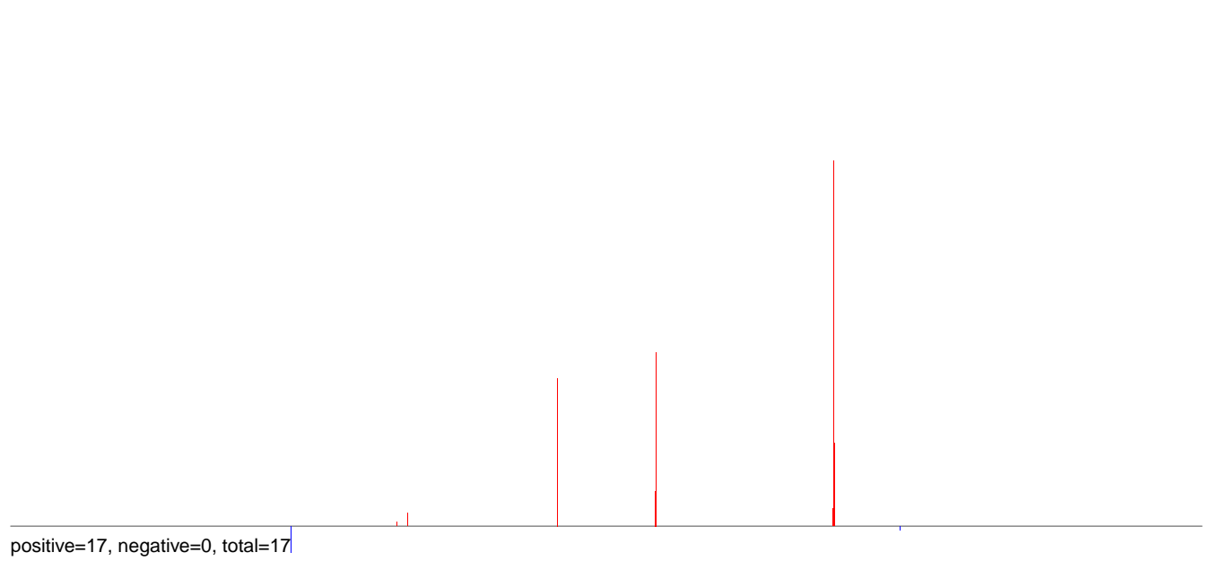
AnGam_larvae_male_TN.rep
