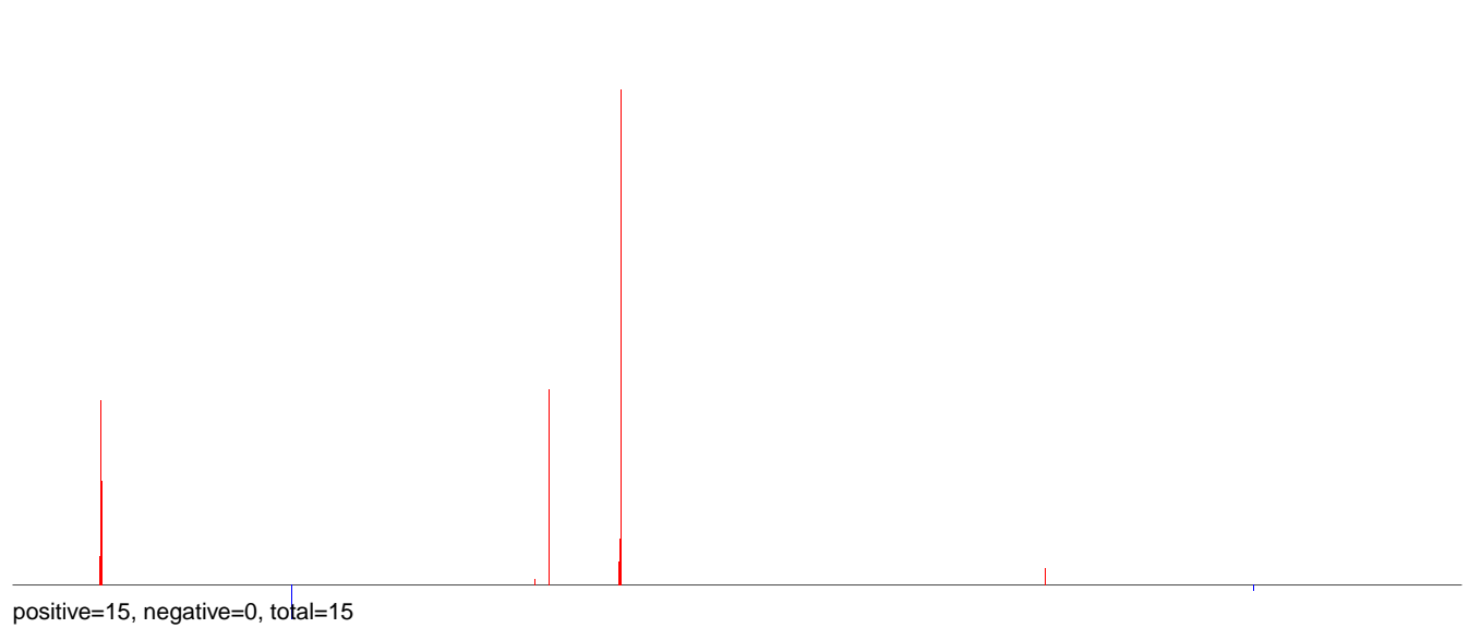
AnGam_larvae_male_TN.rep
