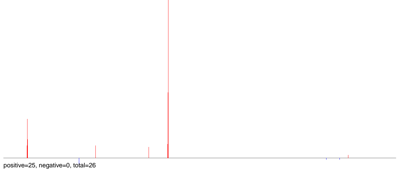
AnGam_larvae_male_TN.24_35.rep
