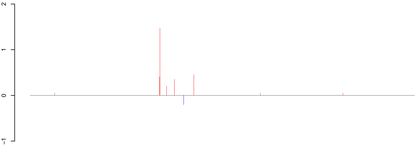
AnGam_larvae_male_TN.18_23.rep
