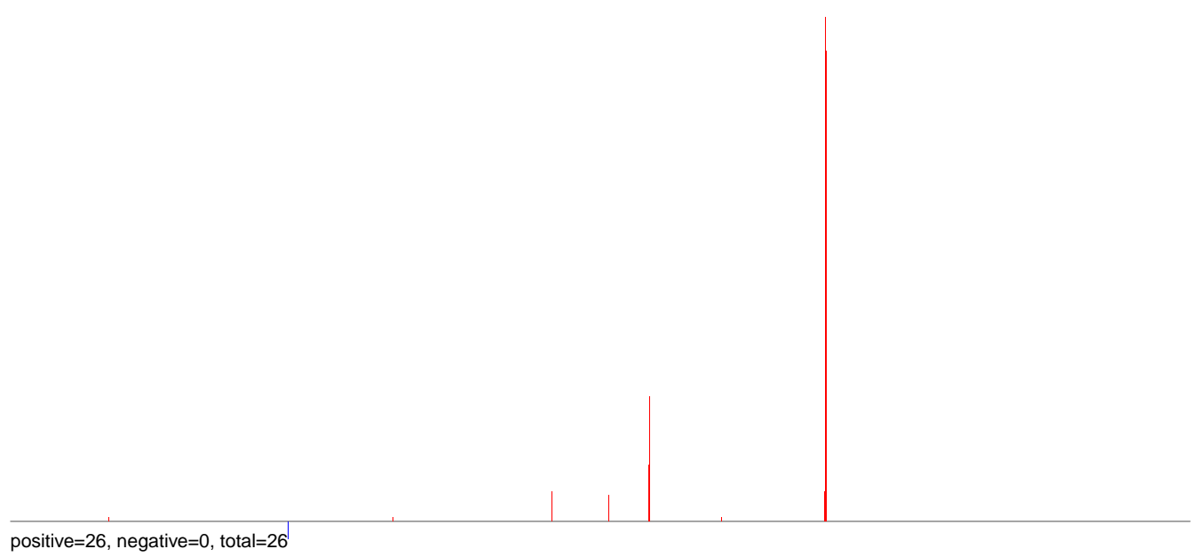
AnGam_larvae_male_TN.24_35.rep
