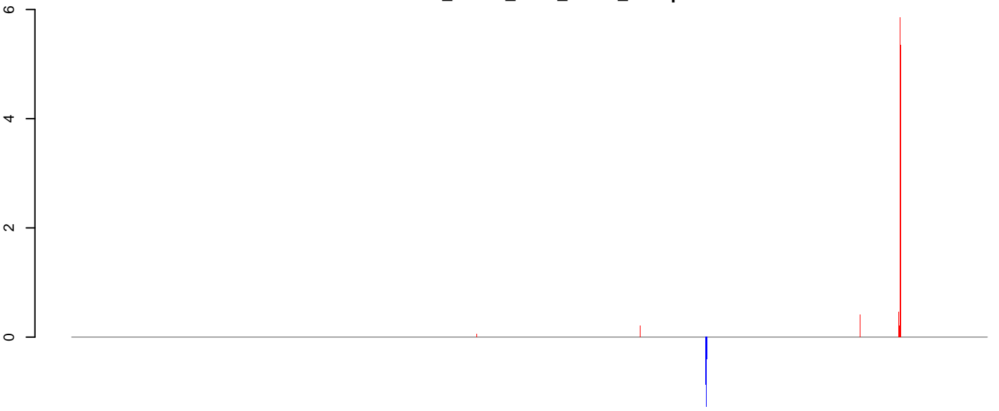
AnGam_larvae_male_TN.18_23.rep
