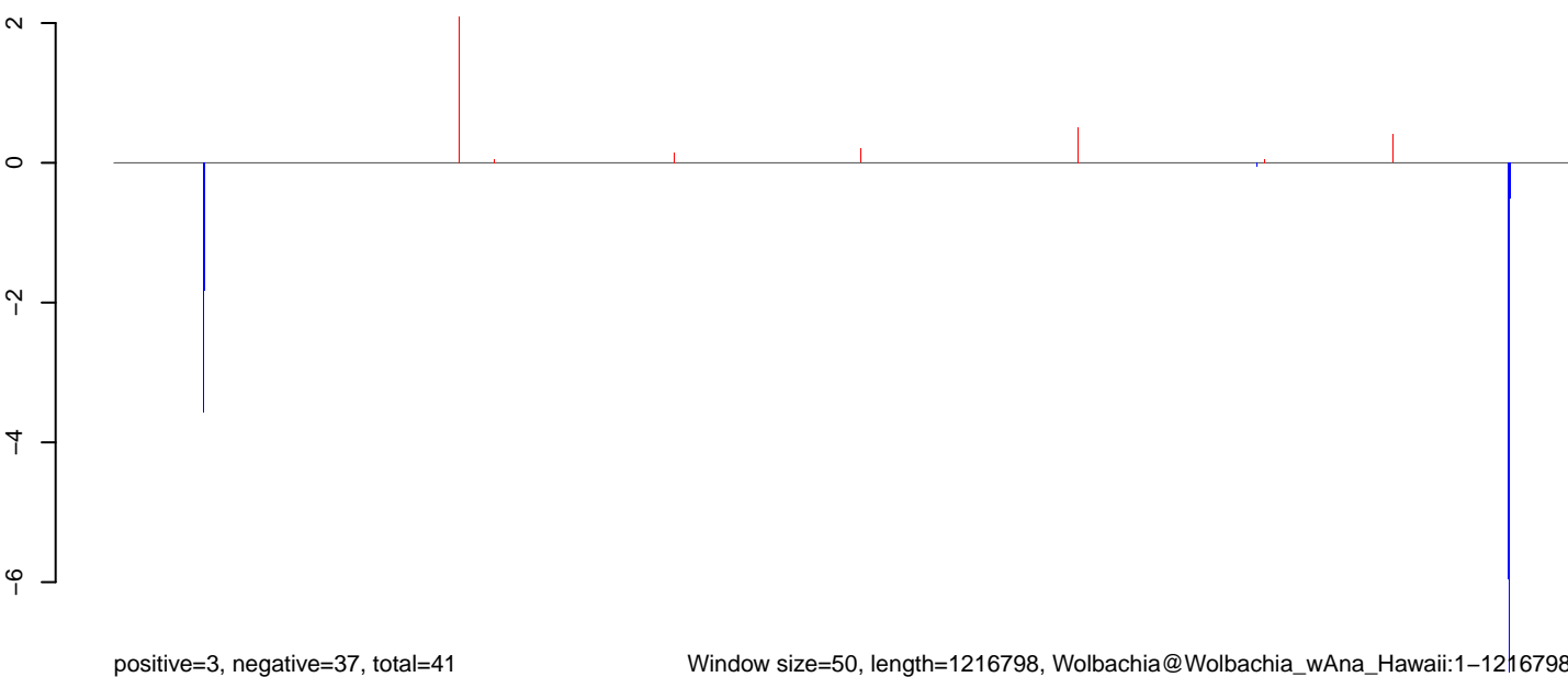
AnGam_larvae_male_TN.rep
