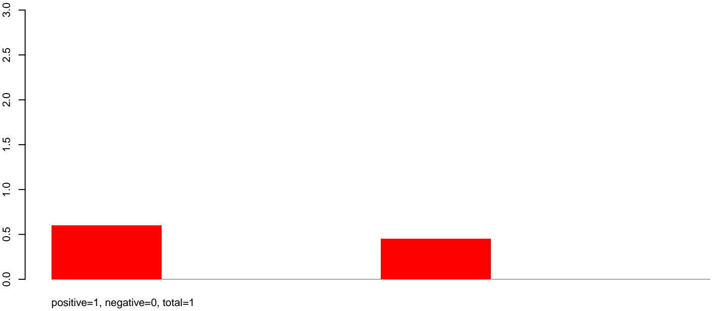
CuQuin_Hsu_30dpi_WNV1.rep
