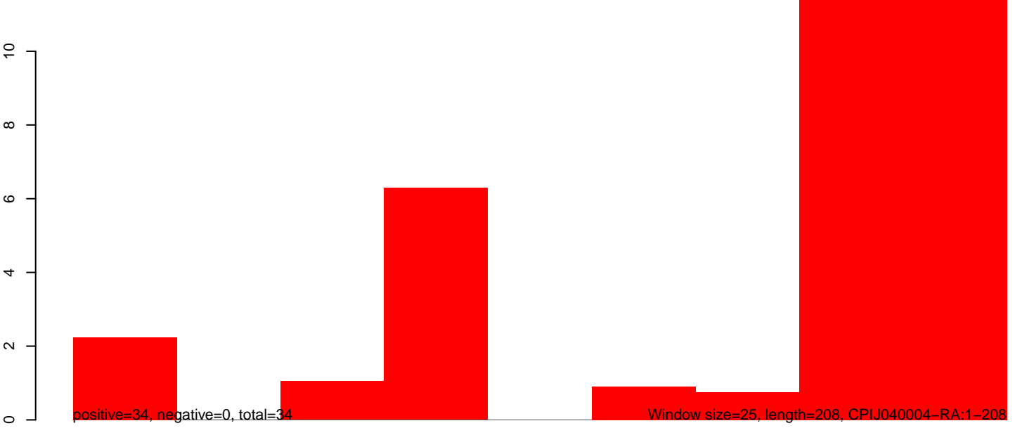
CuQuin_Hsu_30dpi_WNV1.rep
