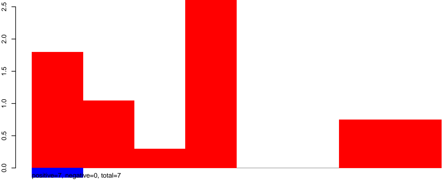
CuQuin_Hsu_30dpi_WNV1.24_35.rep
