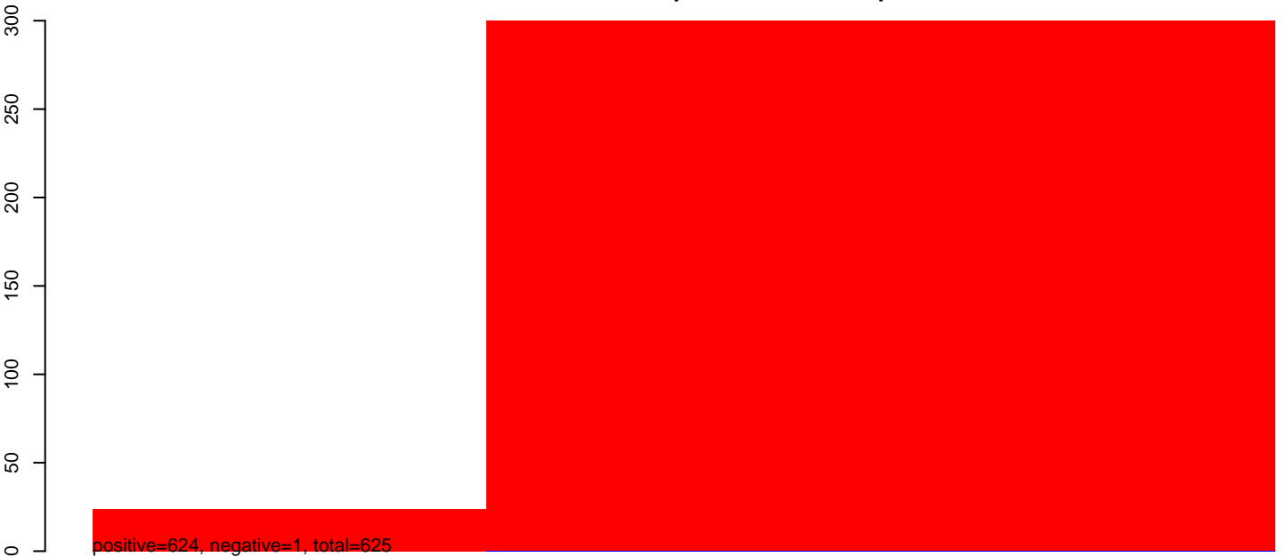
CuQuin_Hsu_30dpi_WNV1.24_35.rep
