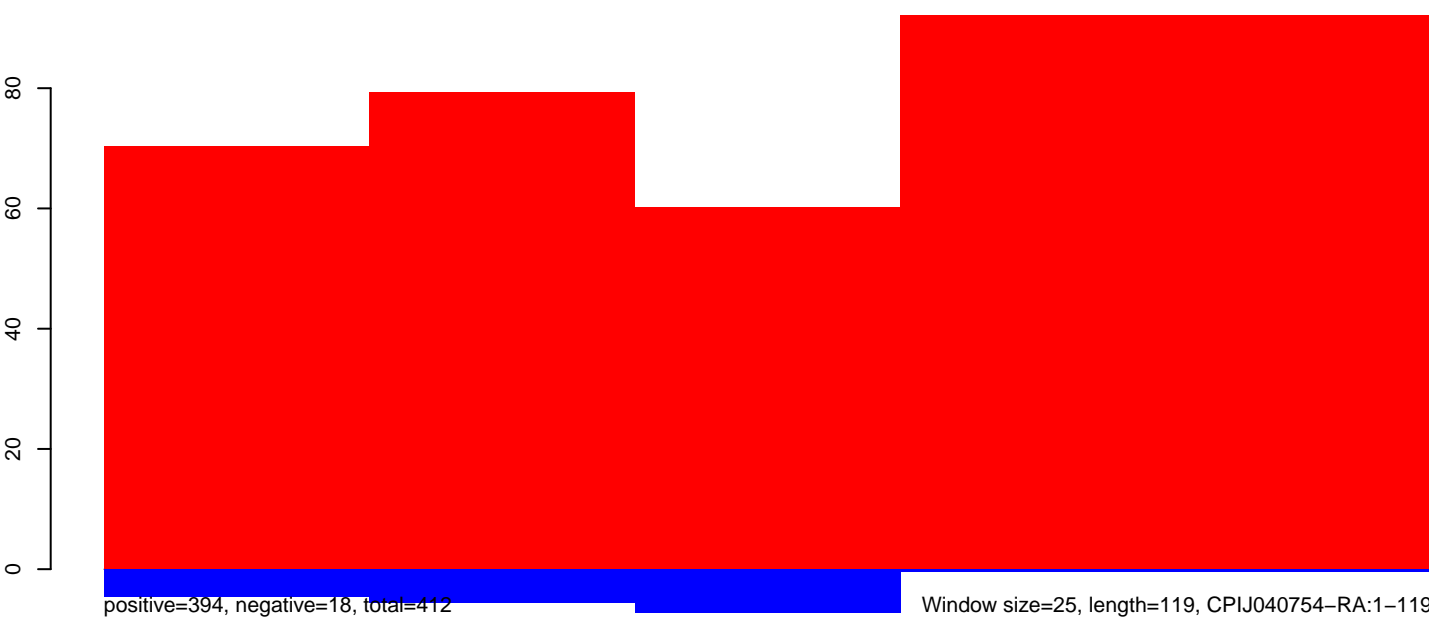
CuQuin_Hsu_30dpi_WNV1.rep
