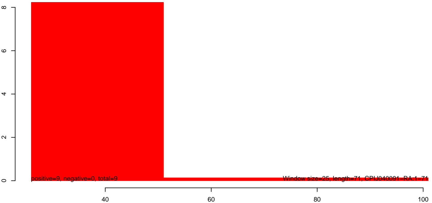
CuQuin_Hsu_30dpi_WNV1.rep
