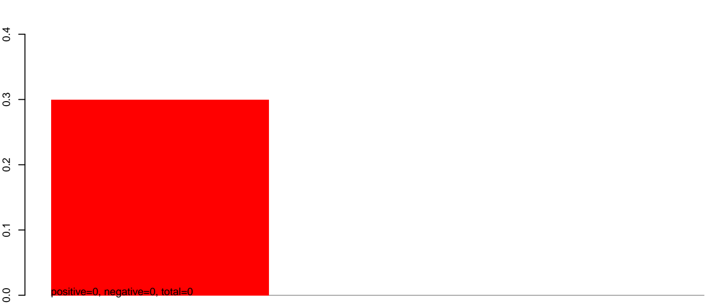
CuQuin_Hsu_30dpi_WNV1.rep
