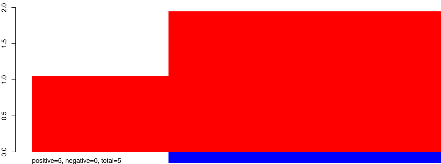
CuQuin_Hsu_30dpi_WNV1.24_35.rep
