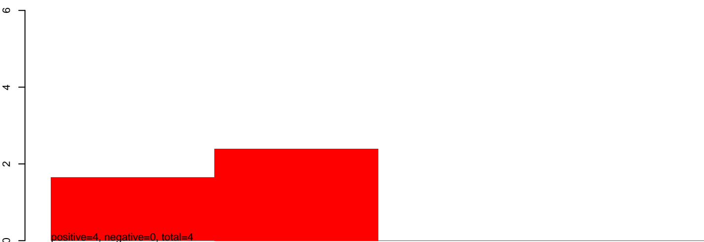
CuQuin_Hsu_30dpi_WNV1.rep
