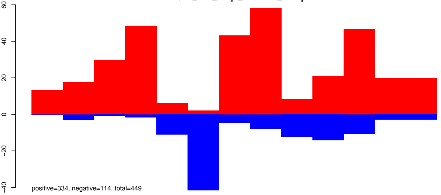
CuQuin_Hsu_30dpi_WNV1.24_35.rep
