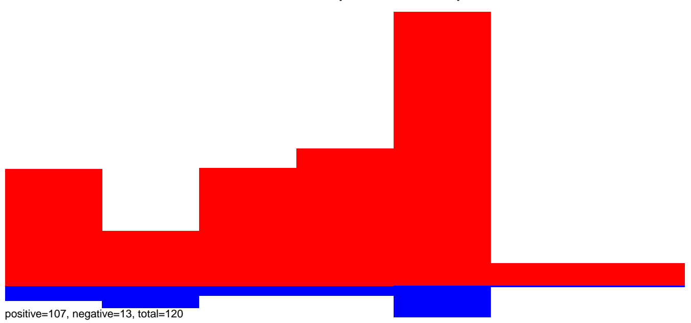
CuQuin_Hsu_30dpi_WNV1.24_35.rep
