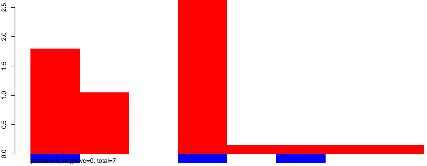
CuQuin_Hsu_30dpi_WNV1.24_35.rep
