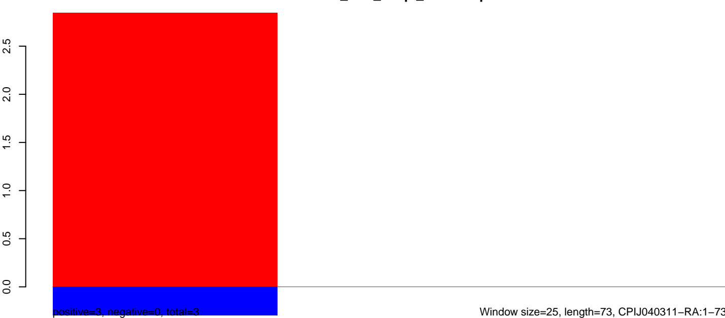
CuQuin_Hsu_30dpi_WNV1.rep
