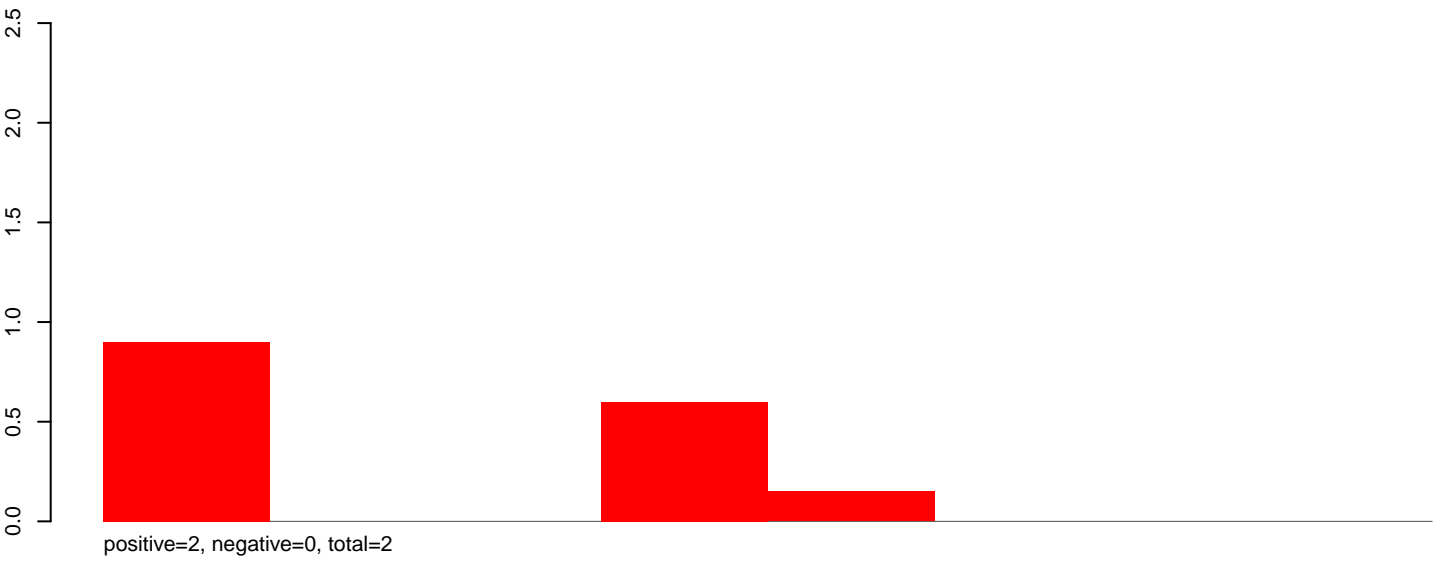
CuQuin_Hsu_30dpi_WNV1.rep
