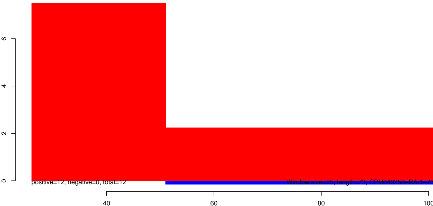
CuQuin_Hsu_30dpi_WNV1.rep
