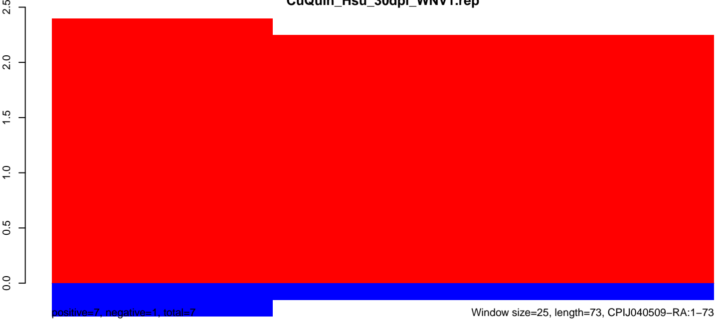
CuQuin_Hsu_30dpi_WNV1.rep
