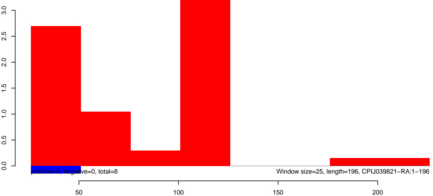
CuQuin_Hsu_30dpi_WNV1.rep
