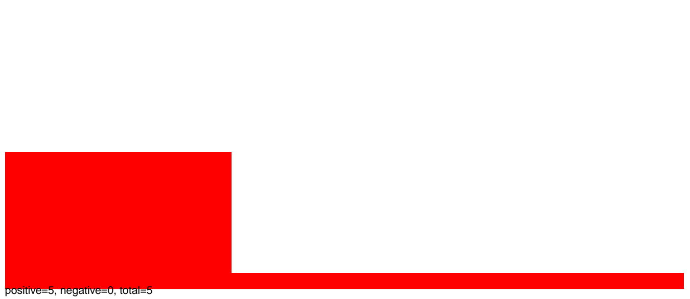
CuQuin_Hsu_30dpi_WNV1.rep
