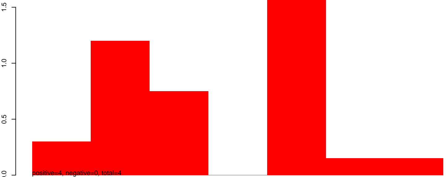
CuQuin_Hsu_30dpi_WNV1.24_35.rep
