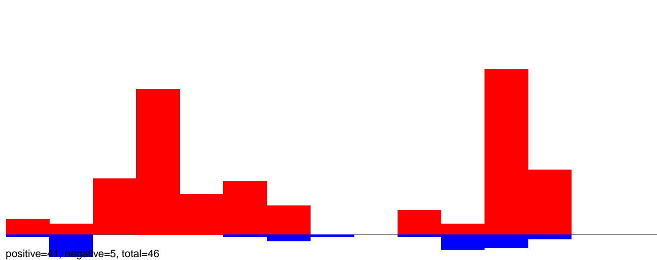
CuQuin_Hsu_30dpi_WNV1.24_35.rep
