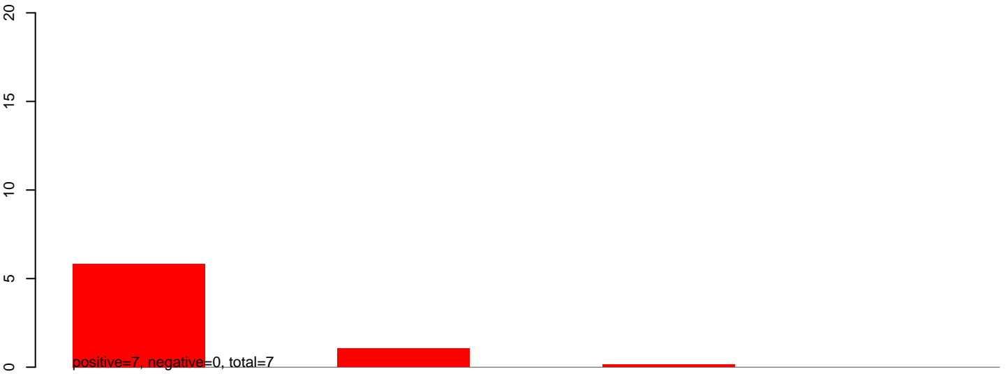
CuQuin_Hsu_30dpi_WNV1.rep
