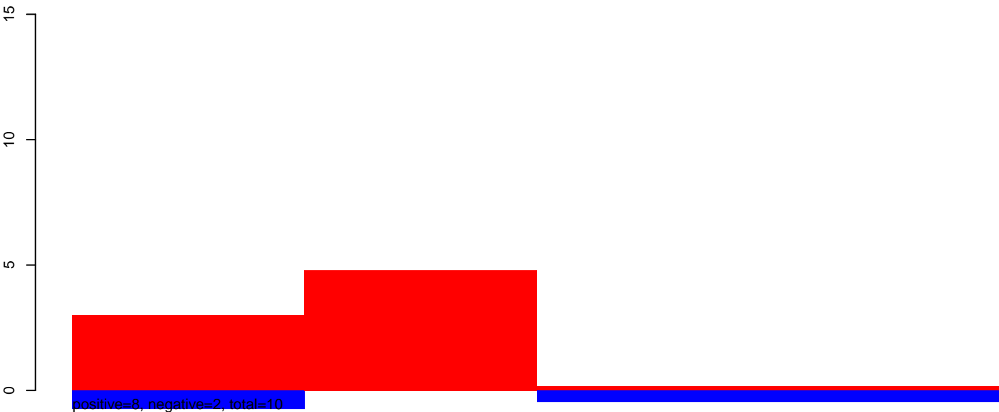
CuQuin_Hsu_30dpi_WNV1.24_35.rep
