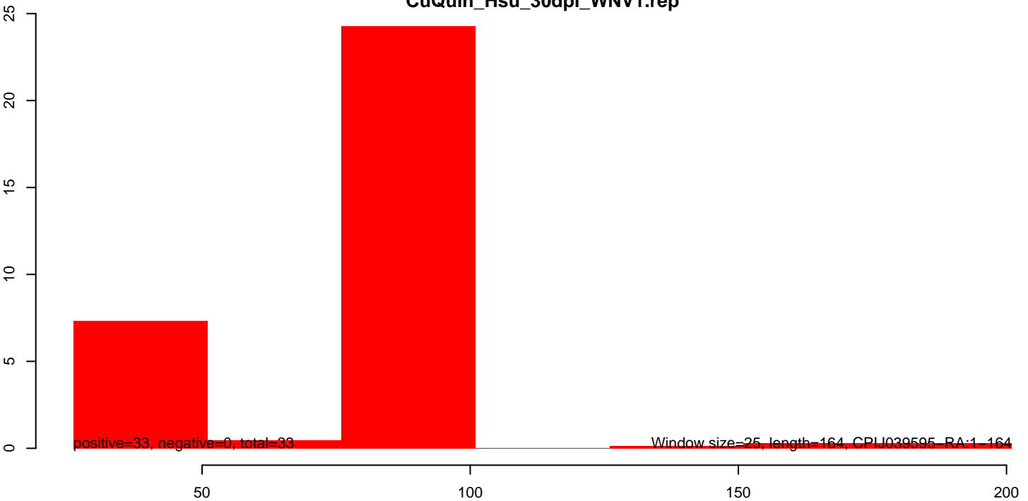
CuQuin_Hsu_30dpi_WNV1.rep
