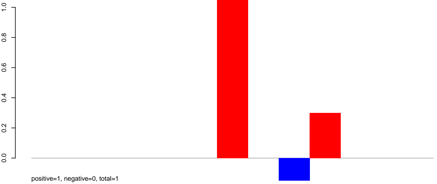
CuQuin_Hsu_30dpi_WNV1.24_35.rep
