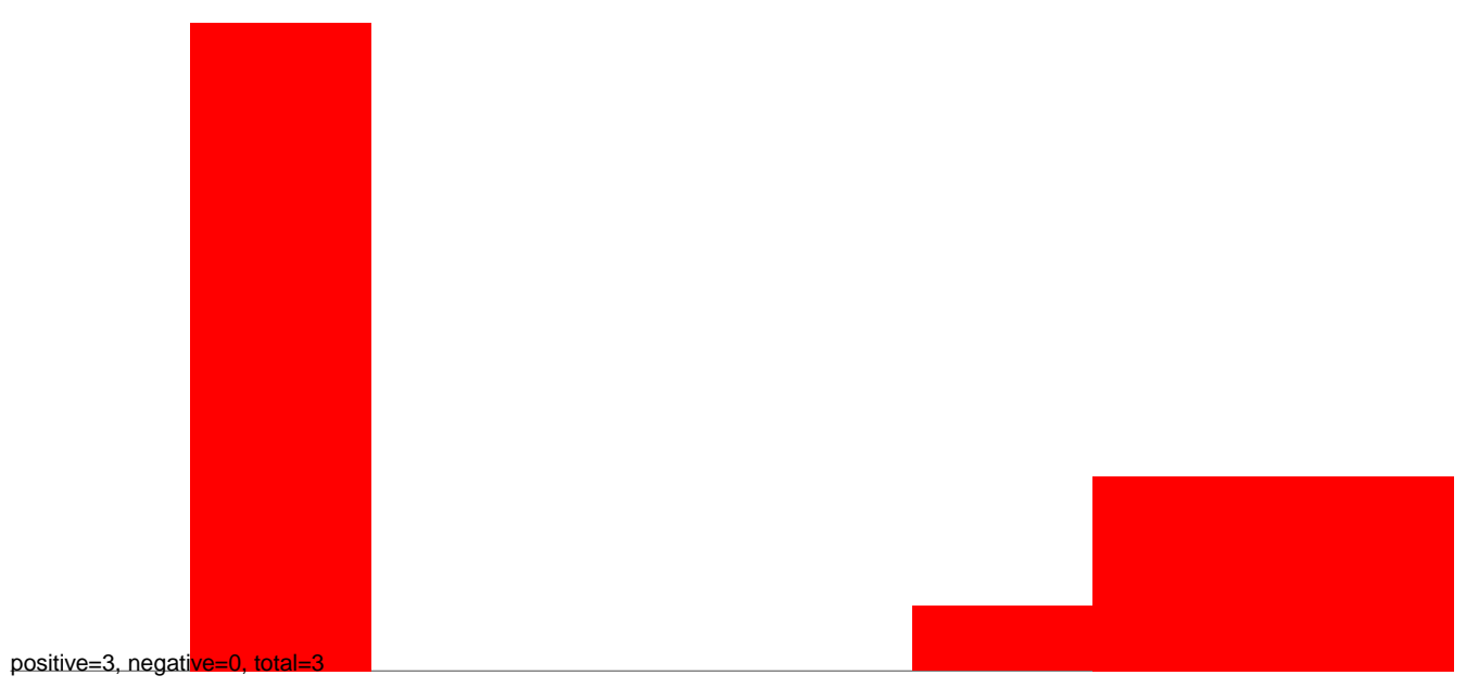
CuQuin_Hsu_30dpi_WNV1.rep
