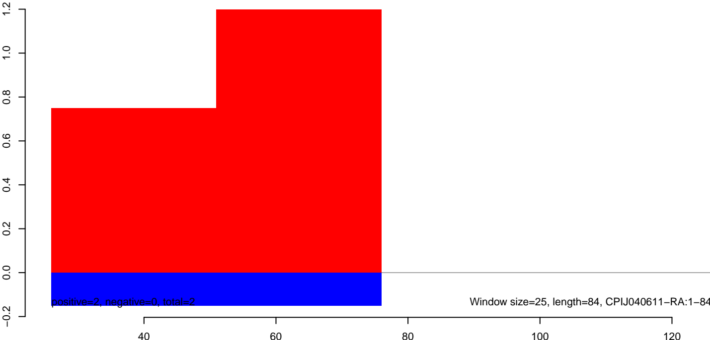
CuQuin_Hsu_30dpi_WNV1.rep
