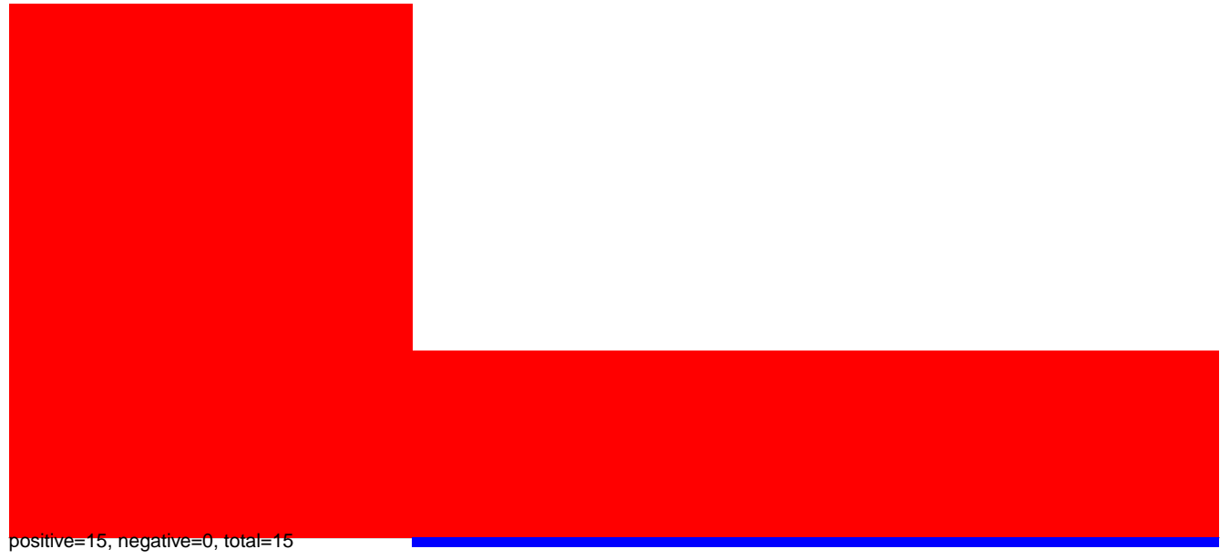
CuQuin_Hsu_30dpi_WNV1.24_35.rep
