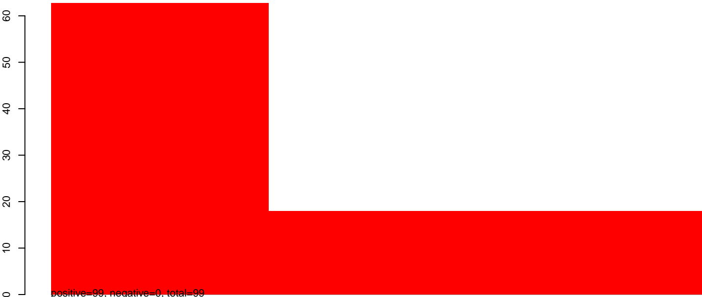
CuQuin_Hsu_30dpi_WNV1.rep
