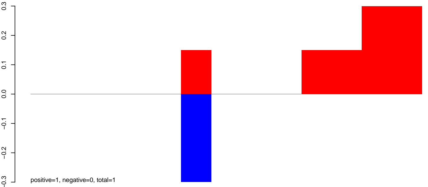
CuQuin_Hsu_30dpi_WNV1.24_35.rep
