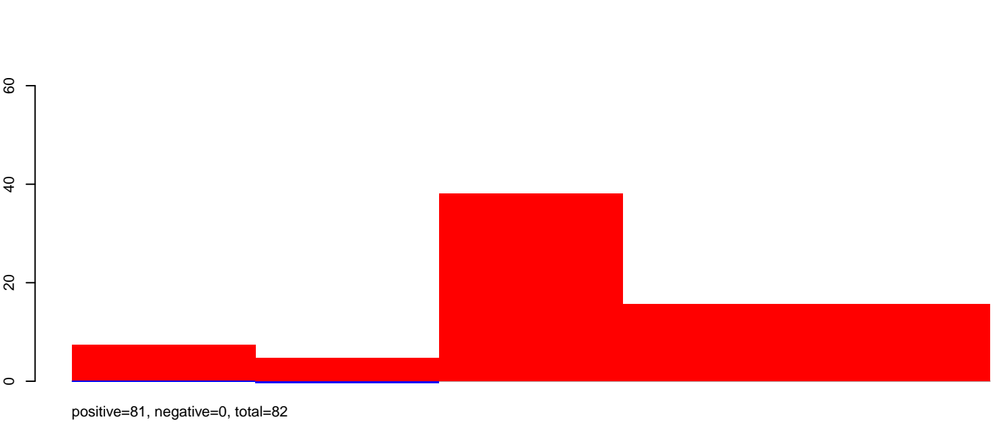
CuQuin_Hsu_30dpi_WNV1.rep
