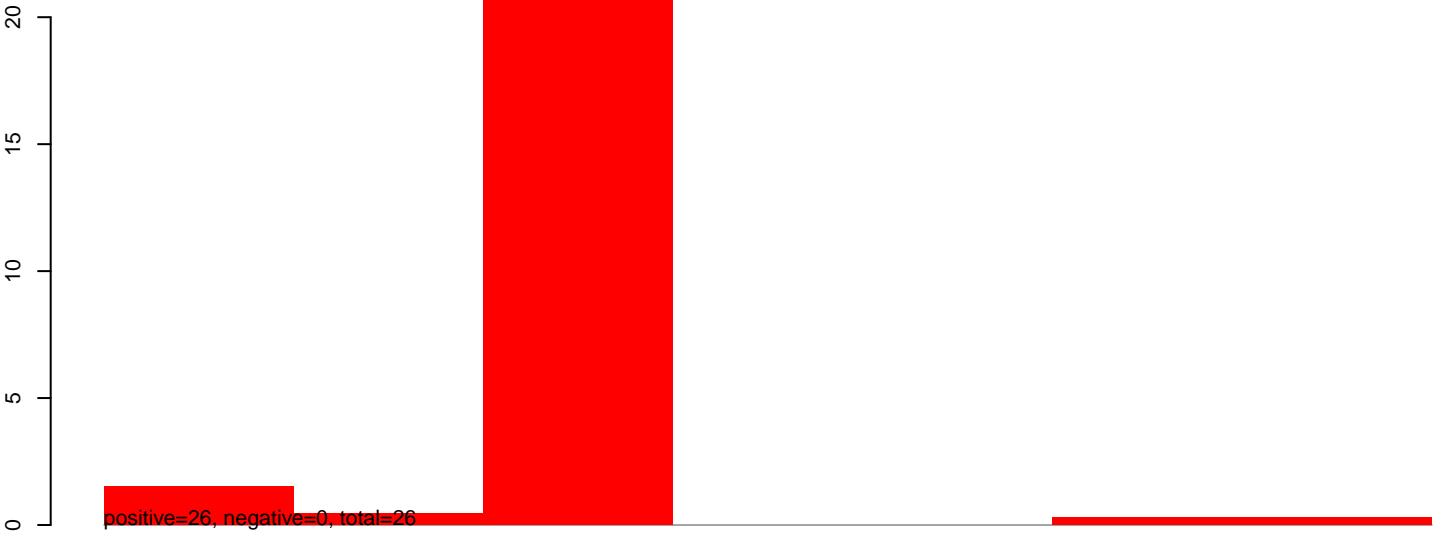
CuQuin_Hsu_30dpi_WNV1.24_35.rep
