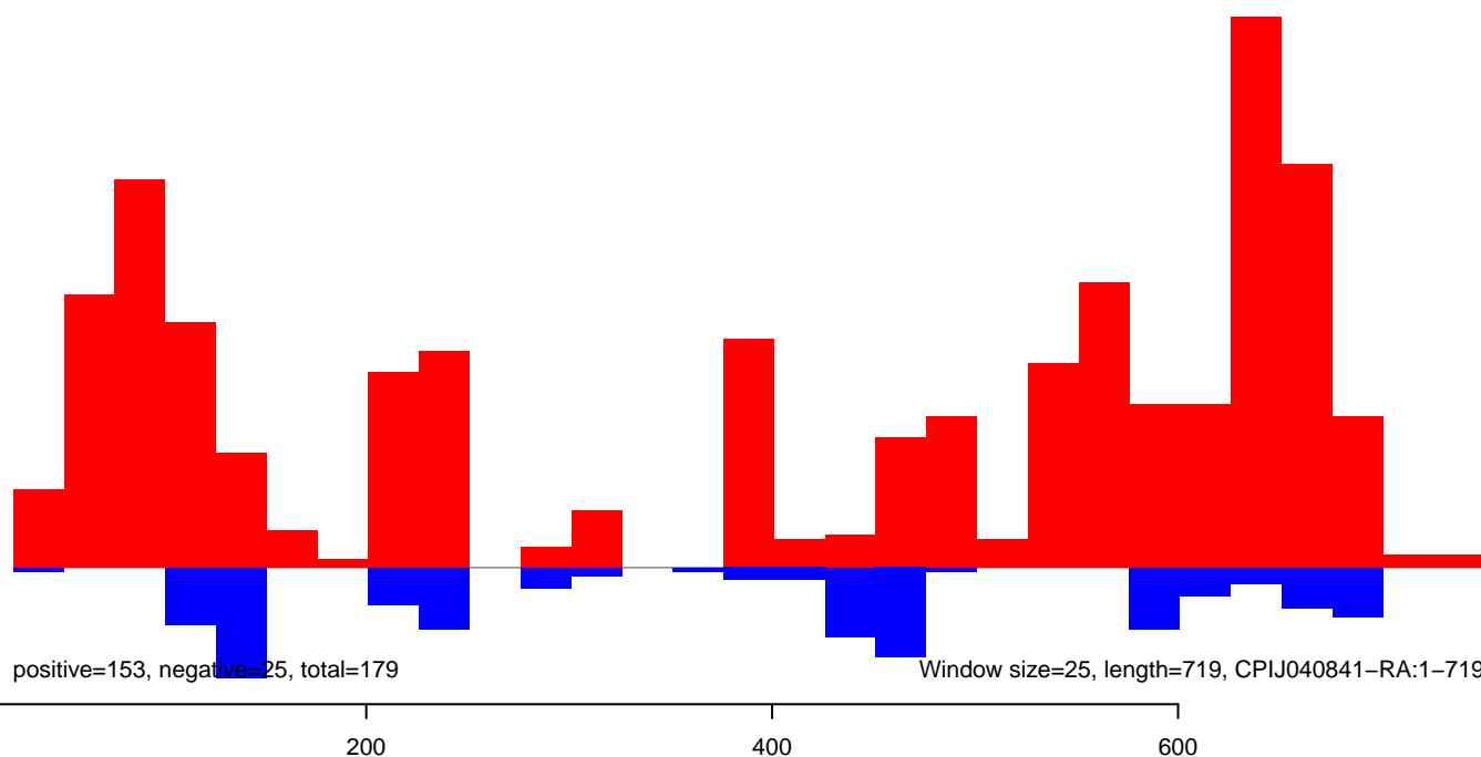
CuQuin_Hsu_30dpi_WNV1.rep
