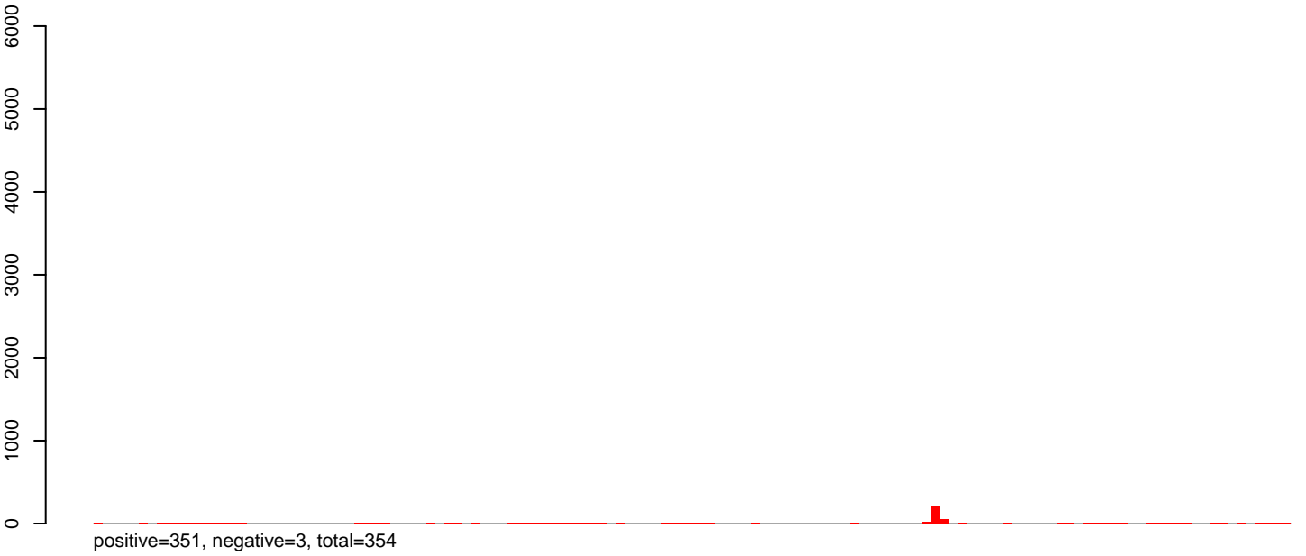
CuQuin_Hsu_30dpi_WNV1.rep
