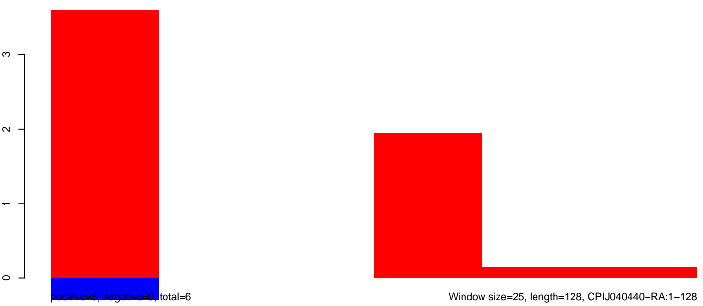
CuQuin_Hsu_30dpi_WNV1.rep
