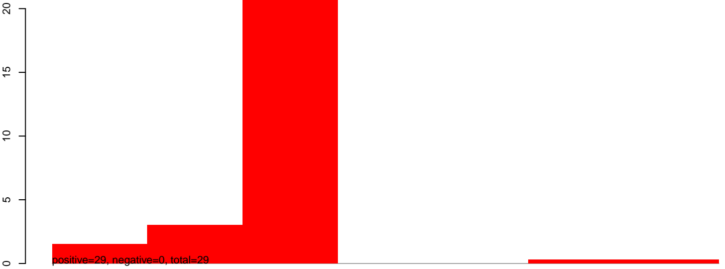
CuQuin_Hsu_30dpi_WNV1.24_35.rep
