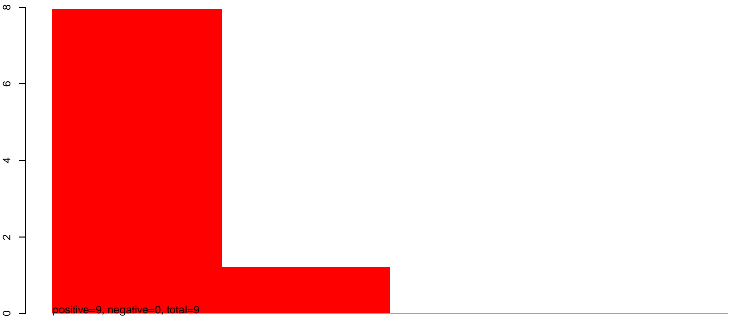
CuQuin_Hsu_30dpi_WNV1.24_35.rep
