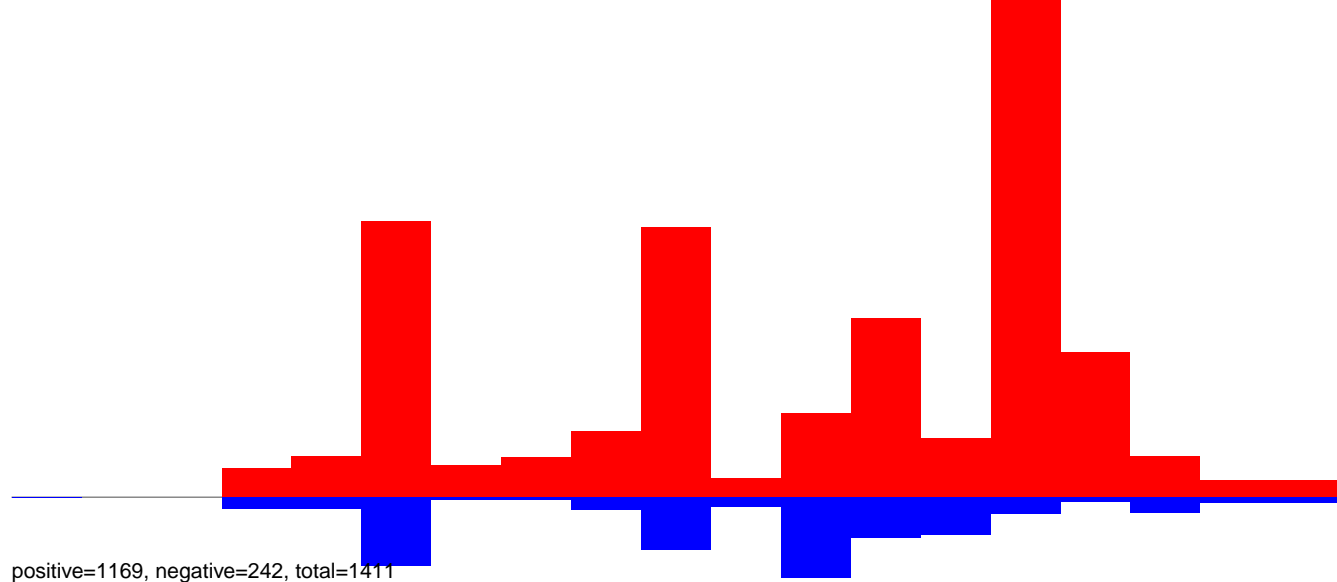
CuQuin_Hsu_30dpi_WNV1.24_35.rep
