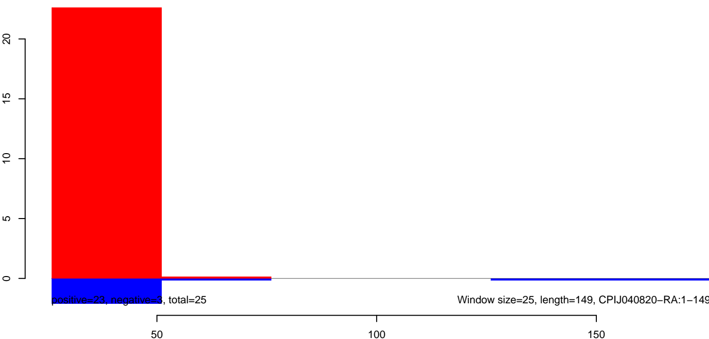
CuQuin_Hsu_30dpi_WNV1.rep
