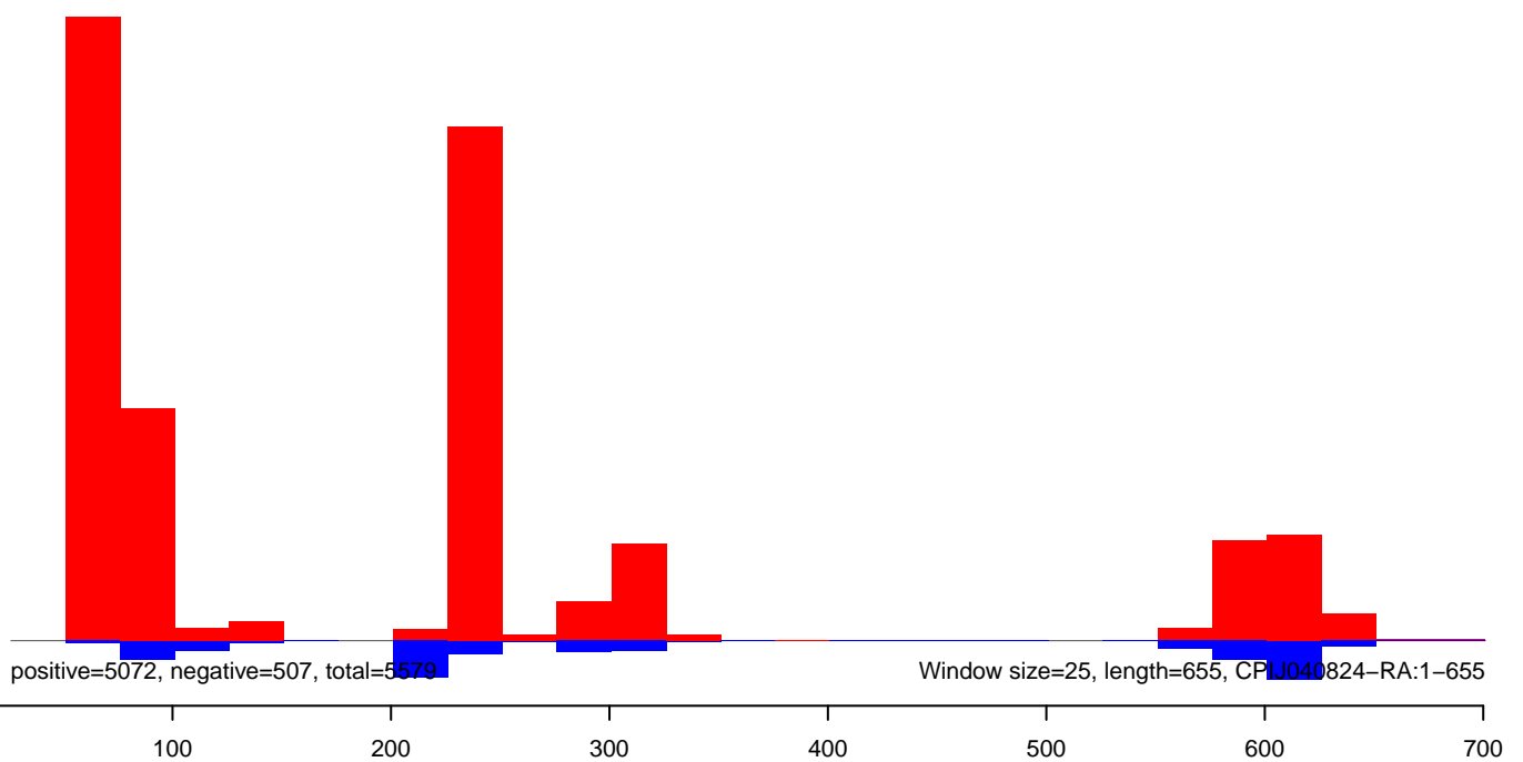
CuQuin_Hsu_30dpi_WNV1.rep
