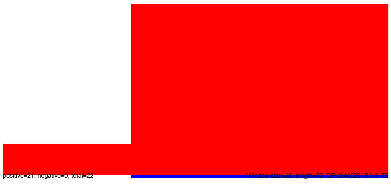
CuQuin_Hsu_30dpi_WNV1.rep
