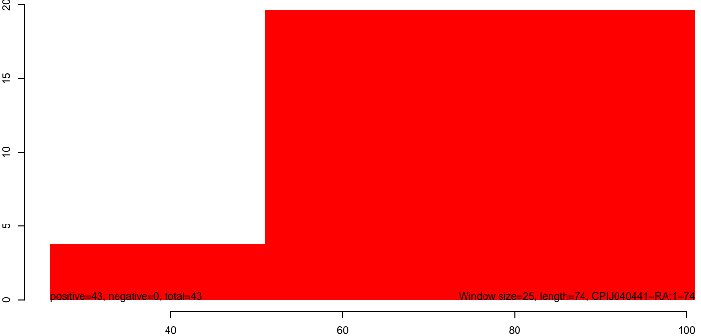
CuQuin_Hsu_30dpi_WNV1.rep
