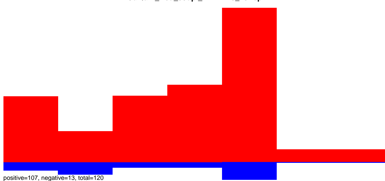
CuQuin_Hsu_30dpi_WNV1.24_35.rep
