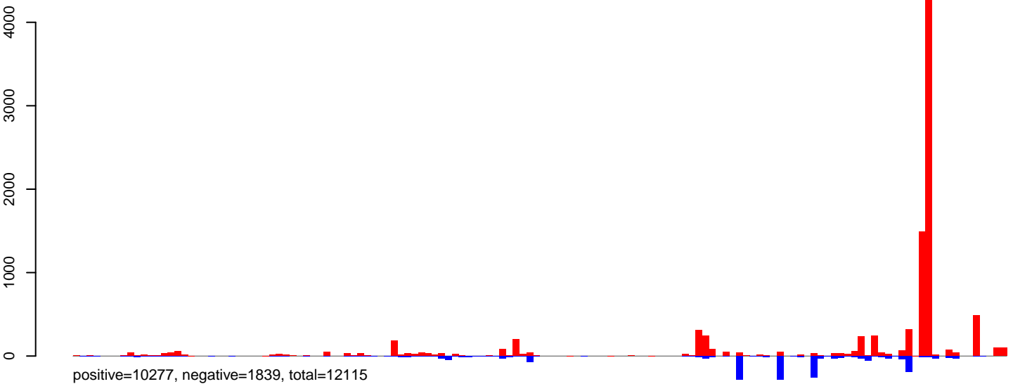
CuQuin_Hsu_30dpi_WNV1.24_35.rep
