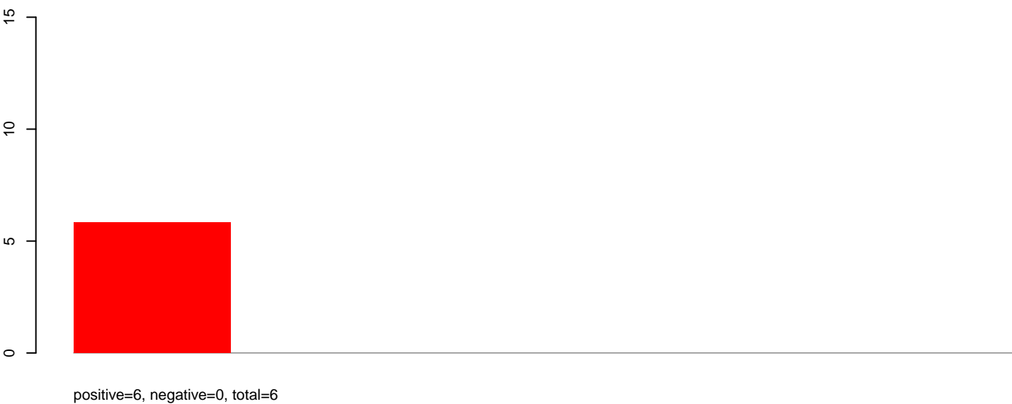
CuQuin_Hsu_30dpi_WNV1.rep
