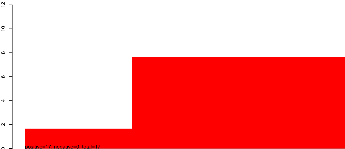
CuQuin_Hsu_30dpi_WNV1.24_35.rep
