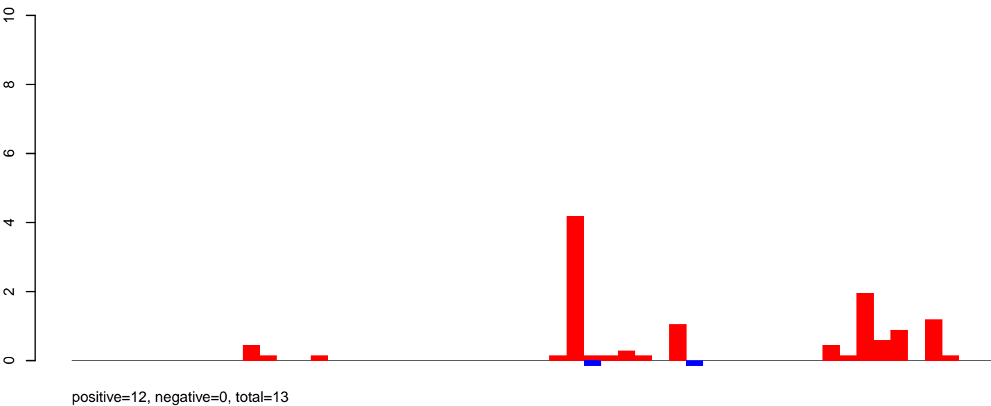
CuQuin_Hsu_30dpi_WNV1.rep
