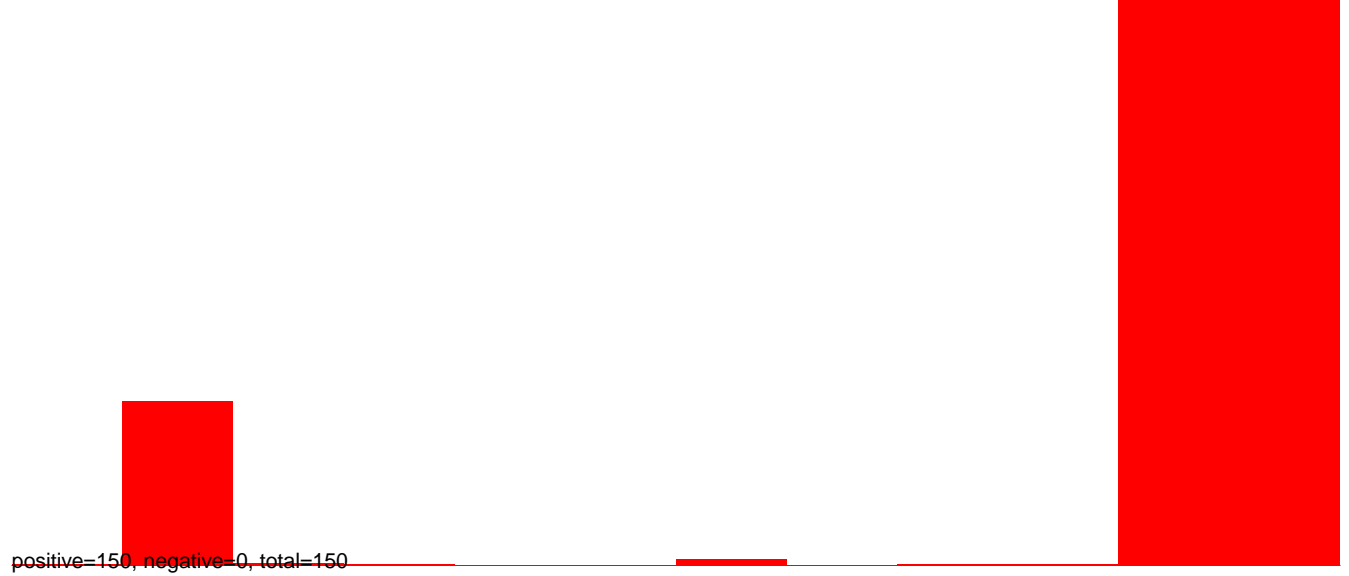
CuQuin_Hsu_30dpi_WNV1.rep
