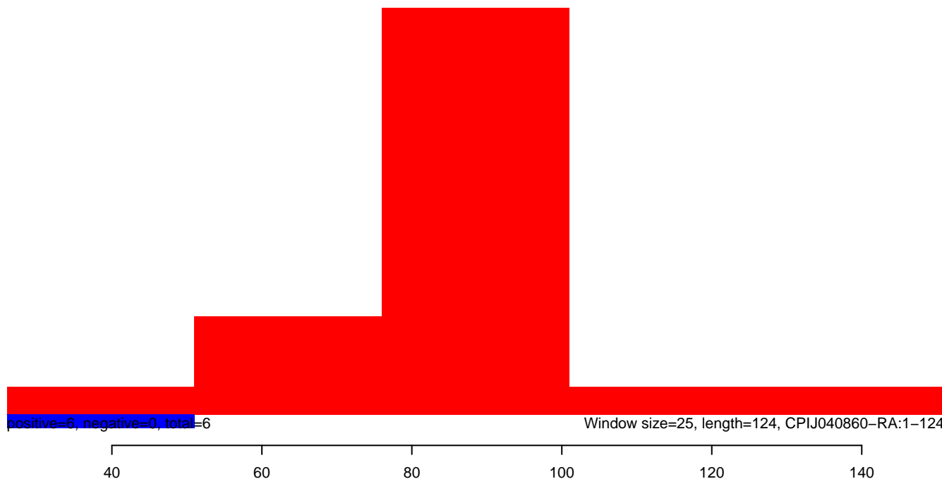
CuQuin_Hsu_30dpi_WNV1.rep
