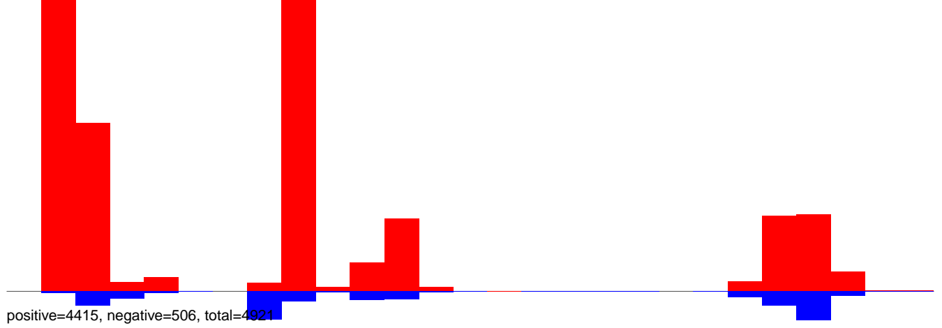
CuQuin_Hsu_30dpi_WNV1.24_35.rep
