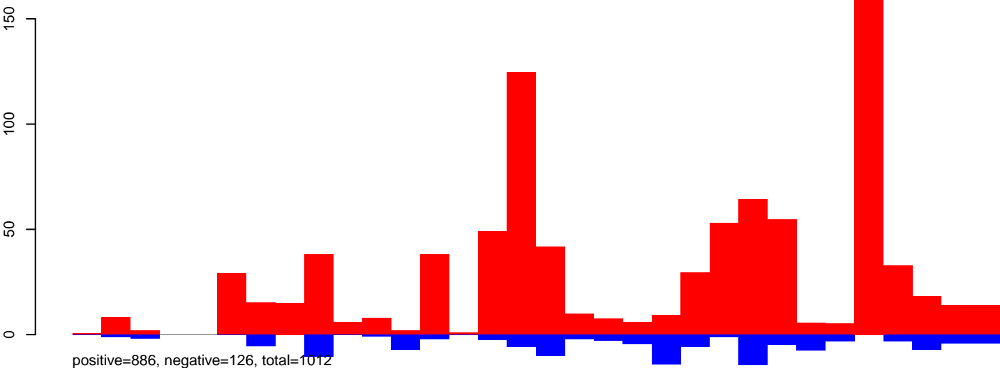
CuQuin_Hsu_30dpi_WNV1.24_35.rep
