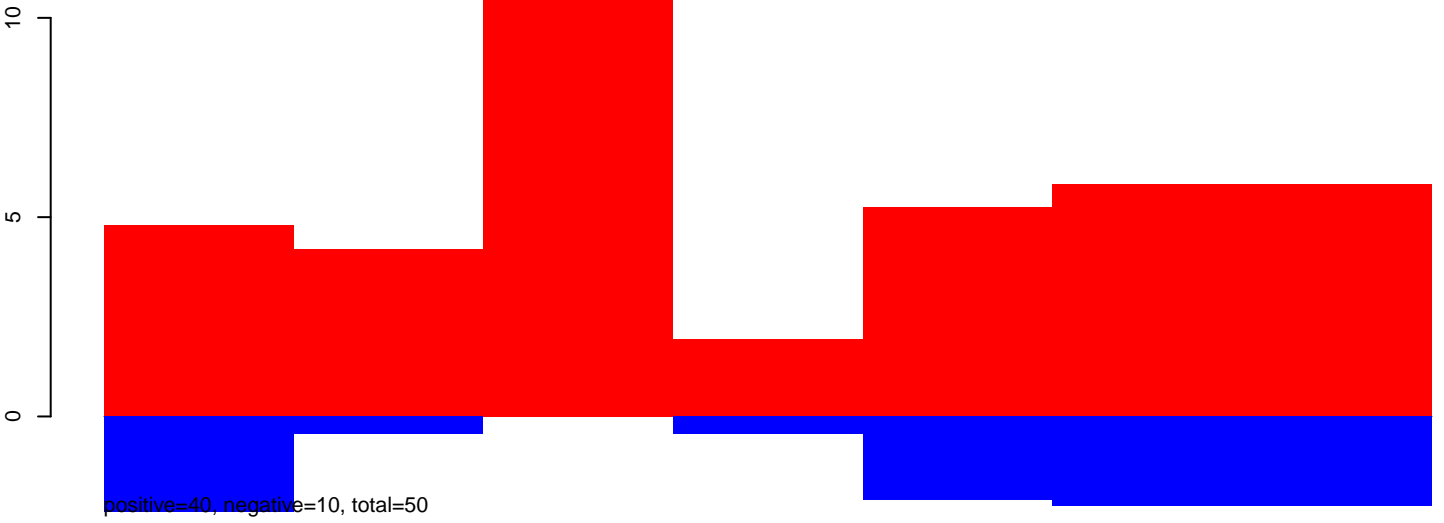
CuQuin_Hsu_30dpi_WNV1.24_35.rep
