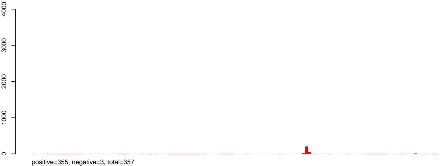
CuQuin_Hsu_30dpi_WNV1.rep
