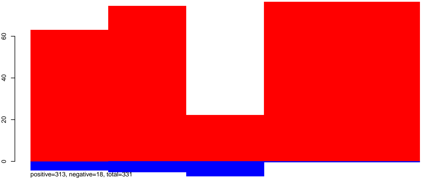
CuQuin_Hsu_30dpi_WNV1.24_35.rep
