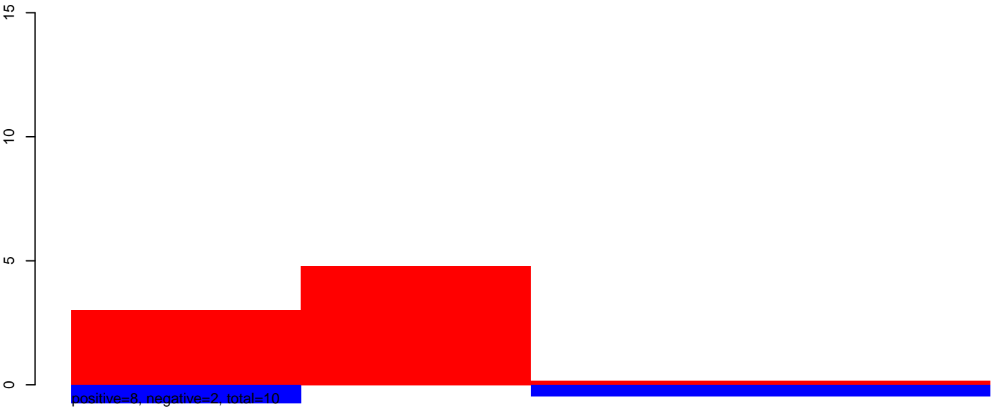
CuQuin_Hsu_30dpi_WNV1.24_35.rep
