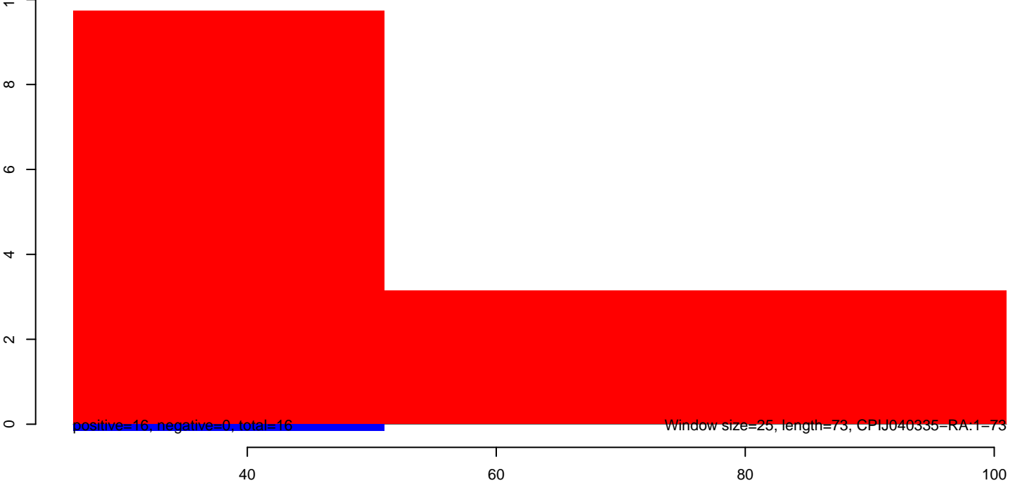
CuQuin_Hsu_30dpi_WNV1.rep
