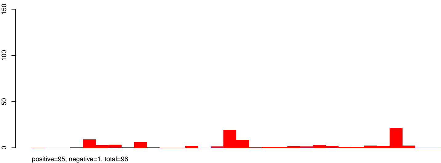
CuQuin_Hsu_30dpi_WNV1.rep
