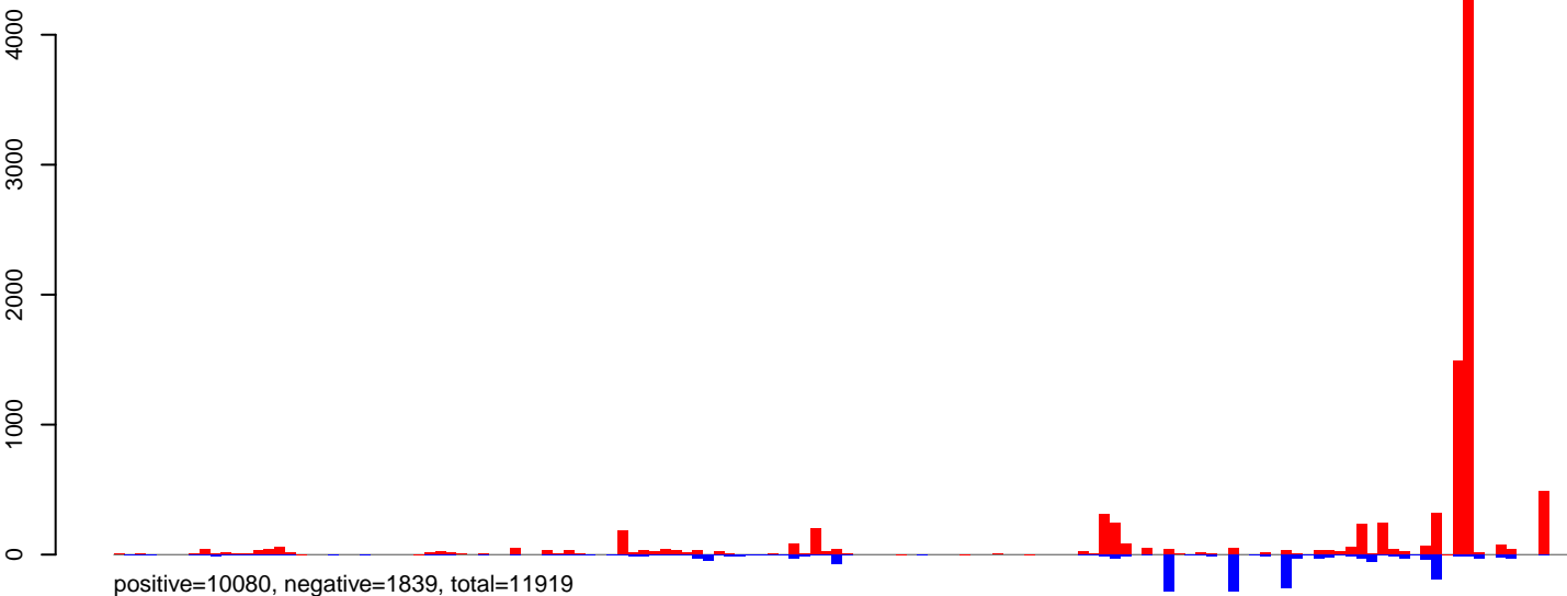
CuQuin_Hsu_30dpi_WNV1.24_35.rep
