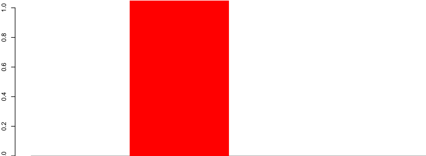
CuQuin_Hsu_30dpi_WNV1.24_35.rep
