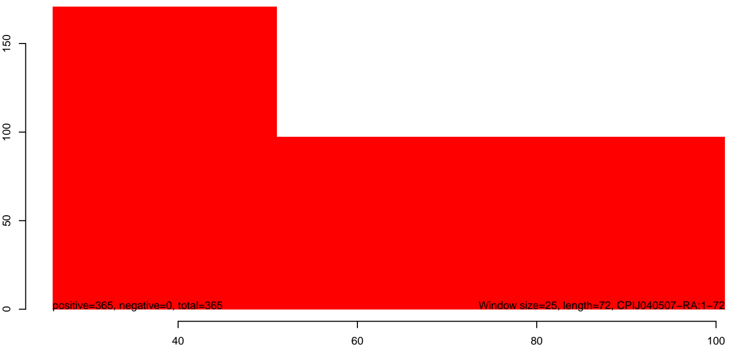
CuQuin_Hsu_30dpi_WNV1.rep
