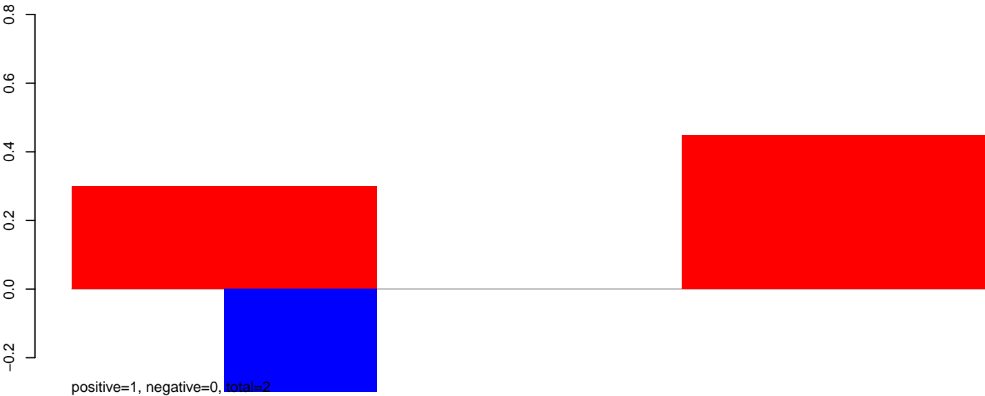
CuQuin_Hsu_30dpi_WNV1.24_35.rep
