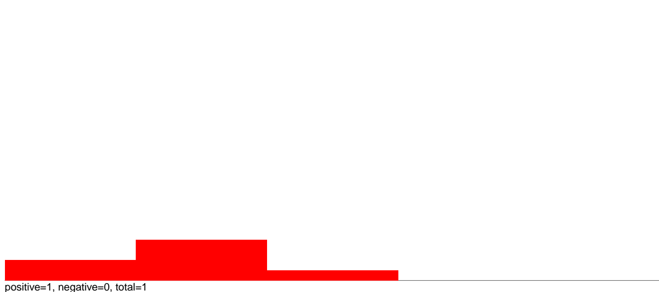
CuQuin_Hsu_30dpi_WNV1.rep
