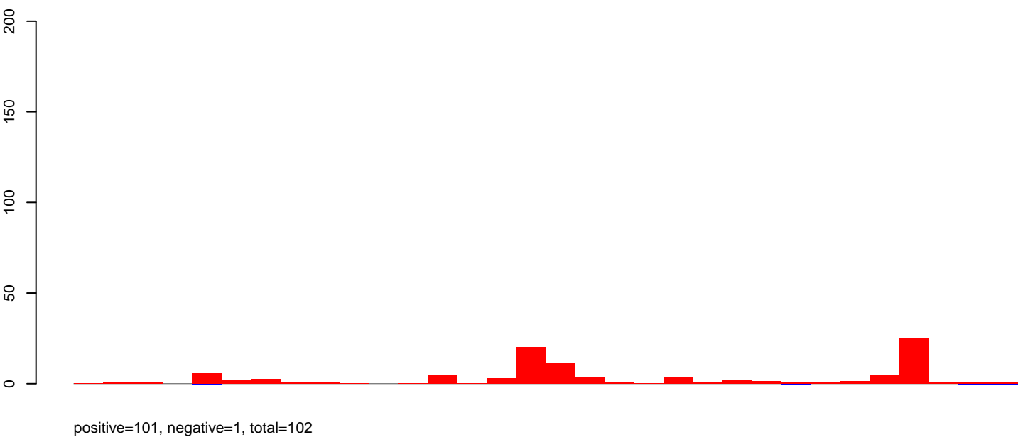
CuQuin_Hsu_6dpi_mock1.rep
