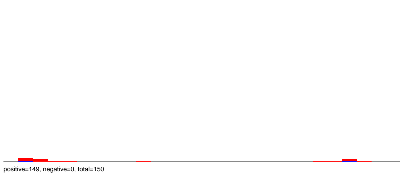
CuQuin_Hsu_6dpi_mock1.rep
