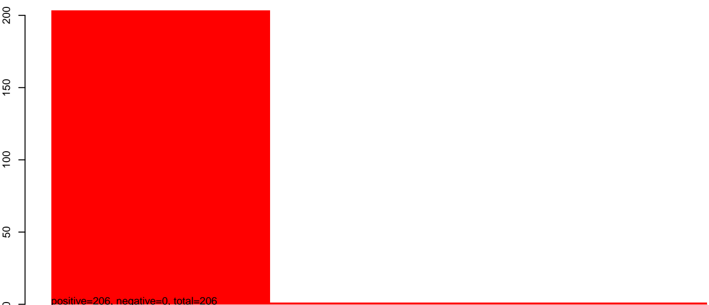
CuQuin_Hsu_6dpi_mock1.rep
