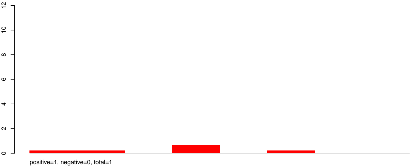
CuQuin_Hsu_6dpi_mock1.rep
