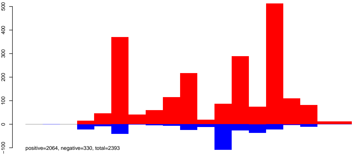
CuQuin_Hsu_6dpi_mock1.24_35.rep
