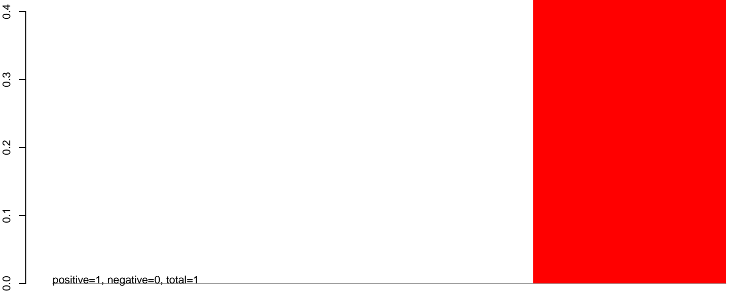
CuQuin_Hsu_6dpi_mock1.24_35.rep
