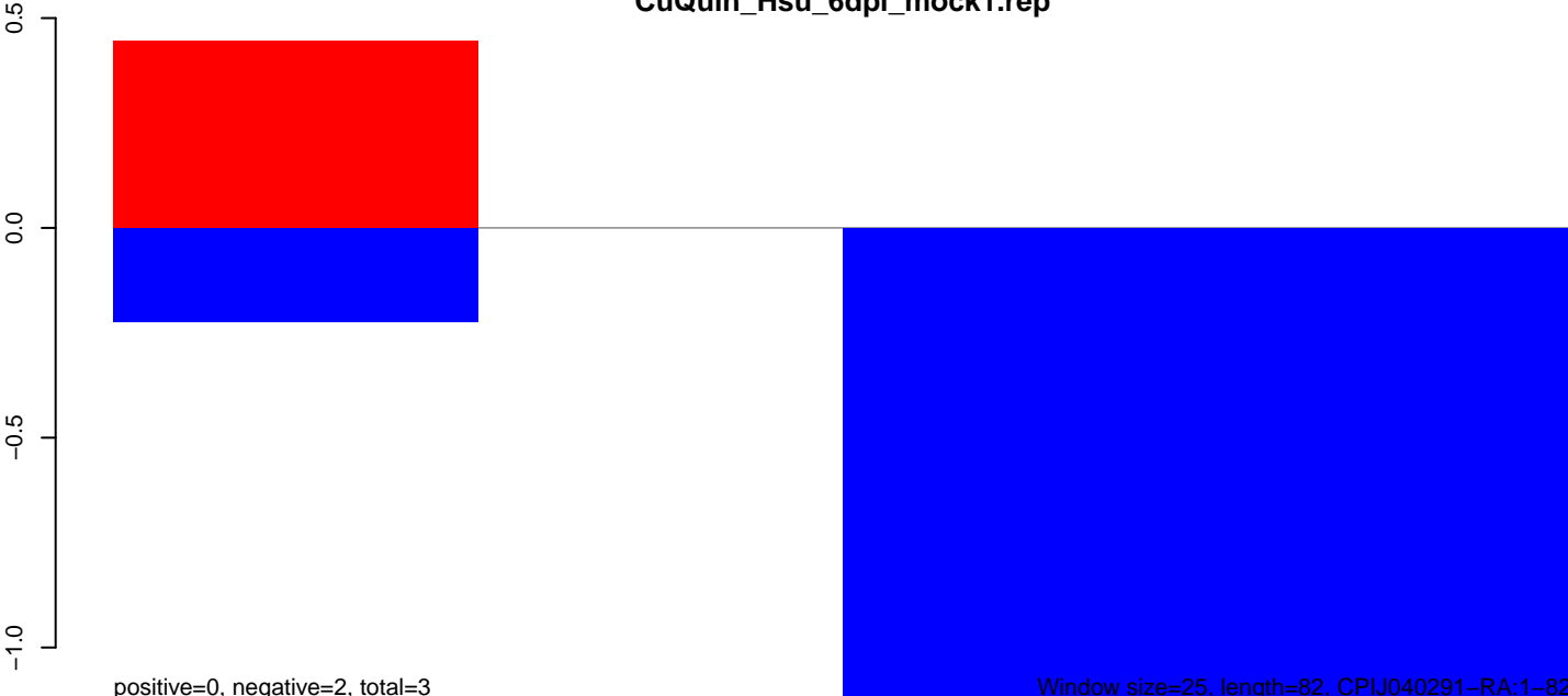
CuQuin_Hsu_6dpi_mock1.rep
