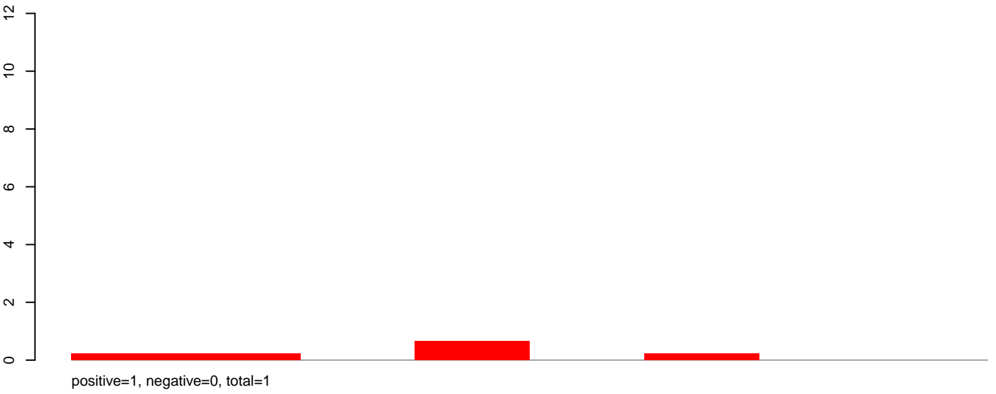
CuQuin_Hsu_6dpi_mock1.rep
