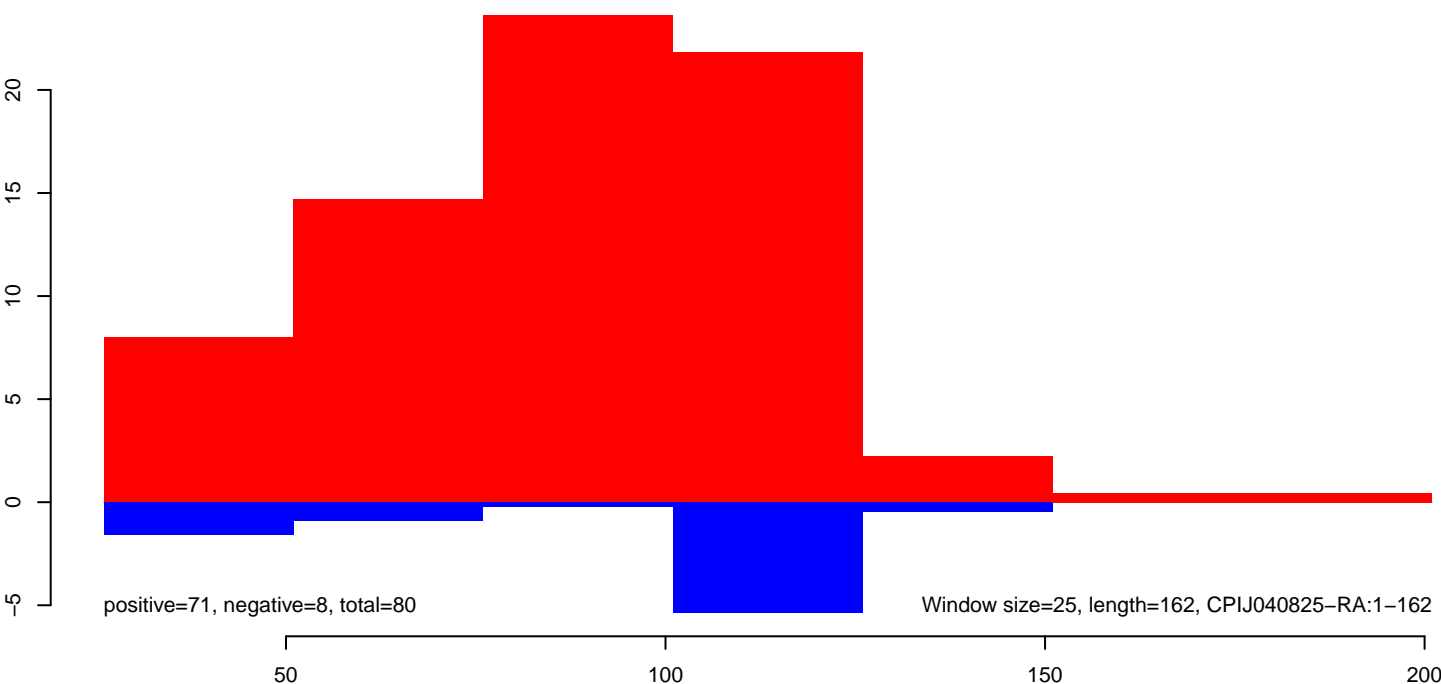
CuQuin_Hsu_6dpi_mock1.rep
