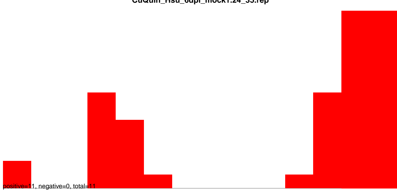
CuQuin_Hsu_6dpi_mock1.rep
