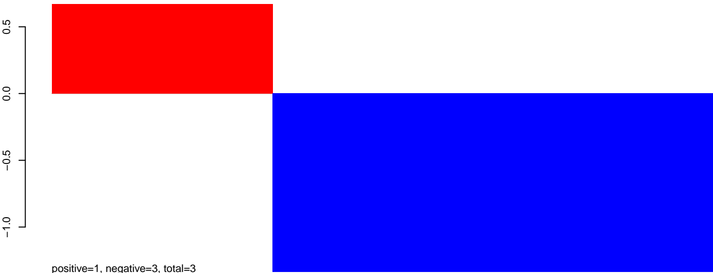
CuQuin_Hsu_6dpi_mock1.24_35.rep
