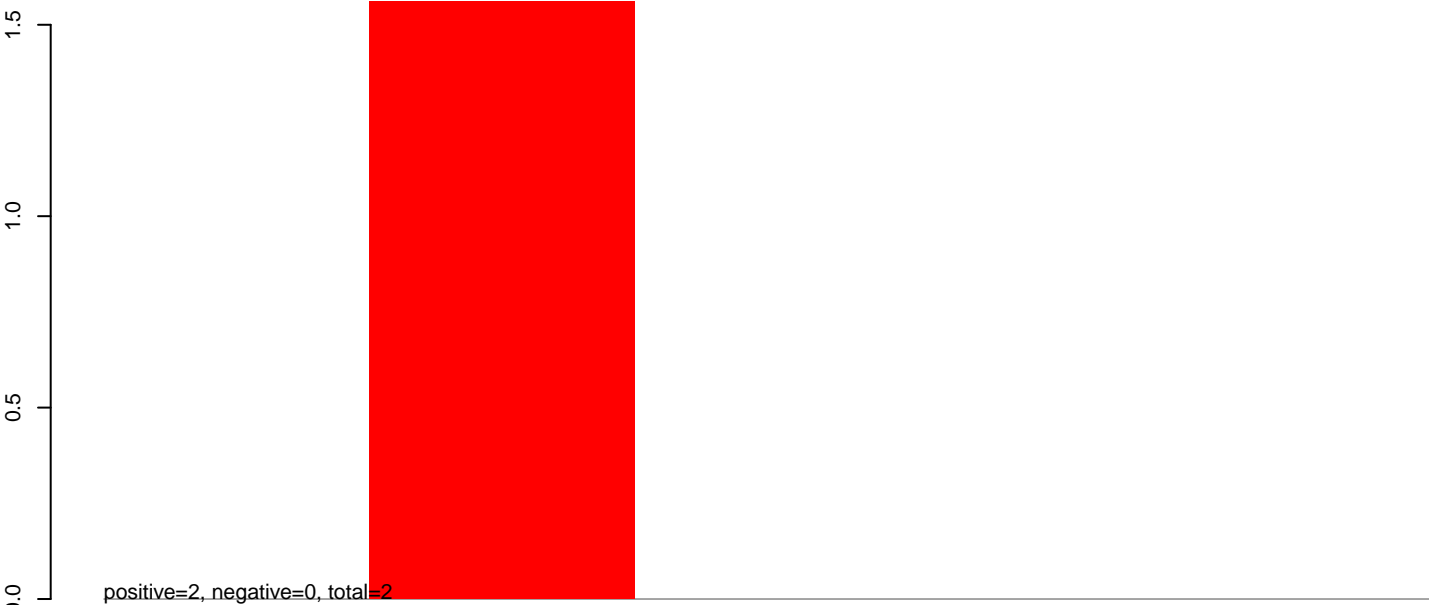
CuQuin_Hsu_6dpi_mock1.24_35.rep
