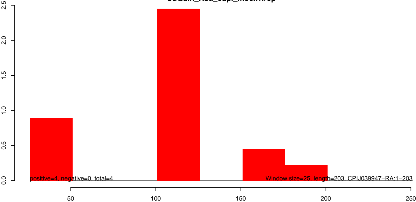
CuQuin_Hsu_6dpi_mock1.rep
