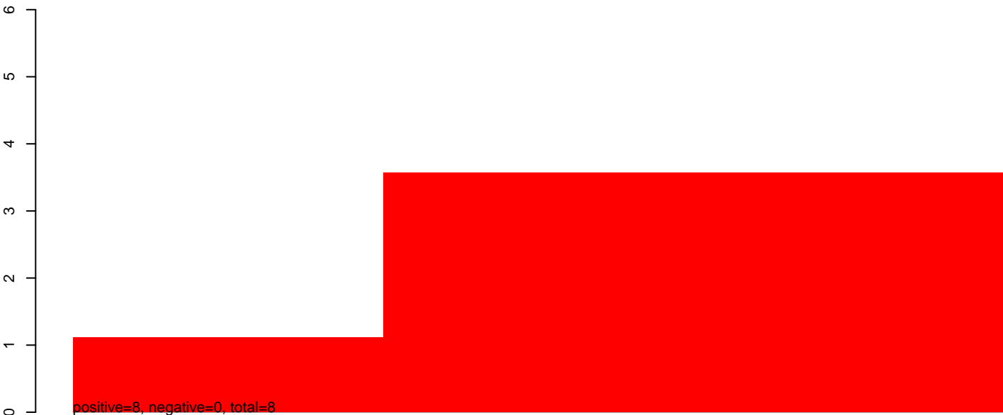
CuQuin_Hsu_6dpi_mock1.24_35.rep
