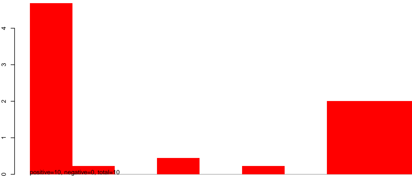
CuQuin_Hsu_6dpi_mock1.24_35.rep
