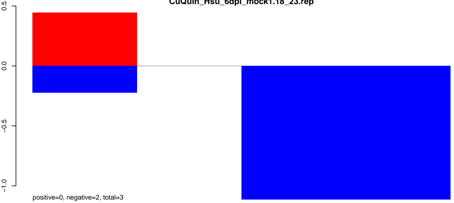
CuQuin_Hsu_6dpi_mock1.24_35.rep
