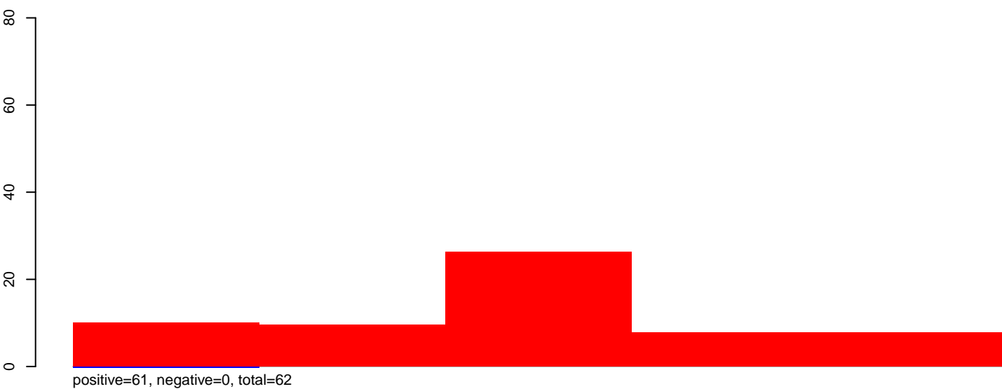
CuQuin_Hsu_6dpi_mock1.rep
