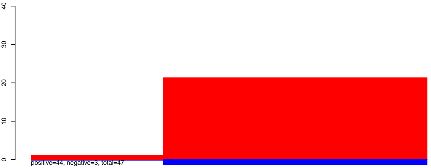
CuQuin_Hsu_6dpi_mock1.24_35.rep
