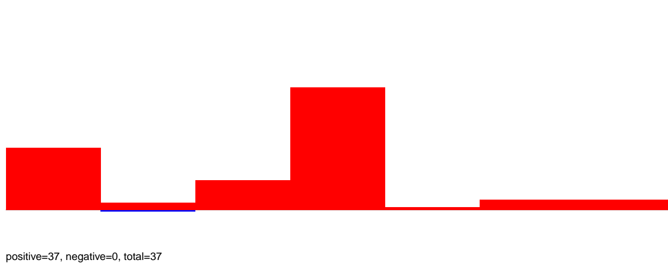
CuQuin_Hsu_6dpi_mock1.rep
