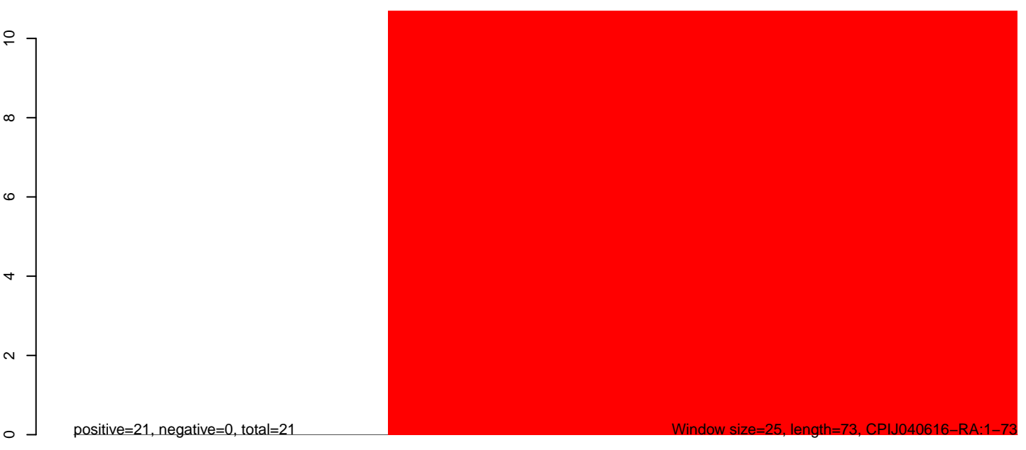
CuQuin_Hsu_6dpi_mock1.rep
