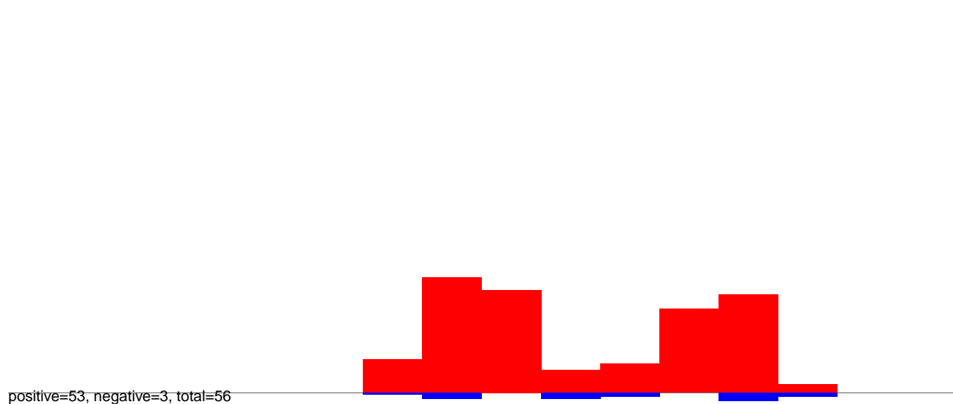
CuQuin_Hsu_6dpi_mock1.24_35.rep
