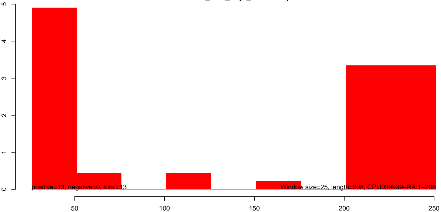
CuQuin_Hsu_6dpi_mock1.rep
