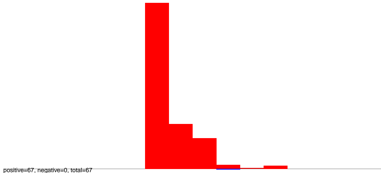
CuQuin_Hsu_6dpi_mock1.rep
