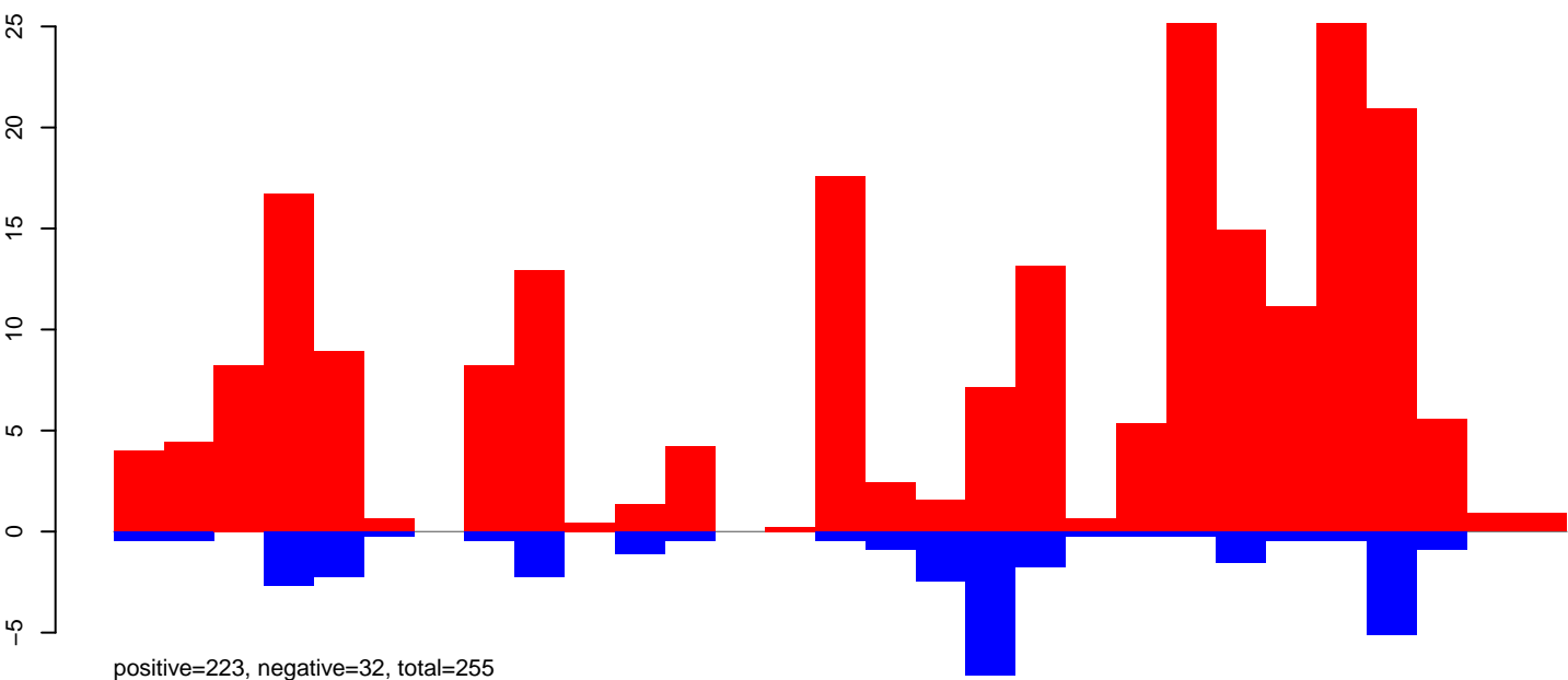
CuQuin_Hsu_6dpi_mock1.24_35.rep
