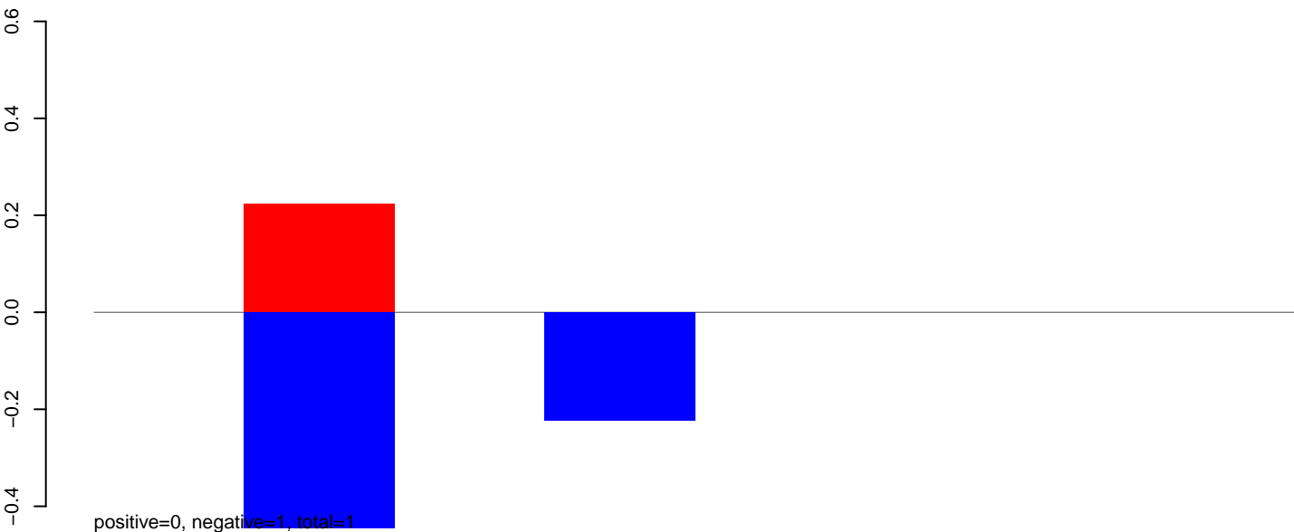
CuQuin_Hsu_6dpi_mock1.24_35.rep
