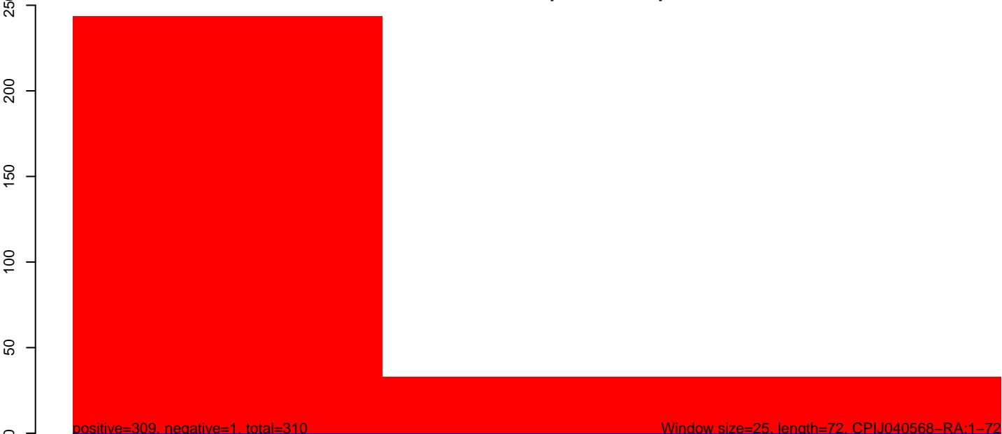
CuQuin_Hsu_6dpi_mock1.rep
