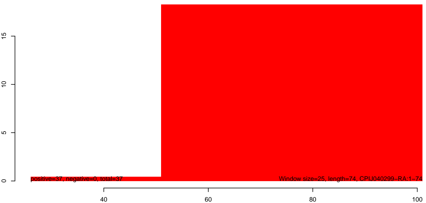
CuQuin_Hsu_6dpi_mock1.rep
