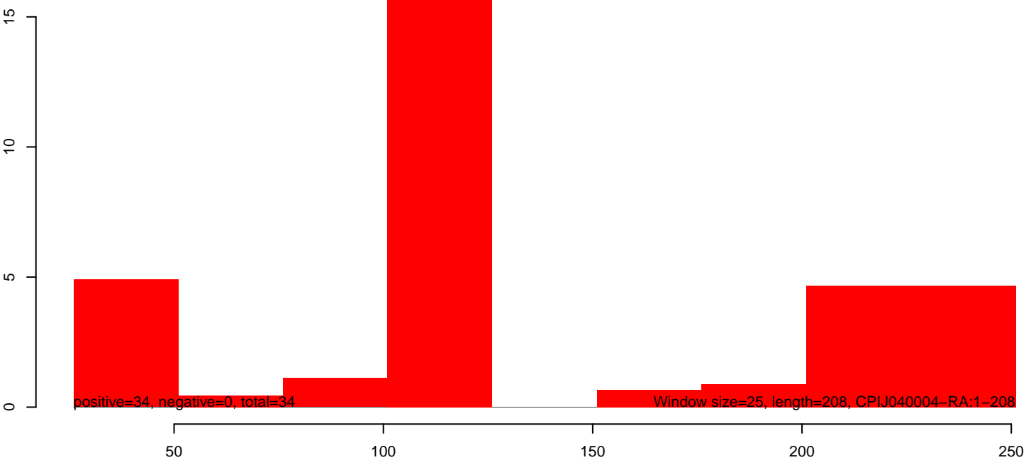
CuQuin_Hsu_6dpi_mock1.rep
