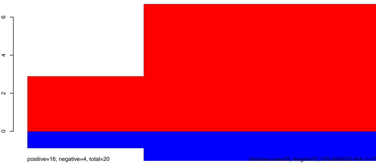
CuQuin_Hsu_6dpi_mock1.rep
