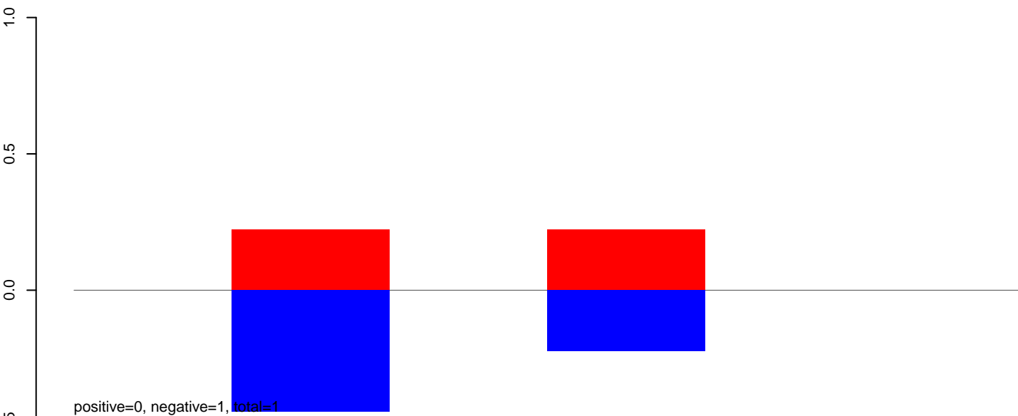
CuQuin_Hsu_6dpi_mock1.24_35.rep
