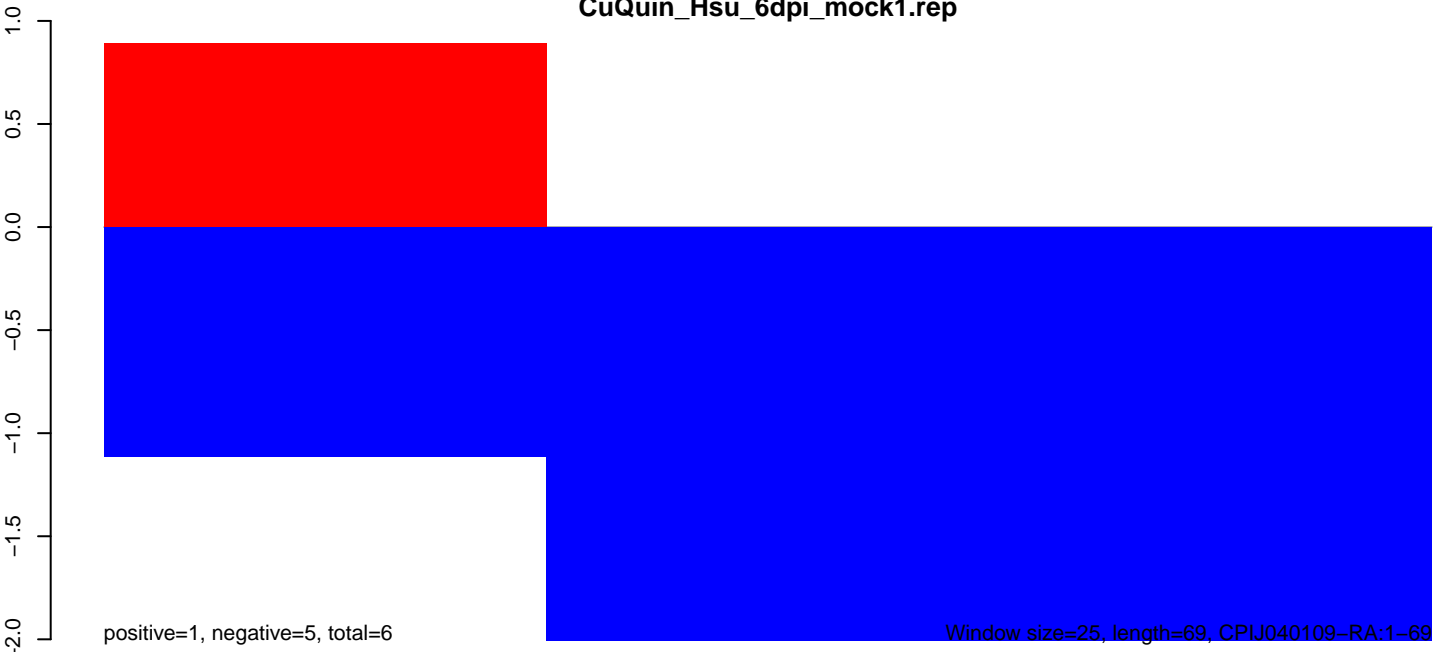
CuQuin_Hsu_6dpi_mock1.rep
