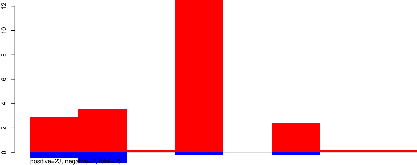
CuQuin_Hsu_6dpi_mock1.24_35.rep
