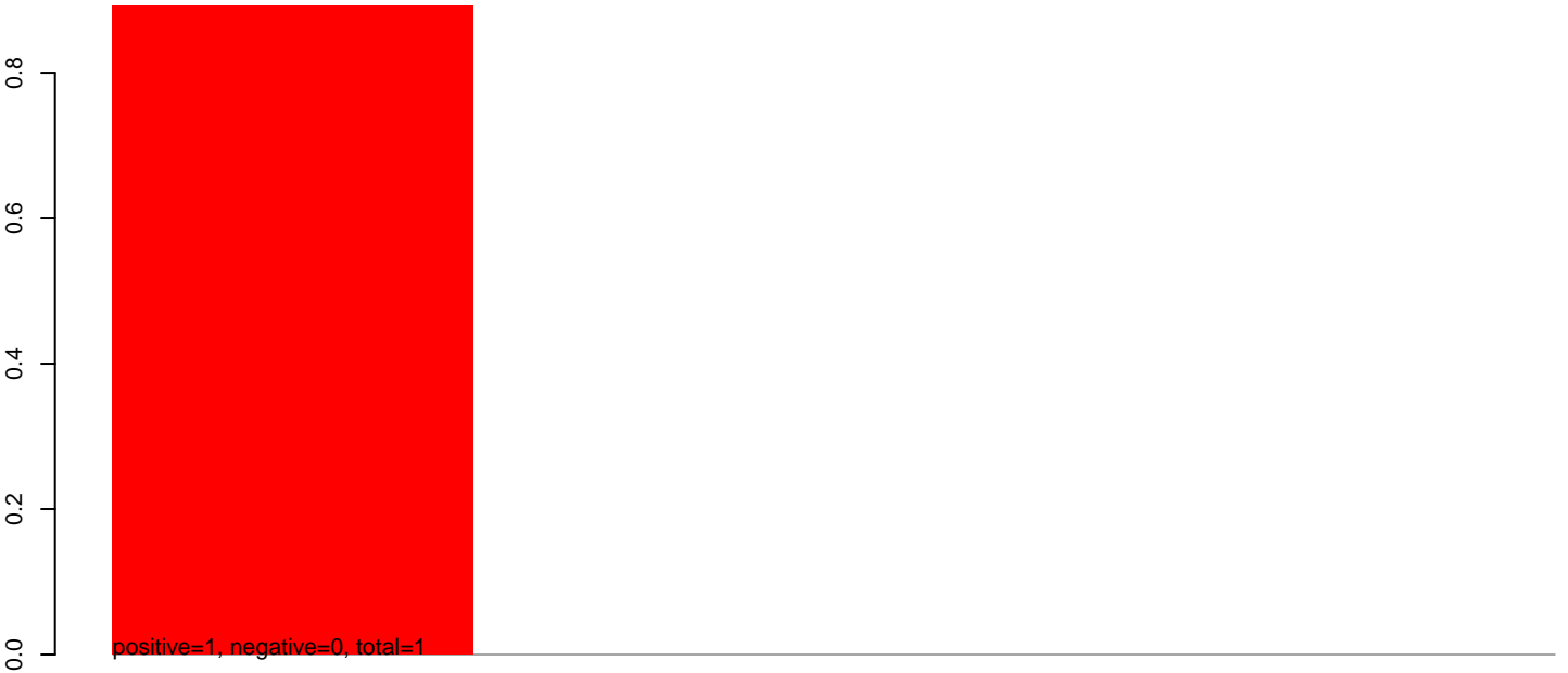
CuQuin_Hsu_6dpi_mock1.24_35.rep
