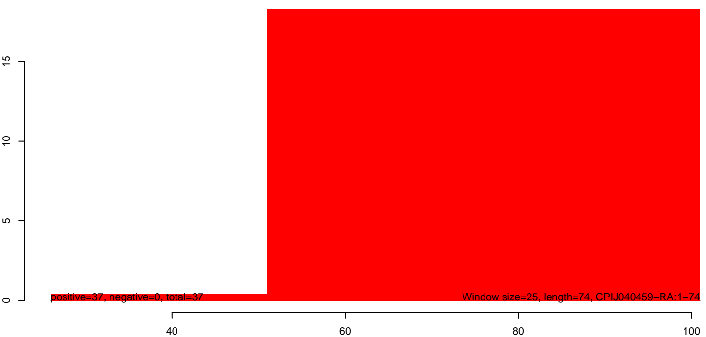
CuQuin_Hsu_6dpi_mock1.rep
