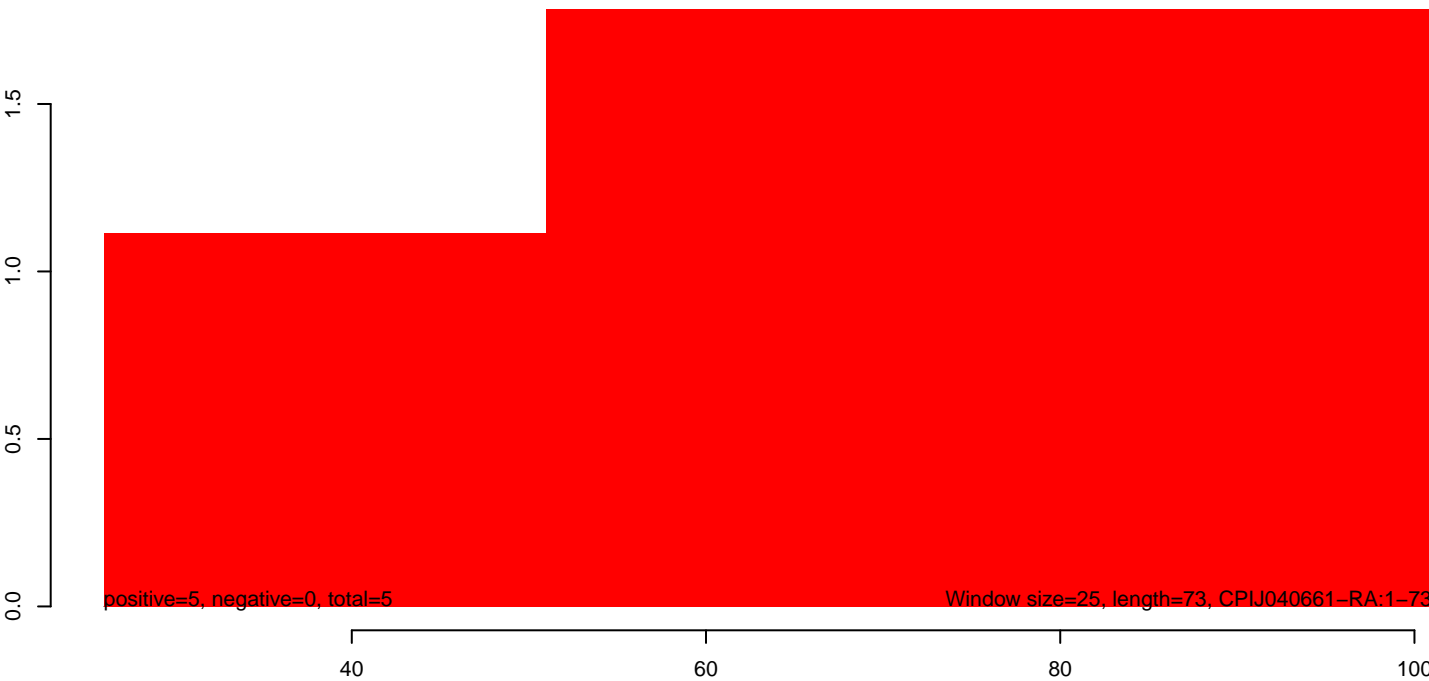
CuQuin_Hsu_6dpi_mock1.rep
