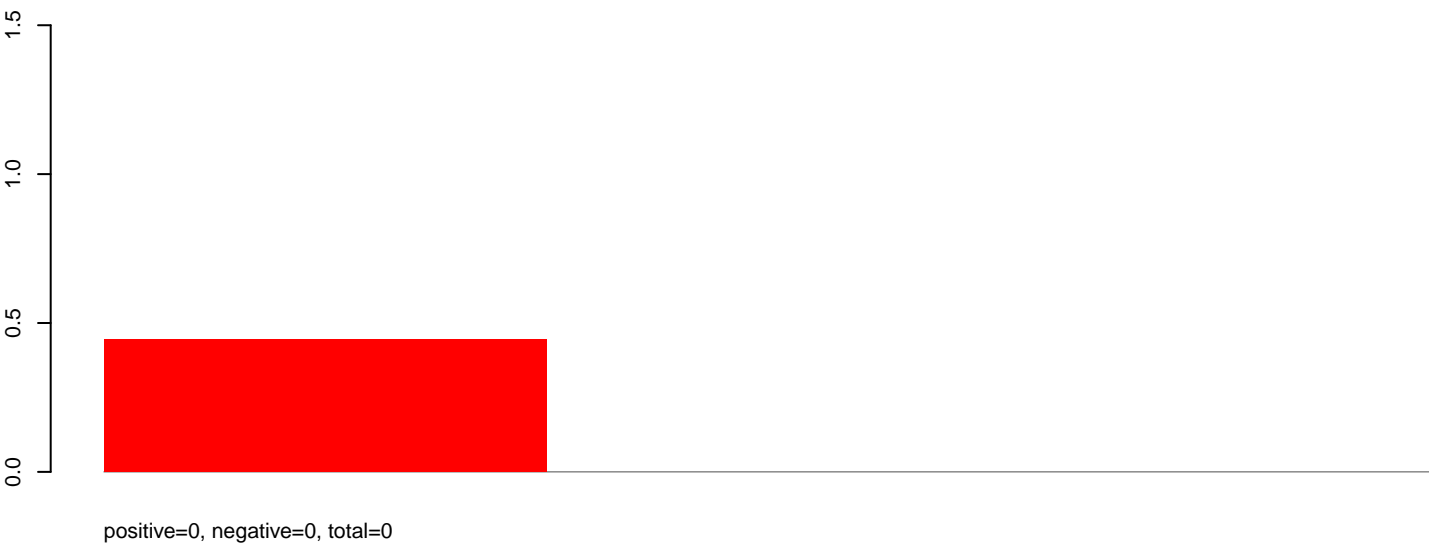
CuQuin_Hsu_6dpi_mock1.rep
