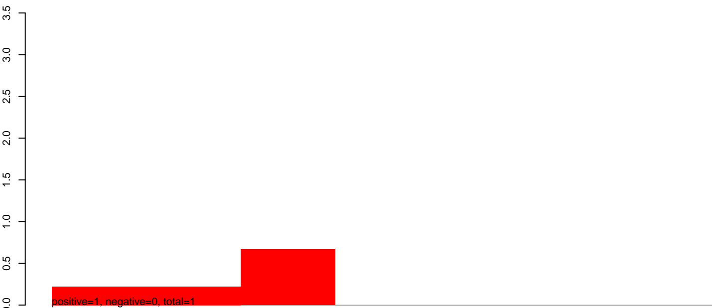
CuQuin_Hsu_6dpi_mock1.rep
