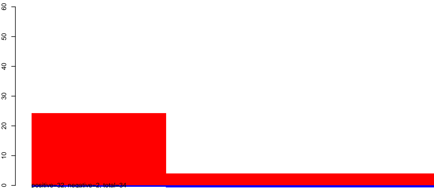
CuQuin_Hsu_6dpi_mock1.24_35.rep
