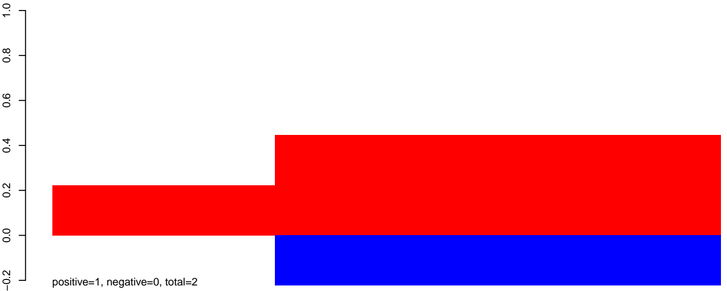
CuQuin_Hsu_6dpi_mock1.24_35.rep
