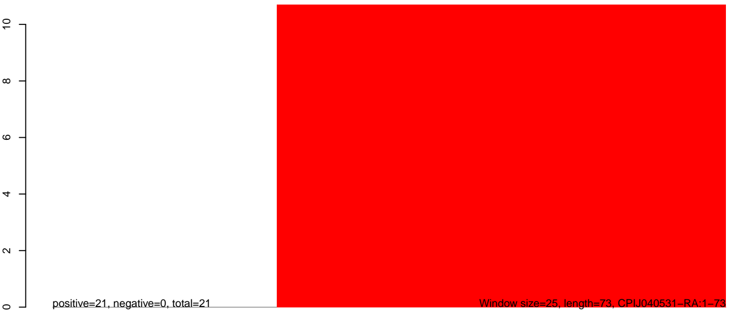
CuQuin_Hsu_6dpi_mock1.rep
