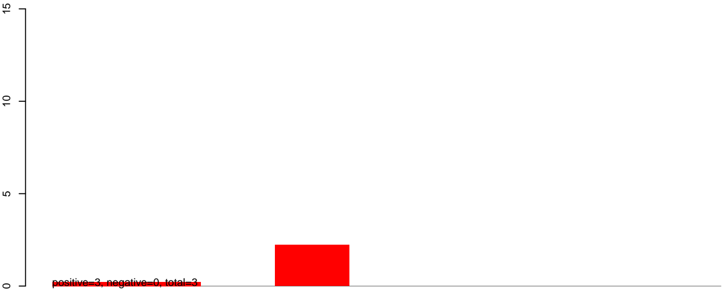
CuQuin_Hsu_6dpi_mock1.rep
