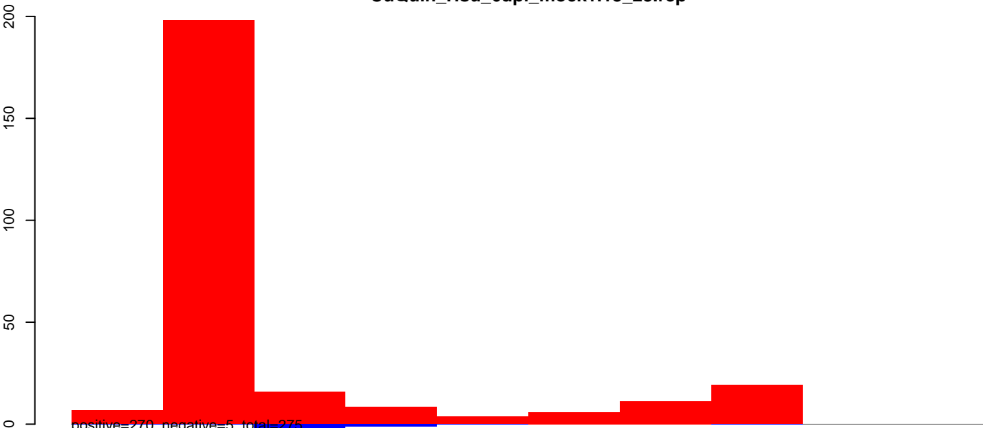
CuQuin_Hsu_6dpi_mock1.24_35.rep
