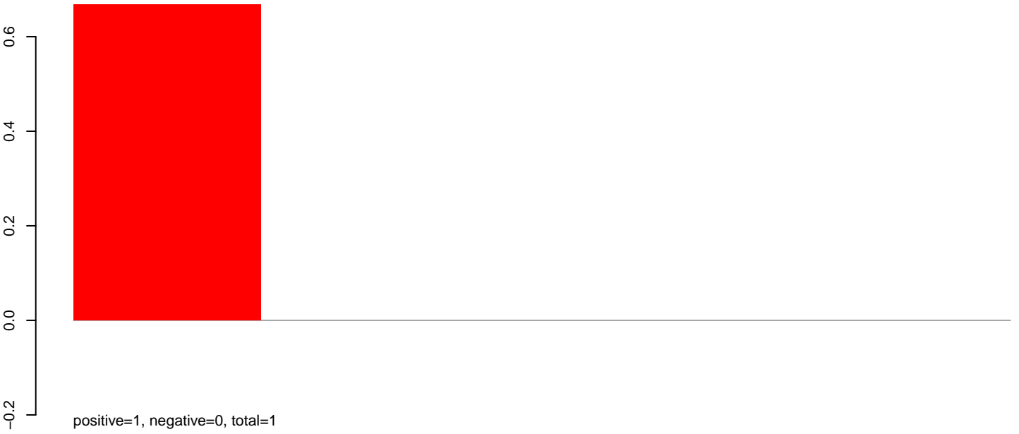
CuQuin_Hsu_6dpi_mock1.rep
