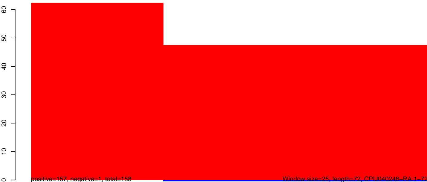
CuQuin_Hsu_6dpi_mock1.rep
