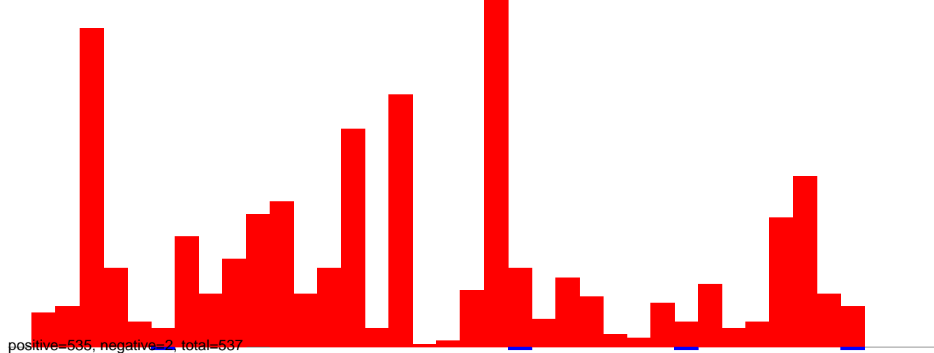
CuQuin_MG_7dpi2.24_35.rep
