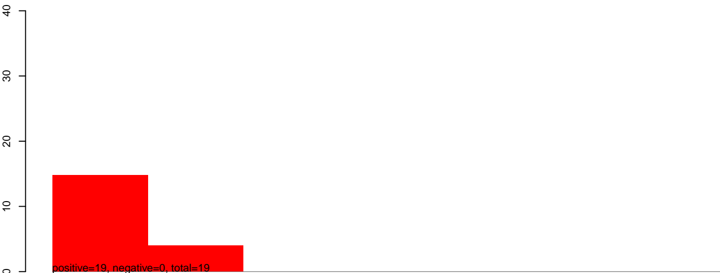
CuQuin_MG_7dpi2.rep
