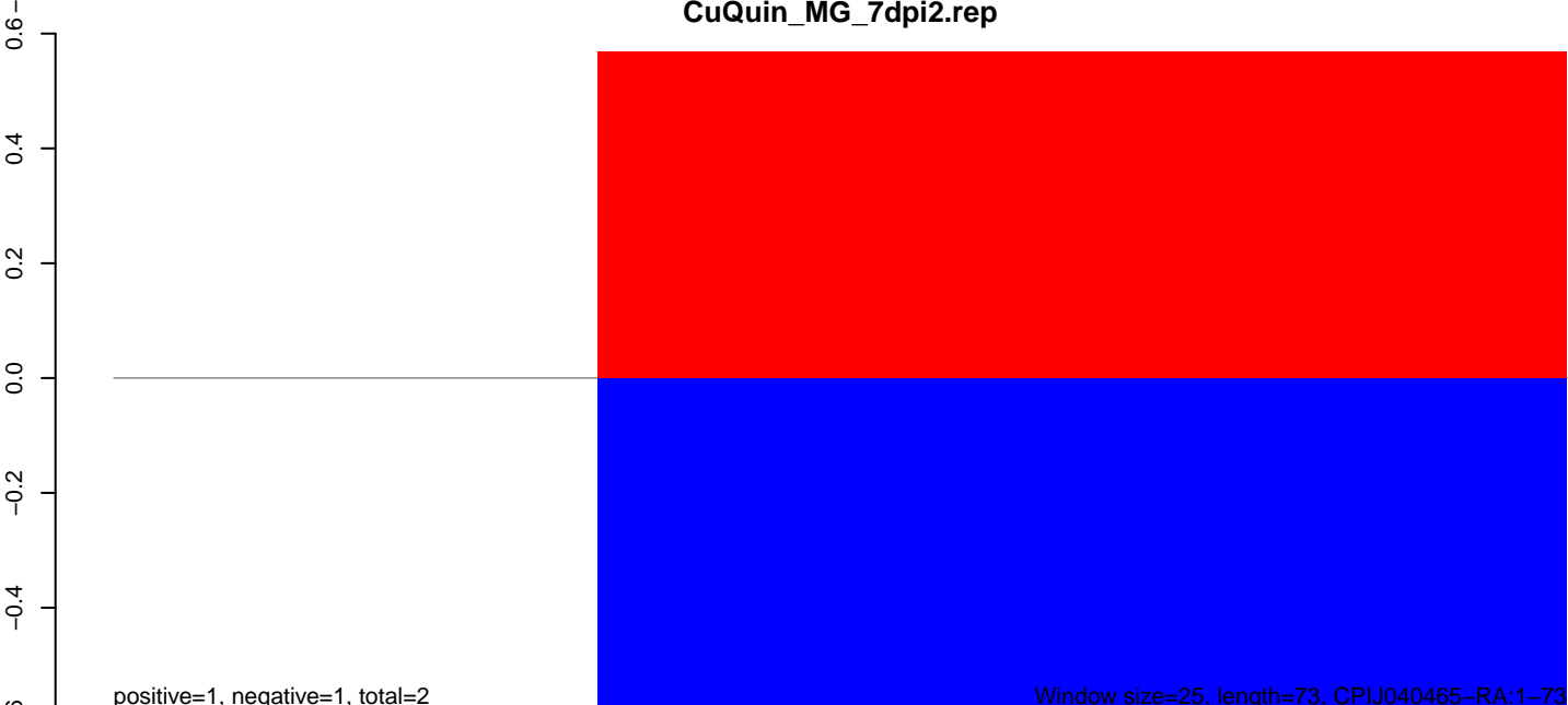
CuQuin_MG_7dpi2.rep
