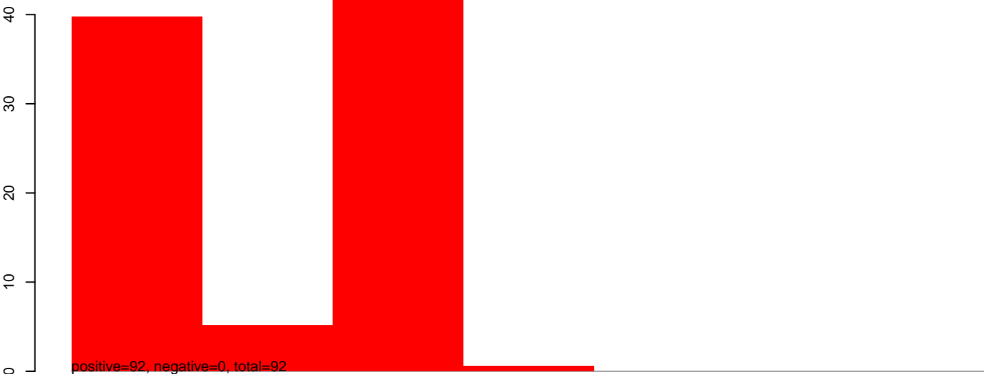
CuQuin_MG_7dpi2.24_35.rep
