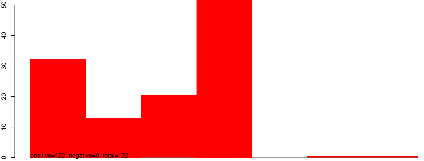
CuQuin_MG_7dpi2.rep
