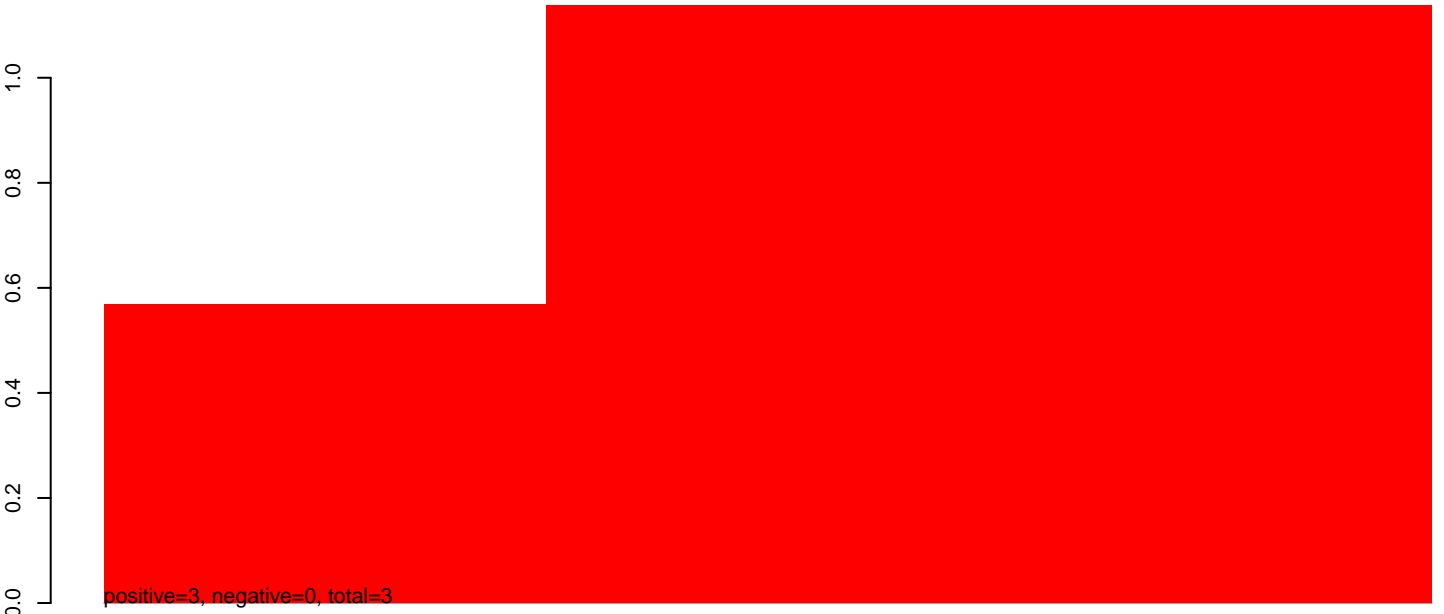
CuQuin_MG_7dpi2.24_35.rep
