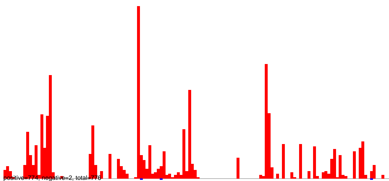
CuQuin_MG_7dpi2.24_35.rep
