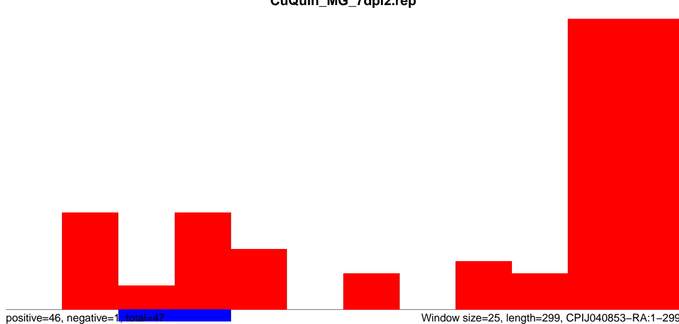
CuQuin_MG_7dpi2.rep
