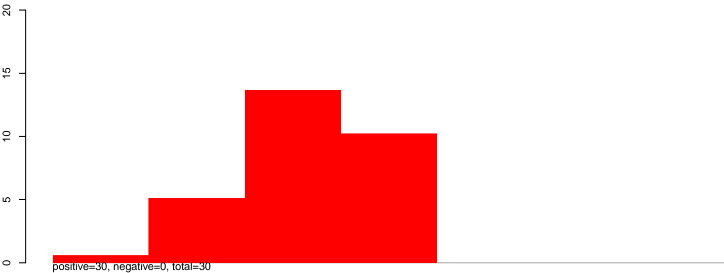
CuQuin_MG_7dpi2.rep
