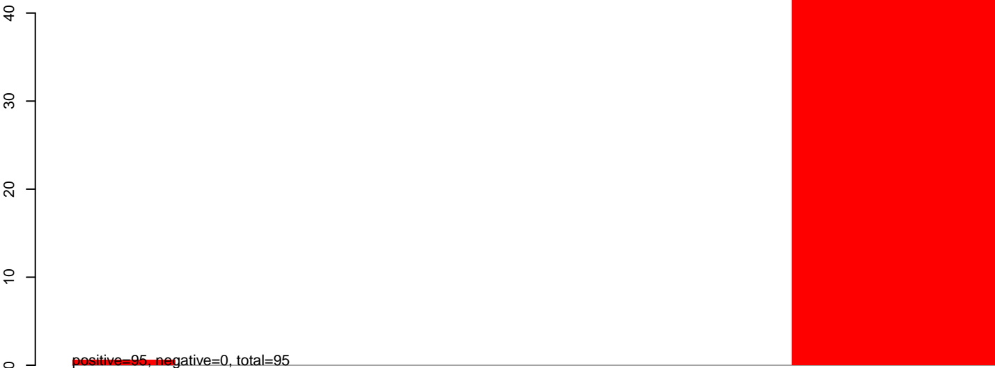
CuQuin_MG_7dpi2.24_35.rep
