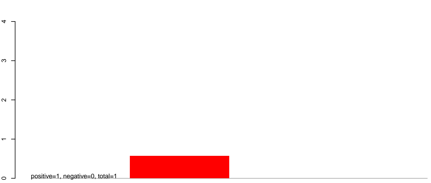
CuQuin_MG_7dpi2.rep
