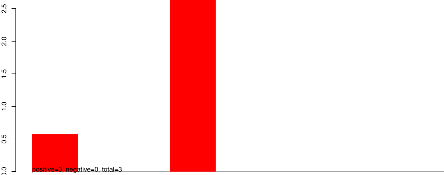
CuQuin_MG_7dpi2.24_35.rep
