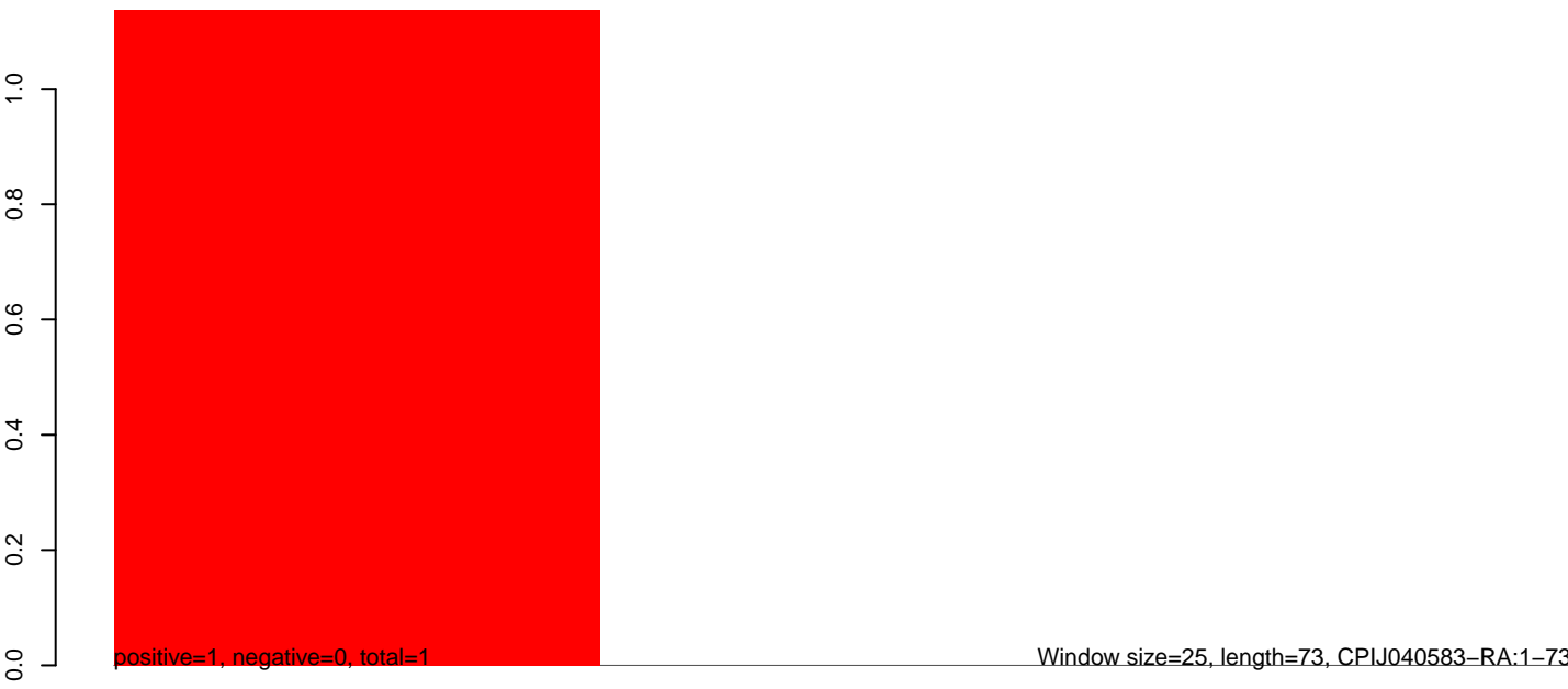
CuQuin_MG_7dpi2.rep
