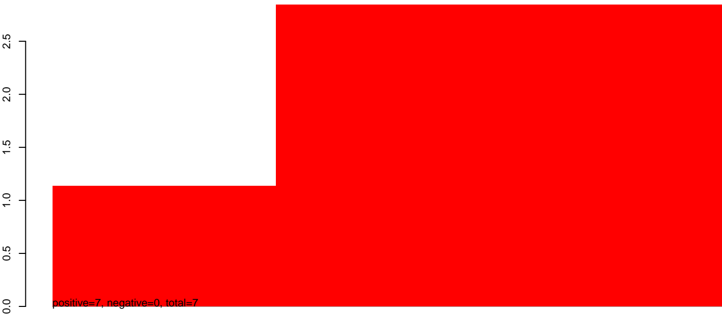
CuQuin_MG_7dpi2.24_35.rep
