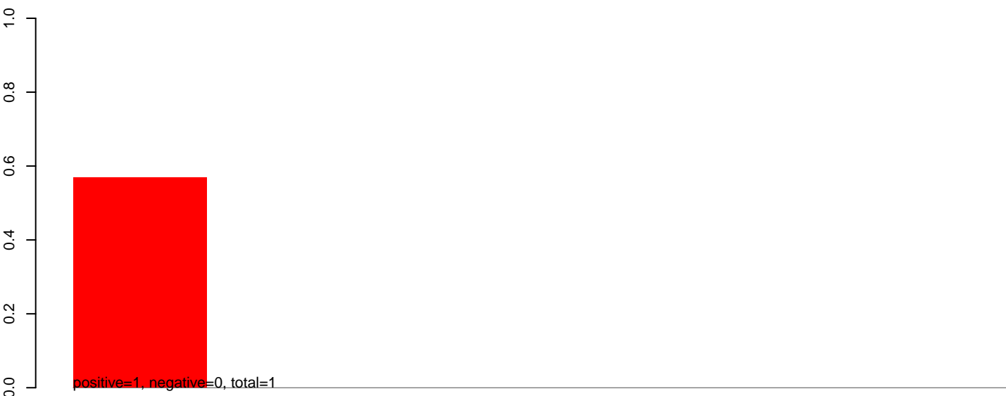
CuQuin_MG_7dpi2.rep
