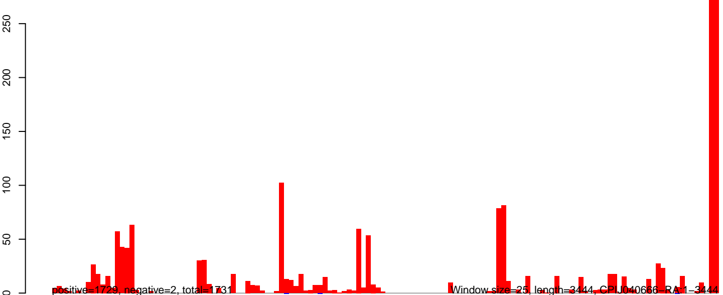
CuQuin_MG_7dpi2.rep
