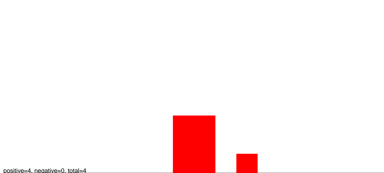
CuQuin_MG_7dpi2.rep
