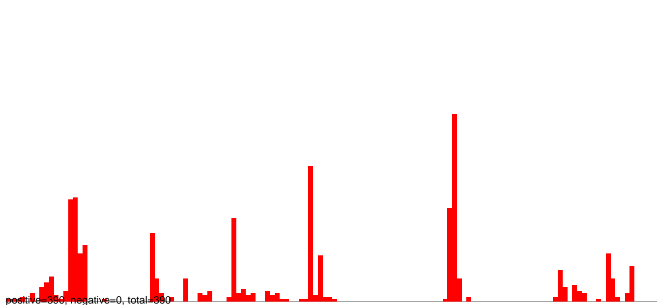
CuQuin_MG_7dpi2.rep
