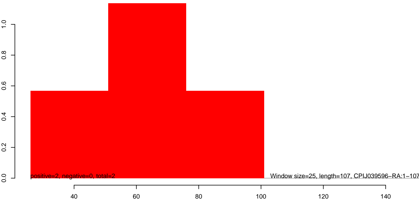
CuQuin_MG_7dpi2.rep
