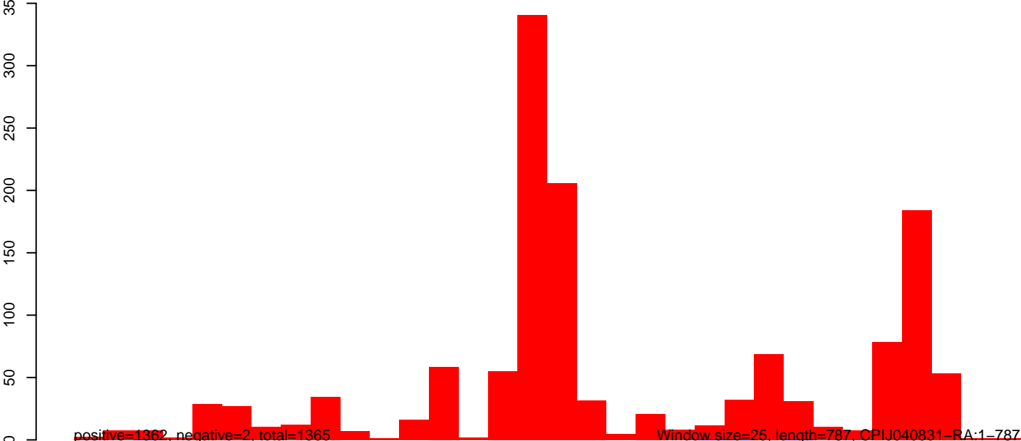
CuQuin_MG_7dpi2.rep
