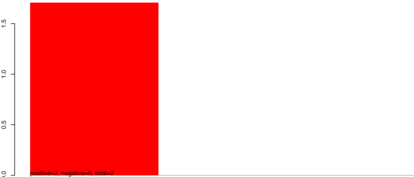
CuQuin_MG_7dpi2.24_35.rep
