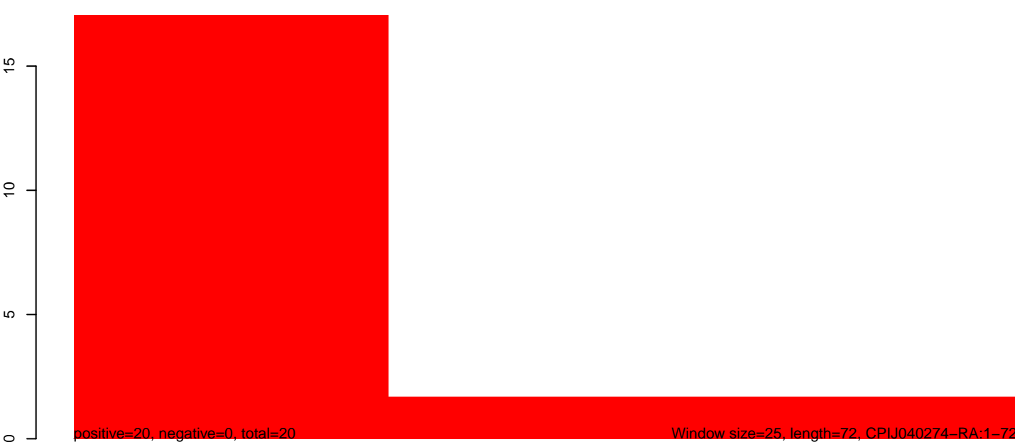
CuQuin_MG_7dpi2.rep
