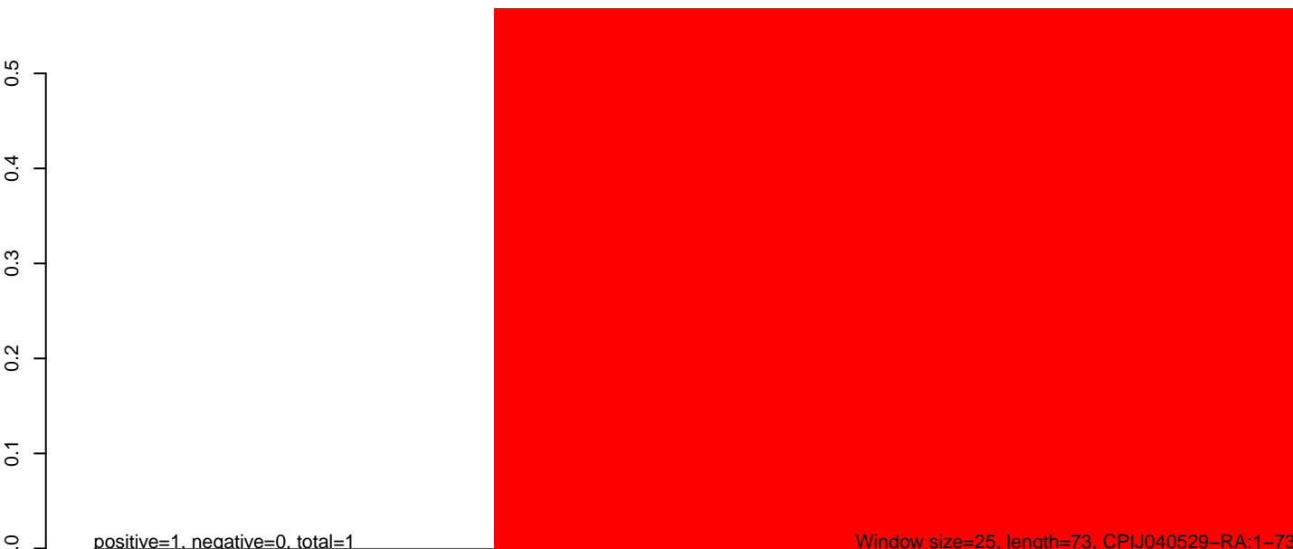
CuQuin_MG_7dpi2.rep
