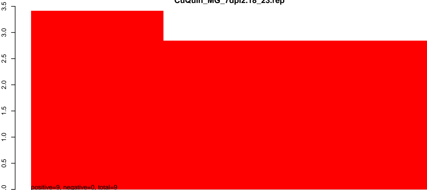
CuQuin_MG_7dpi2.24_35.rep
