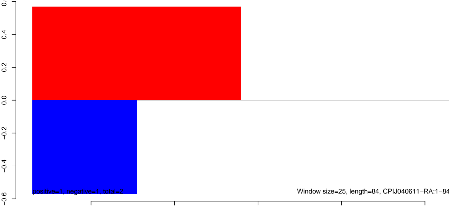
CuQuin_MG_7dpi2.rep
