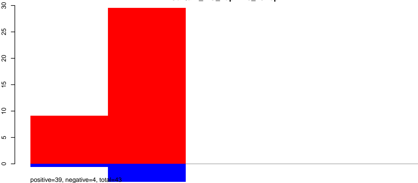
CuQuin_MG_7dpi2.24_35.rep
