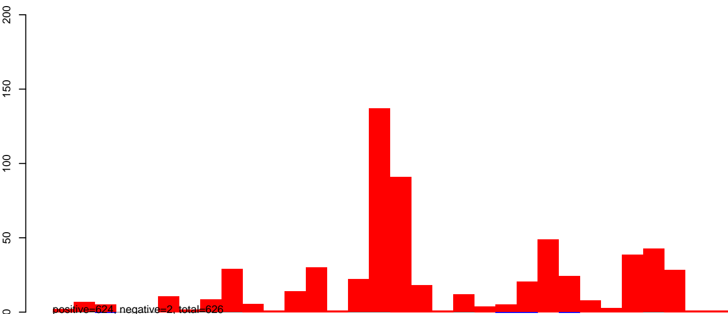
CuQuin_MG_7dpi2.24_35.rep
