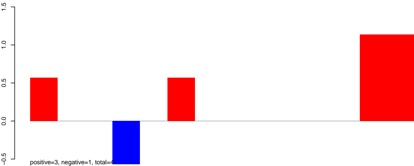
CuQuin_MG_7dpi2.24_35.rep
