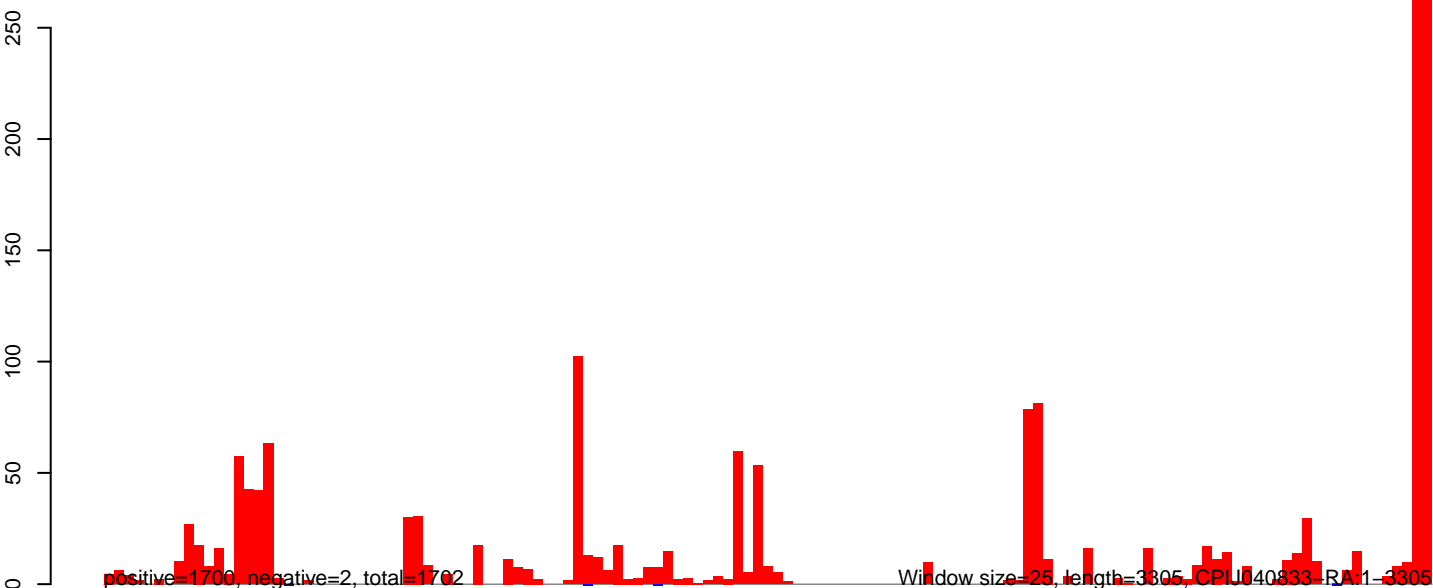
CuQuin_MG_7dpi2.rep
