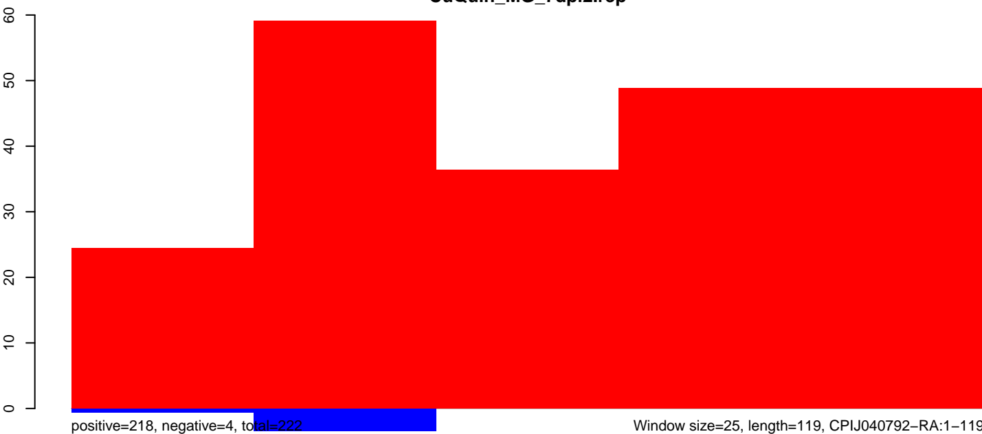
CuQuin_MG_7dpi2.rep
