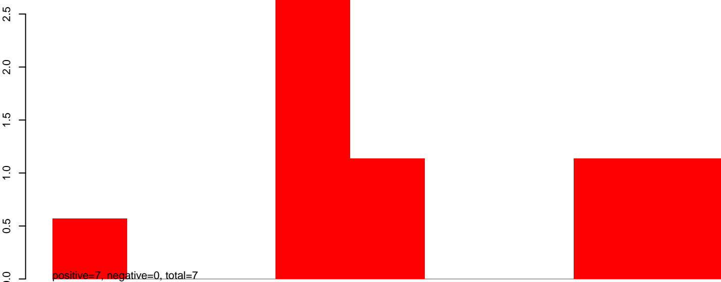
CuQuin_MG_7dpi2.24_35.rep
