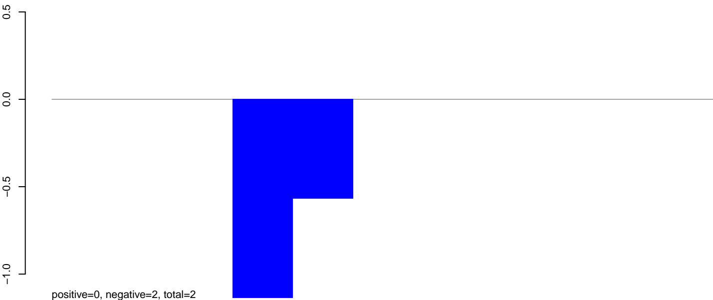
CuQuin_MG_7dpi2.24_35.rep
