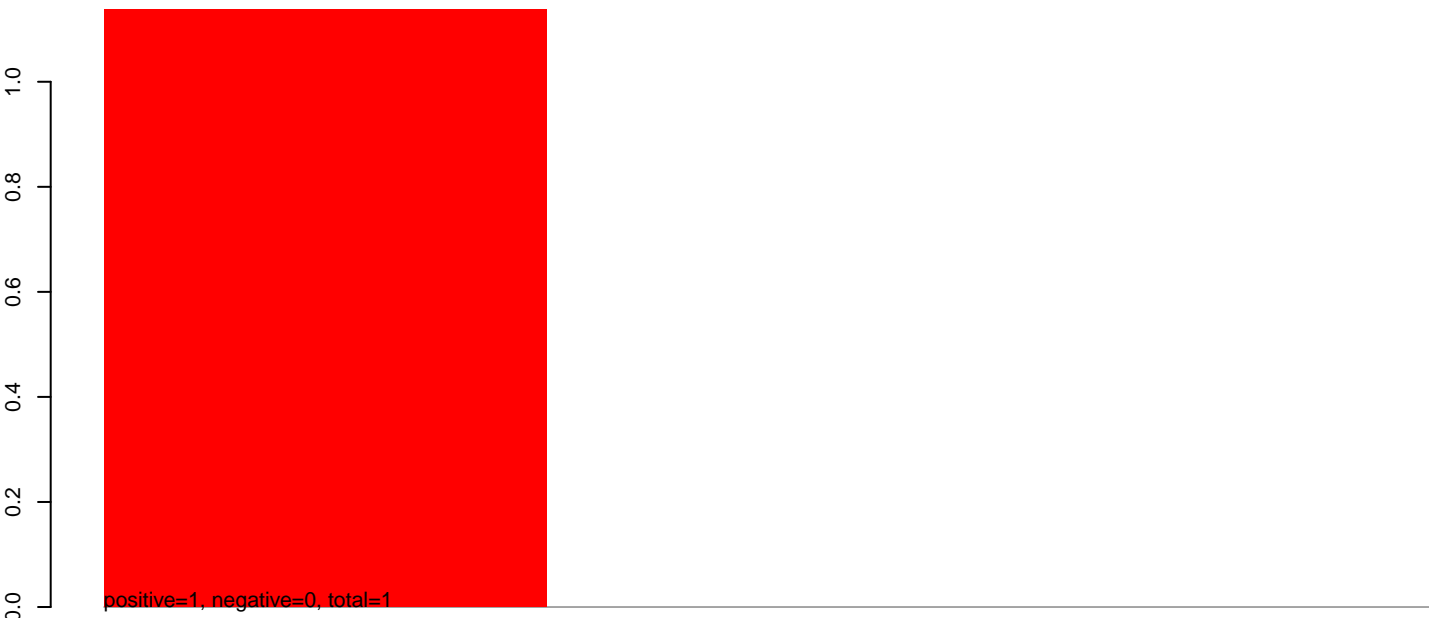
CuQuin_MG_7dpi2.24_35.rep
