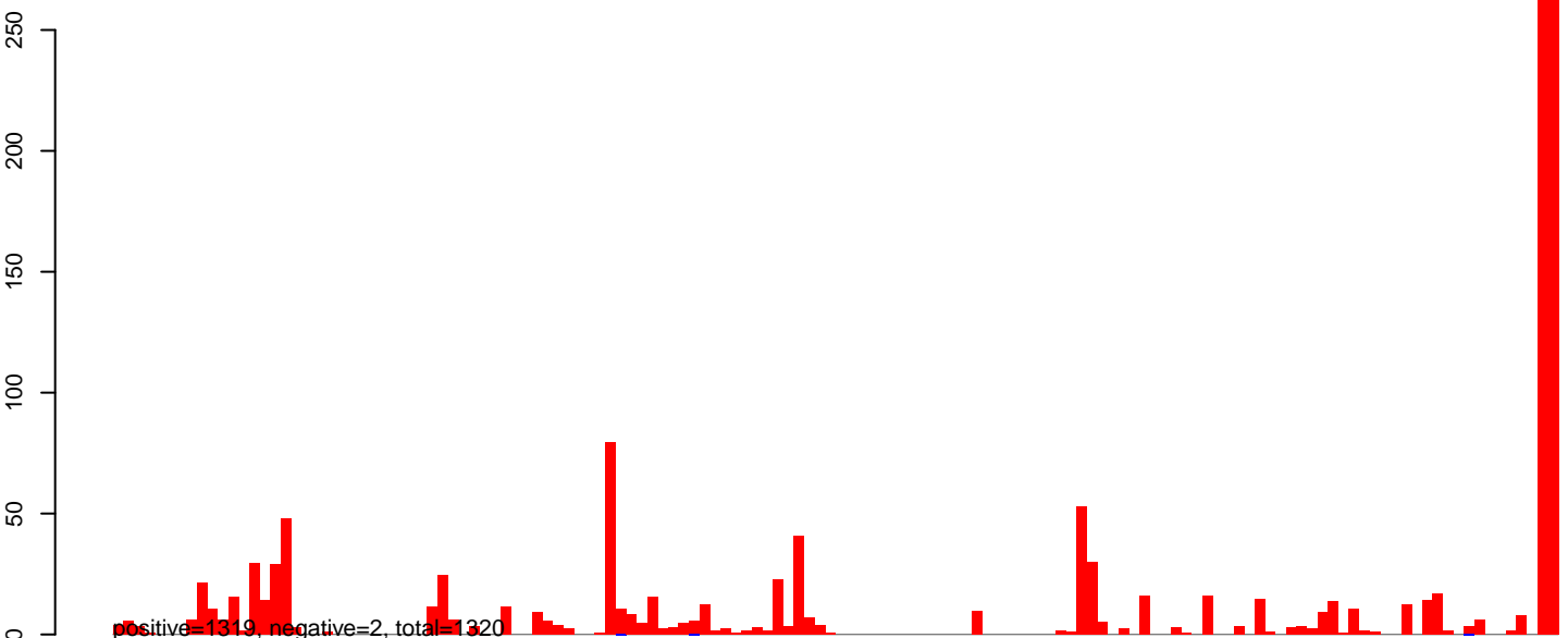
CuQuin_MG_7dpi2.24_35.rep
