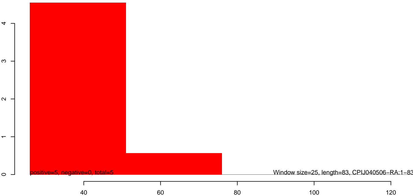
CuQuin_MG_7dpi2.rep
