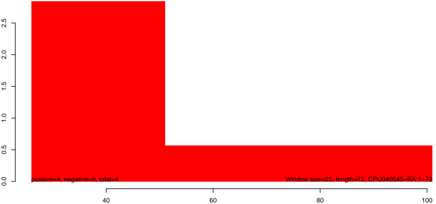
CuQuin_MG_7dpi2.rep
