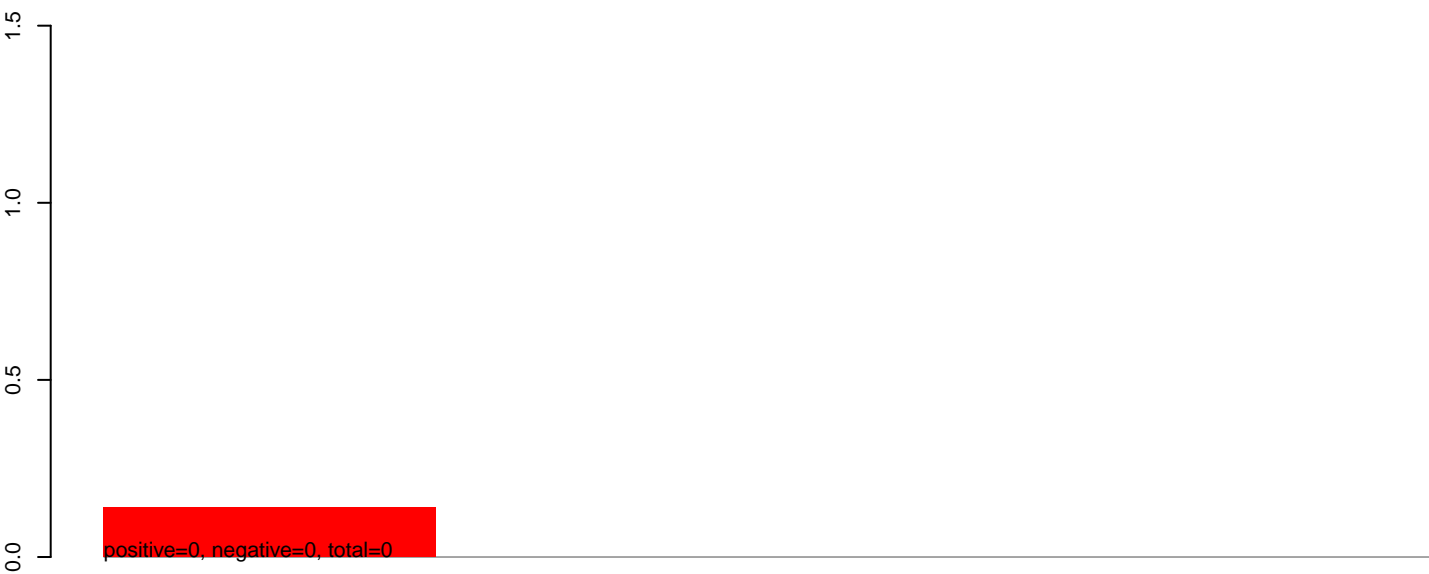
CuQuin_SG_14dpi2.24_35.rep
