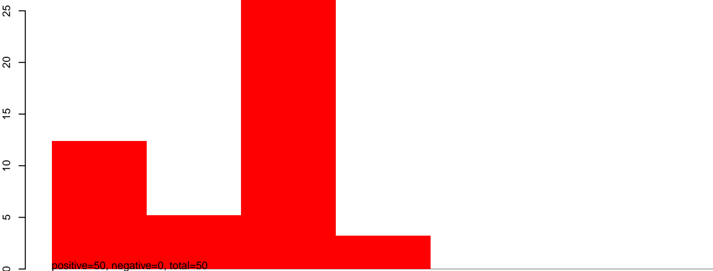
CuQuin_SG_14dpi2.24_35.rep
