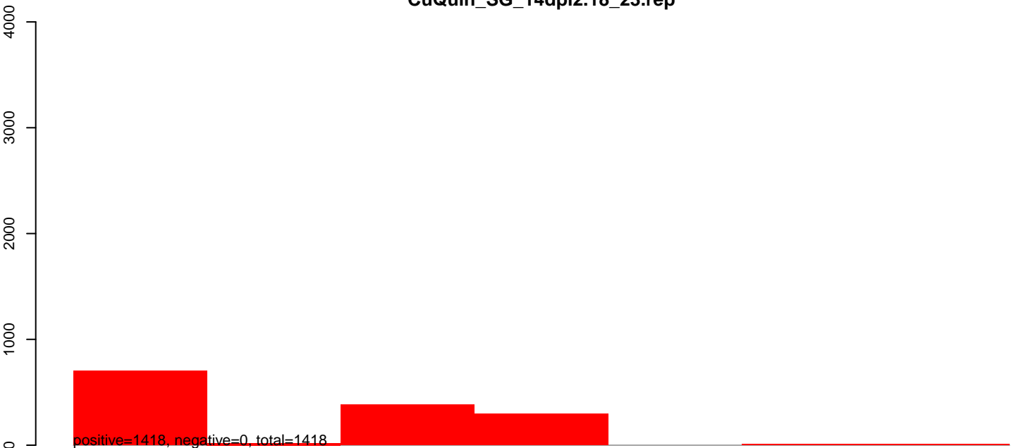
CuQuin_SG_14dpi2.24_35.rep
