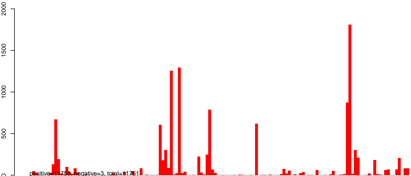
CuQuin_SG_14dpi2.24_35.rep
