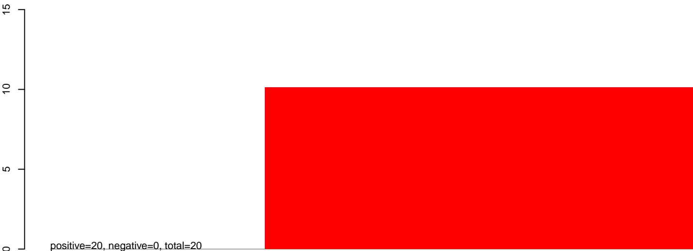
CuQuin_SG_14dpi2.24_35.rep
