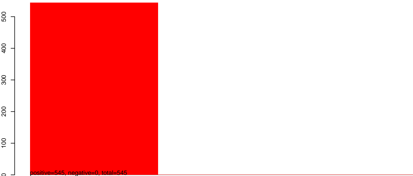
CuQuin_SG_14dpi2.24_35.rep
