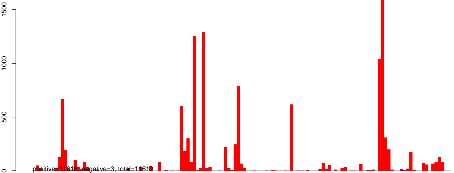
CuQuin_SG_14dpi2.24_35.rep
