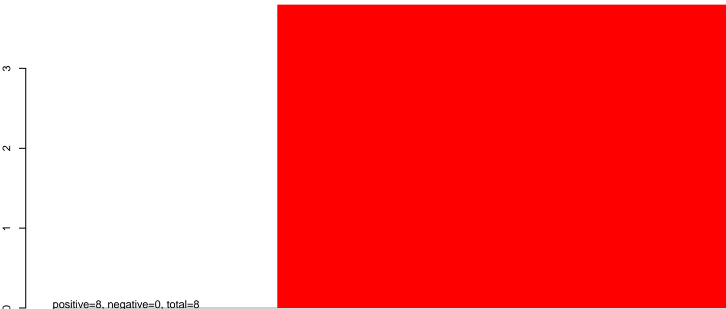
CuQuin_SG_14dpi2.24_35.rep
