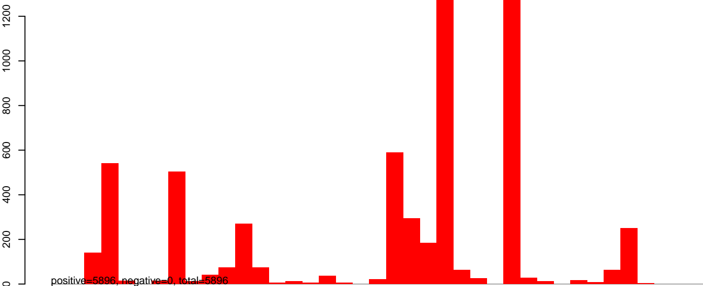
CuQuin_SG_14dpi2.24_35.rep
