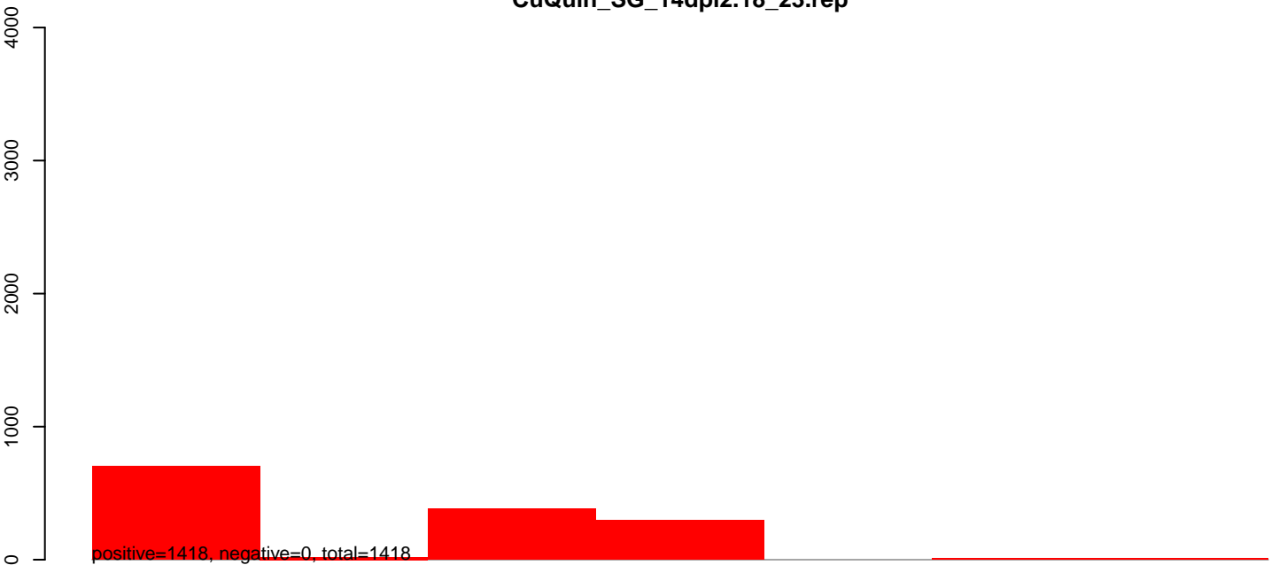
CuQuin_SG_14dpi2.24_35.rep
