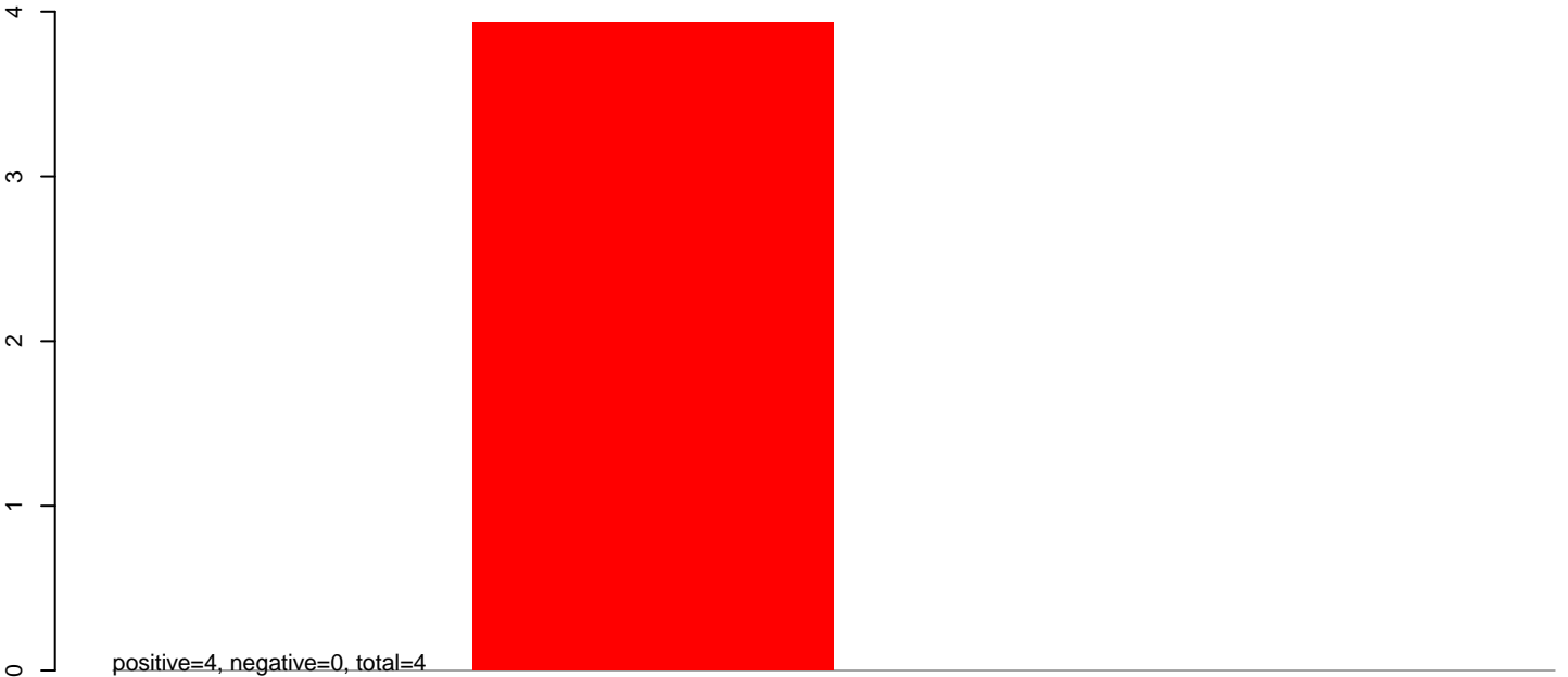
CuQuin_SG_14dpi2.24_35.rep
