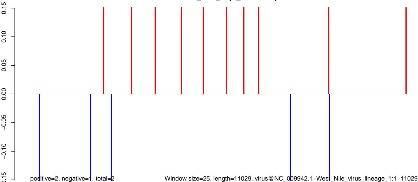
CuQuin_Hsu_2dpi_mock1.rep
