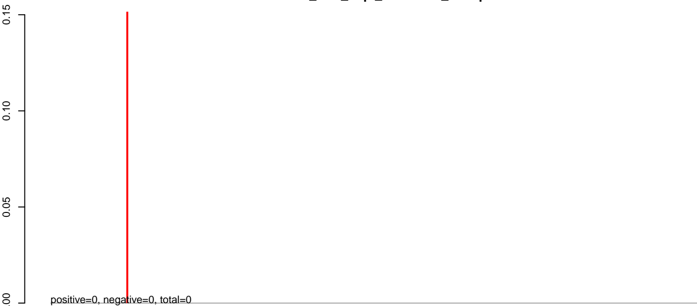
CuQuin_Hsu_2dpi_mock1.24_35.rep
