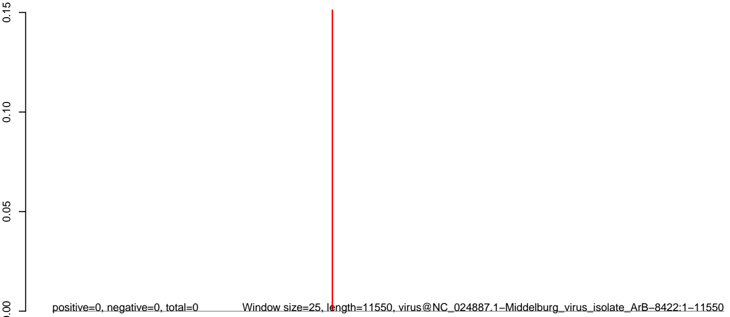
CuQuin_Hsu_2dpi_mock1.rep
