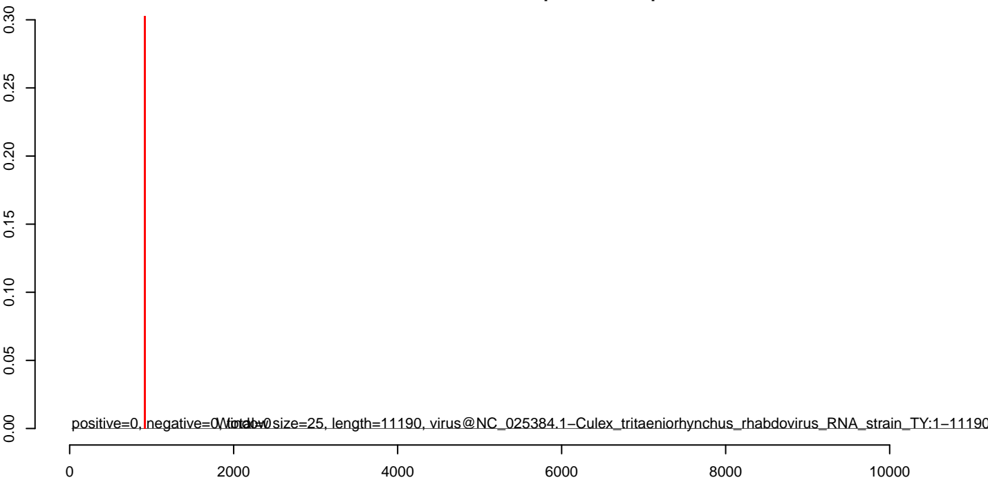
CuQuin_Hsu_2dpi_mock1.rep
