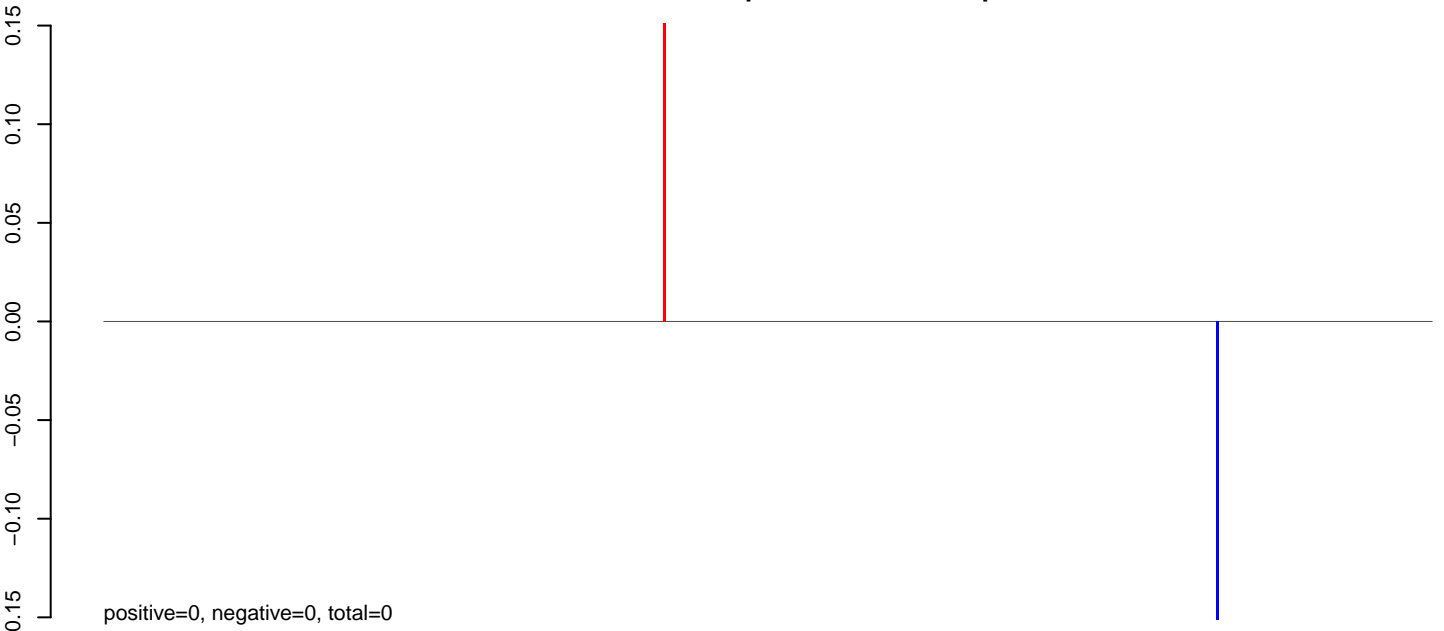
CuQuin_Hsu_2dpi_mock1.24_35.rep
