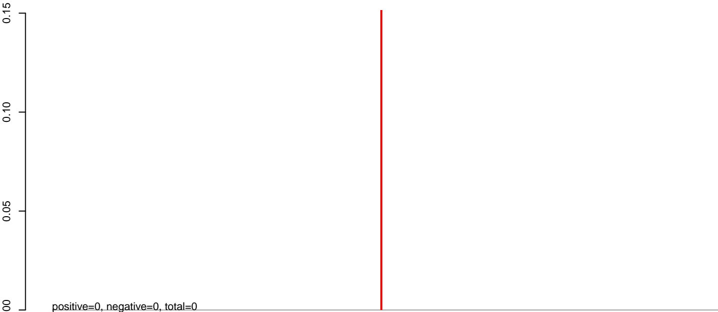
CuQuin_Hsu_2dpi_mock1.24_35.rep
