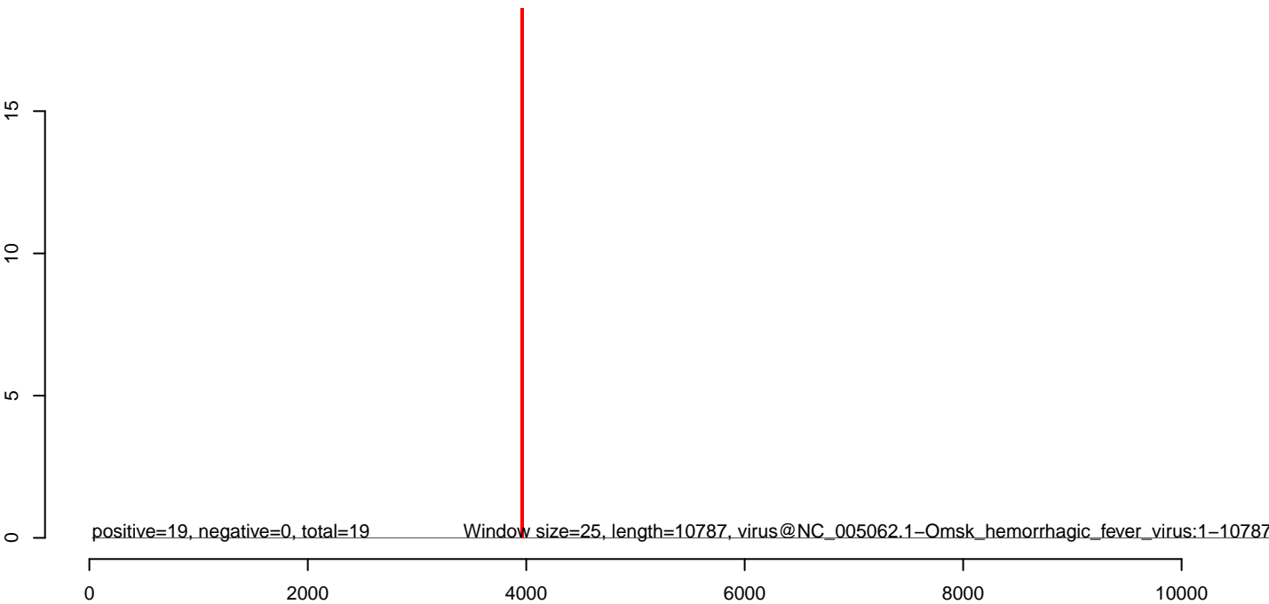
CuQuin_Hsu_2dpi_mock1.rep
