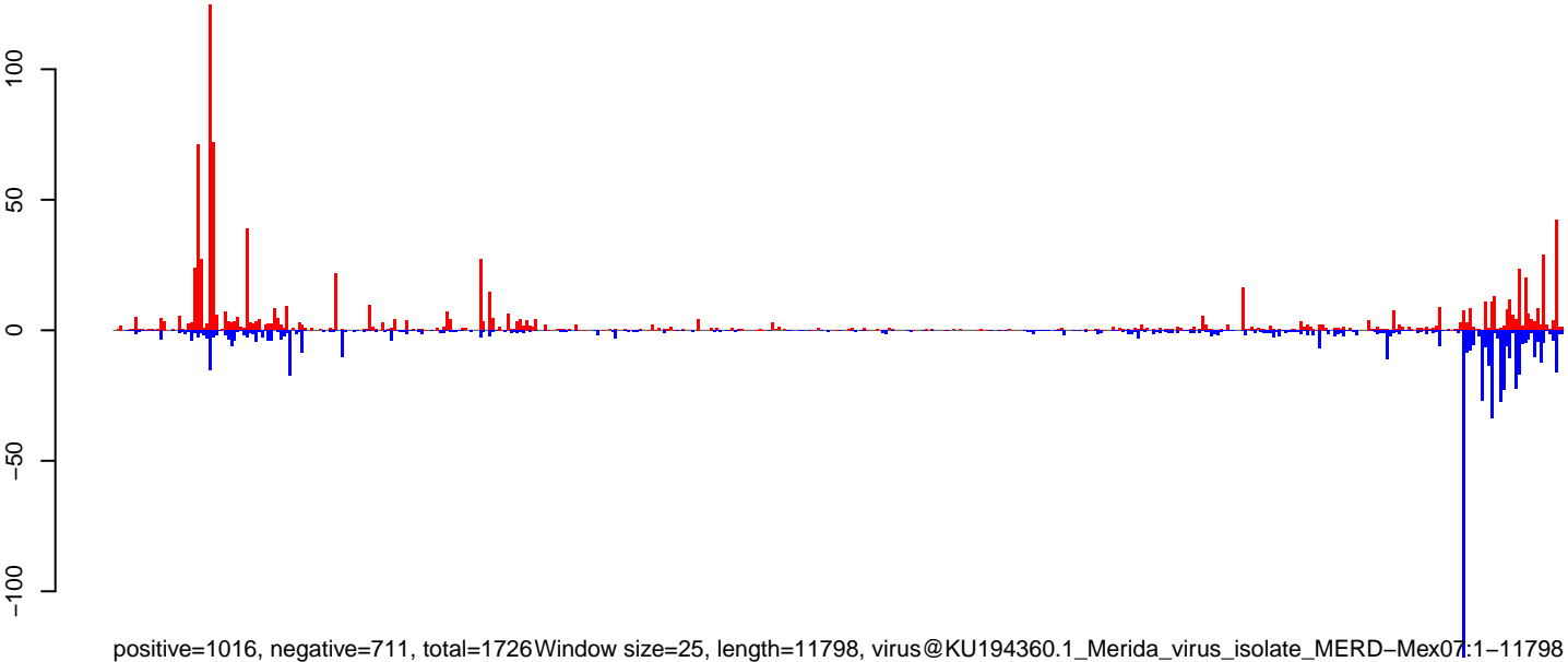
CuQuin_Hsu_2dpi_mock1.rep
