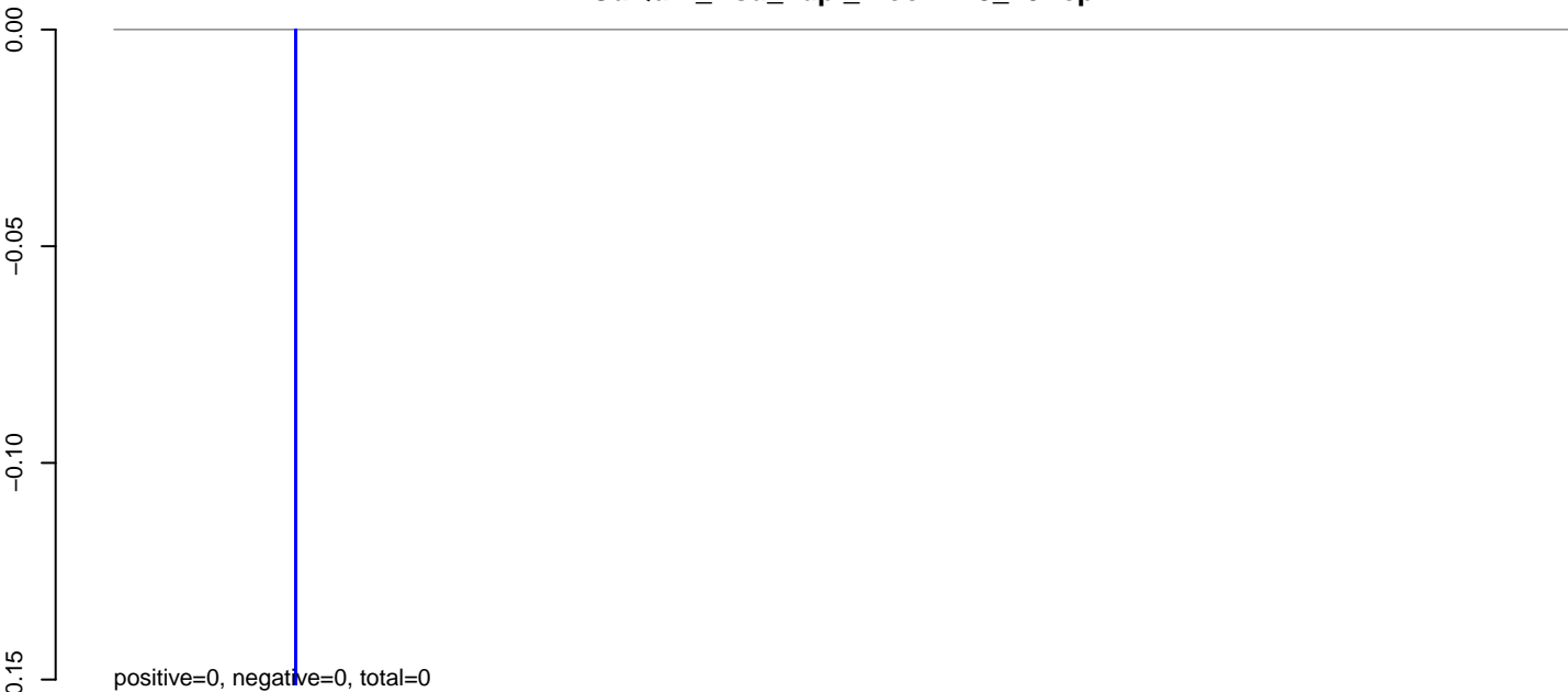
CuQuin_Hsu_2dpi_mock1.24_35.rep
