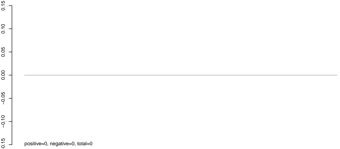
CuQuin_Hsu_2dpi_mock1.rep
