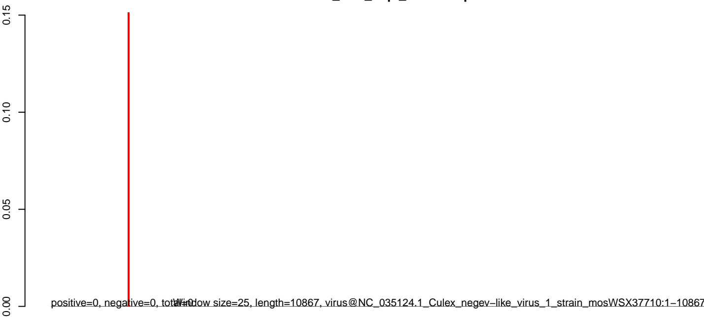
CuQuin_Hsu_2dpi_mock1.rep
