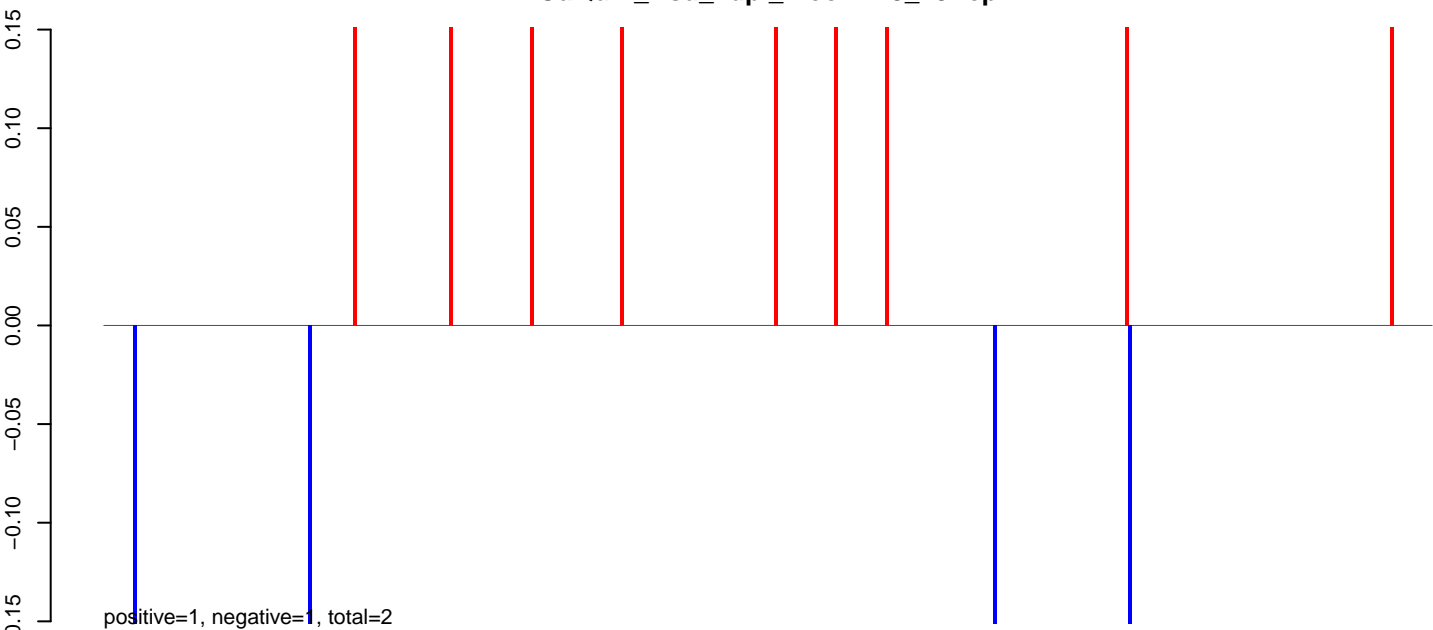
CuQuin_Hsu_2dpi_mock1.24_35.rep
