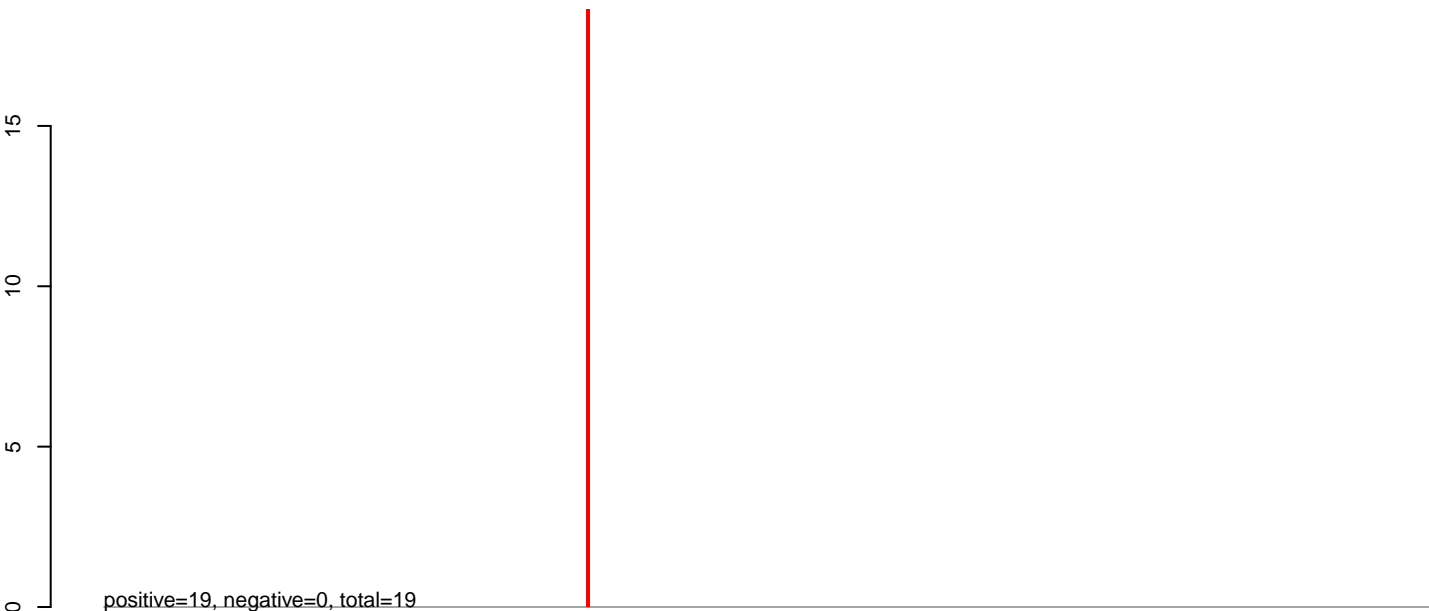
CuQuin_Hsu_2dpi_mock1.24_35.rep
