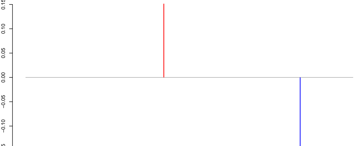
CuQuin_Hsu_2dpi_mock1.rep
