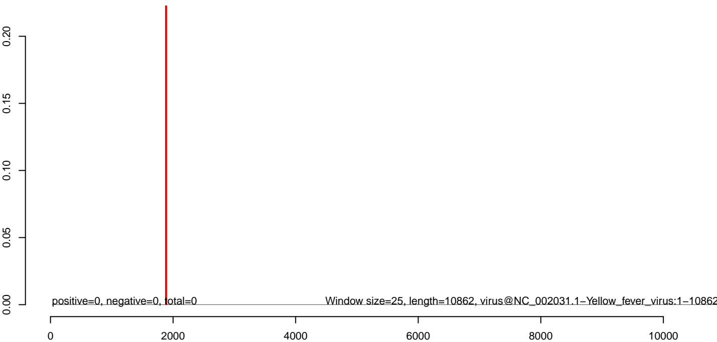
CuQuin_Hsu_6dpi_mock1.rep
