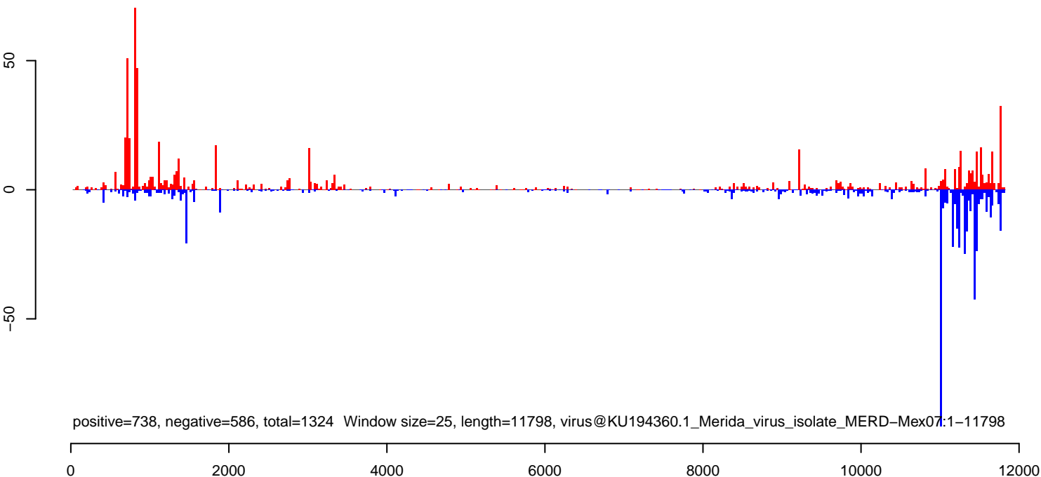
CuQuin_Hsu_6dpi_mock1.rep
