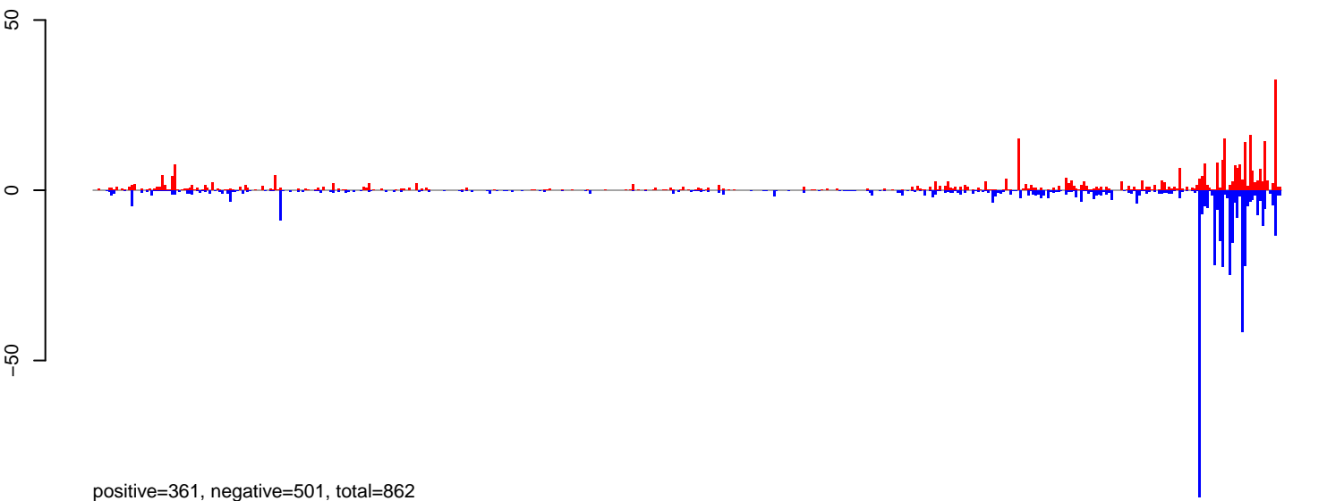
CuQuin_Hsu_6dpi_mock1.24_35.rep
