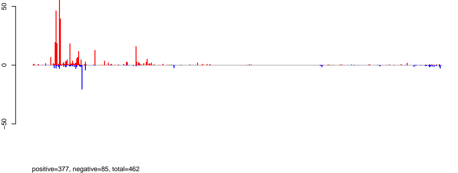
CuQuin_Hsu_6dpi_mock1.rep
