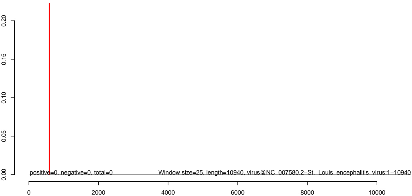
CuQuin_Hsu_6dpi_mock1.rep
