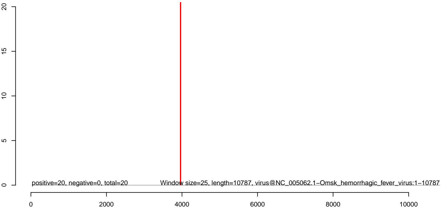
CuQuin_Hsu_6dpi_mock1.rep
