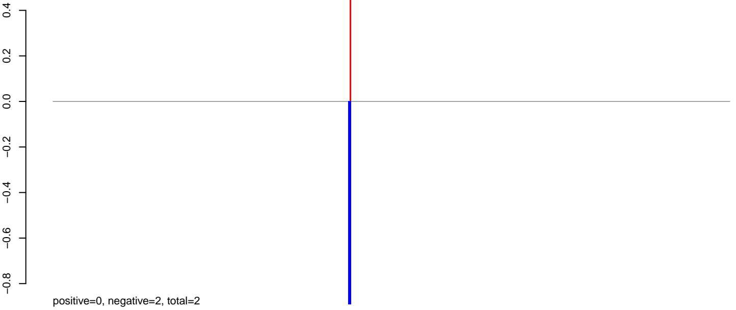
CuQuin_Hsu_6dpi_mock1.24_35.rep
