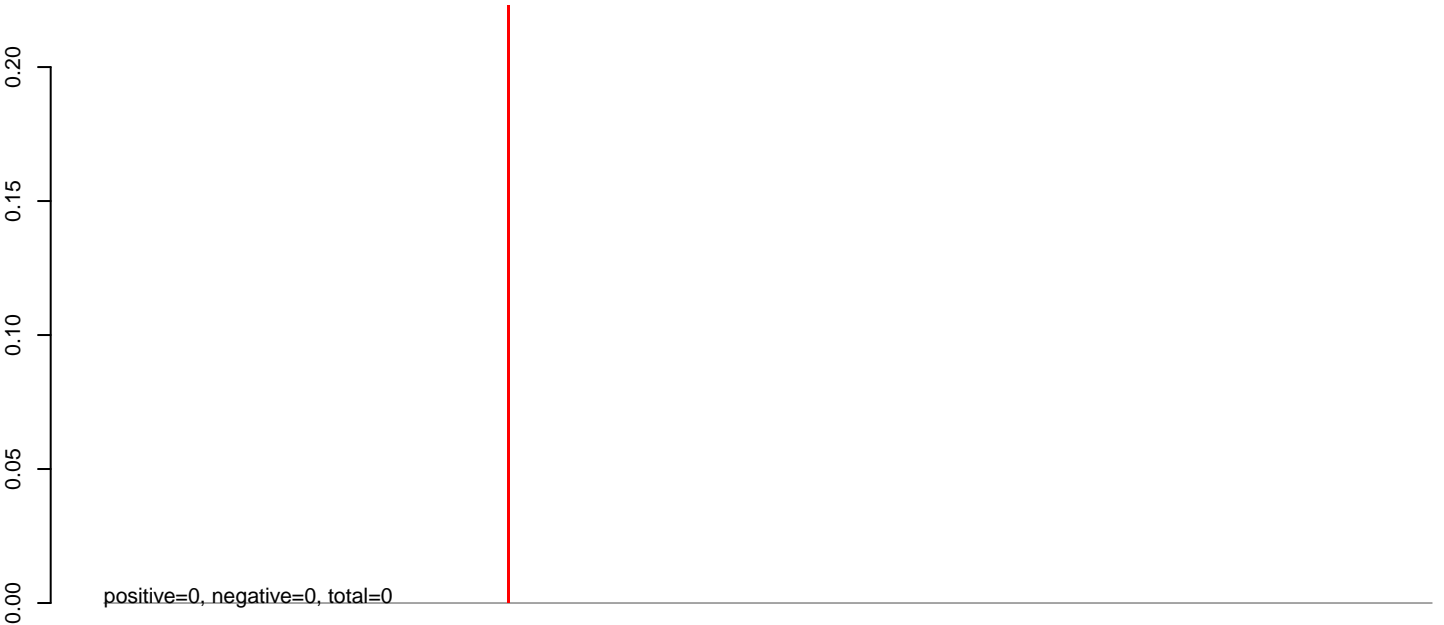
CuQuin_Hsu_6dpi_mock1.24_35.rep
