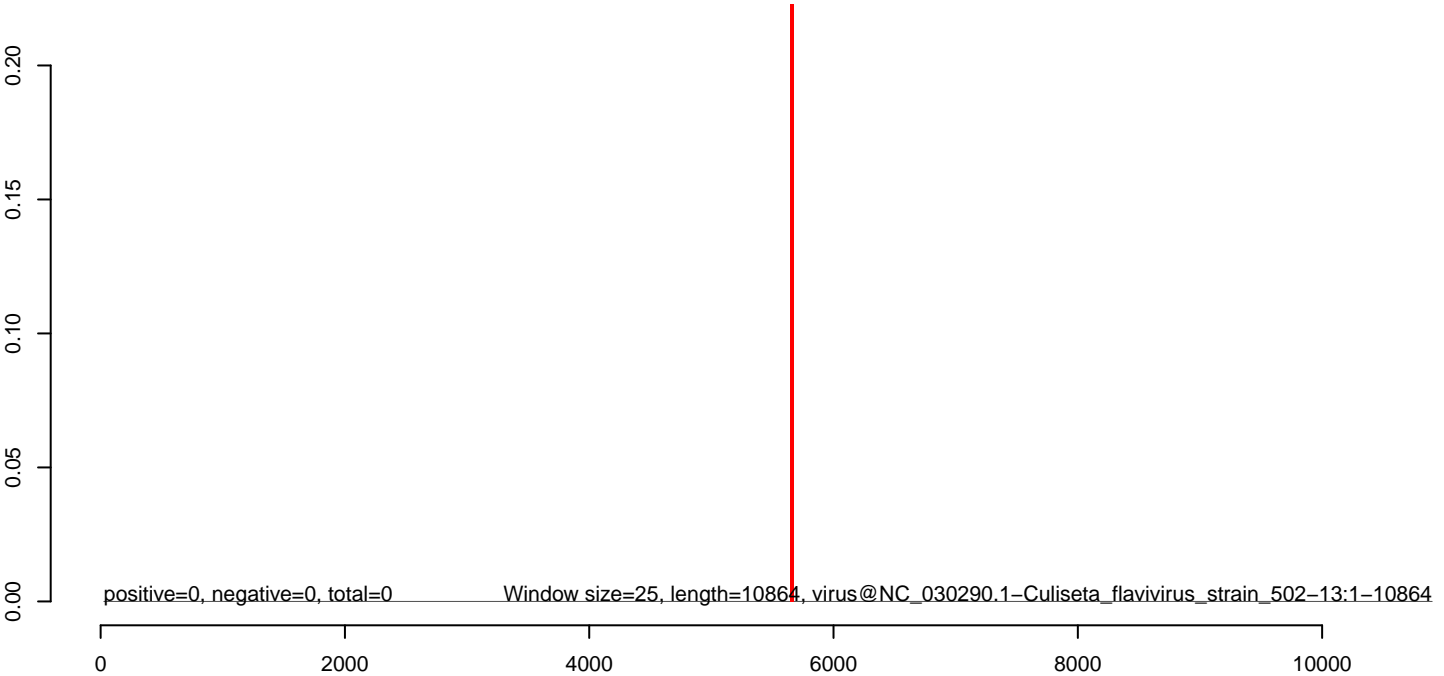
CuQuin_Hsu_6dpi_mock1.rep
