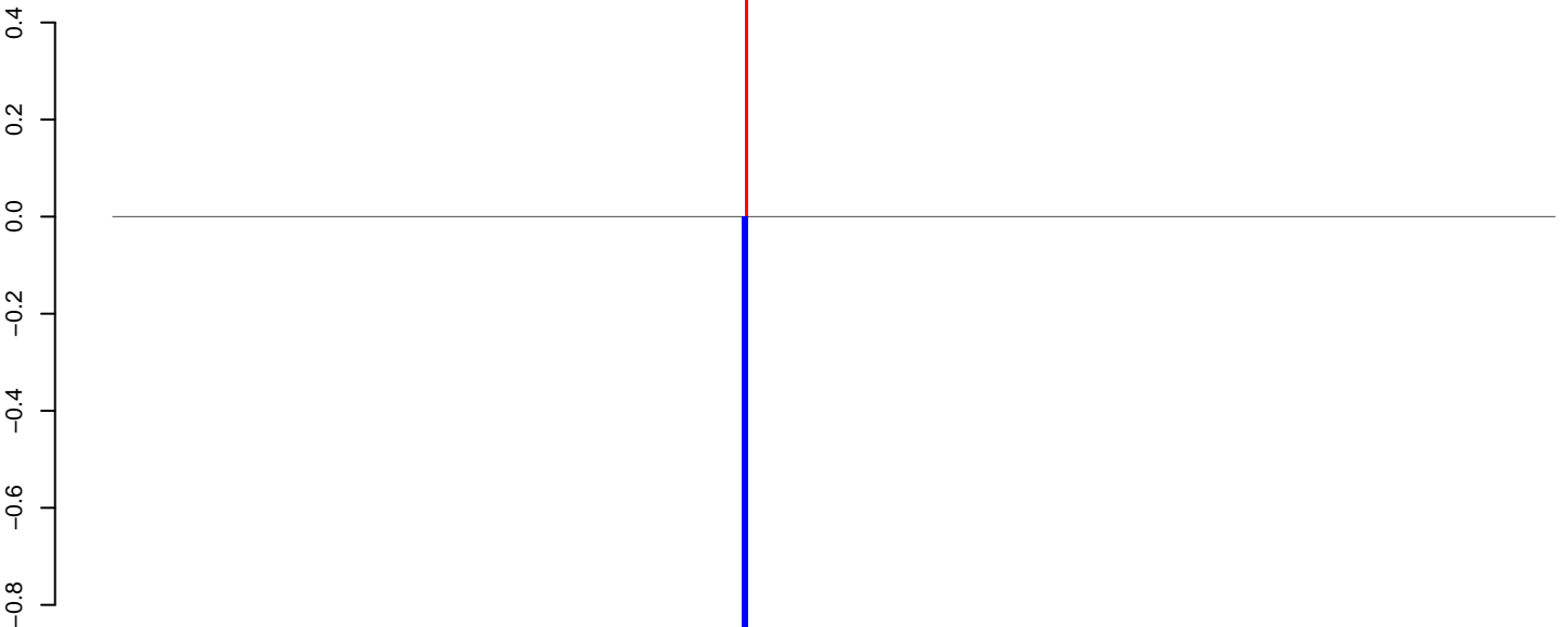
CuQuin_Hsu_6dpi_mock1.rep
