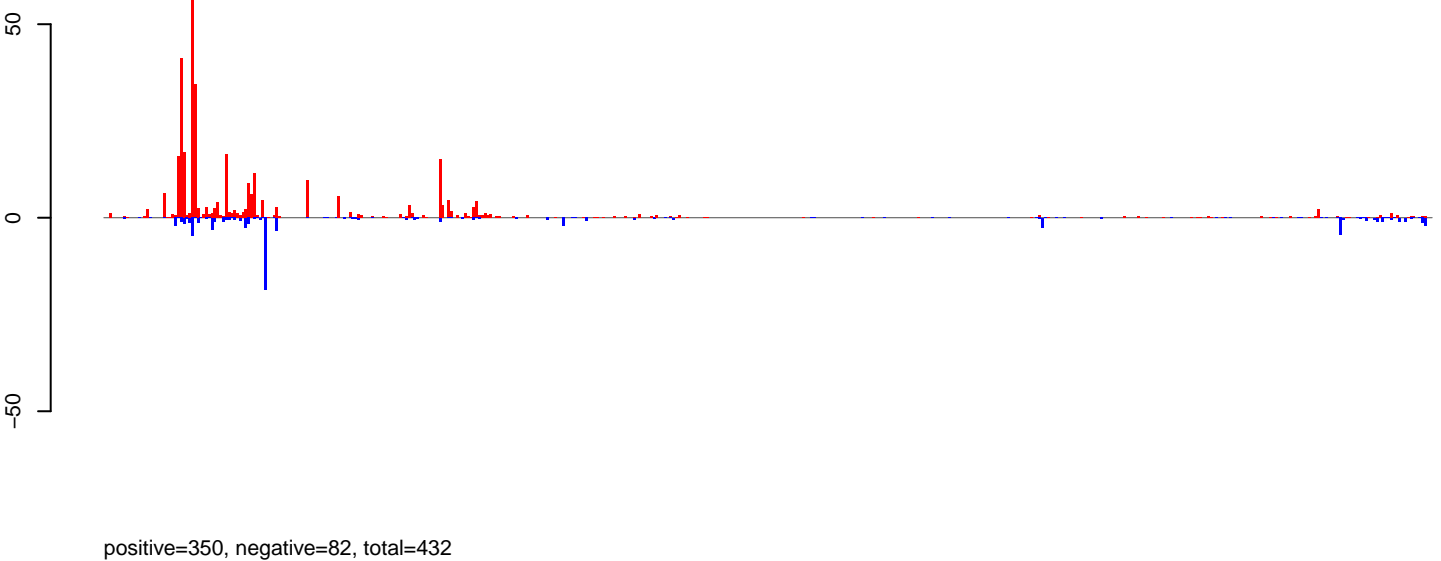
CuQuin_Hsu_6dpi_mock2.rep
