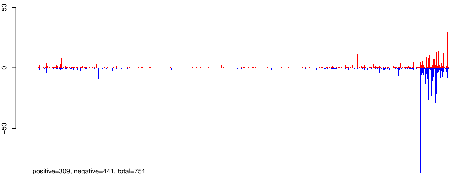
CuQuin_Hsu_6dpi_mock2.24_35.rep
