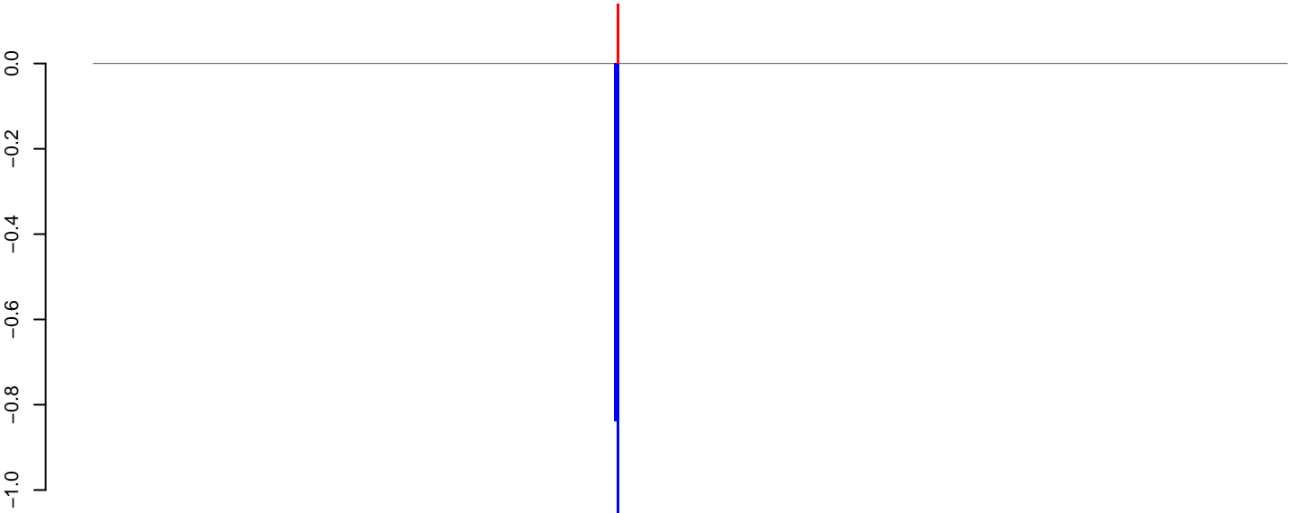
CuQuin_Hsu_6dpi_mock2.rep
