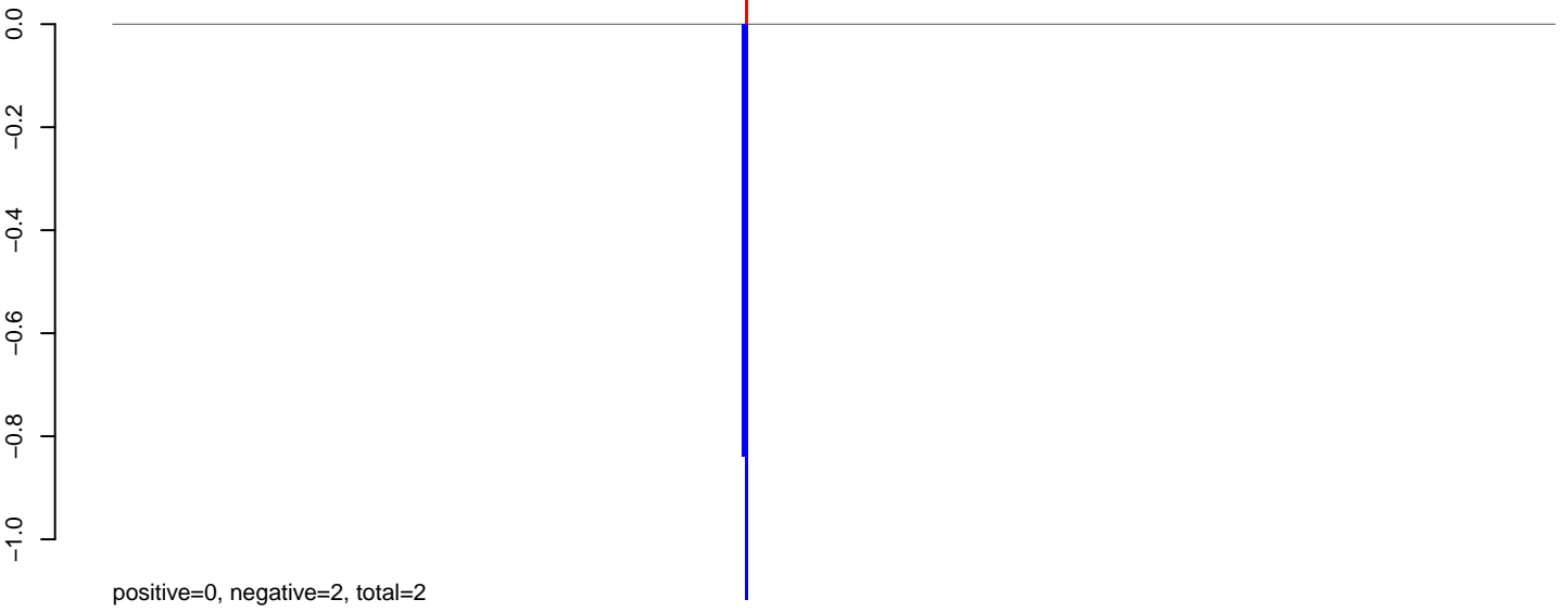
CuQuin_Hsu_6dpi_mock2.24_35.rep
