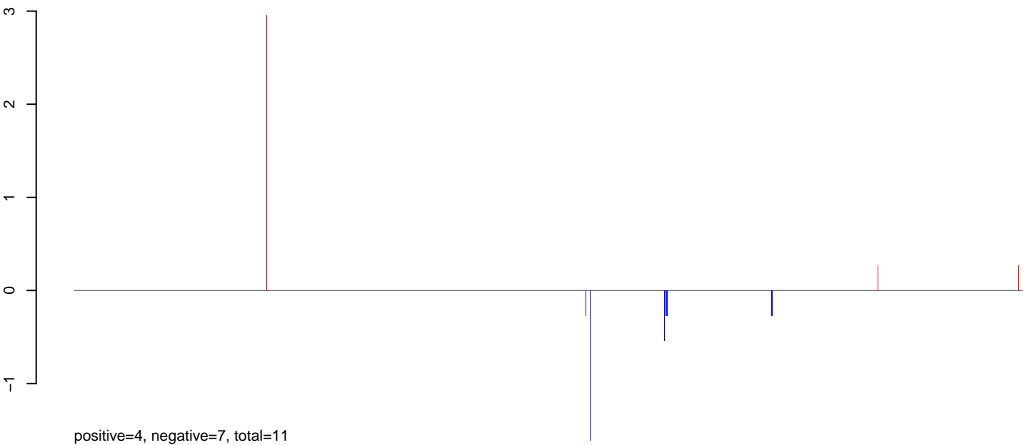
CuQuin_Hsu_30dpi_WNV2.24_35.rep
