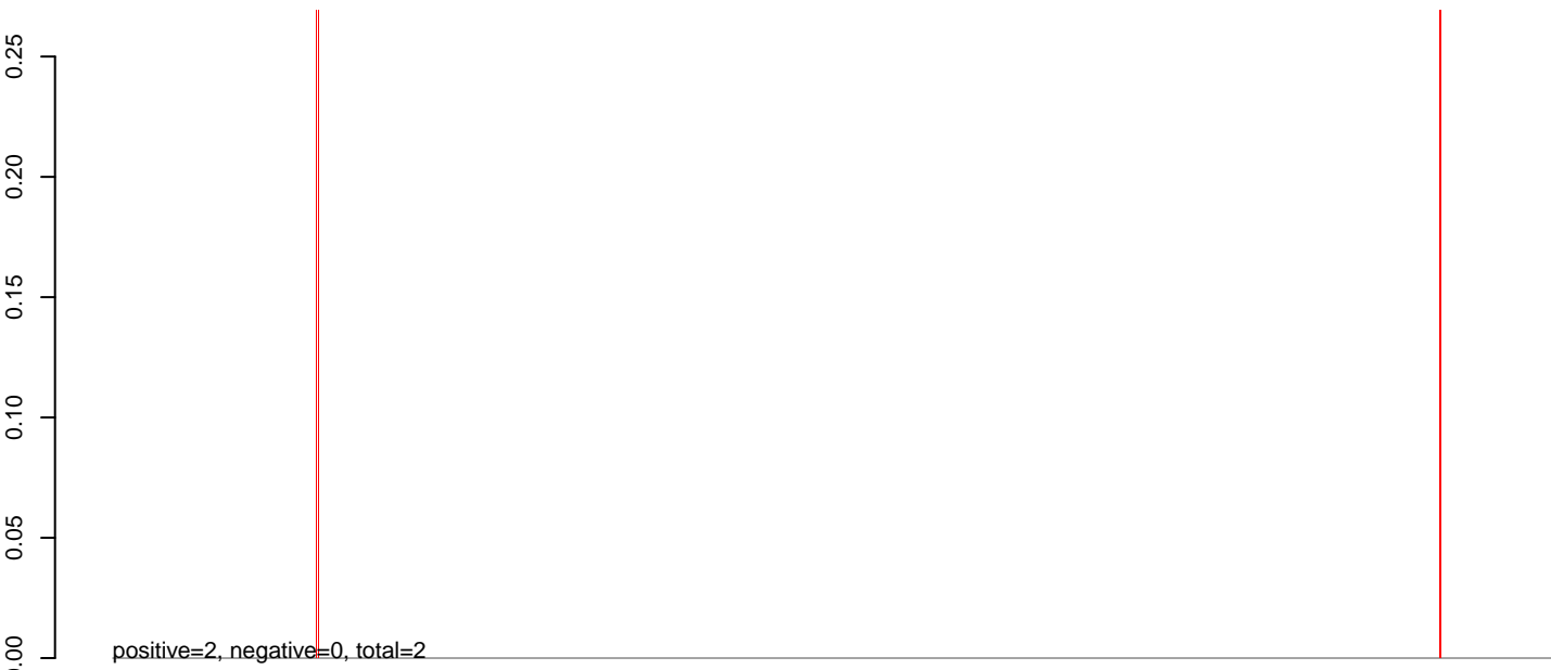
CuQuin_Hsu_30dpi_WNV2.24_35.rep
