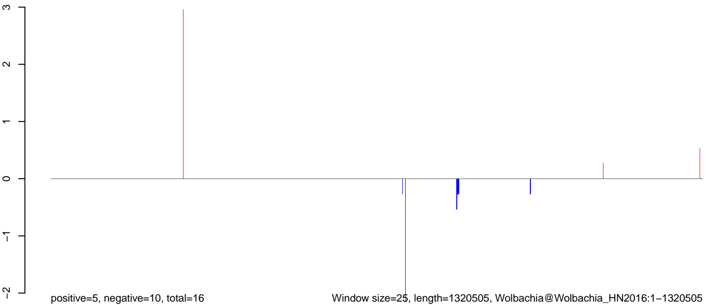
CuQuin_Hsu_30dpi_WNV2.rep
