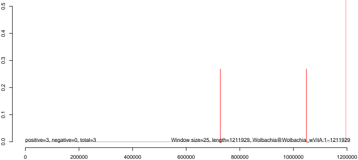
CuQuin_Hsu_30dpi_WNV2.rep
