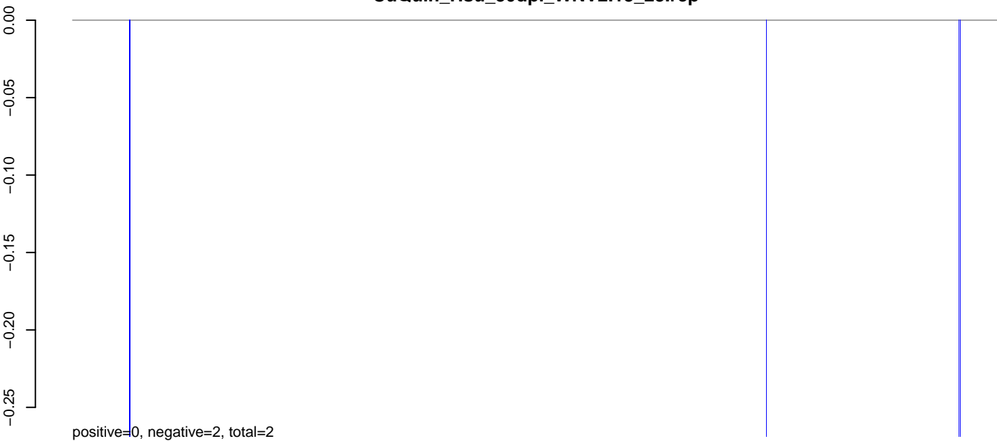
CuQuin_Hsu_30dpi_WNV2.24_35.rep
