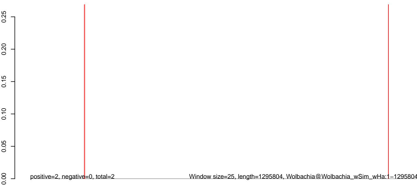
CuQuin_Hsu_30dpi_WNV2.rep
